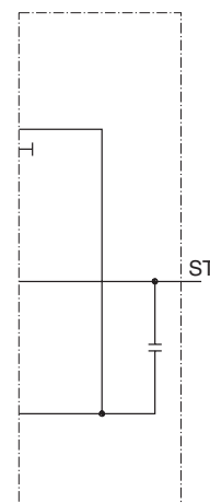
Tank connection T1 open. Free-flow gallery not connected with tank (series connected). ST at item [33].
