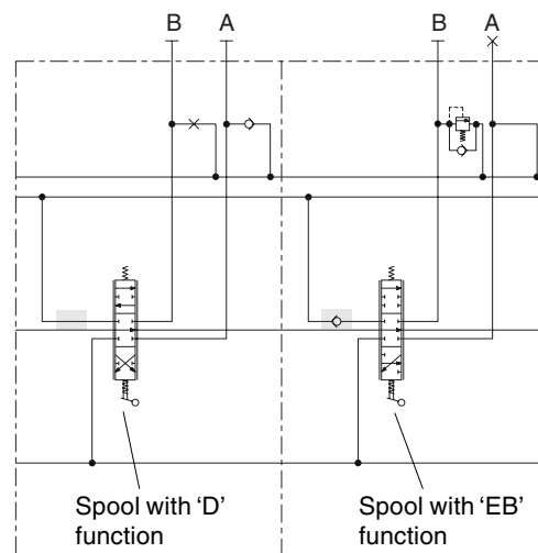
Pressure gallery open (X) in first section and fitted with check valve (N) in second section.
