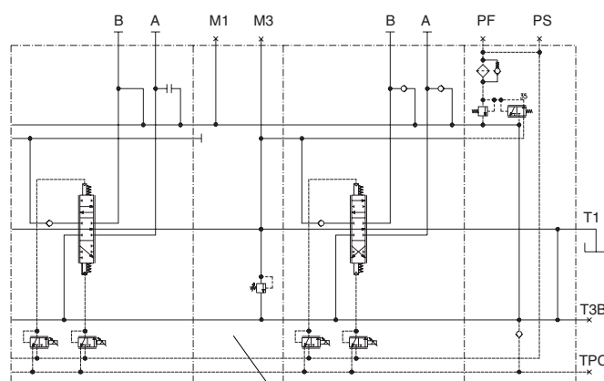
Mid-inlet section
