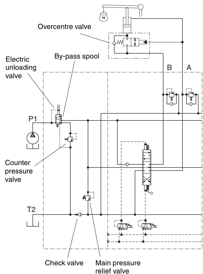
Circuit diagram for pump unloading
