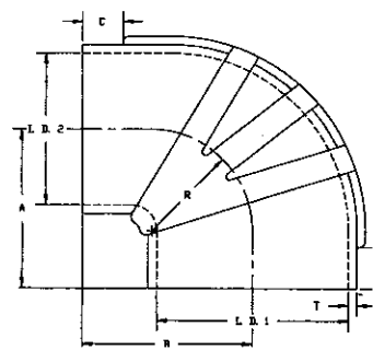
90° Reducing Elbow
