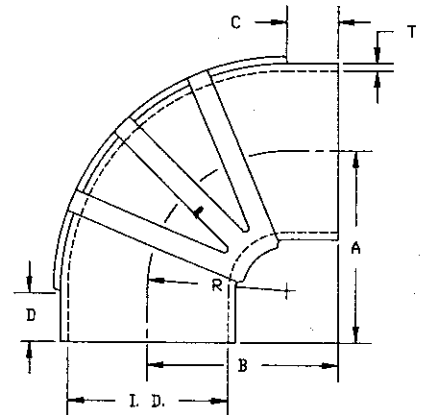
90° Elbow
