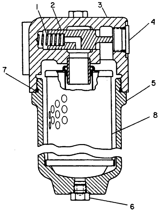
GY3557 FILTER GP-TRANSMISSION An Attachment
