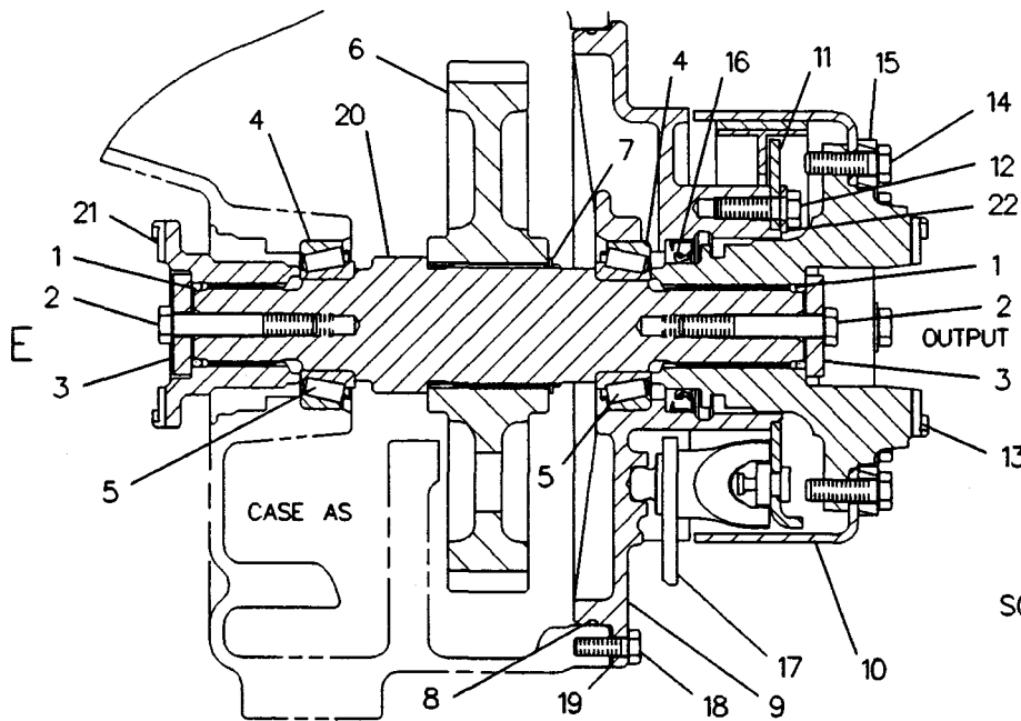
GY0235 GEAR GP-OUTPUT
