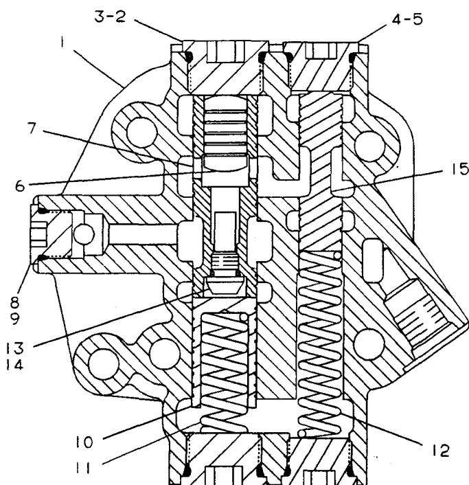
GY7622 VALVE GP-DUMP An Attachment
