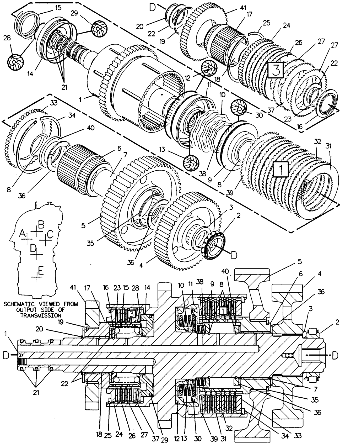
KW6884 CLUTCH GP No. 1 & 3
