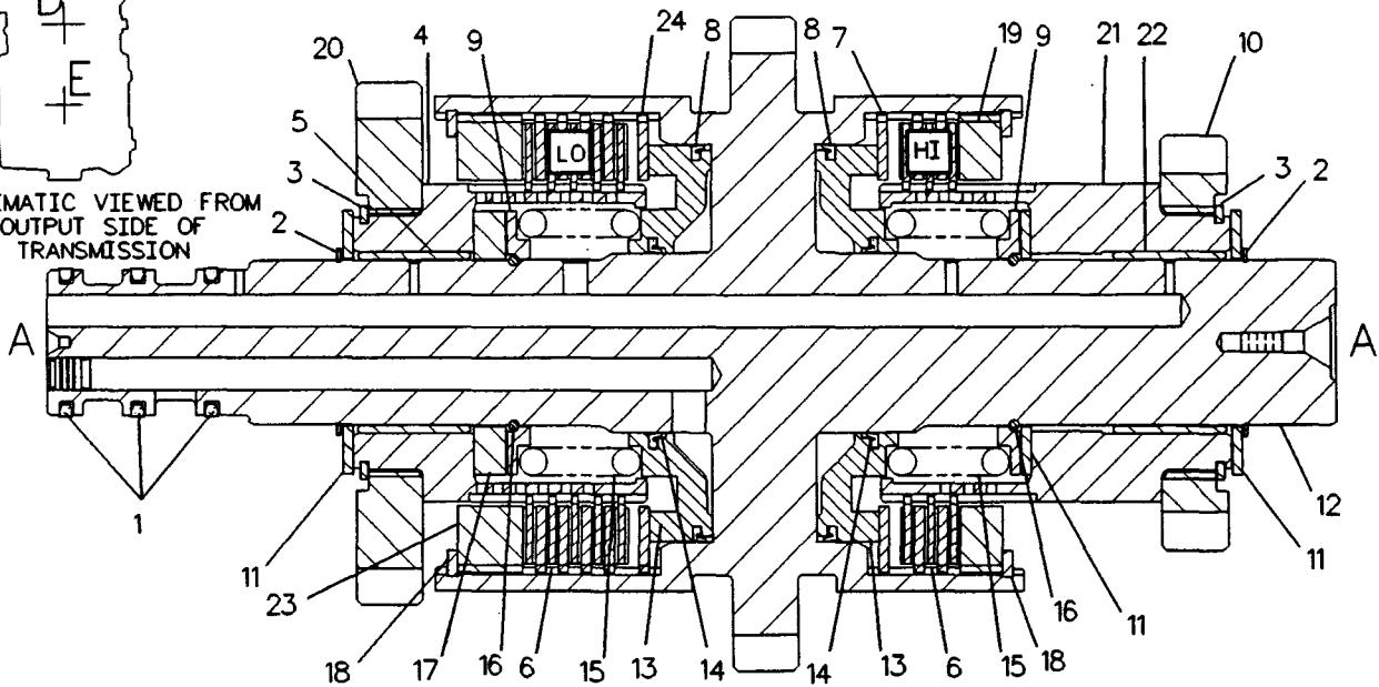
KW7726 CLUTCH GP Forward Low & Forward High
