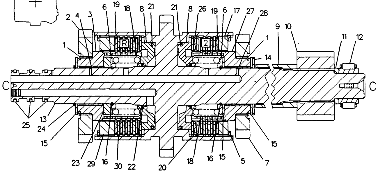
KW6883 CLUTCH GP Reverse & No. 2
