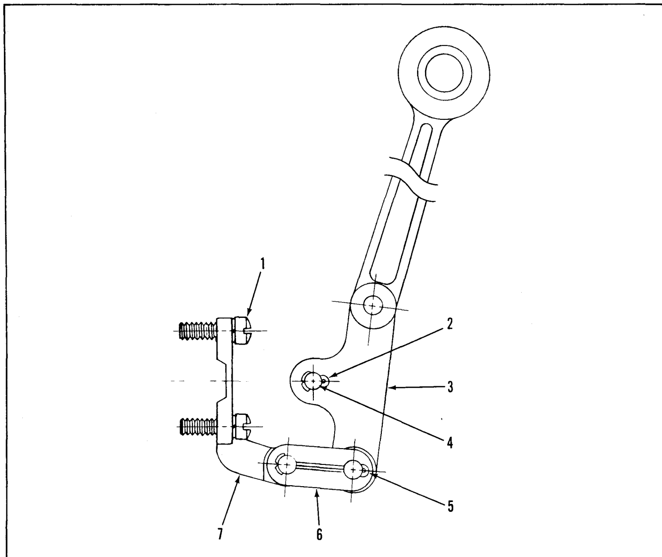
Figure 4-20. Vertical Handle
