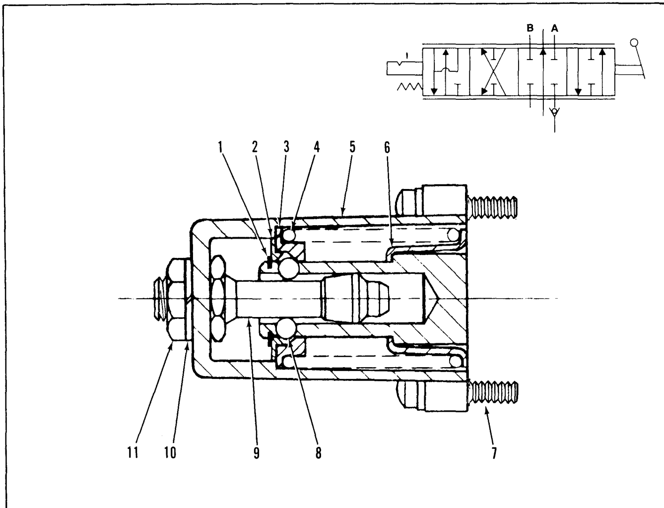
Figure 4-15. Float Positioner
