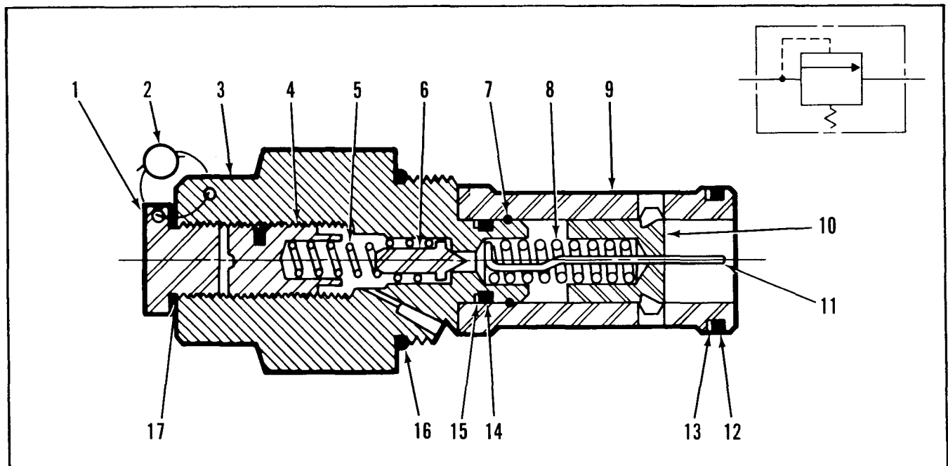
Figure 4-26. Model DPK Relief Valve
