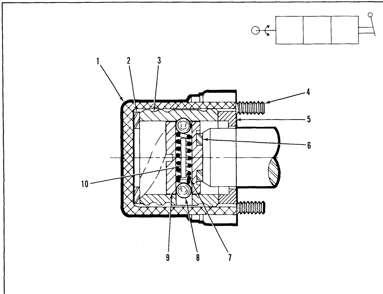
Figure 4-16. Rotary Positioner
