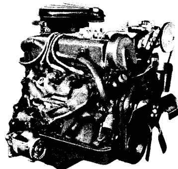
LSG-423 & LSG 633 4 & 6-Cylinder, Gasoline 2.3 Litre and 3.3 Litre
