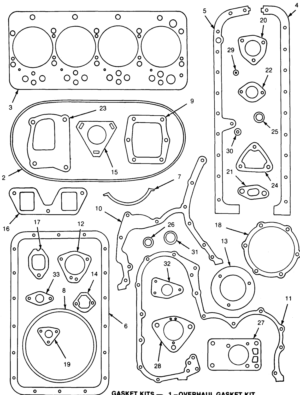
GASKET KITS — 1 — OVERHAUL GASKET KIT 34 — VALVE GRIND GASKET KIT
