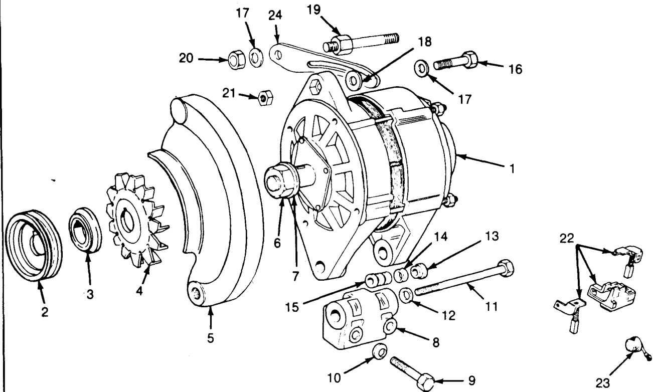
ALTERNATOR, BRACKETS AND RELATED PARTS
