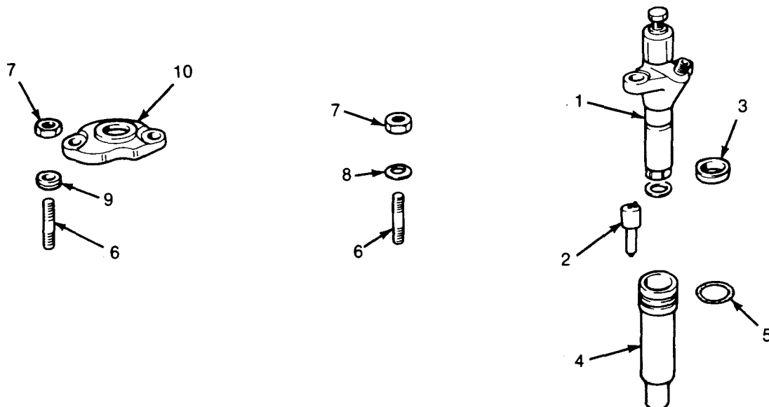
FUEL INJECTOR ASSEMBLY
