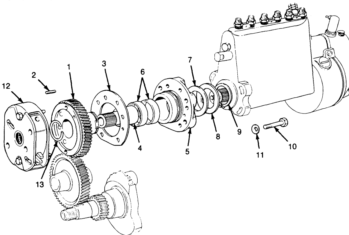
INLINE INJECTION PUMP DRIVE AND RELATED PARTS
