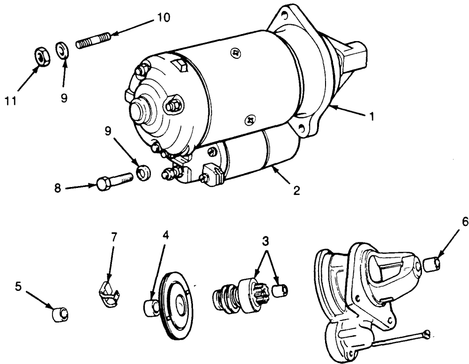
STARTING MOTOR ASSEMBLY
