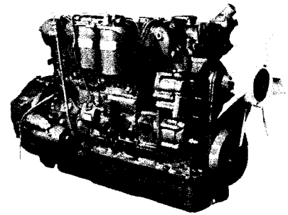
SSD-681 6 Cylinder 8.1 Litre, 495 CID
