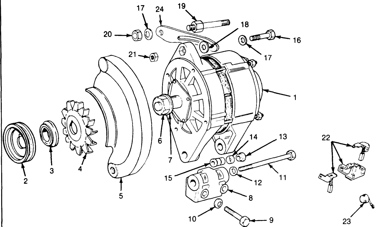
ALTERNATOR, BRACKETS AND RELATED PARTS
