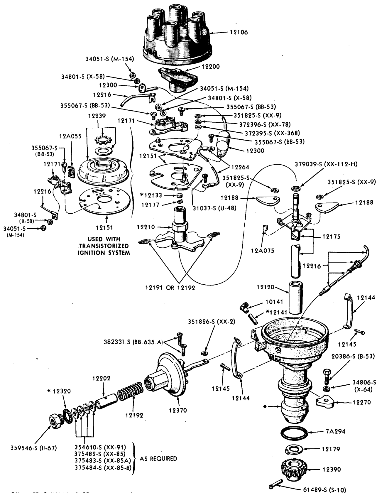
DUAL ADVANCE DISTRIBUTOR – TYPICAL
