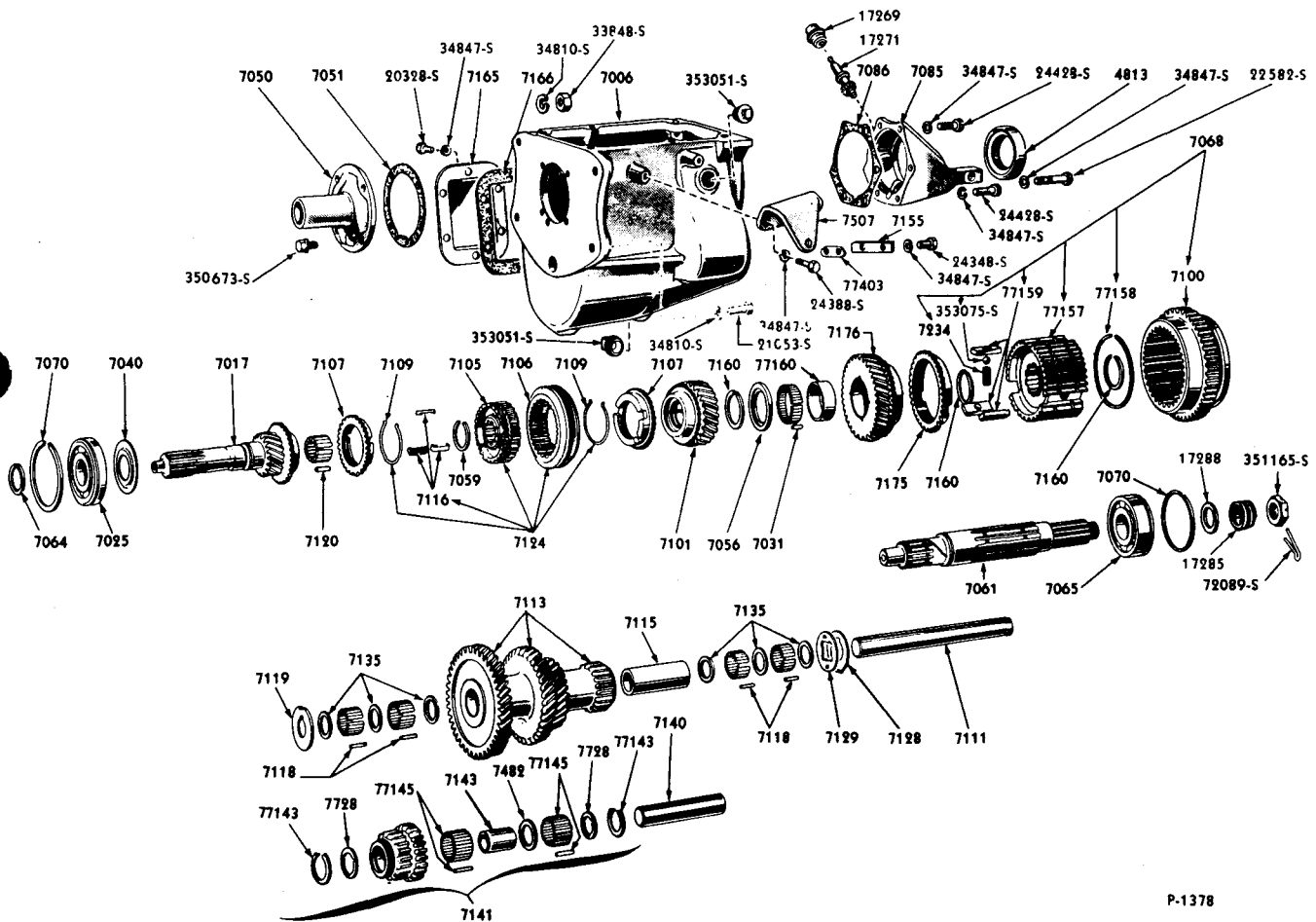
TYPICAL 4 SPEED HELICAL SYNCHRONIZED TRANSMISSION—JE-7000-A
