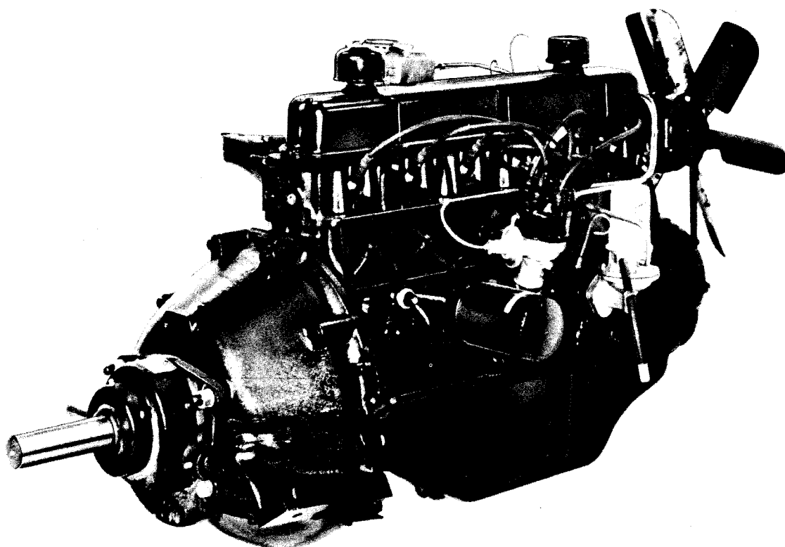
LEFT - REAR VIEW HIGH MOUNTED FAN
