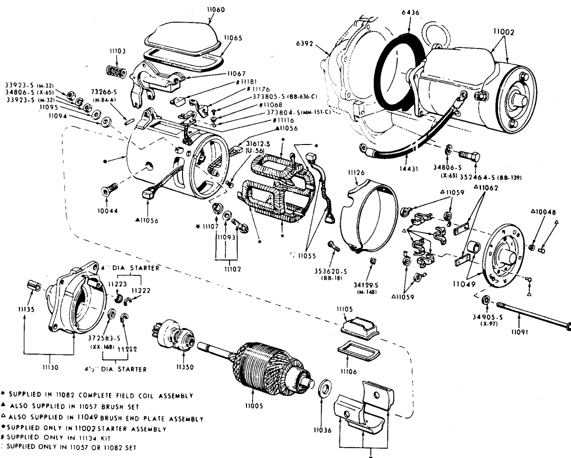
STARTER & DRIVE ASSEMBLY (FORD 12 VOLT)
