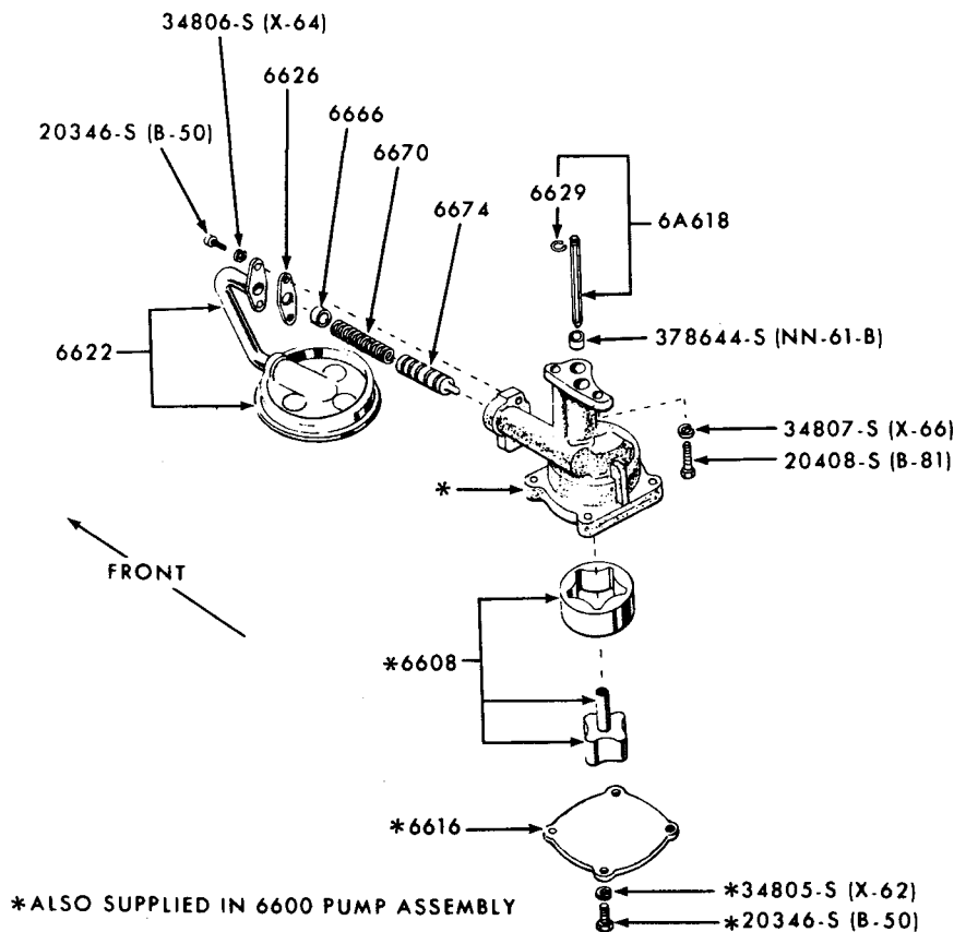
ENGINE OIL PUMP & RELATED PARTS
