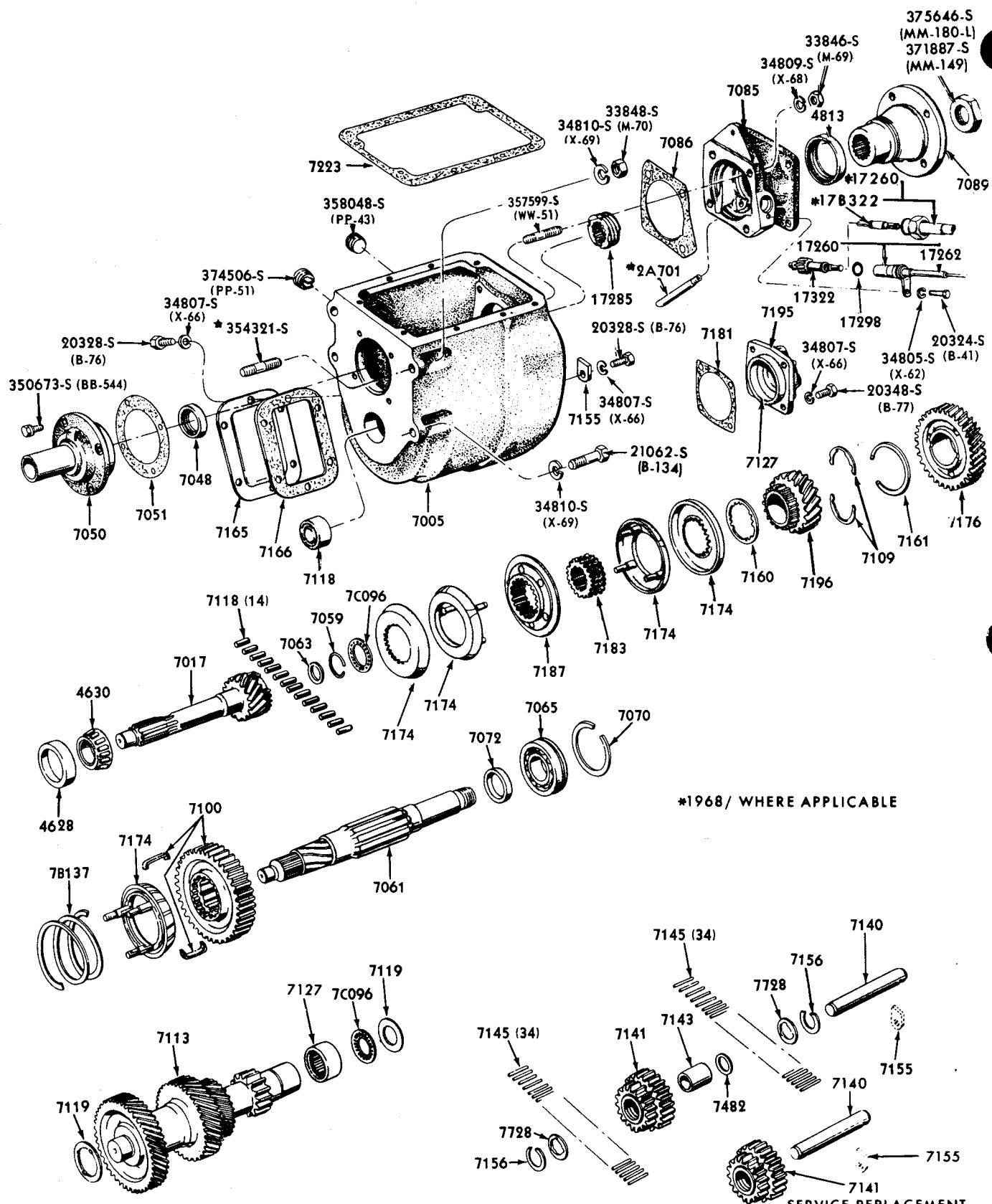
TRANSMISSION-4 SPEED SYNCHRO. HELICAL GEAR (NEW PROCESS 435)-D1TZ-7004-A SERVICE REPLACEMENT REVERSE IDLER GEAR ASSEMBLY
