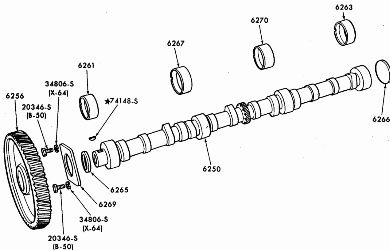
ENGINE CAMSHAFT, GEAR, BEARINGS & RELATED PARTS – TYPICAL
