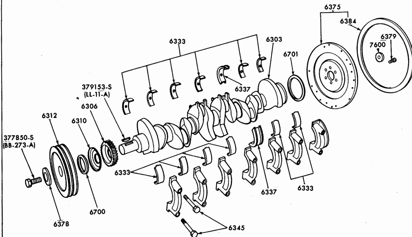
ENGINE CRANKSHAFT, FLYWHEEL & RELATED PARTS - TYPICAL
