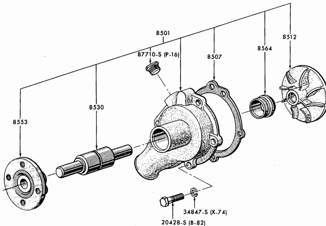
WATER PUMP
