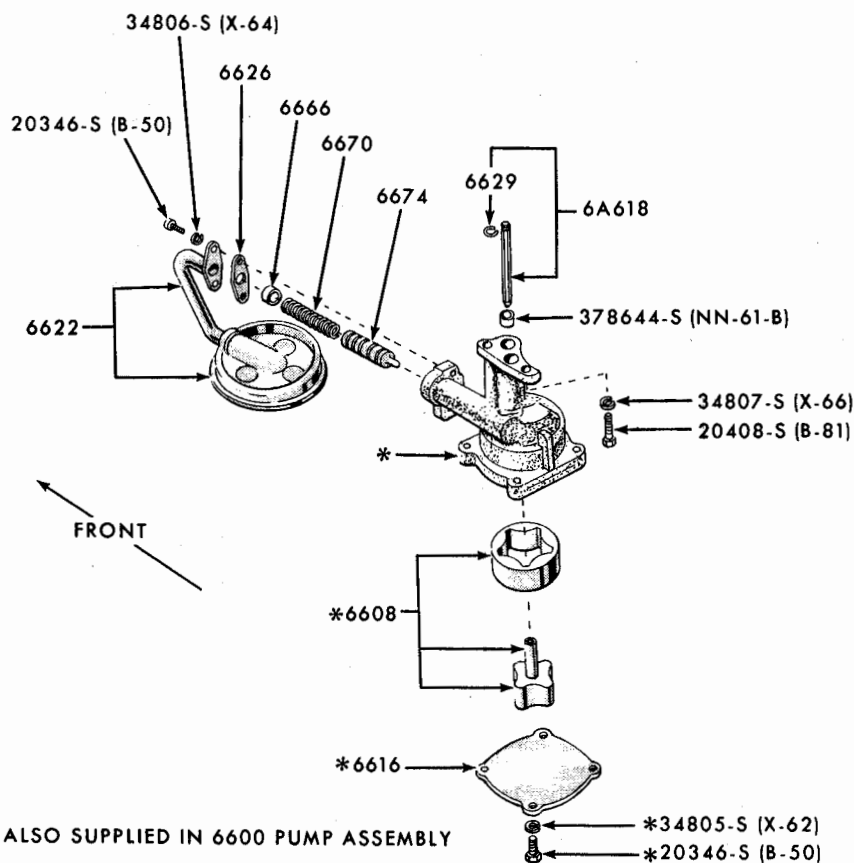
ENGINE OIL PUMP & RELATED PARTS
