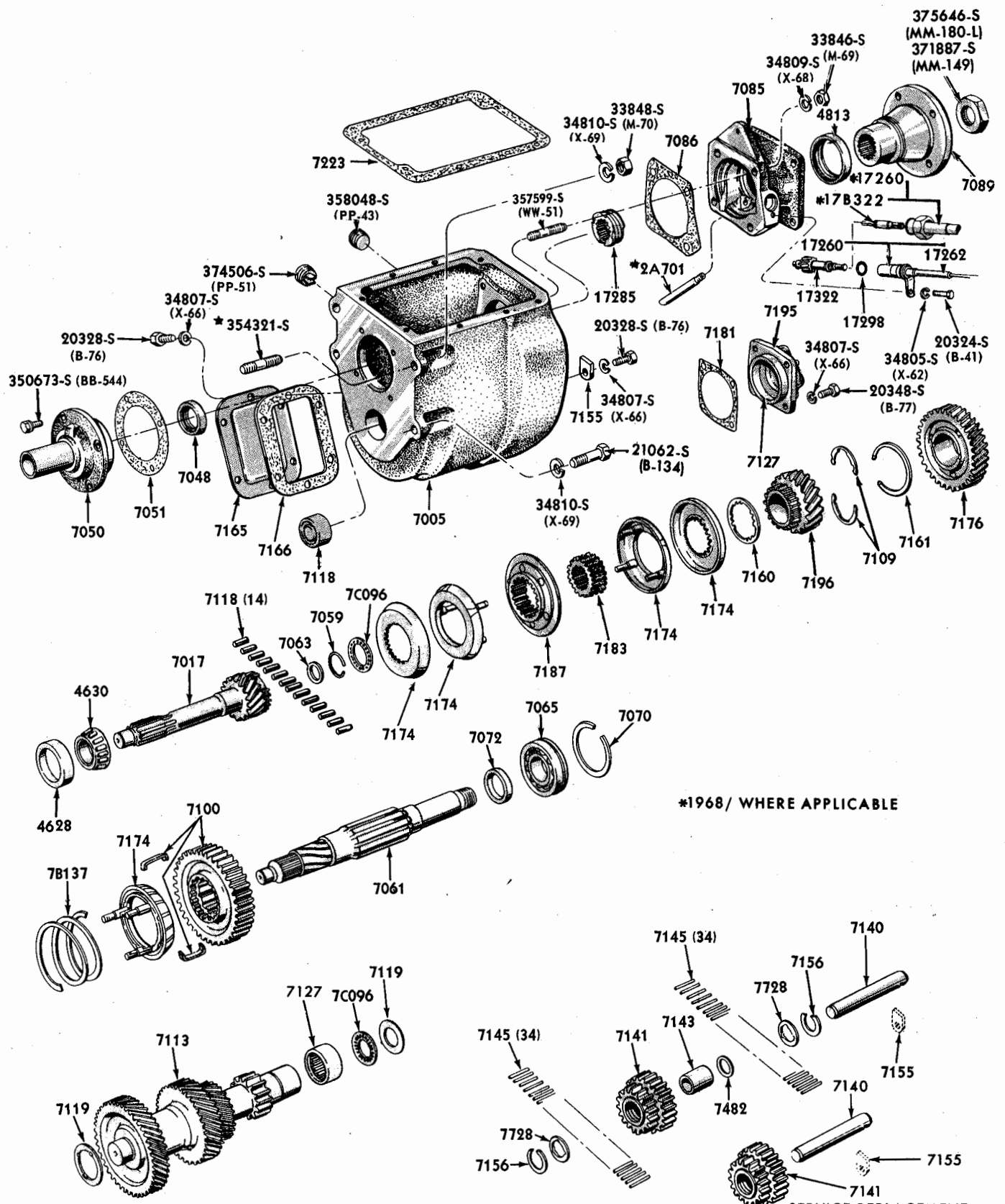
TRANSMISSION-4 SPEED SYNCHRO. HELICAL GEAR (NEW PROCESS 435)-D1TZ-7004-A
