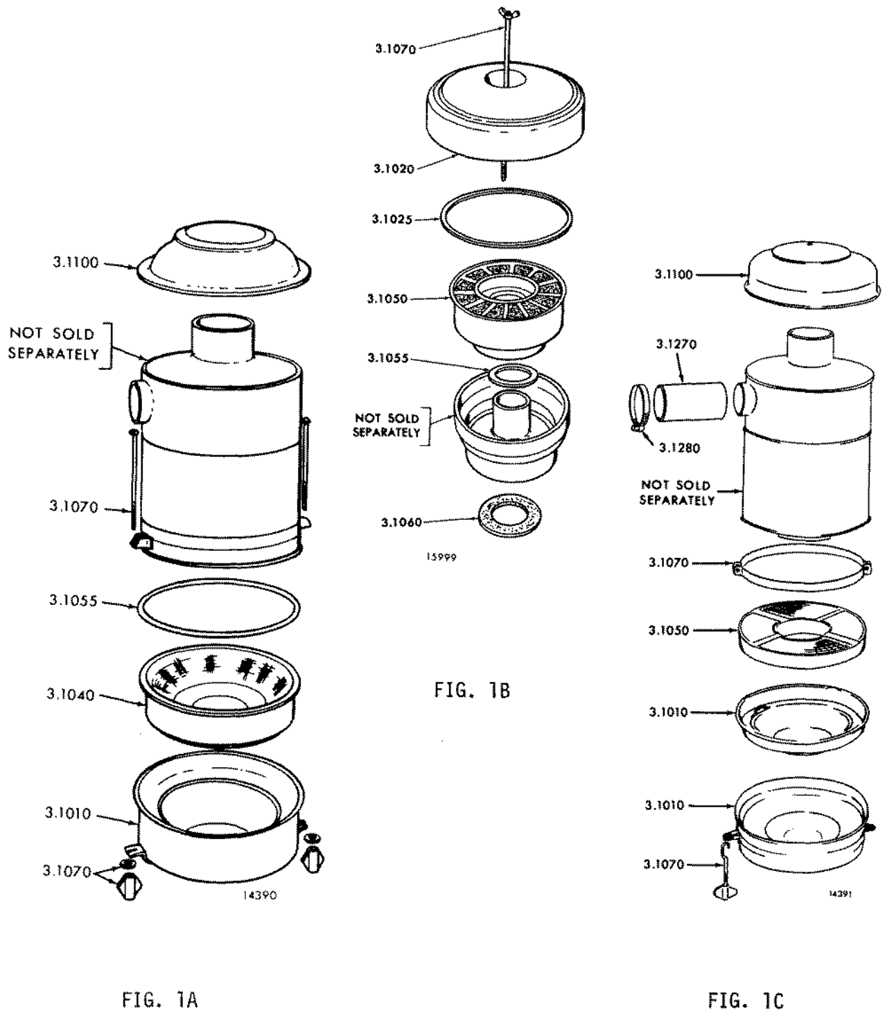
AIR CLEANER
