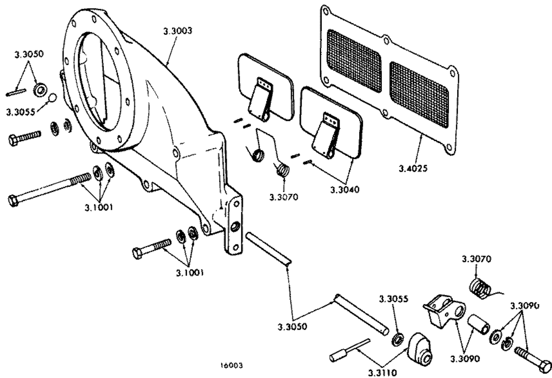
FIG. 3C AIR INLET HOUSING (6V-53)
