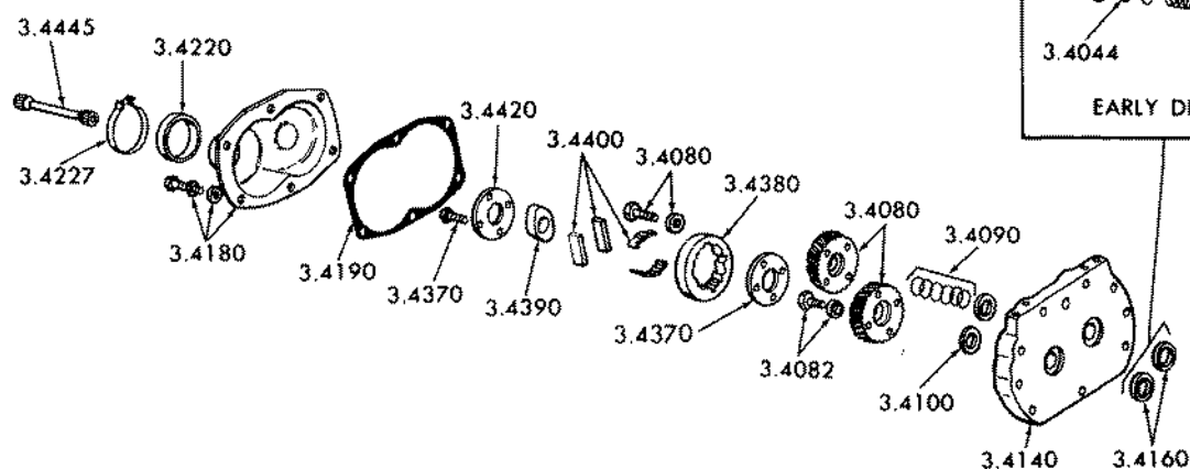
FIG. 4C BLOWER DRIVE
