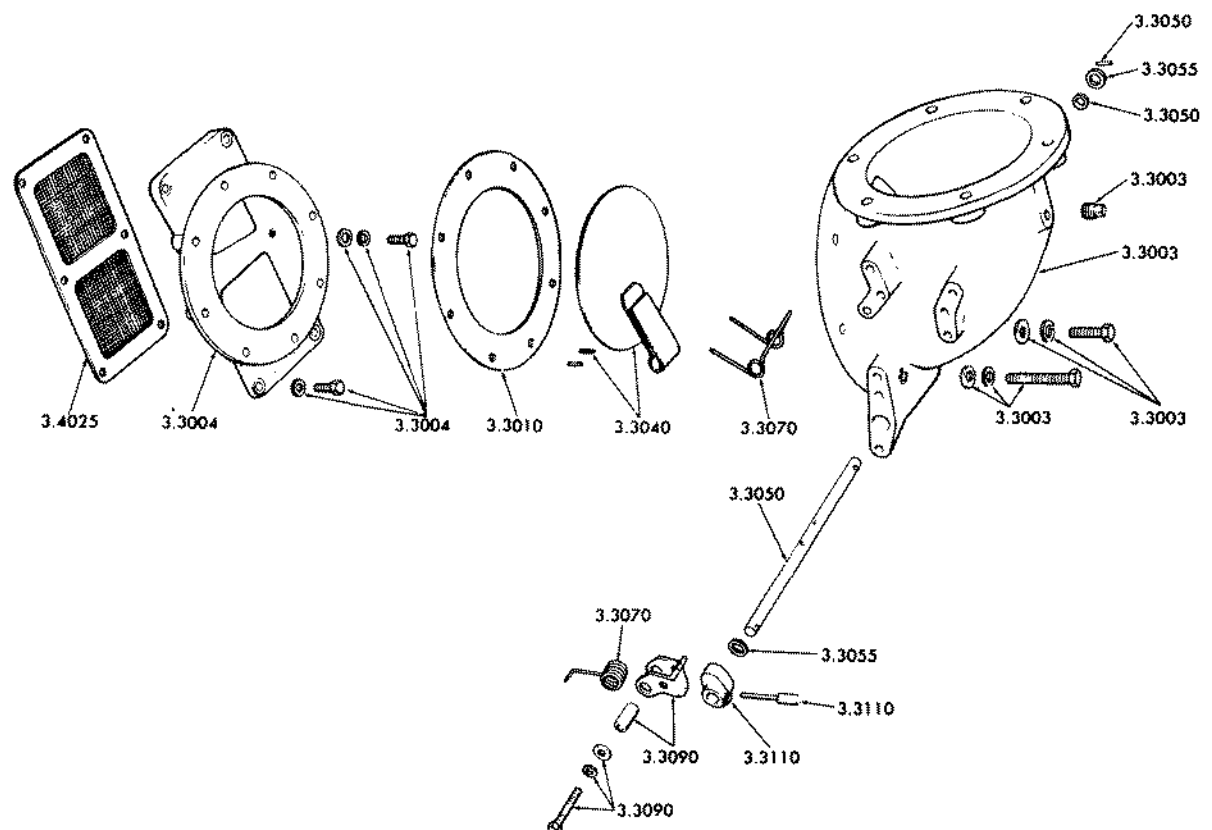
FIG. 3D AIR INLET HOUSING (8V)
