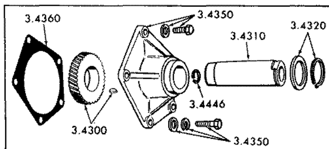
FIG. 4C BLOWER DRIVE
