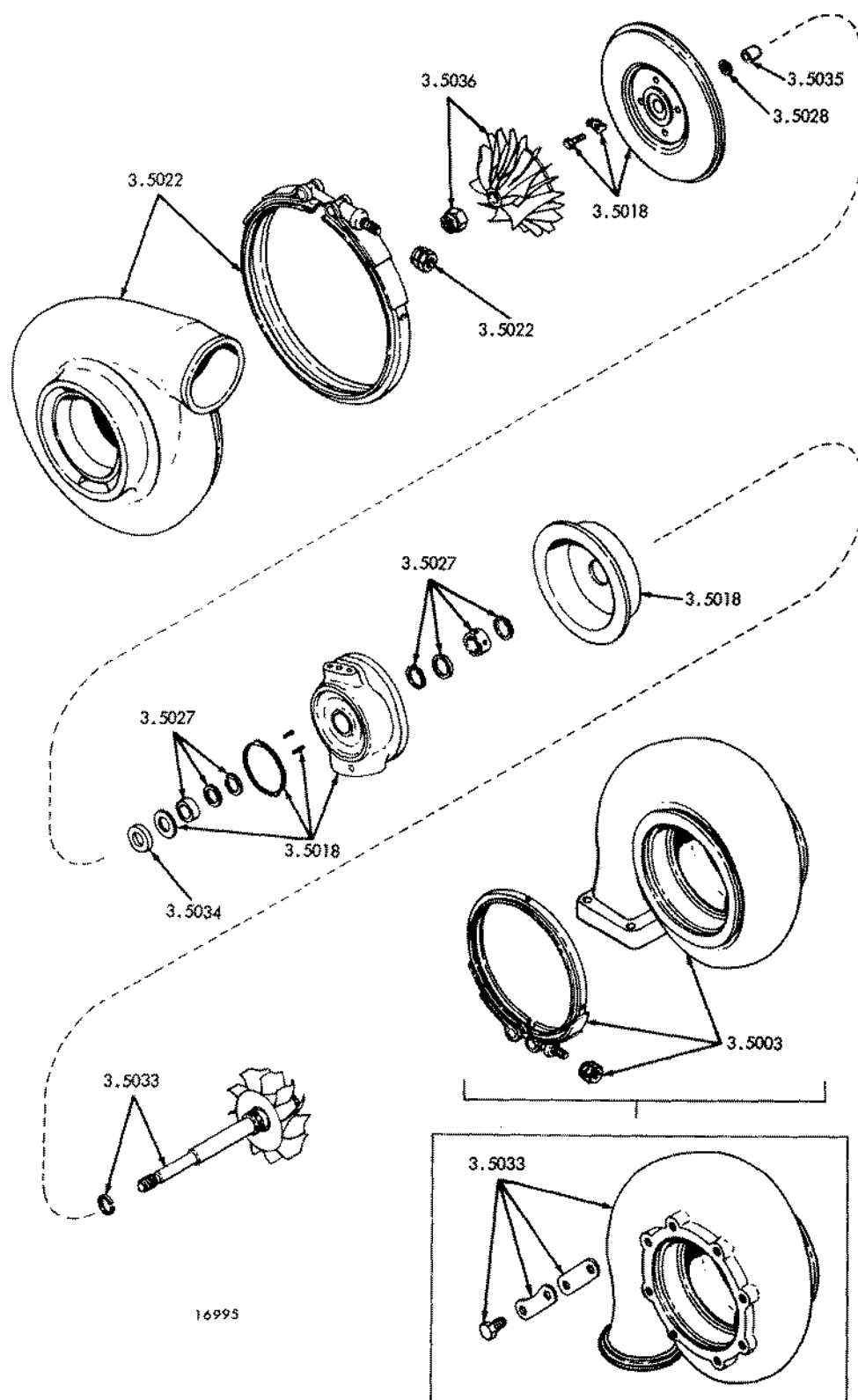
FIG. 5B TURBOCHARGER ASSEMBLY
