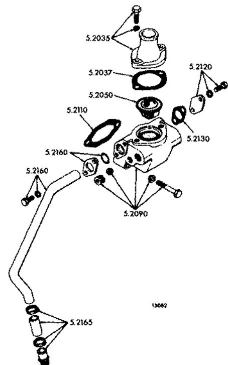
FIG. 3B THERMOSTAT (In-Line Models)
