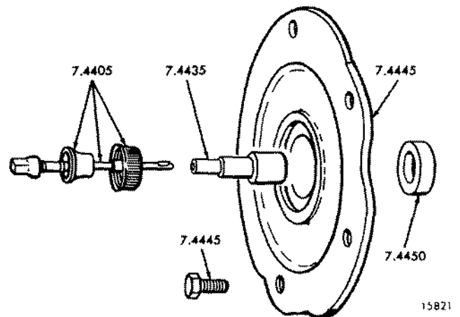
FIG. 5B REAR MOUNTED WITH FLEXIBLE SHAFT
