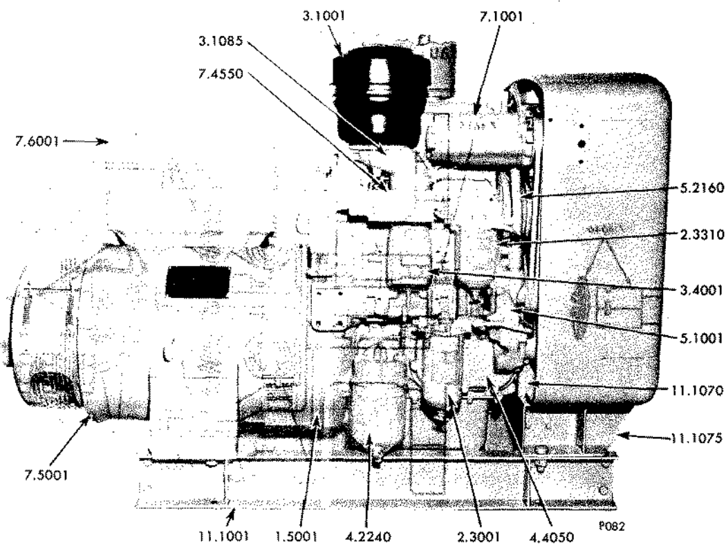
FIG. 10A POWER GENERATOR UNIT
