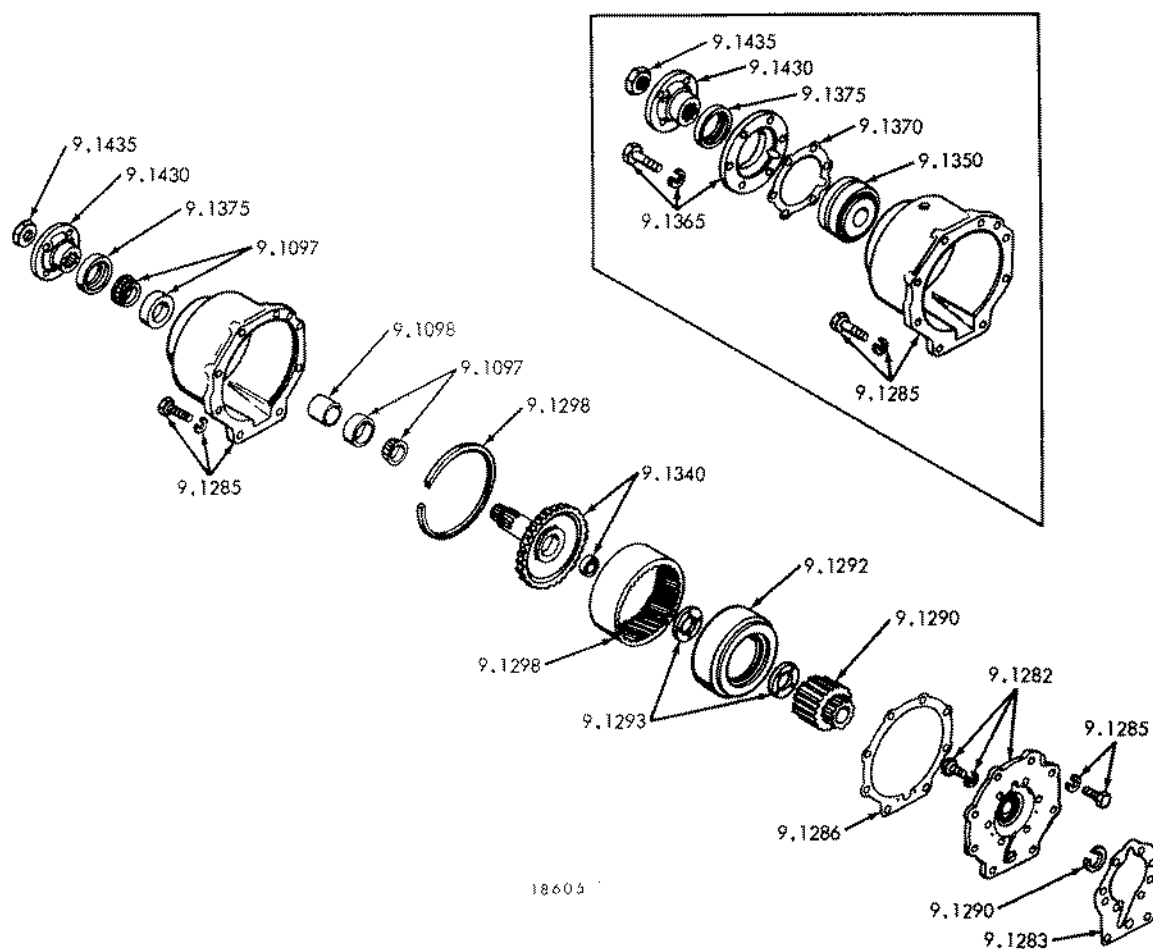
FIG. 2C REDUCTION GEAR (Model 71 and 72)
