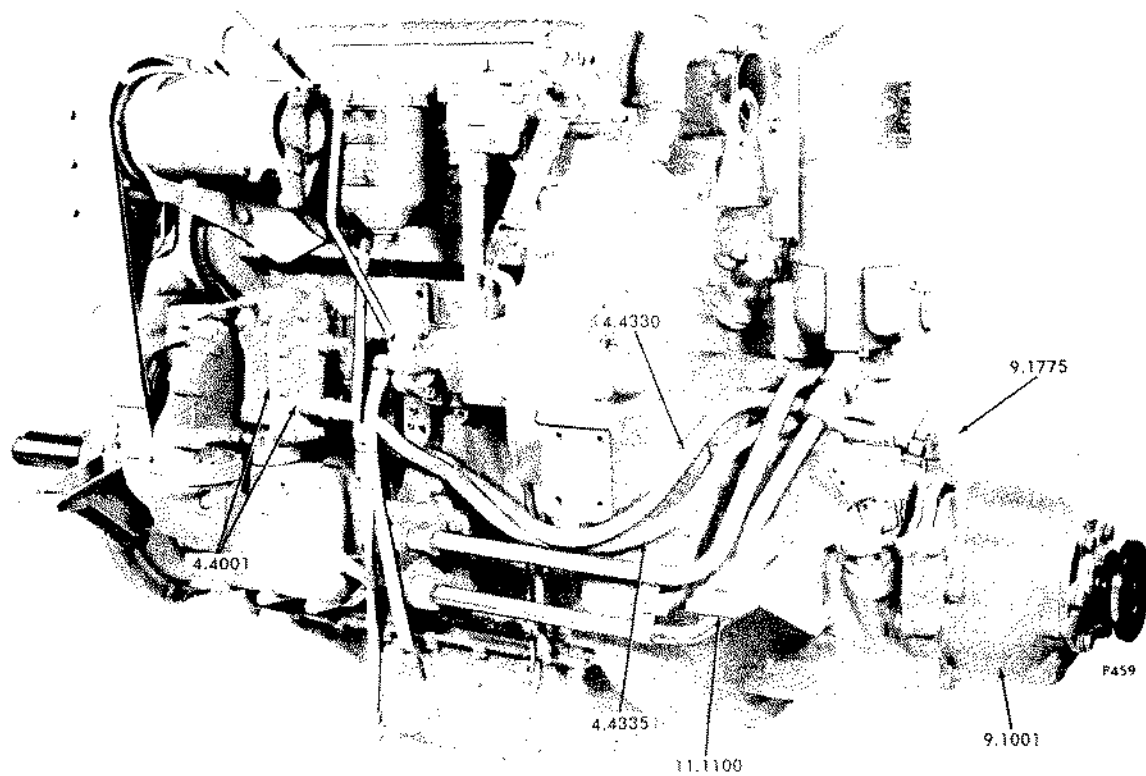
FIG. 1A TYPICAL INLINE MARINE GEAR INSTALLATION
