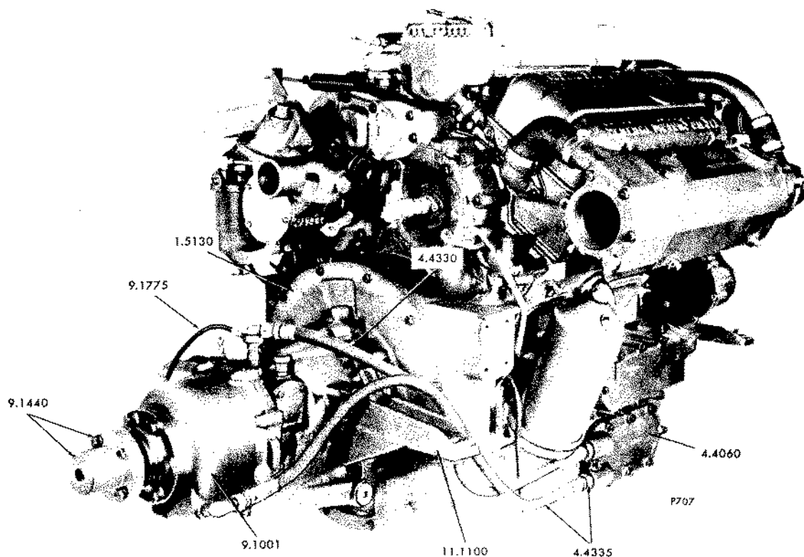
FIG. 1B TYPICAL V-53 MARINE GEAR INSTALLATION
