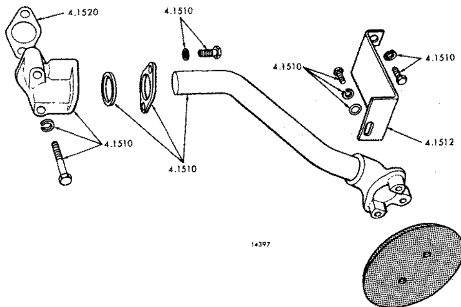
FIG. 2B OIL DISTRIBUTION SYSTEM (8V)
