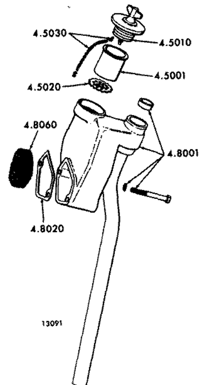
FIG. 8B BREATHING AND OIL FILLER
