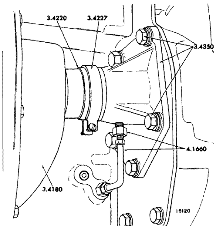
FIG. 2C OIL DISTRIBUTION SYSTEM
