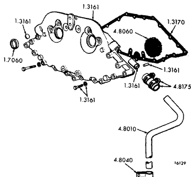
FIG. 8C BREATHING (6V)
