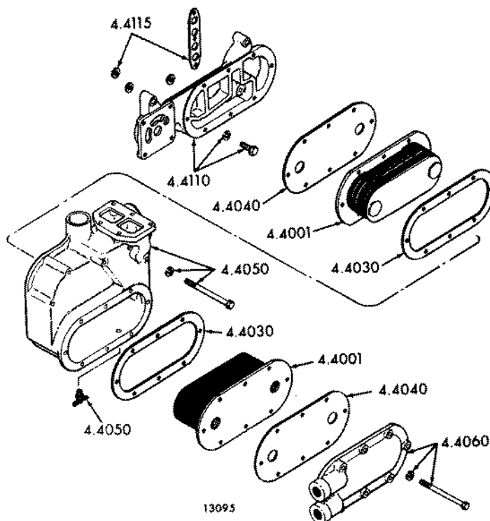
FIG. 4B TORQUE CONVERTER OIL COOLER
