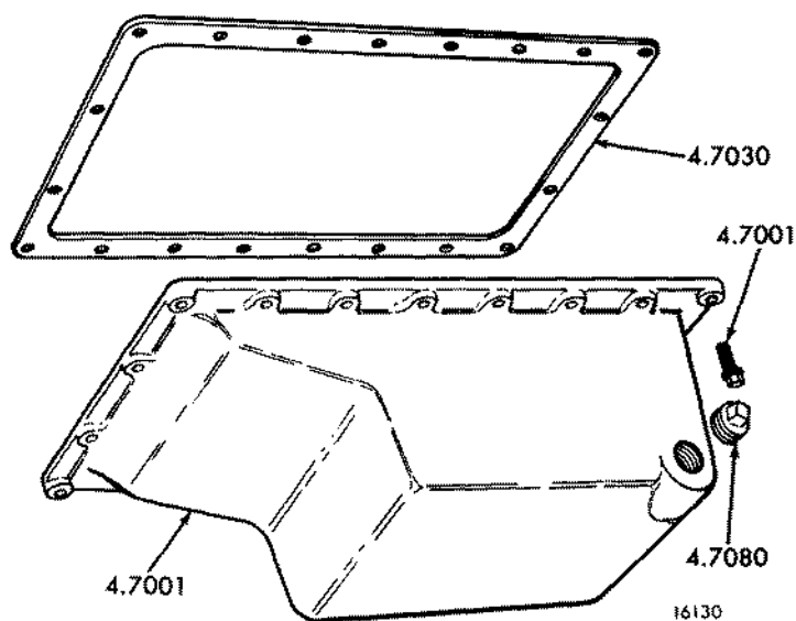
FIG. 7A OIL PAN (CAST)
