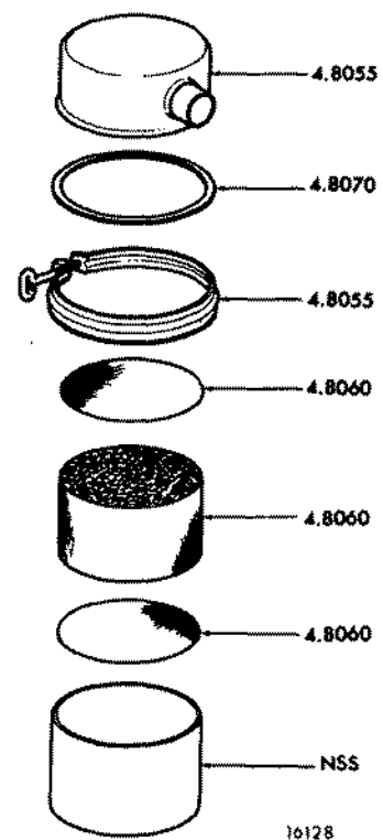
FIG. 8D BREATHER ASSEMBLY
