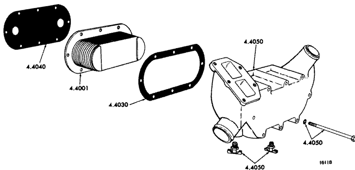
FIG. 4C OIL COOLER
