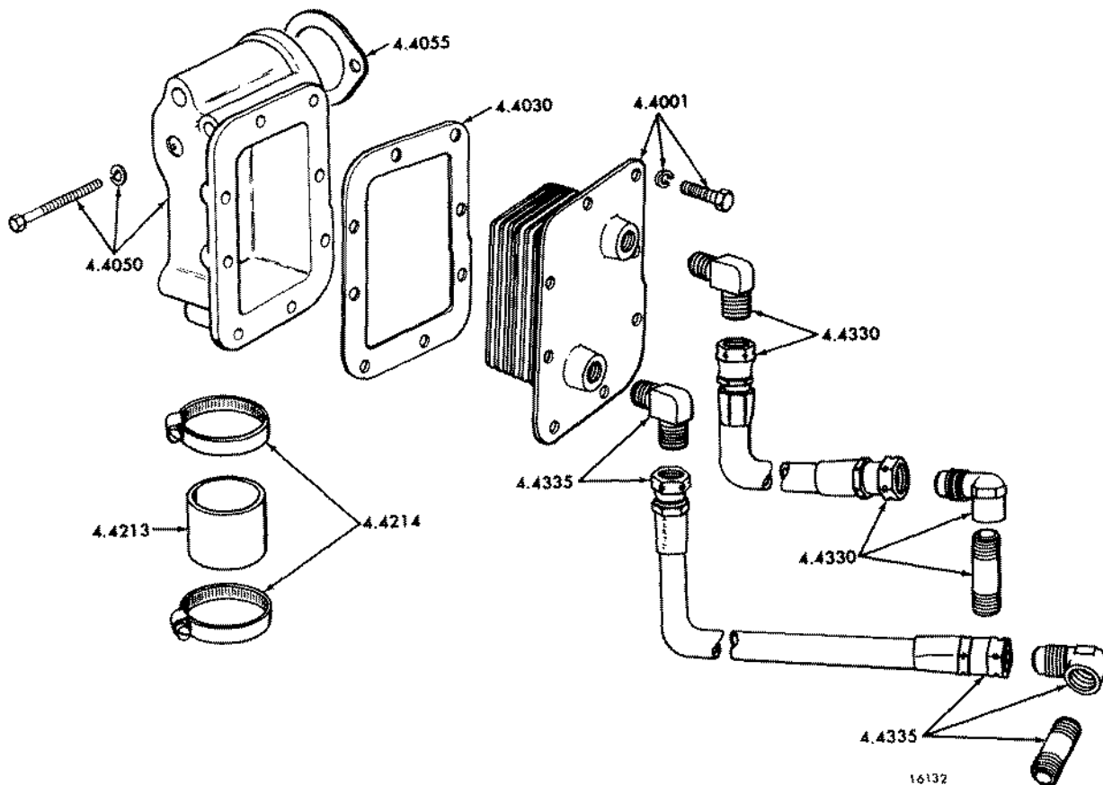
FIG. 4D MARINE GEAR OIL COOLER
