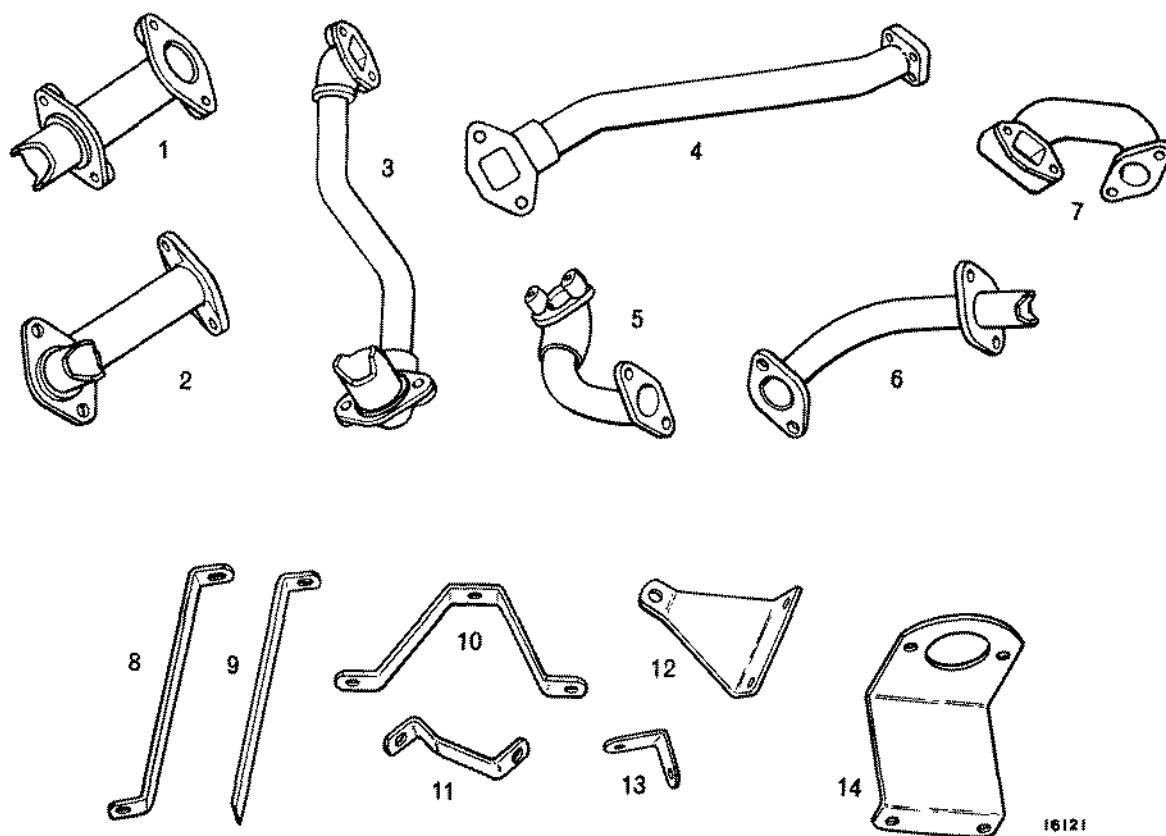
FIG. 2D OIL INLET PIPES
