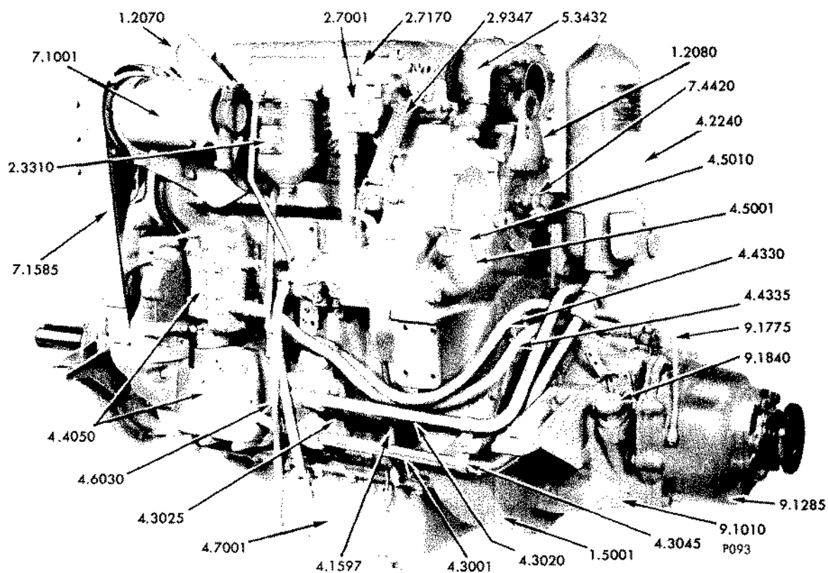
FIG. 10A OIL COOLER AND LINES (In-Line Engine)
