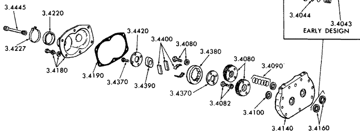
FIG. 4C BLOWER DRIVE
