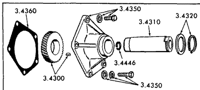
FIG. 4C BLOWER DRIVE
