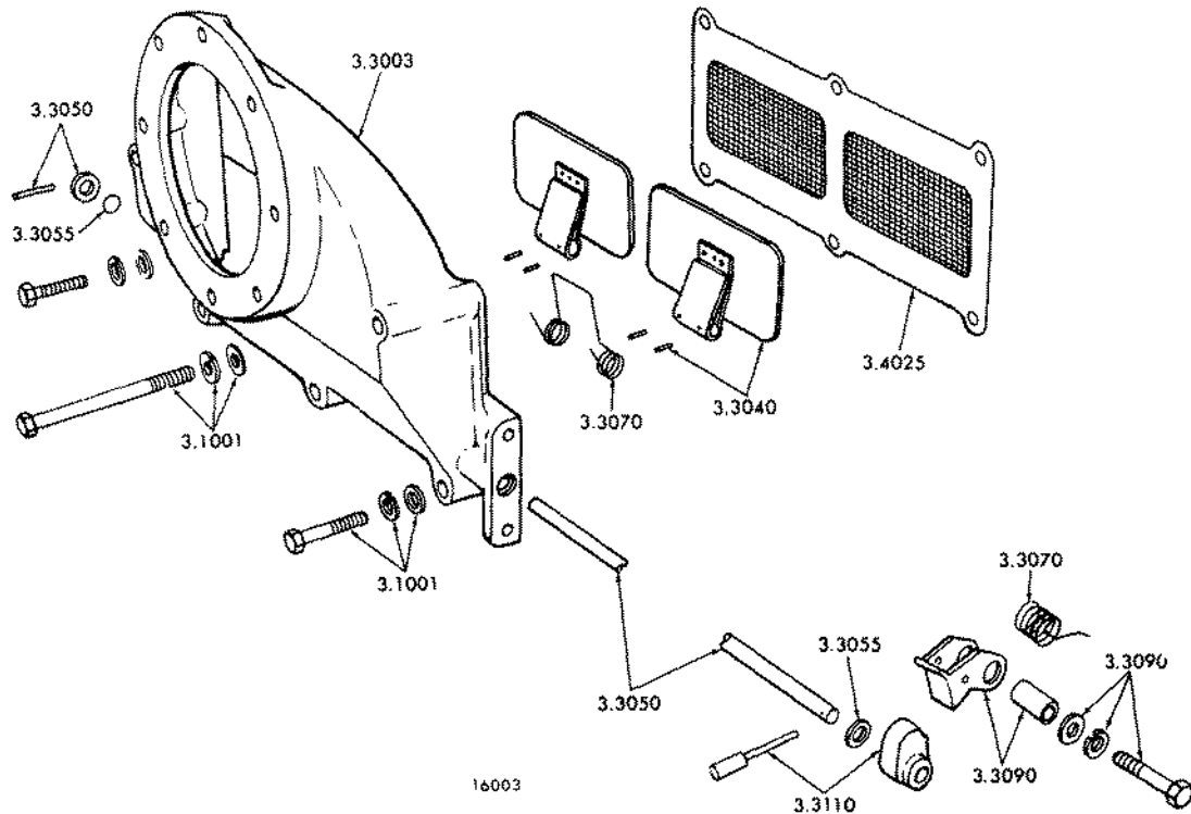
FIG. 3C AIR INLET HOUSING (6V-53)
