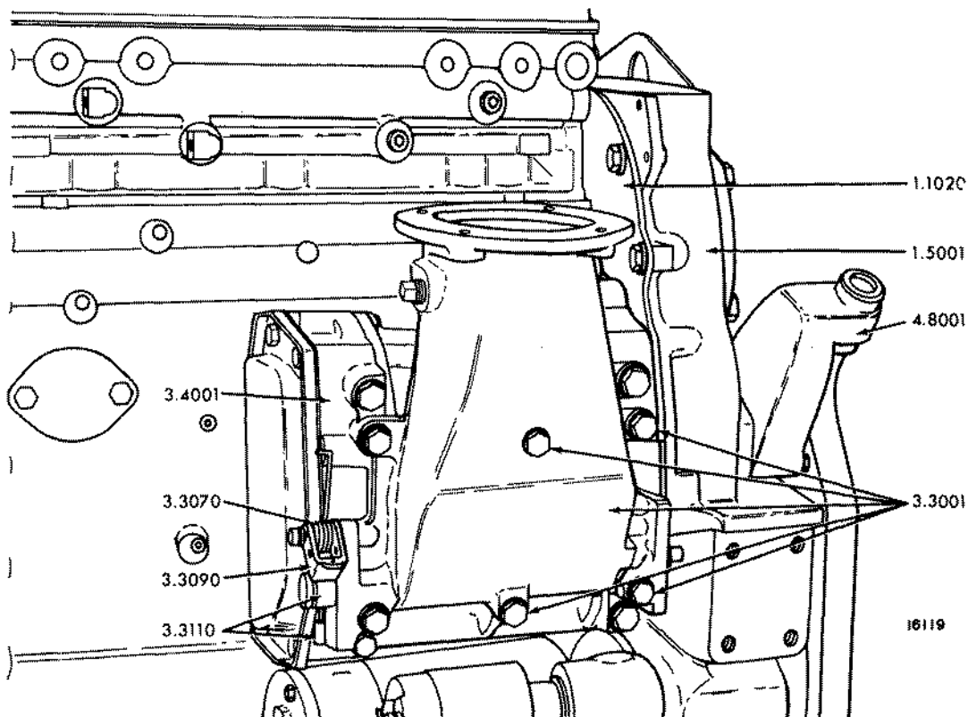
FIG. 3B BLOWER AND AIR INLET HOUSING
