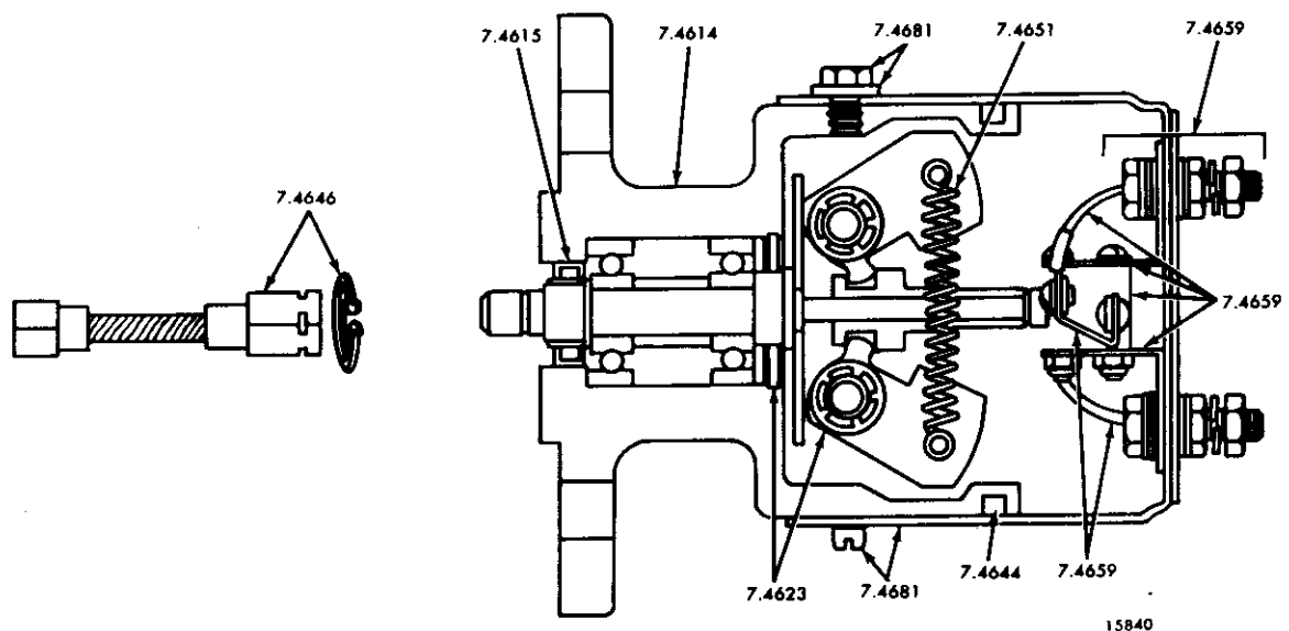
FIG. 6C OVERSPEED GOVERNOR (Single Switch Electric)
