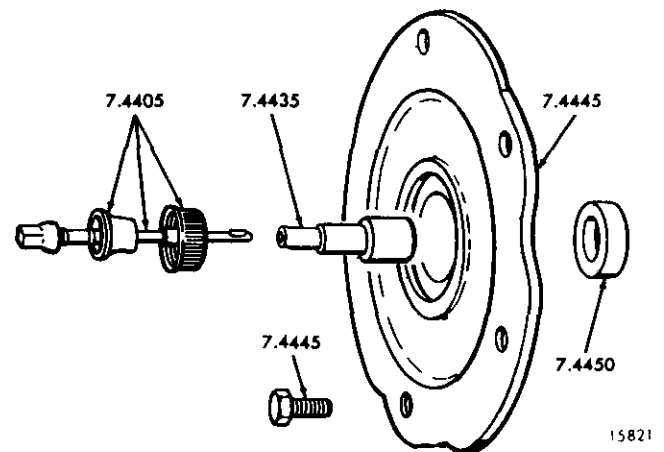
FIG. 5B REAR MOUNTED WITH FLEXIBLE SHAFT
