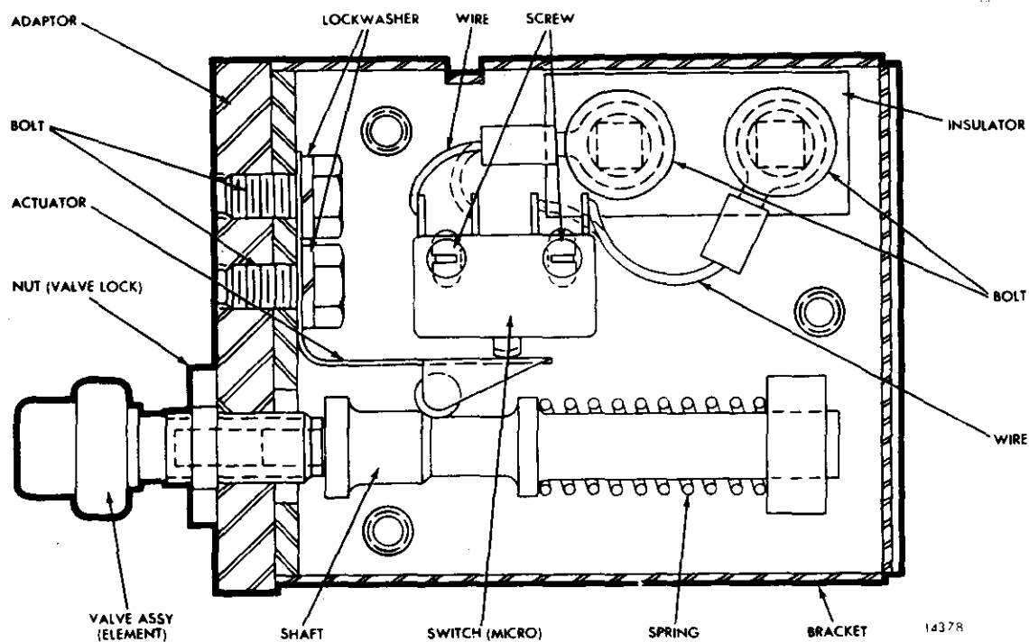
FIG. 4B SWITCH ASSY., WATER TEMPERATURE SHUTDOWN (7.4505)
