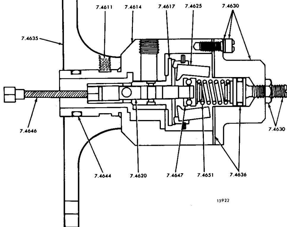
FIG. 6B OVERSPEED GOVERNOR (Hydraulic Dump Type)
