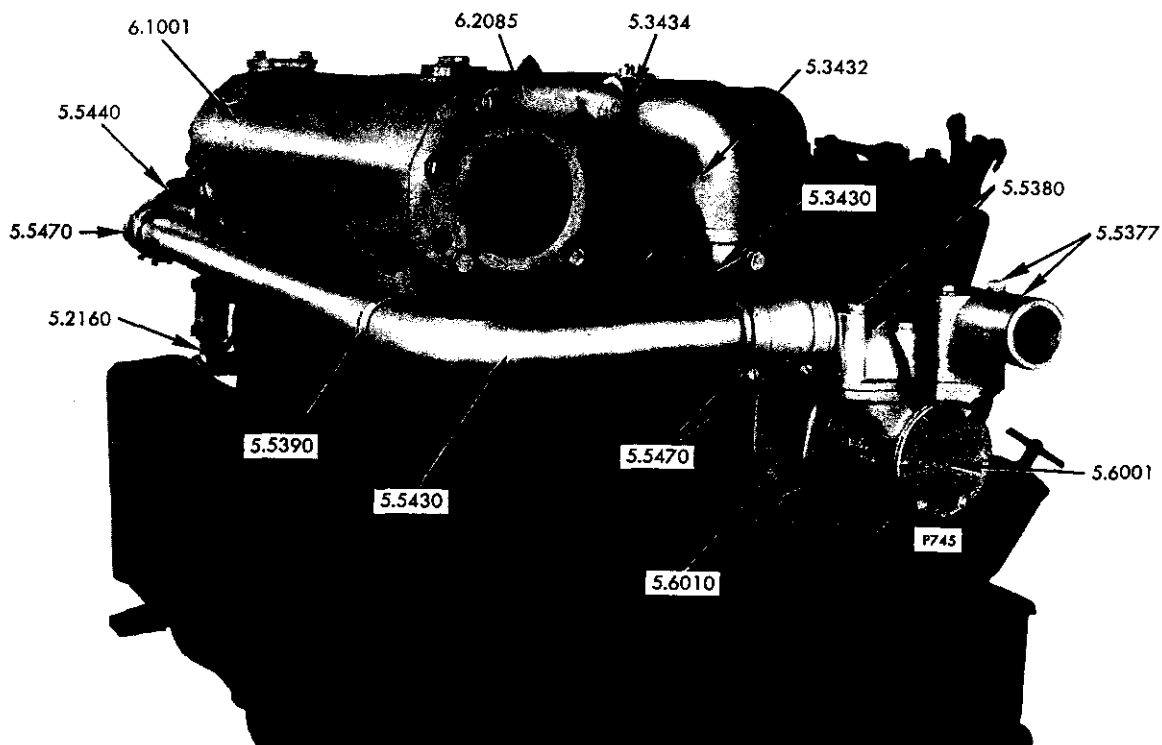
FIG. 7A TYPICAL RAW WATER PUMP INSTALLATION (In-Line Engines)
