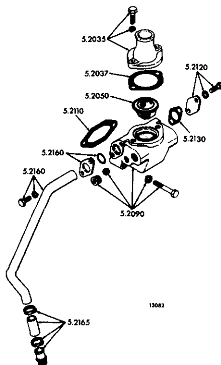
FIG. 3B THERMOSTAT (In-Line Models)
