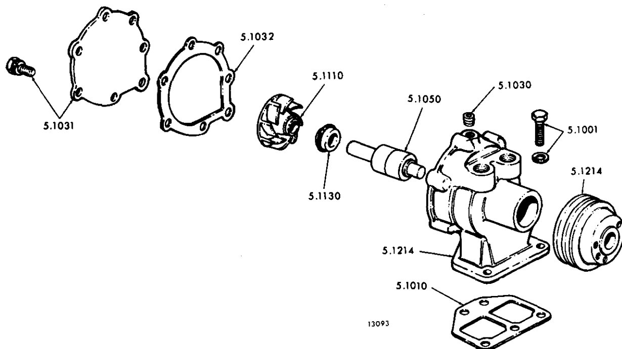
FIG. 2A FRESH WATER PUMP
