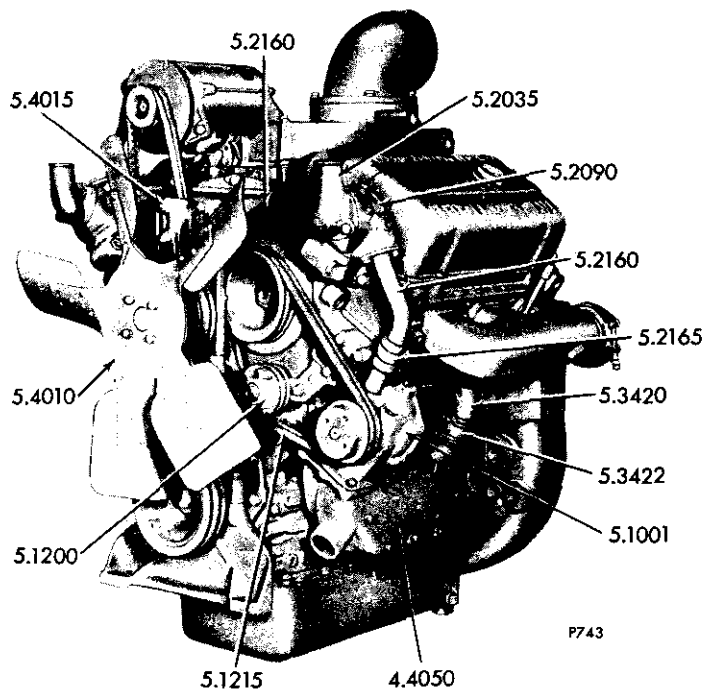
FIG. 1B TYPICAL COOLING SYSTEM (V-Engine)
