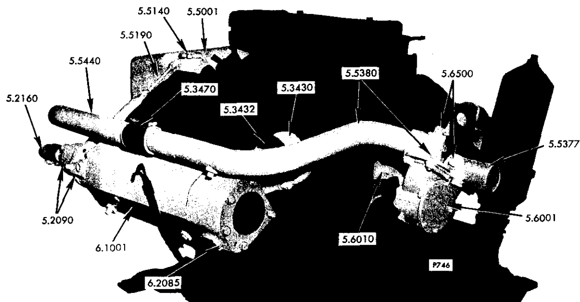
FIG. 7B TYPICAL RAW WATER PUMP INSTALLATION (V-Engines)
