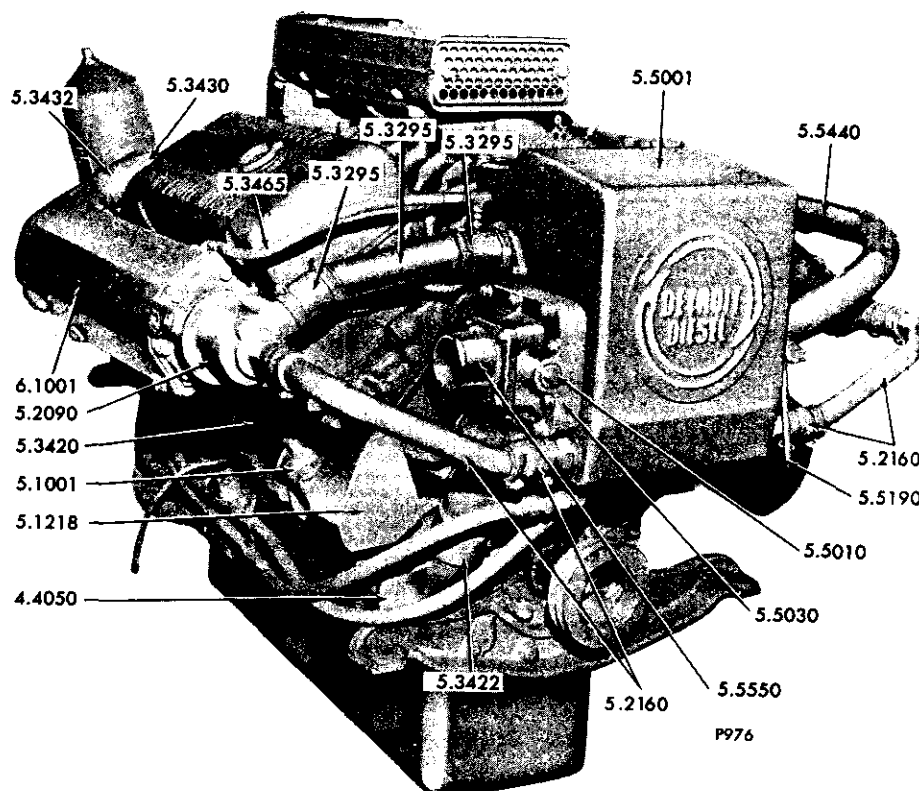
FIG. 5B TYPICAL HEAT EXCHANGER COOLING SYSTEM (V-Model)
