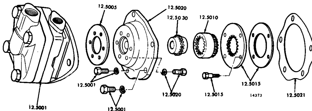
FIG. 4A HYDRAULIC PUMP
