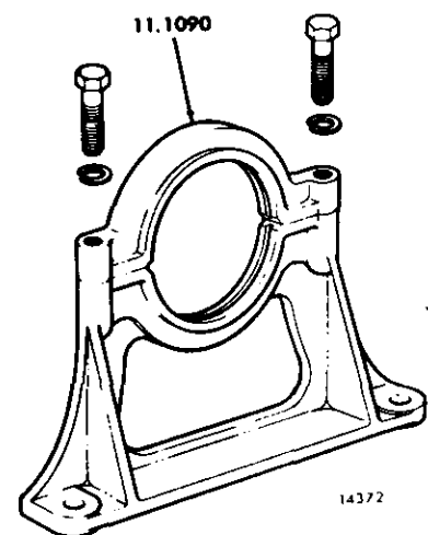
FIG. 1D FRONT ENGINE SUPPORT (Trunnion)
