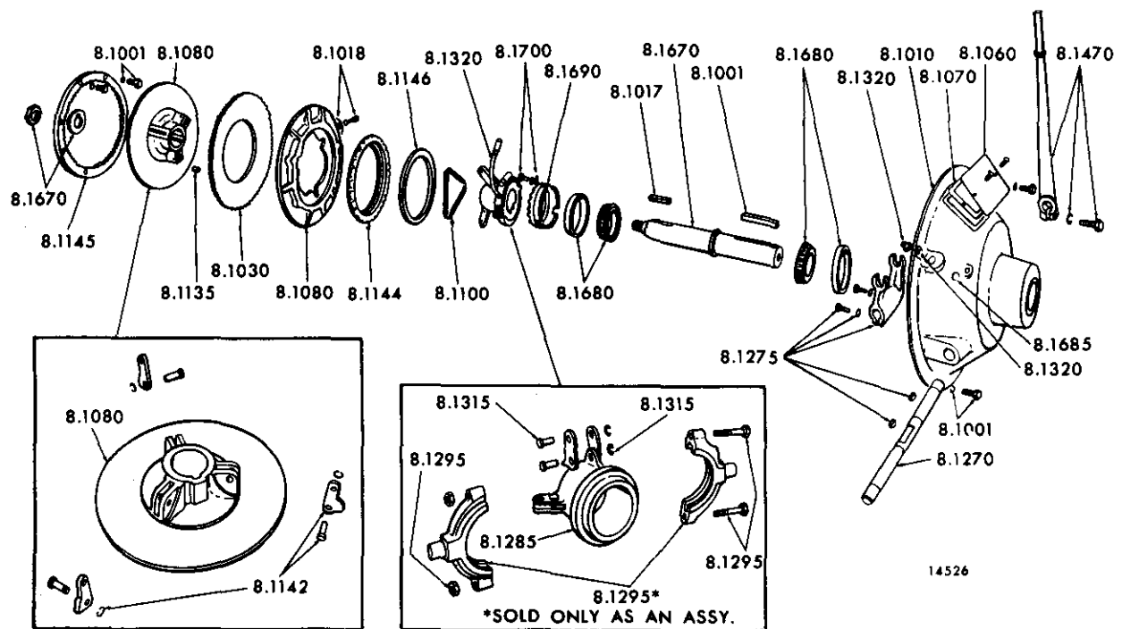
FIG. 1A POWER TAKE-OFF
