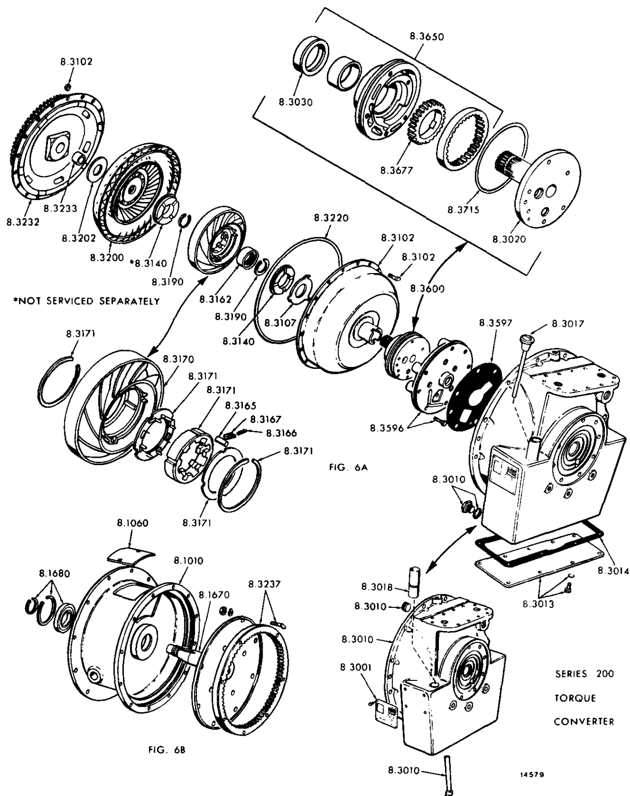
SERIES 200 TORQUE CONVERTER
