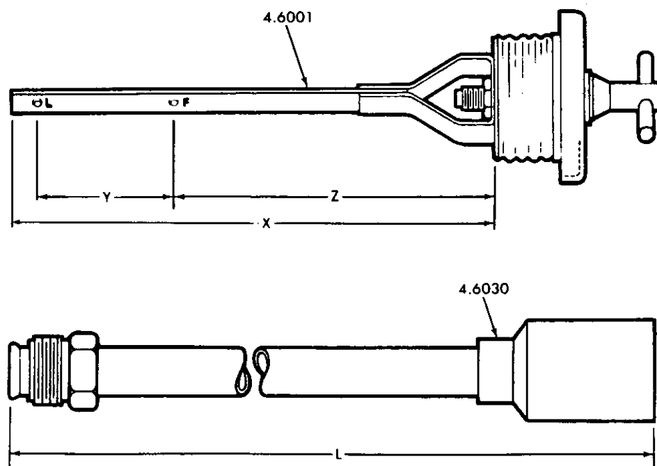
FIG. 6B DIPSTICK
