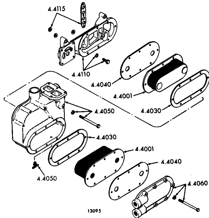
FIG. 4B TORQUE CONVERTER OIL COOLER
