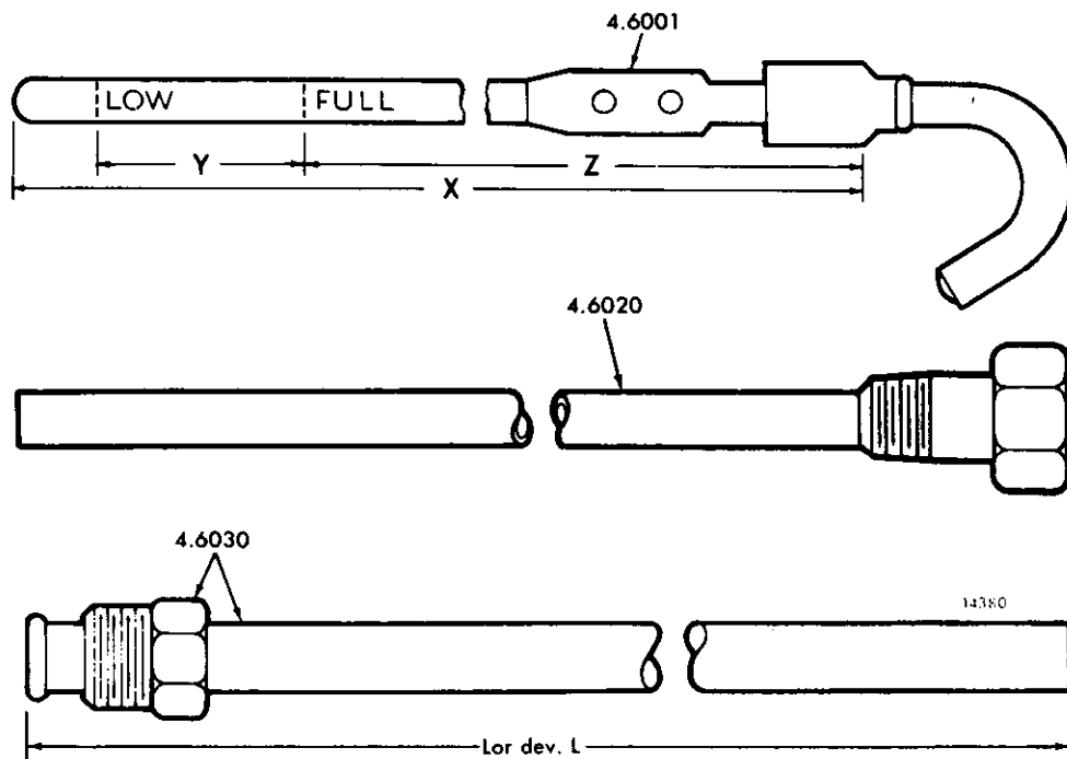
FIG. 6A DIPSTICK
