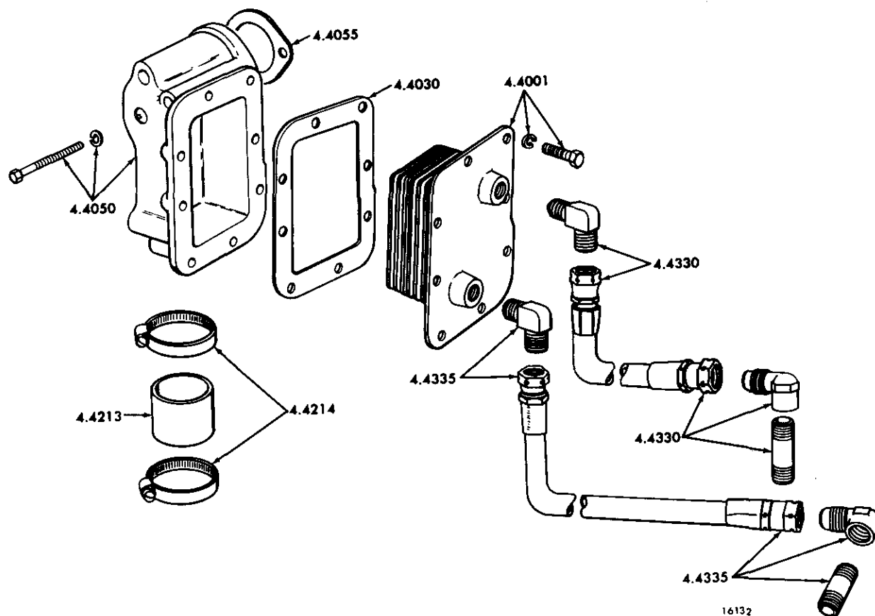
FIG. 4D MARINE GEAR OIL COOLER
