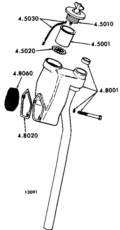
FIG. 8B BREATHER AND OIL FILLER
