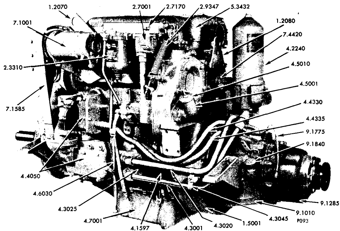
FIG. 10A OIL COOLER AND LINES (In-Line Engine)
