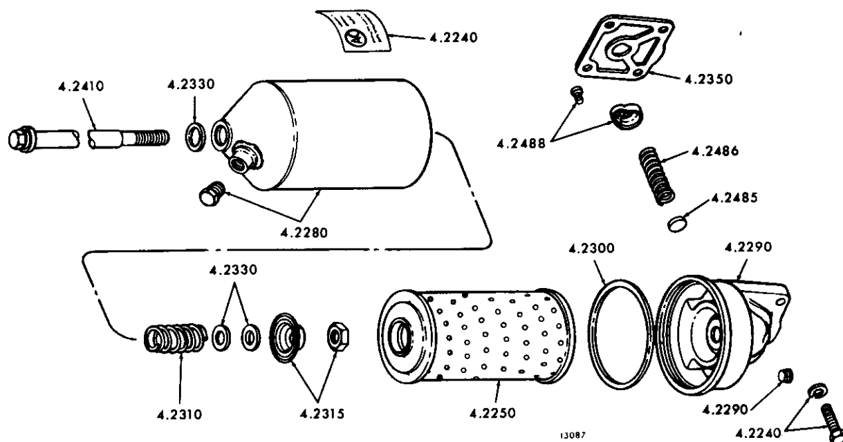
FIG. 3A OIL FILTER
