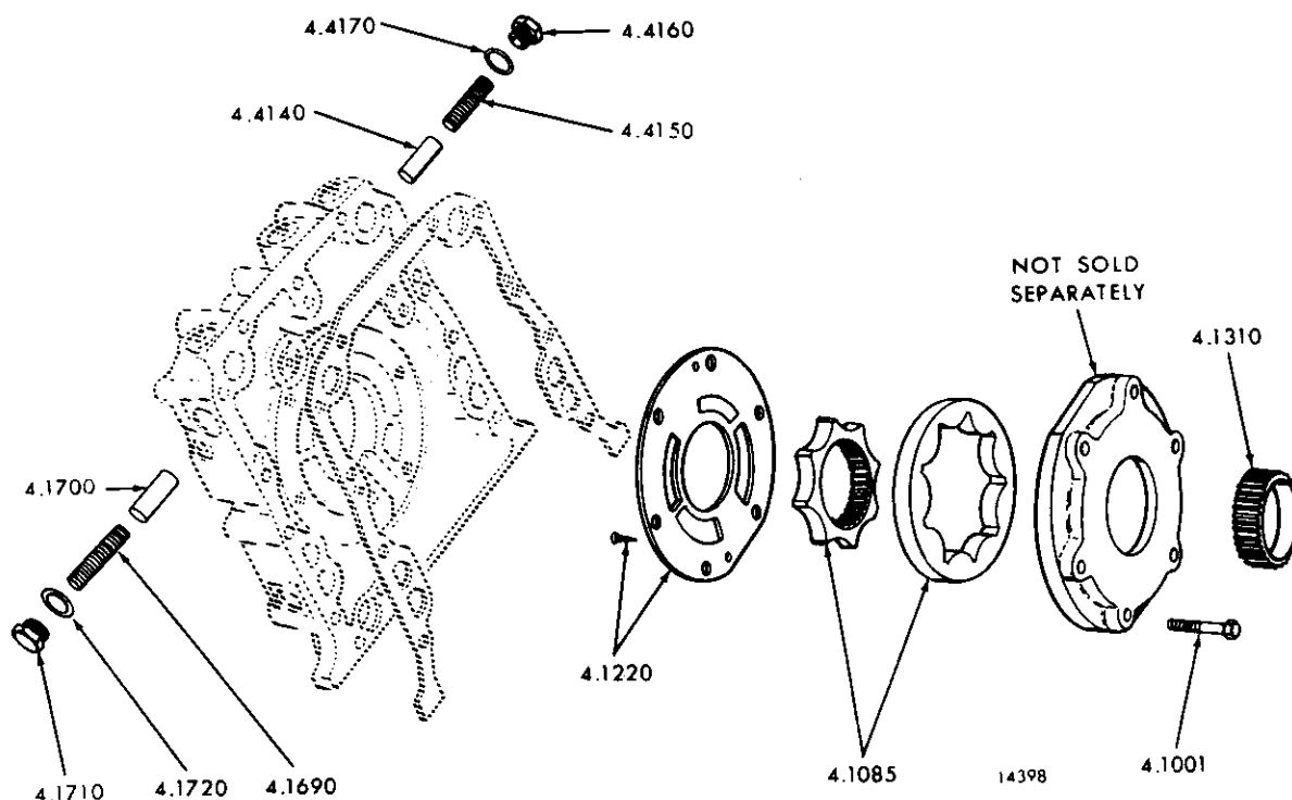
FIG. 1A OIL PUMP AND PRESSURE REGULATOR (In-Line Models)
