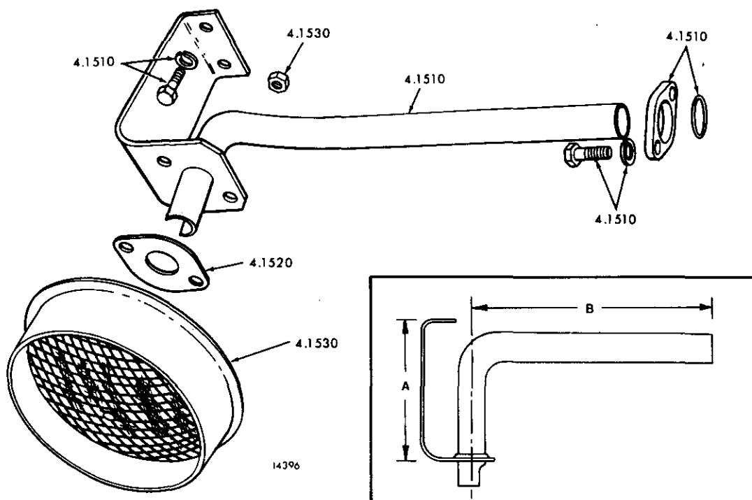
FIG. 2A OIL DISTRIBUTION SYSTEM
