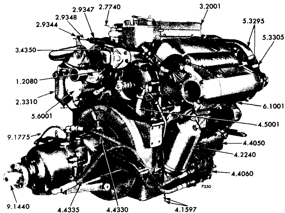
FIG. 10B OIL COOLER AND LINES (V-Engine)
