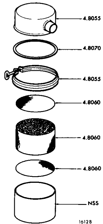
FIG. 8D BREATHER ASSEMBLY
