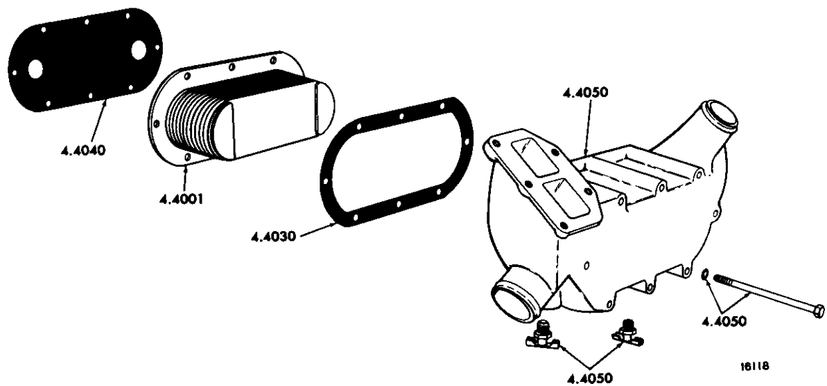
FIG. 4C OIL COOLER
