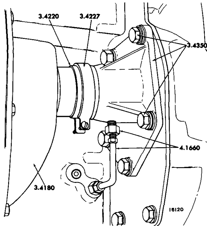
FIG. 2C OIL DISTRIBUTION SYSTEM
