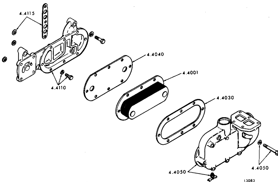
FIG. 4A OIL COOLER
