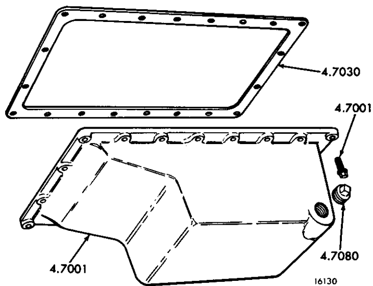
FIG. 7A OIL PAN (CAST)
