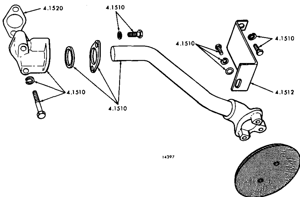
FIG. 2B OIL DISTRIBUTION SYSTEM (8V)
