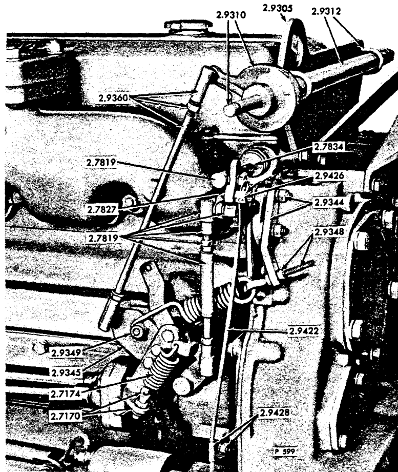
FIG. 8A THROTTLE CONTROL (PIERCE GOVERNOR)
