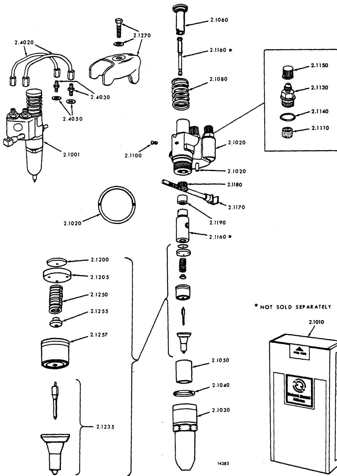
FIG. 1B FUEL INJECTOR
