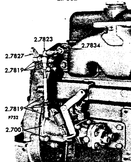
FIG. 5A GOVERNOR (PIERCE)
