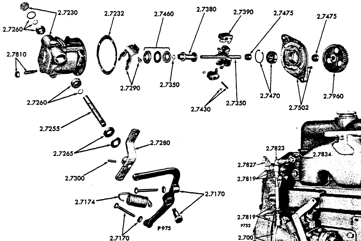
FIG. 5C GOVERNOR
