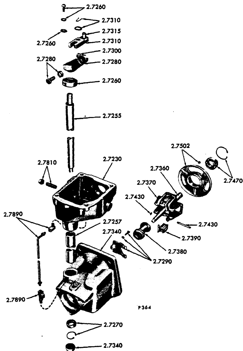
FIG. 5D - MECHANICAL GOVERNOR HOUSING WEIGHTS AND LEVER (CLOSED LINKAGE)
