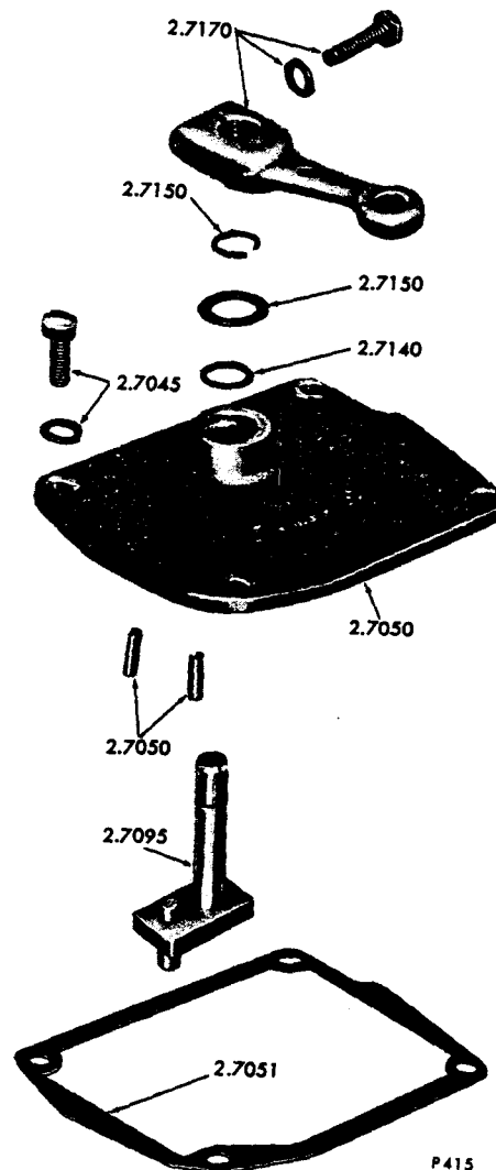
FIG. 5E - MECHANICAL GOVERNOR COVER (SINGLE LEVER)
