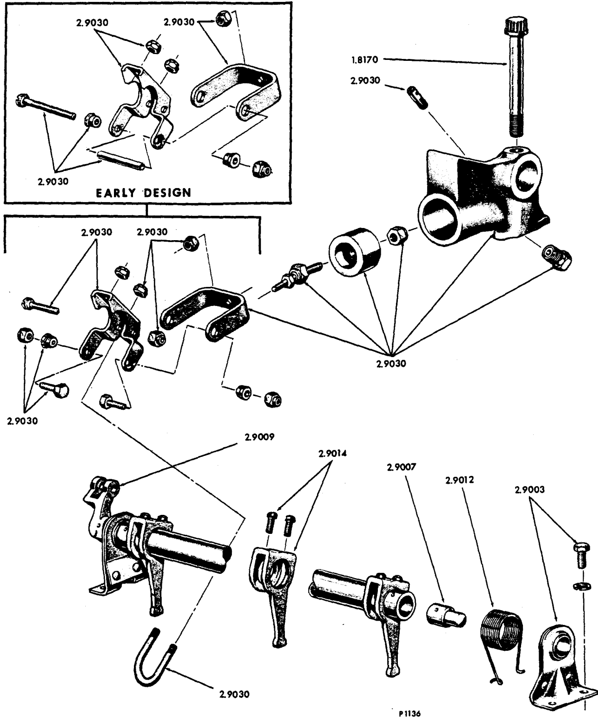
FIG. 7C INJECTOR CONTROL TUBE AND THROTTLE DELAY MECHANISM (8V)
