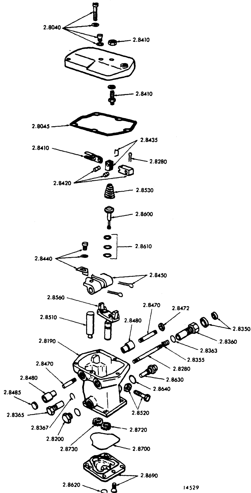
FIG. 6A HYDRAULIC GOVERNOR
