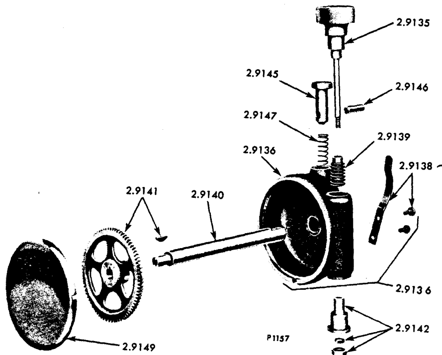
FIG. 8B VERNIER THROTTLE CONTROL
