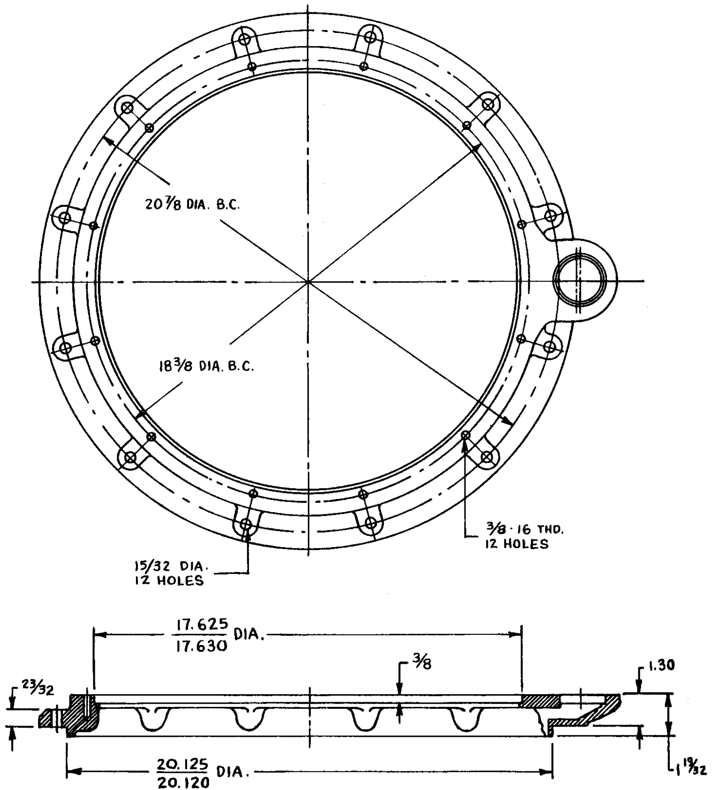
6C3A-22 Flywheel Housing Adaptor For Allison Marine Gear SAE #1 to #2 @ 1.30" Offset C5-60-9
