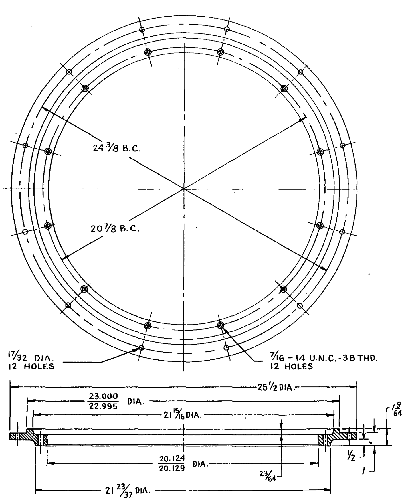
GC3A-28 Flywheel Housing Adaptor SAE #1/2 to #1 @ 1" Offset C5-60-14
