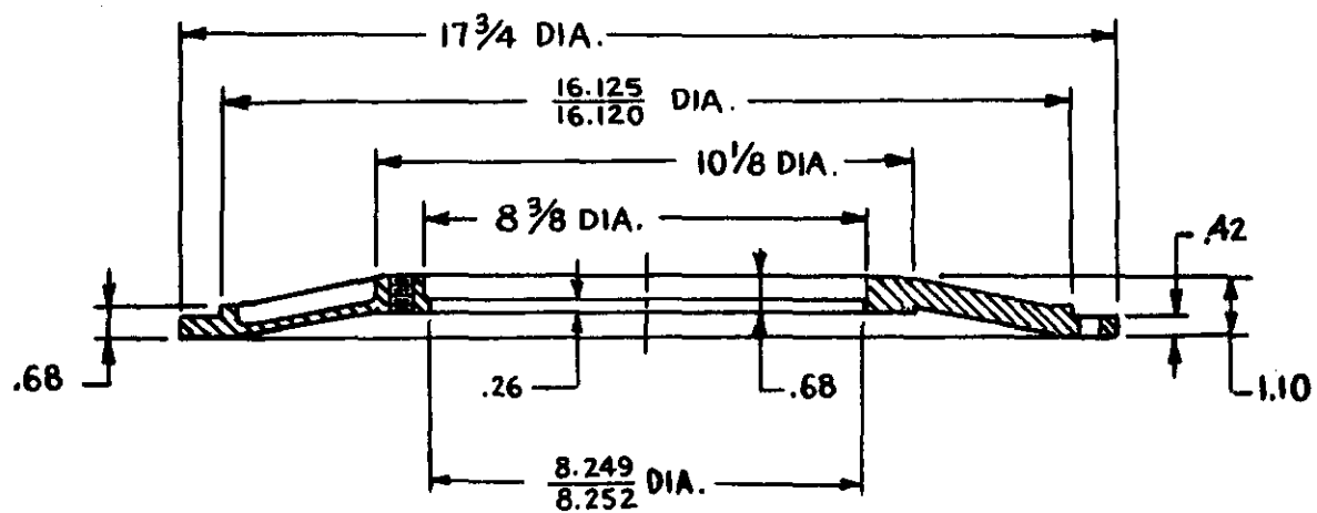
6C3A-30 Flywheel Housing Adaptor SAE #3 to Warner Transmission C5-60-16
