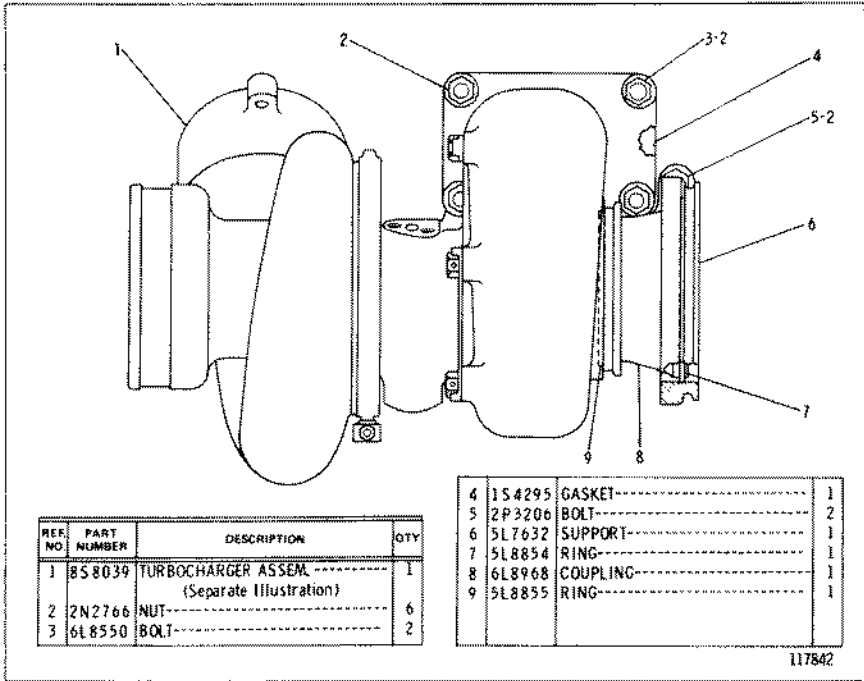
2N5892 TURBOCHARGER GROUP
