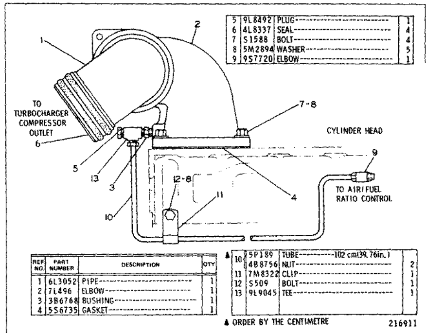
7N5455 AIR LINES GROUP
