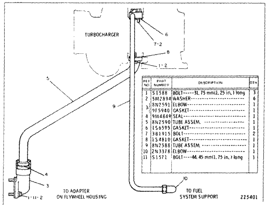
8N2589 TURBOCHARGER OIL LINES GROUP
