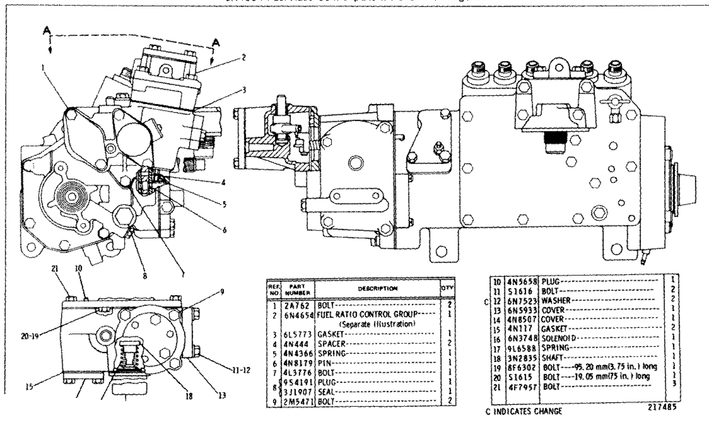
6N5275 GOVERNOR AND FUEL INJECTION PUMP GROUP—Part 2—Type 1 Part of 7N5304 Governor and Fuel Injection Pump Group shown on Page 184 6N4654 Fuel Ratio Control parts are shown on Page 224
