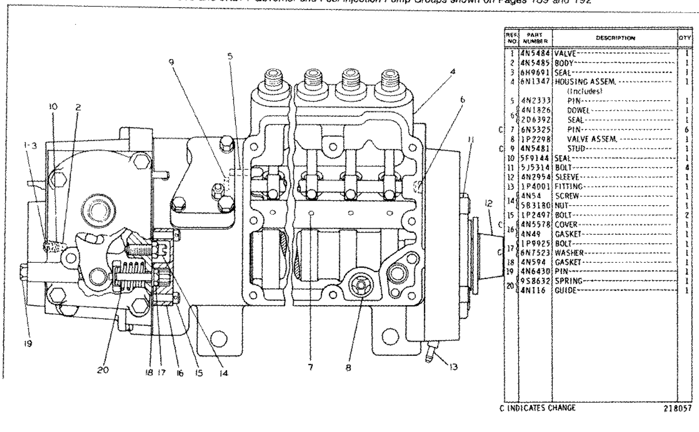
4N9754 GOVERNOR AND FUEL INJECTION PUMP GROUP—Part 2 of 4—Type 1 Part of 6N7613 and 6N271 Governor and Fuel Injection Pump Groups shown on Pages 189 and 192
