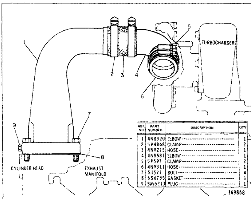
7N3884 AIR LINES GROUP
