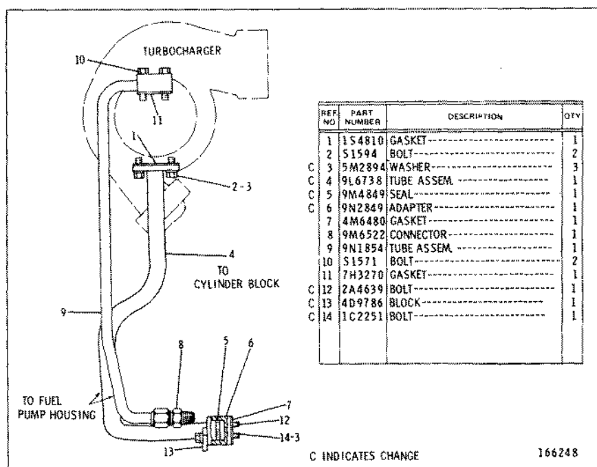
9L5801 TURBOCHARGER OIL LINES GROUP
