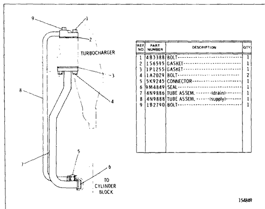
6N25 TURBOCHARGER OIL LINES GROUP
