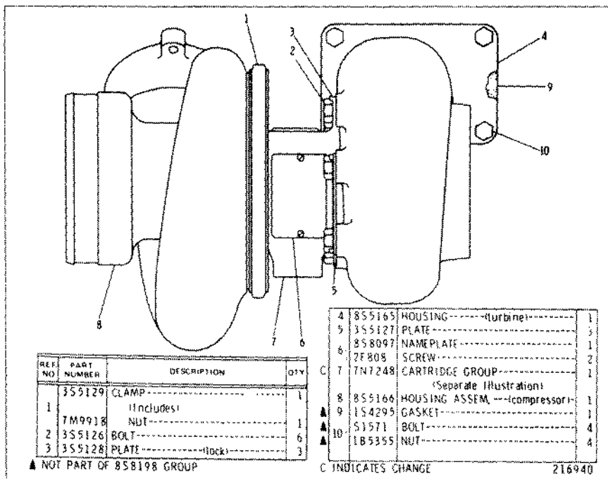
8S8198 TURBOCHARGER GROUP (8S8200 N/S)—Replaced by
