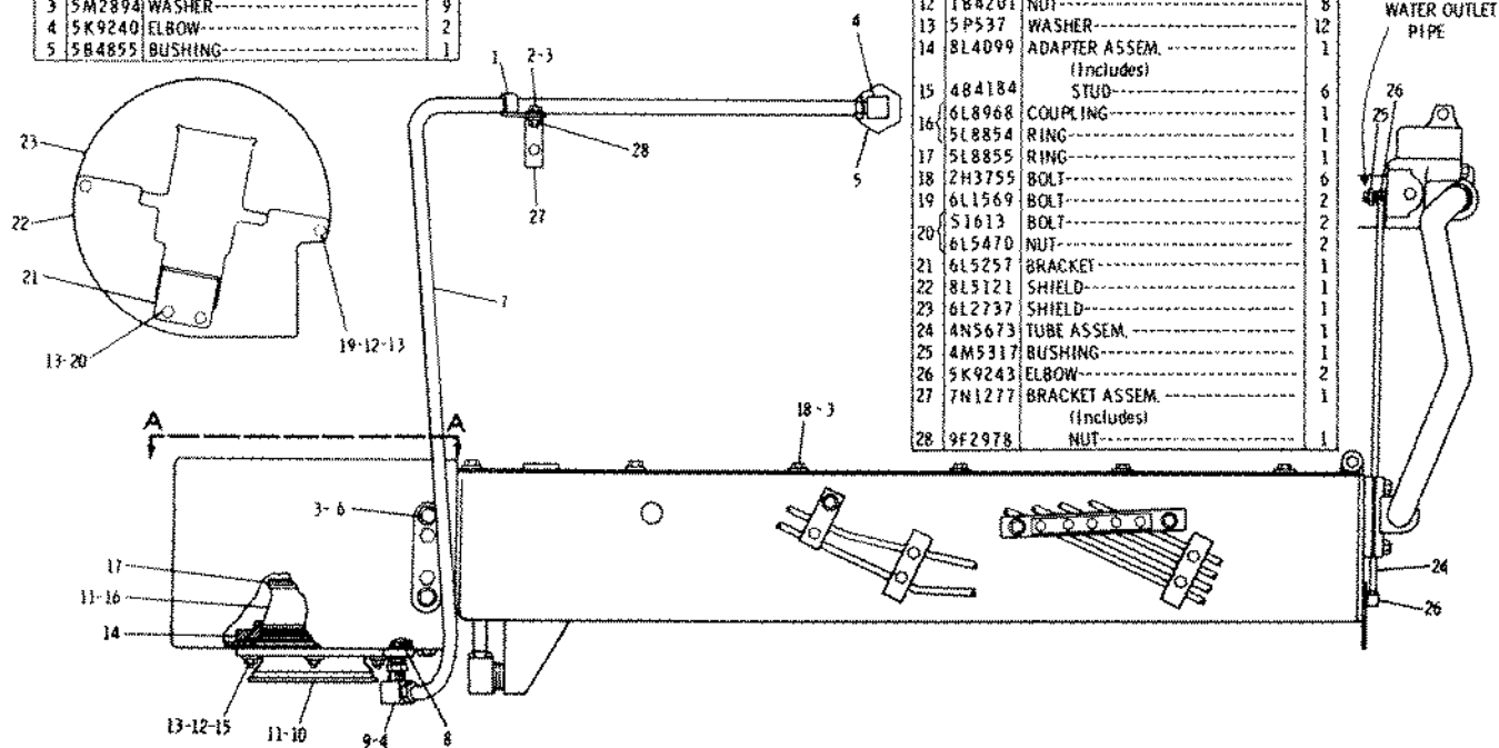
8N865 MANIFOLD SHIELD GROUP—Water Cooled—Part 1 Serial No. 66D33234—Up. AN ATTACHMENT
