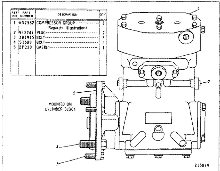
9N8069 AIR COMPRESSOR GROUP—David Brown Also available as an Attachment 6N7582 Compressor parts are shown on Page 168
