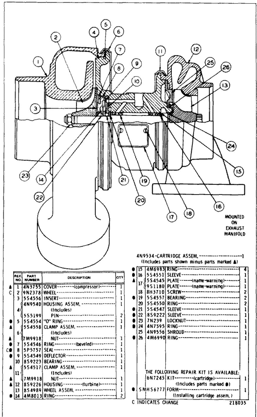
9N1280 TURBOCHARGER GROUP—Field installation
