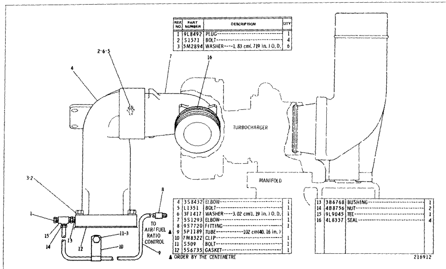
7N3624 AIR LINES GROUP
