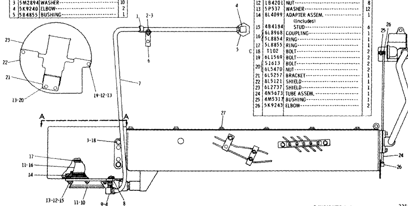
6N1302 MANIFOLD SHIELD GROUP—Water Cooled—Part 1—Type 2 Serial No. 66D26832 to 66D33233 inclusive CANNOT BE USED WITH TURBOCHARGED AFTERCOOLED ENGINE
