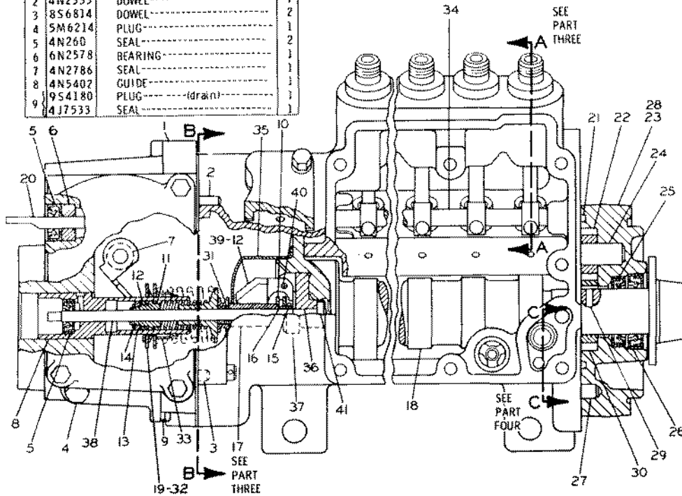
4N9754 GOVERNOR AND FUEL INJECTION PUMP GROUP—Part 1 of 4—Type 2 Part of 6N7613 & 6N271 Governor and Fuel Injection Pump Groups shown on Pages 189 & 192
