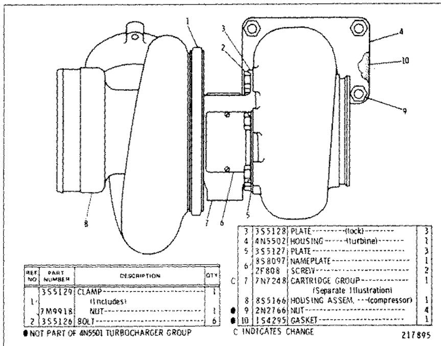
4N5501 TURBOCHARGER GROUP (3N3280 N/S)
