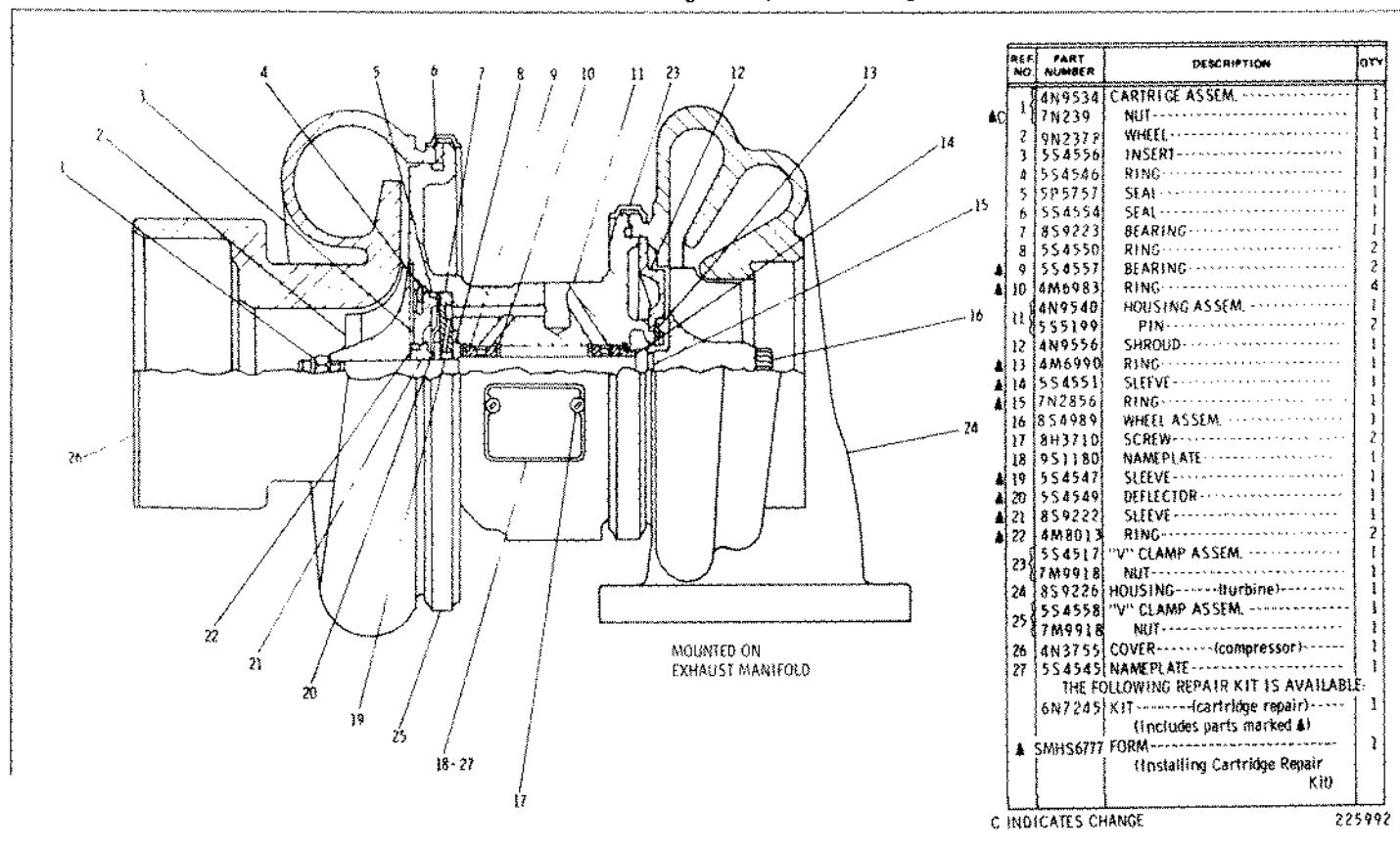
8N3367 TURBOCHARGER GROUP Part of 8N3382 Turbocharger Group shown on Page 147A
