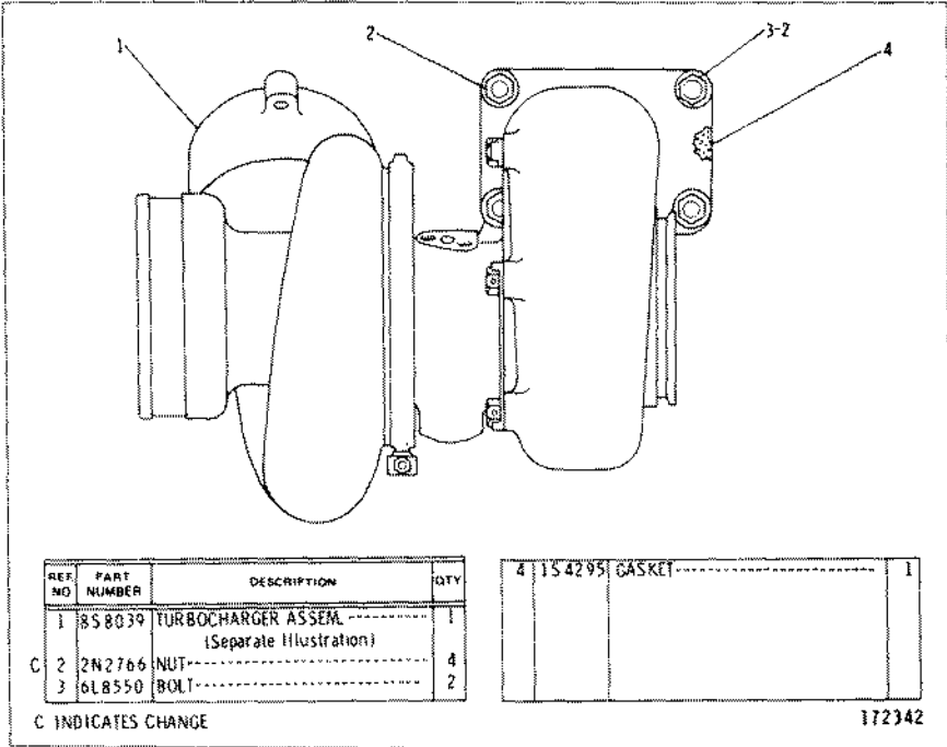
3N2882 TURBOCHARGER GROUP
