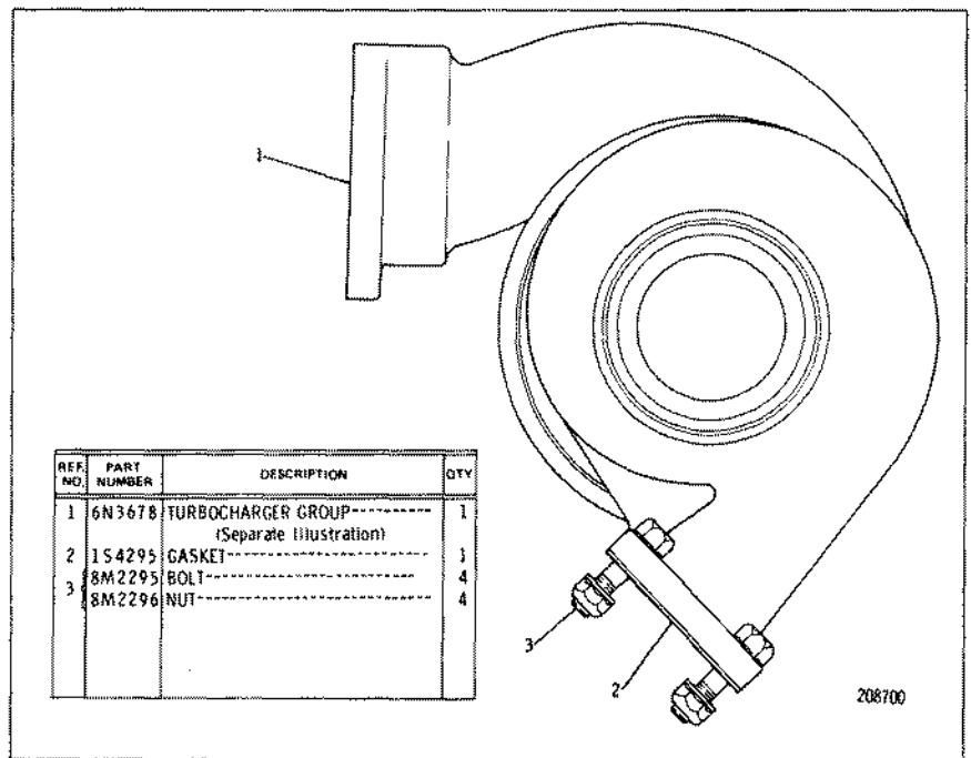
6N3477 TURBOCHARGER GROUP 6N3678 Turbocharger parts are shown on Page 154
