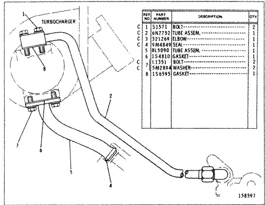
4N7122 TURBOCHARGER OIL LINES GROUP
