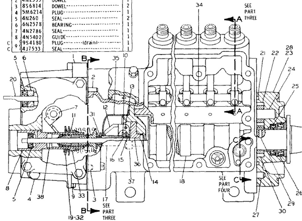
4N9754 GOVERNOR AND FUEL INJECTION PUMP GROUP—Part 1 of 4—Type 1 Part of 6N7613 and 6N271 Governor and Fuel Injection Pump Groups shown on Pages 189 and 192
