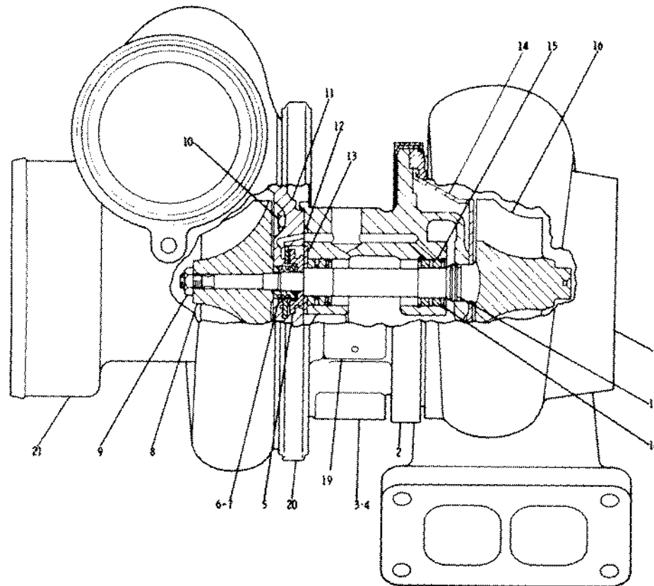
6N3678 TURBOCHARGER GROUP Part of 6N3477 Turbocharger Group shown on Page 145
