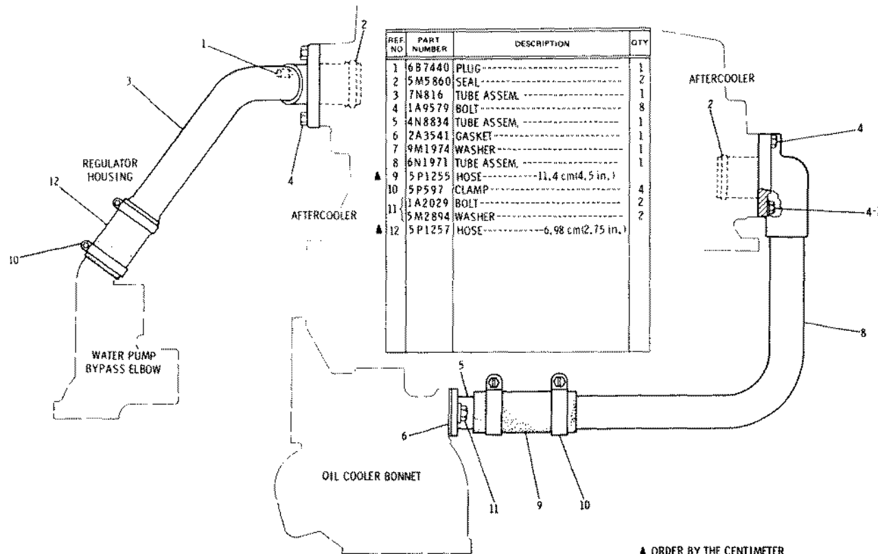
8N755 AFTERCOOLER WATER LINES GROUP
