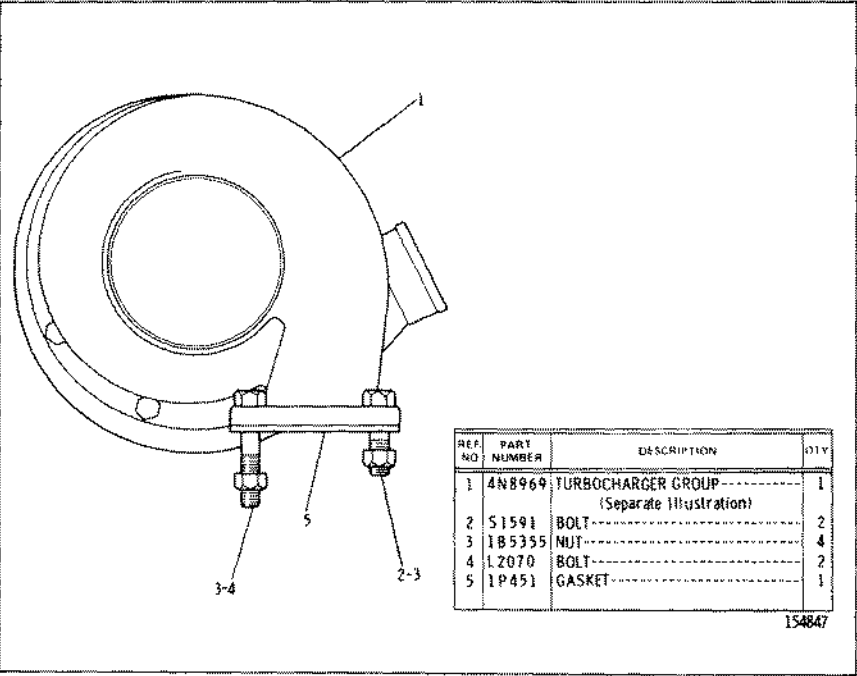
4N8970 TURBOCHARGER GROUP 4N8969 Turbocharger parts are shown on Page 149B
