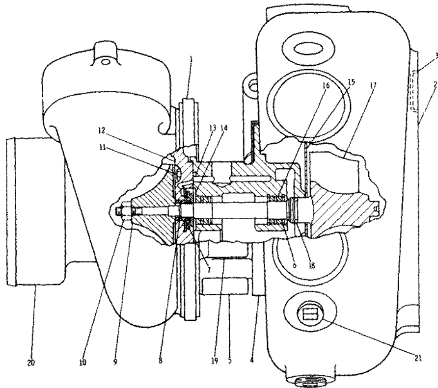
6N7509 TURBOCHARGER GROUP Part of 6N5961 Turbocharger Group shown on Page 144
