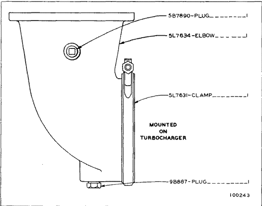
5L7661 EXHAUST ELBOW GROUP—5 in. FOR USE WITH WATER COOLED HOT TURBOCHARGERS
