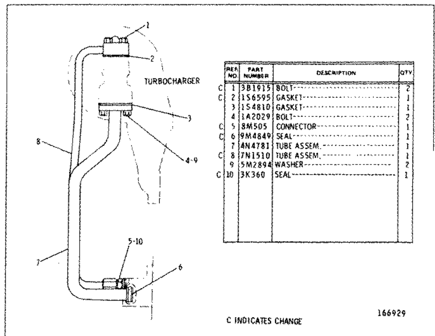
6N1305 TURBOCHARGER OIL LINES GROUP
