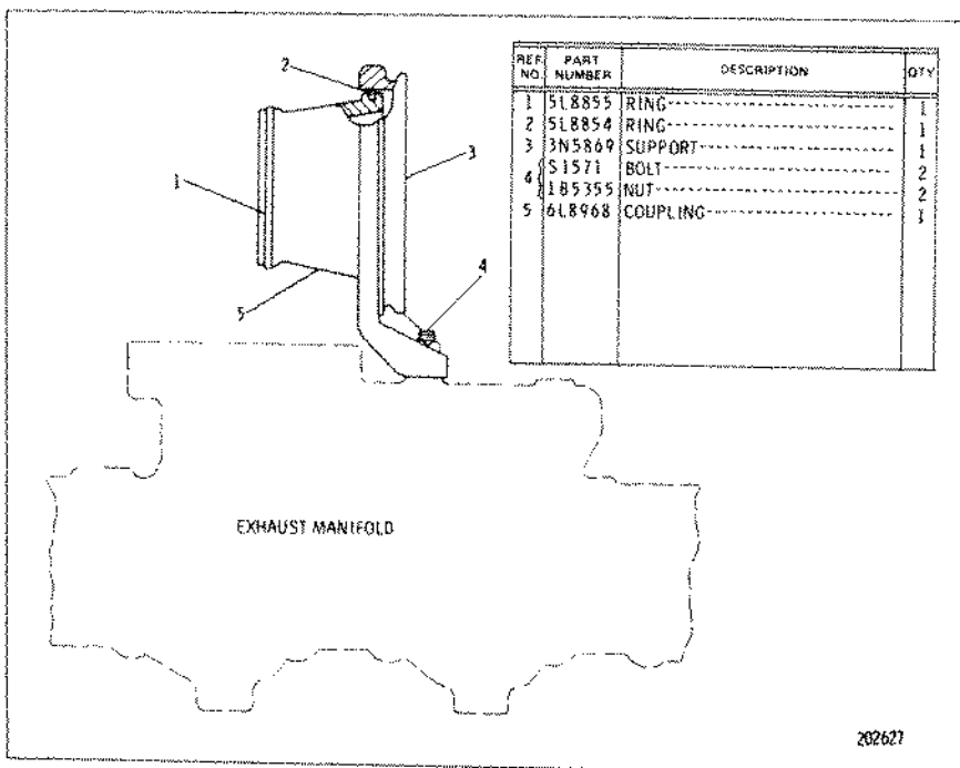
3N5870 EXHAUST ELBOW ADAPTER GROUP—Steiger Turbocharged Engine
