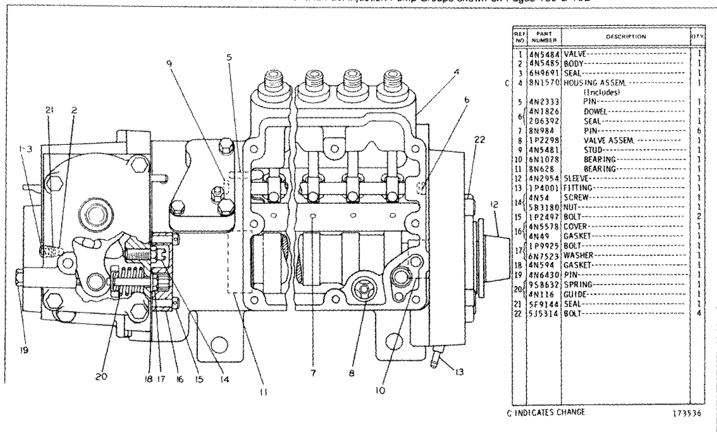
4N9754 GOVERNOR AND FUEL INJECTION PUMP GROUP—Part 2 of 4—Type 2 Part of 6N7613 & 6N271 Governor and Fuel Injection Pump Groups shown on Pages 189 & 192
