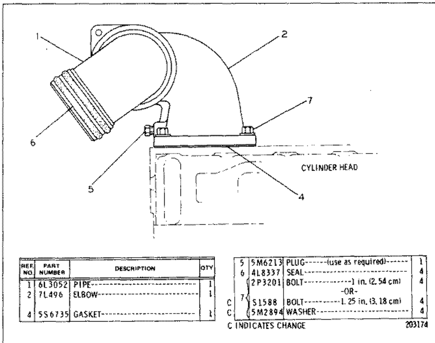
3N2880 AIR LINES GROUP
