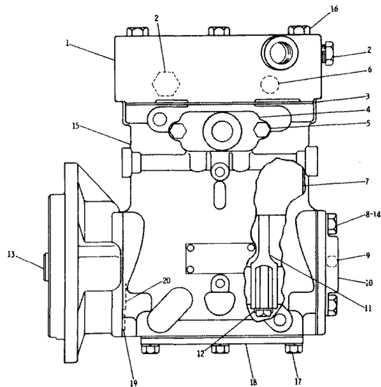
6N7582 AIR COMPRESSOR GROUP Part of 9N8069 Air Compressor Group shown on Page 167
