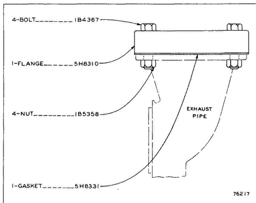
5L8601 EXHAUST FITTING GROUP—6 inch (152 mm) FOR USE WHEN 166 H.P. TO MAXIMUM H.P. IS SPECIFIED
