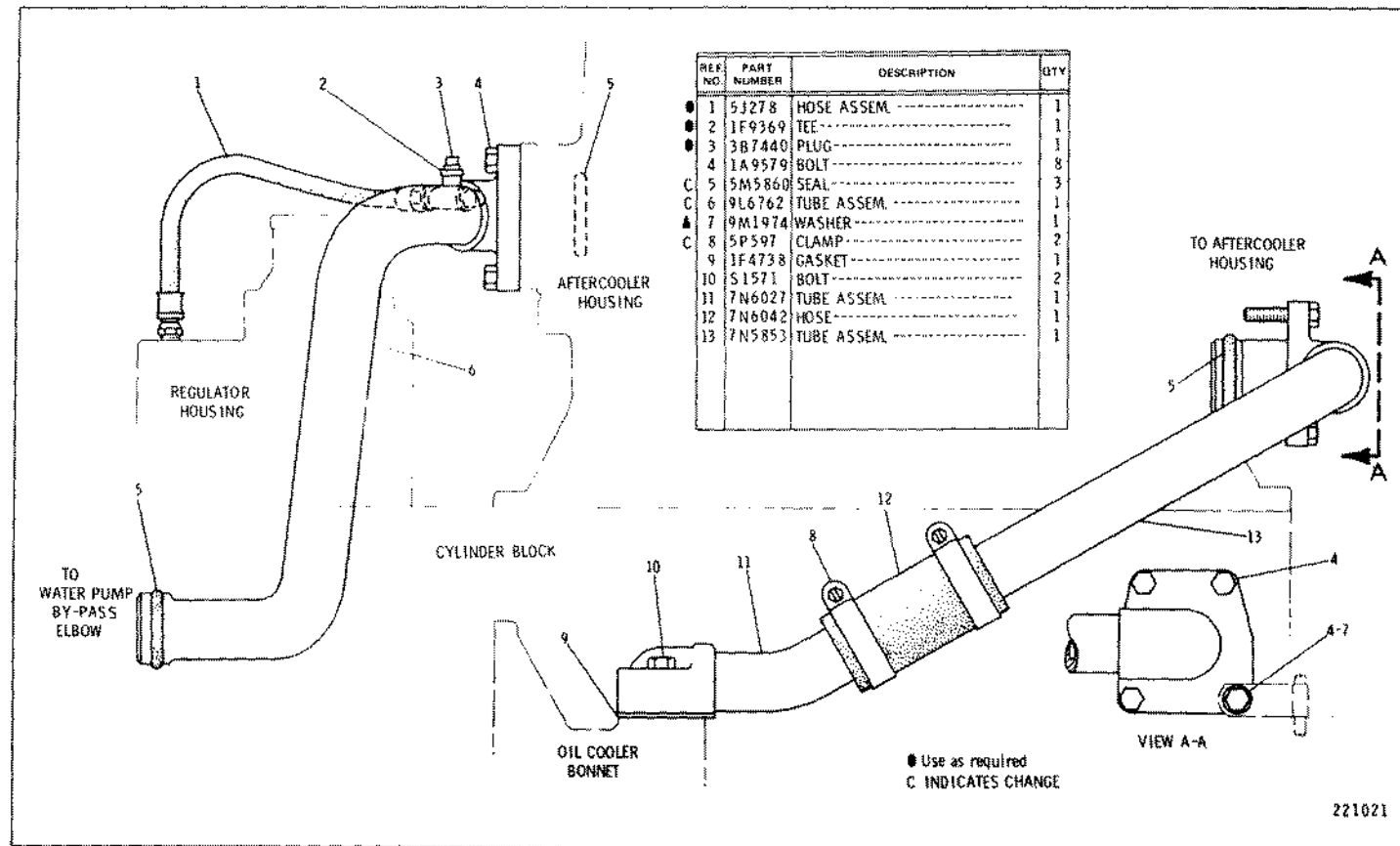
7N6055 AFTERCOOLER WATER LINES GROUP FOR USE WITH 7N3379 & 7N3386 ENGINE ARRANGEMENTS AN ATTACHMENT
