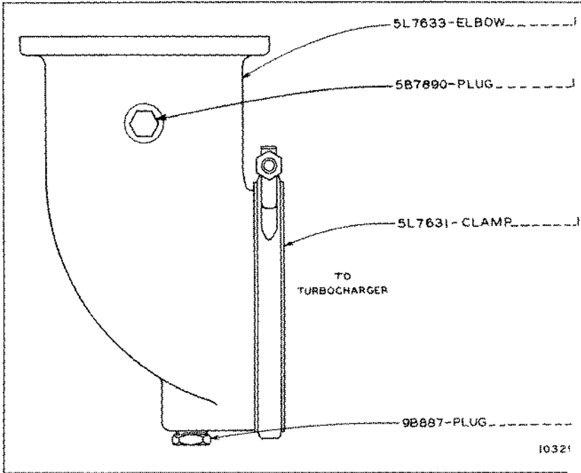
5L7660 EXHAUST ELBOW GROUP—4 Inch (102 mm) AN ATTACHMENT
