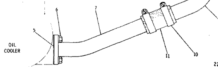
6N8492 AFTERCOOLER WATER LINES GROUP Serial No. 66D26832 to 66D33233 inclusive
