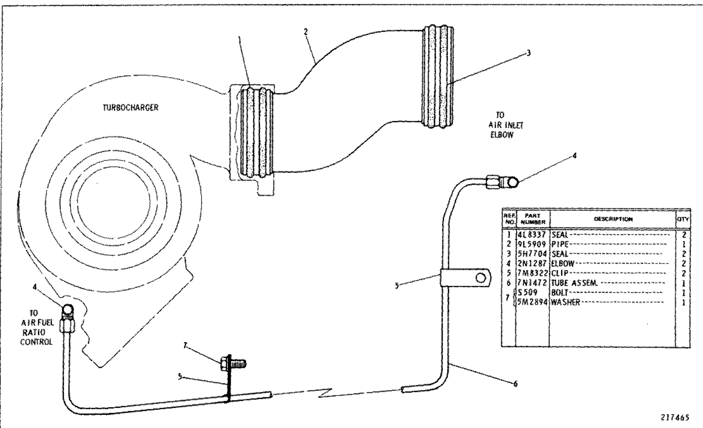
9N3262 AIR LINES GROUP
