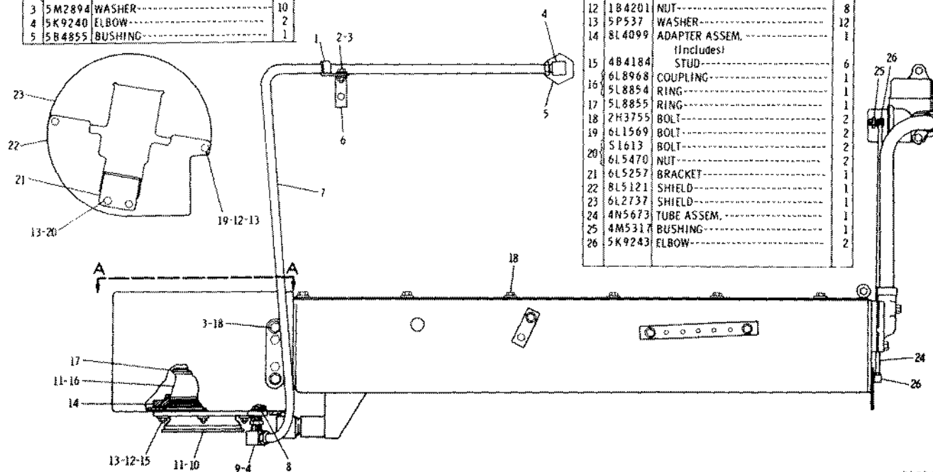
6N1302 MANIFOLD SHIELD GROUP—Water Cooled—Part 1—Type 1 Serial No. 66D26832 to 66D33233 inclusive CANNOT BE USED WITH TURBOCHARGED AFTERCOOLED ENGINE AN ATTACHMENT
