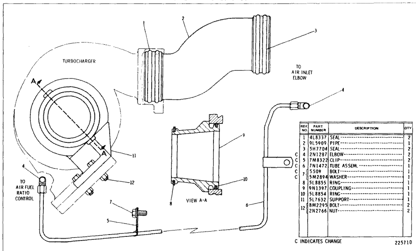
9N1247 AIR LINES GROUP
