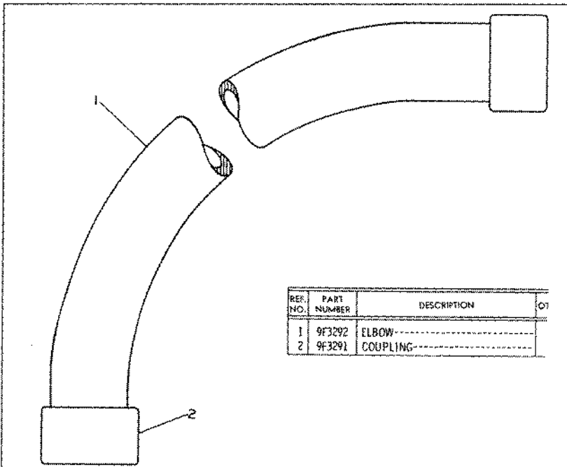
5L7660 Exhaust Elbow Group—5 Inch (127 mm)
