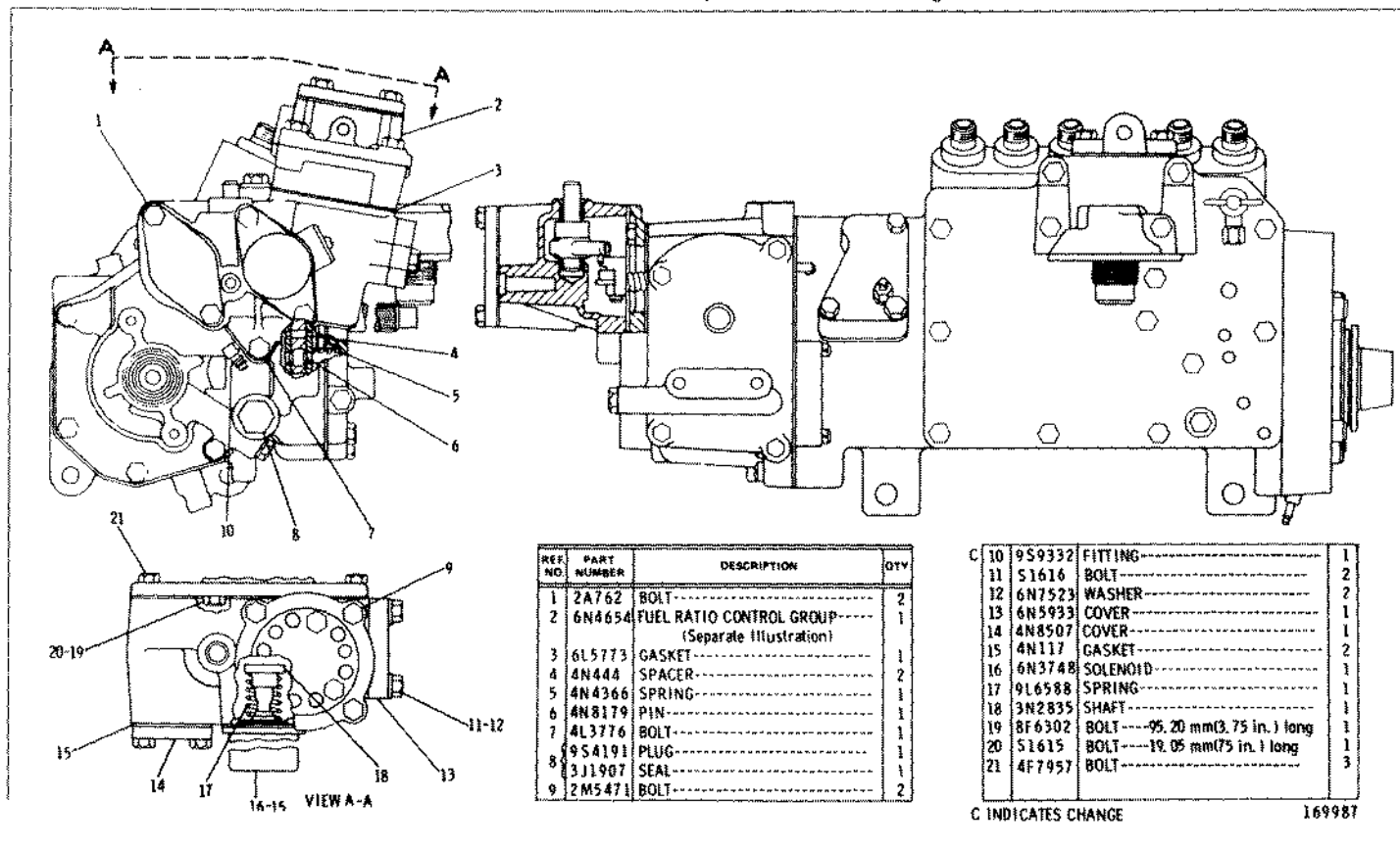
6N5275 GOVERNOR AND FUEL INJECTION PUMP GROUP—Part 2—Type 2 Part of 7N5304 Governor and Fuel Injection Pump Group shown on Pages 184 and 184A 6N4654 Fuel Ratio Control parts are shown on Page 224
