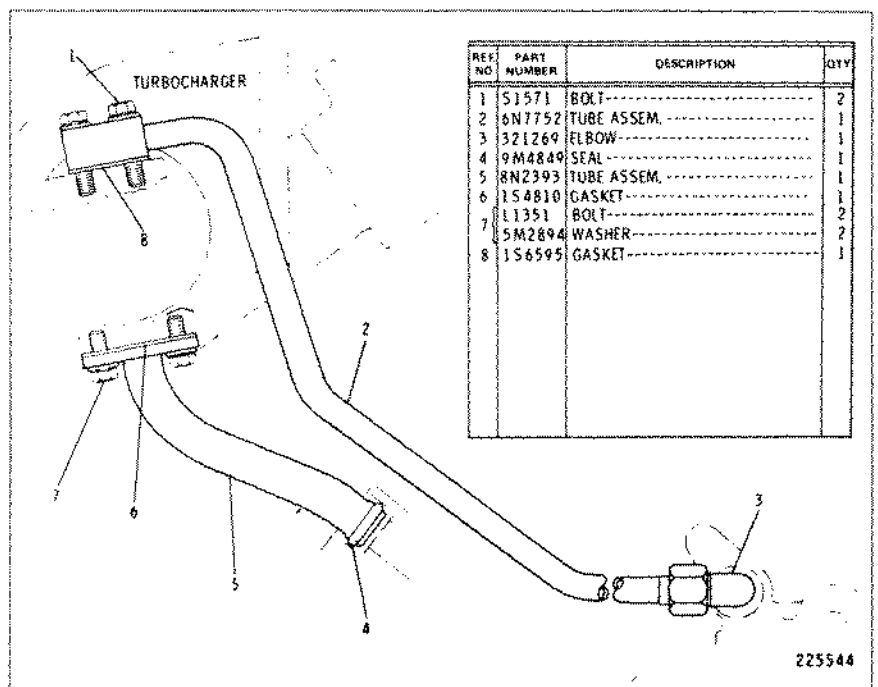
8N4572 TURBOCHARGER OIL LINES GROUP
