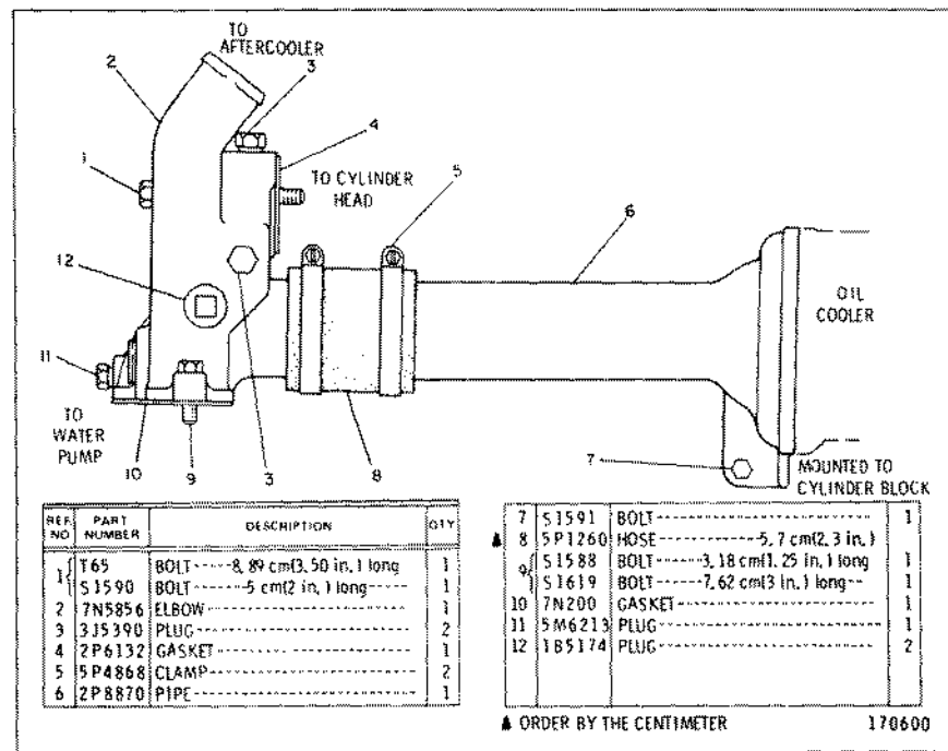
7N6587 WATER LINES GROUP
