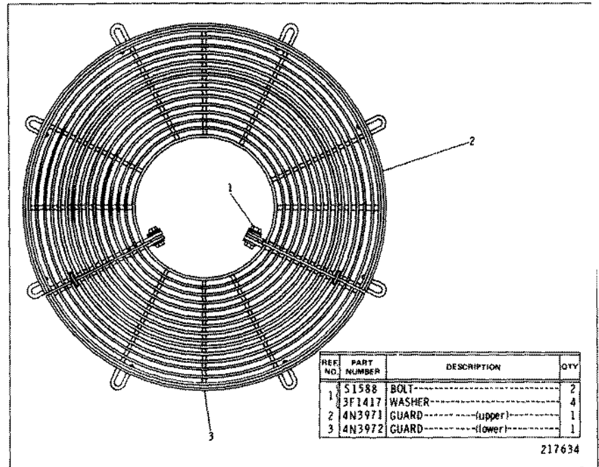
7N7077 FAN GUARD GROUP Part of 3N2789 and 3N7208 Radiator Groups shown on Pages 91 and 92 AN ATTACHMENT
