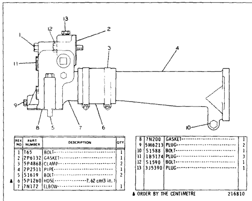
7N7211 WATER LINES GROUP
