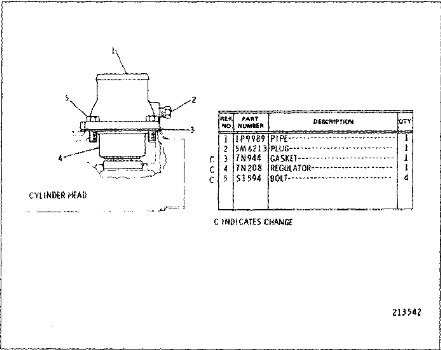
3N3271 HOUSING AND REGULATOR GROUP---Steiger Also available as an attachment for 7N3379, 7N3380, 7N3381, 7N3384, 7N3385, 7N3386, 7N3387, 7N6739 & 7N9638 Engine Arrangements
