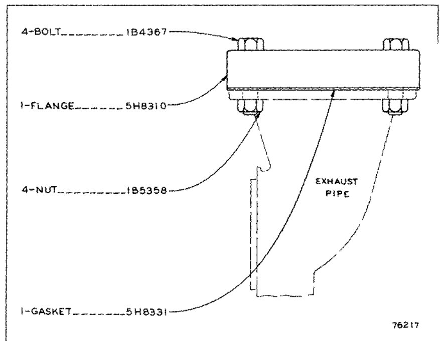
5L8601 EXHAUST FITTING GROUP—6 inch (152 mm) FOR USE WHEN 166 H.P. TO MAXIMUM H.P. IS SPECIFIED AN ATTACHMENT
