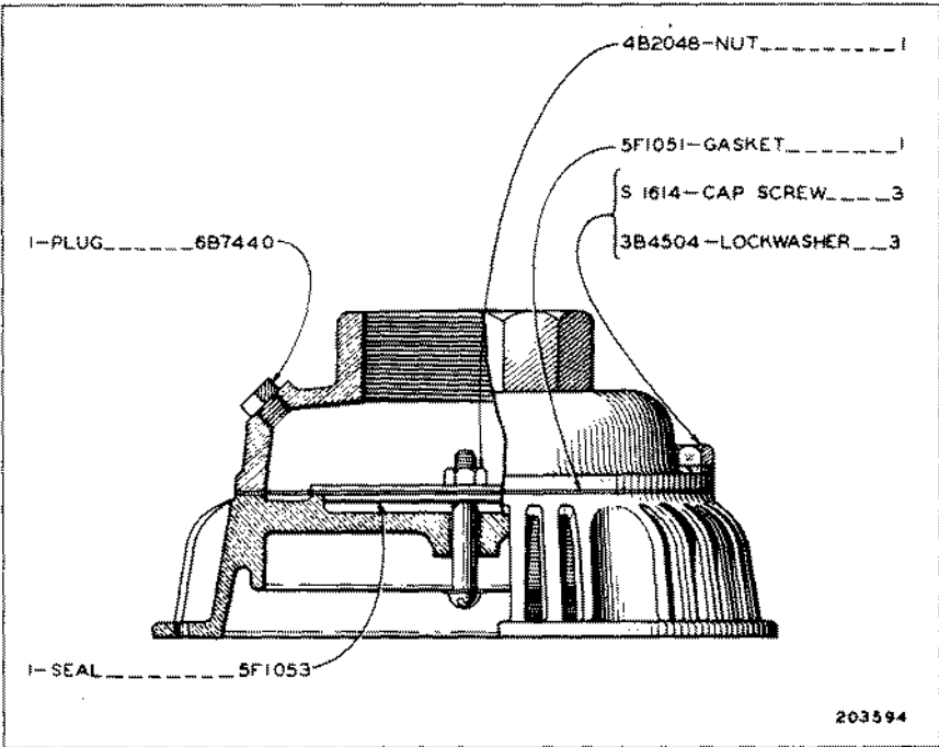
3F4394 FOOT VALVE AND STRAINER ASSEMBLY Part of 6L5858 Bilge Water Pump Group shown on Page 114 AN ATTACHMENT
