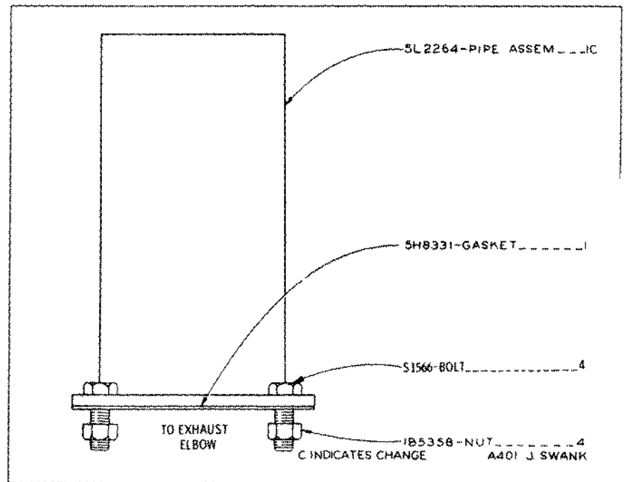
4L5801 EXHAUST PIPE GROUP—6 Inch (152 mm) AN ATTACHMENT
