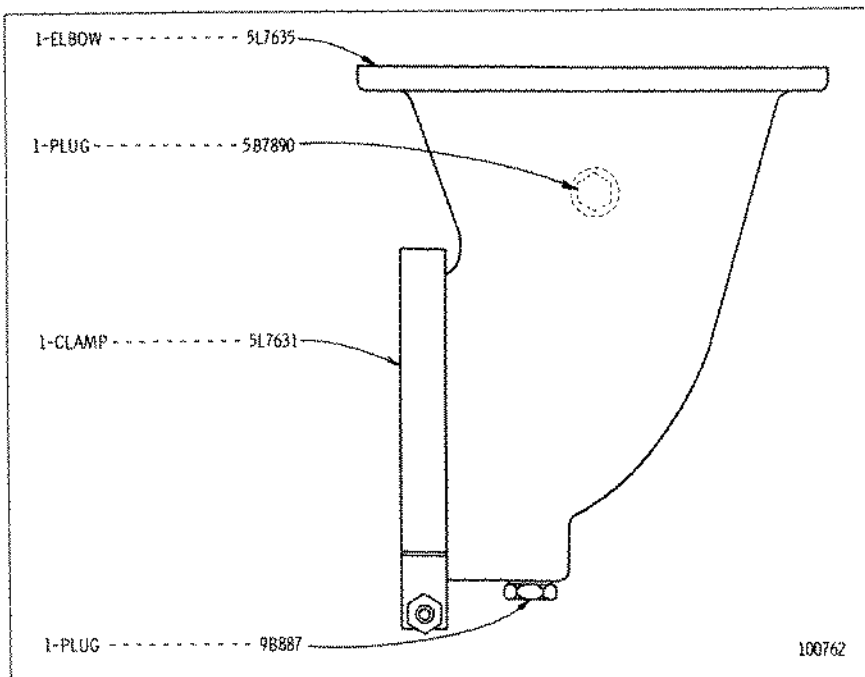
6L2927 EXHAUST ELBOW GROUP—6 Inch (152 mm) AN ATTACHMENT
