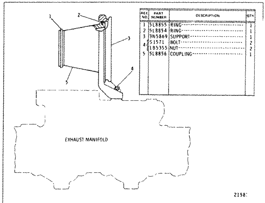
5N1768 EXHAUST ELBOW ADAPTER GROUP
