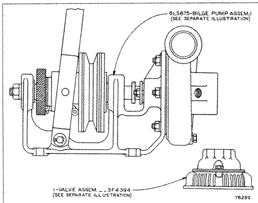
6L5858 BILGE WATER PUMP GROUP—Small Capacity FOR USE WITH MARINE AUXILIARY ENGINE 6L5875 Bilge Pump and 3F4394 Valve parts are shown on Pages 114 and 115 AN ATTACHMENT
