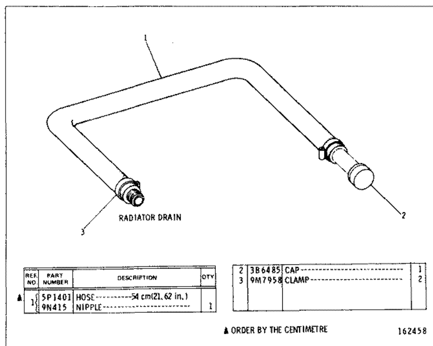
5N3869 COOLANT DRAIN LINES GROUP For use with 3N6267 Base Group shown on Page 381 AN ATTACHMENT
