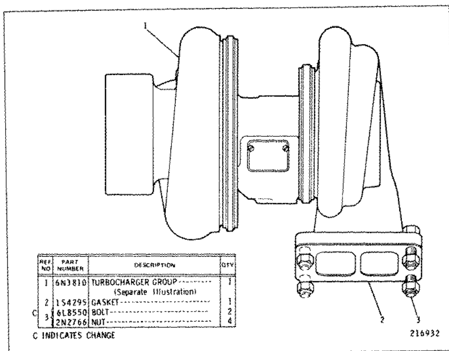
6N3744 TURBOCHARGER GROUP 6N3810 Turbocharger parts are shown on Page 150
