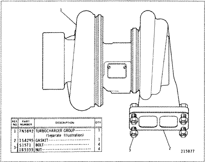
7N5890 TURBOCHARGER GROUP 7N5892 Turbocharger parts are shown on Page 156
