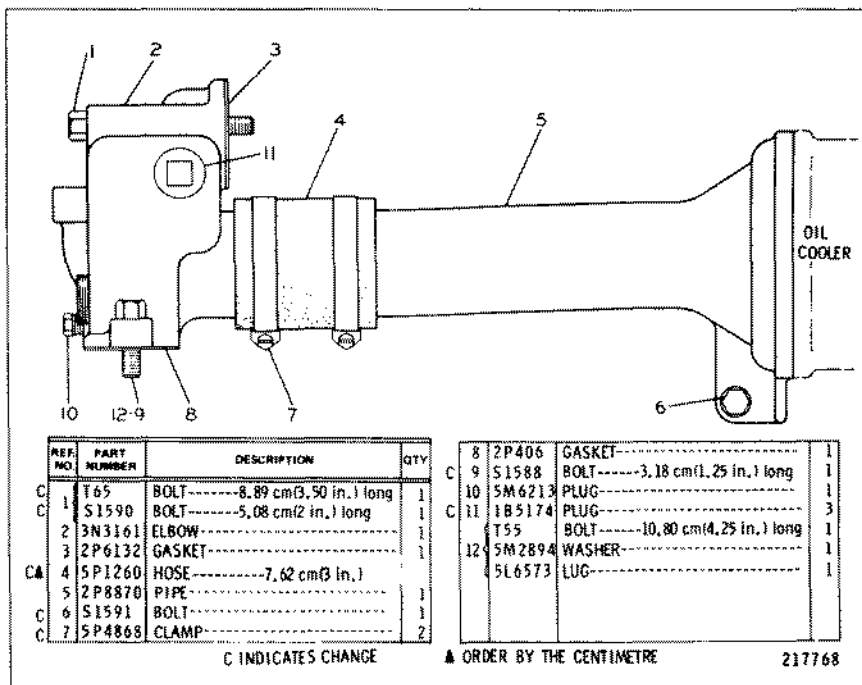
3N3914 WATER LINES GROUP—Marine Auxiliary Turbocharged Engine
