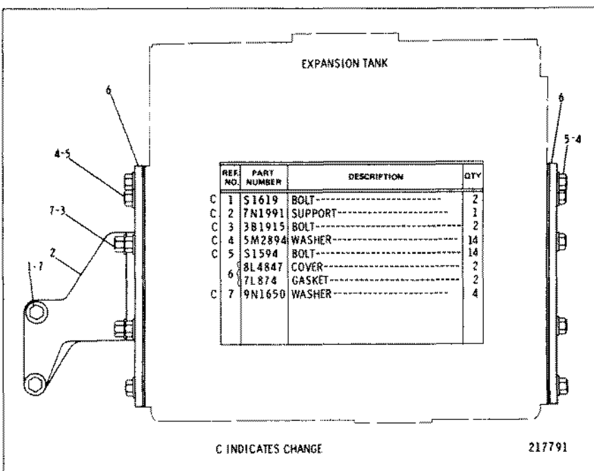
3N4924 EXPANSION TANK COVER GROUP FOR USE WITH EXPANSION TANK AND WITHOUT HEAT EXCHANGER Also part of 3N4921 Water Lines Group shown on Page 107 AN ATTACHMENT
