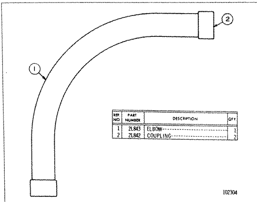
7L447 EXHAUST ELBOW GROUP—90 Degree Bend—6 Inch (152 mm) AN ATTACHMENT
