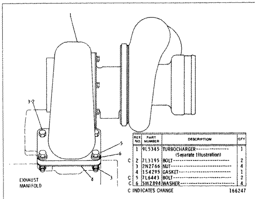
9L5802 TURBOCHARGER GROUP 9L5345 Turbocharger parts are shown on Page 149
