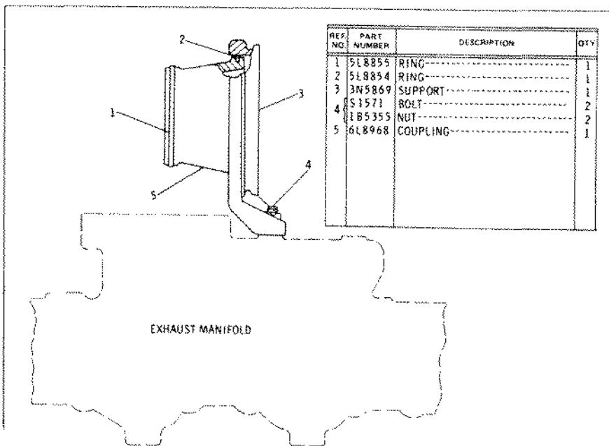
3N5870 EXHAUST ELBOW ADAPTER GROUP—Steiger Turbocor
