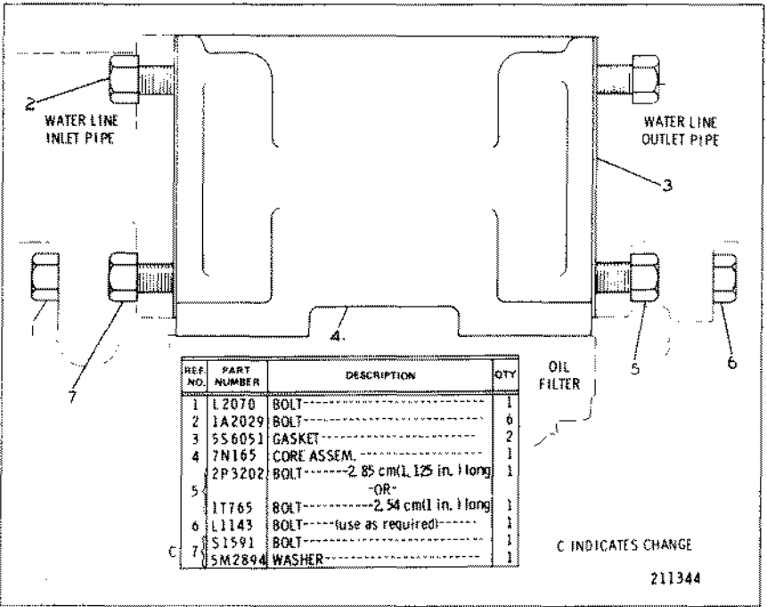
2P6215 ENGINE OIL COOLER GROUP
