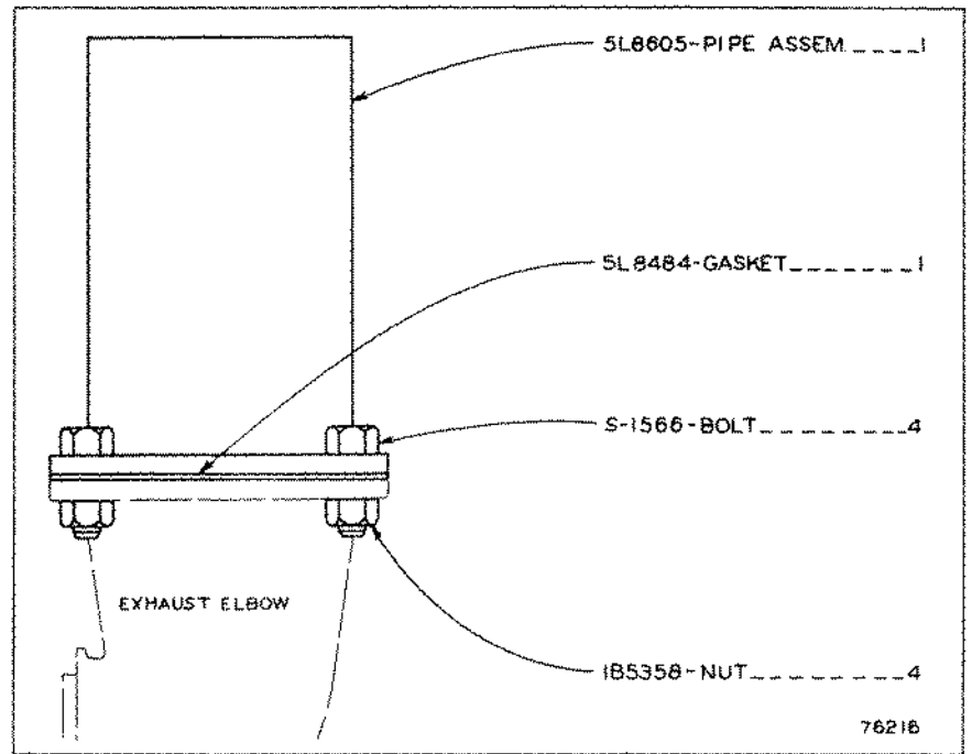
5L8632 EXHAUST PIPE GROUP—5 Inch (127 mm) AN ATTACHMENT
