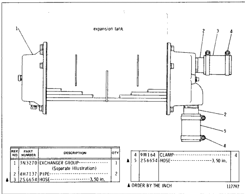
3N4925 HEAT EXCHANGER GROUP FOR USE WITHOUT AUXILIARY WATER PUMP & AUXILIARY WATER LINES AN ATTACHMENT
