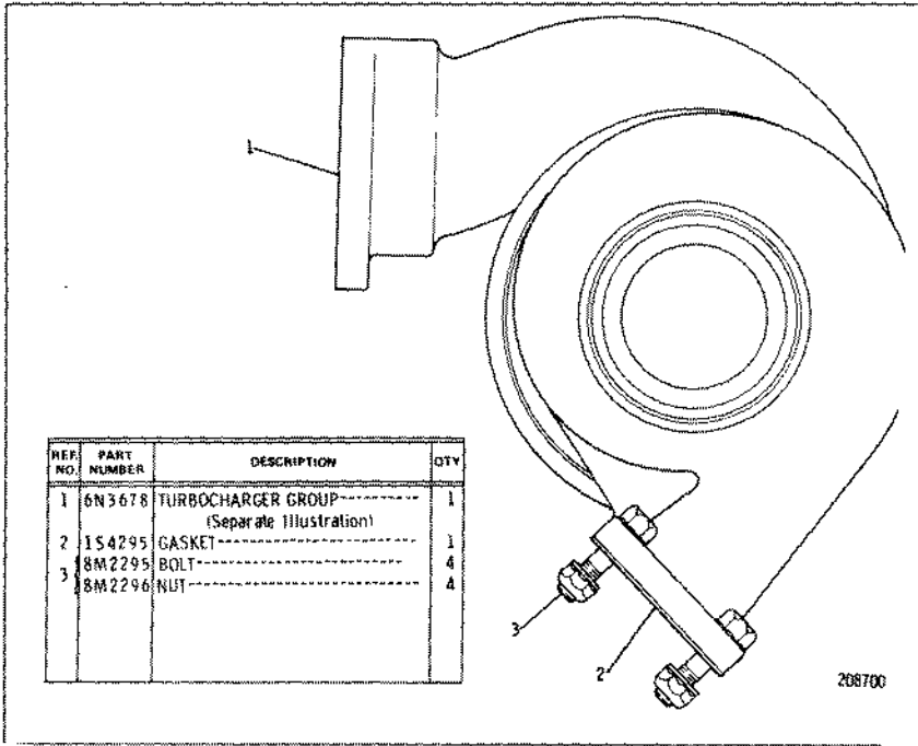
6N3678 TURBOCHARGER GROUP
