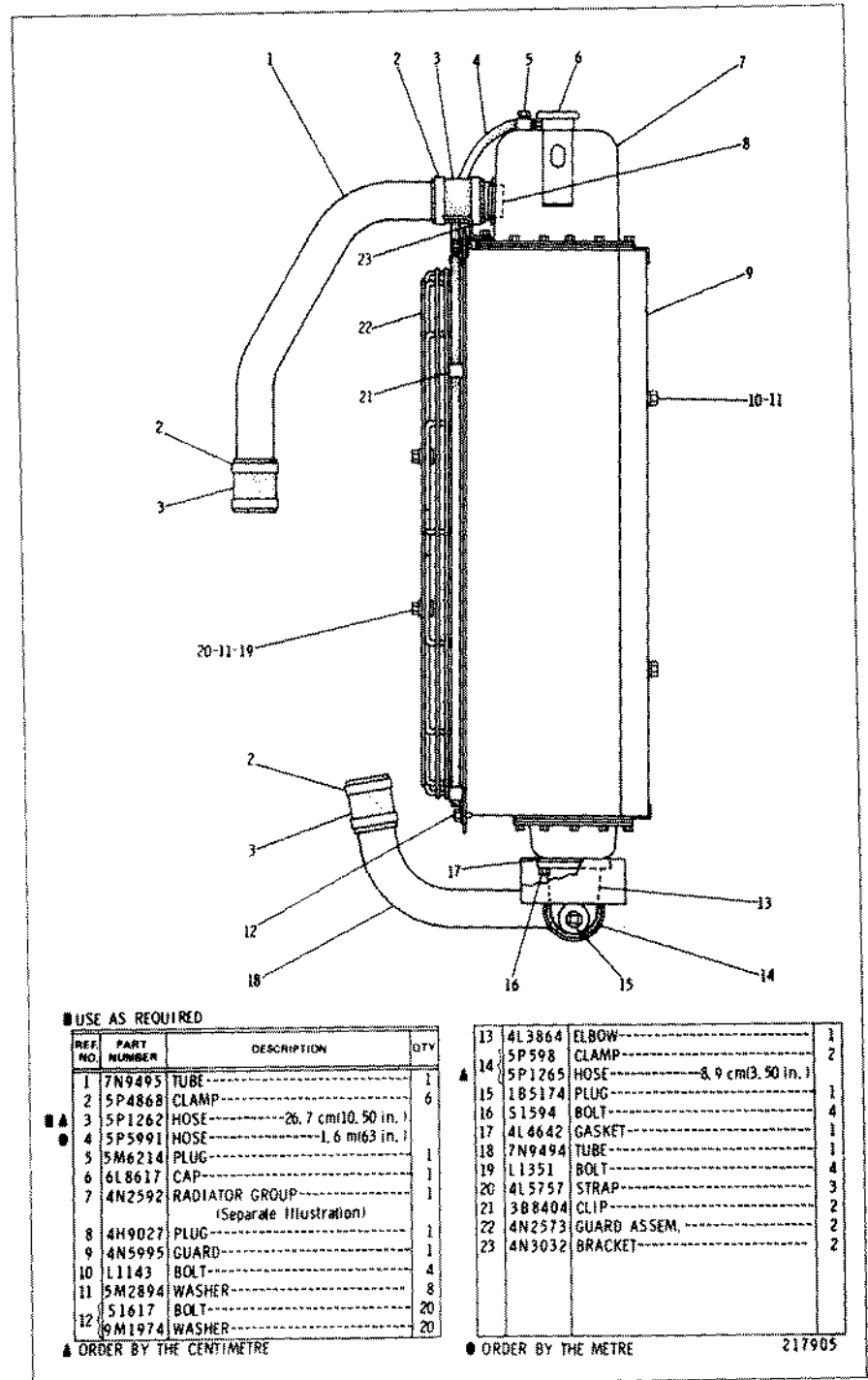
7N9517 RADIATOR GROUP—Type 1
