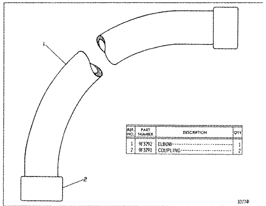
2N1273 EXHAUST ELBOW GROUP—90 Degree Bend—5 inch (127 mm) AN ATTACHMENT
