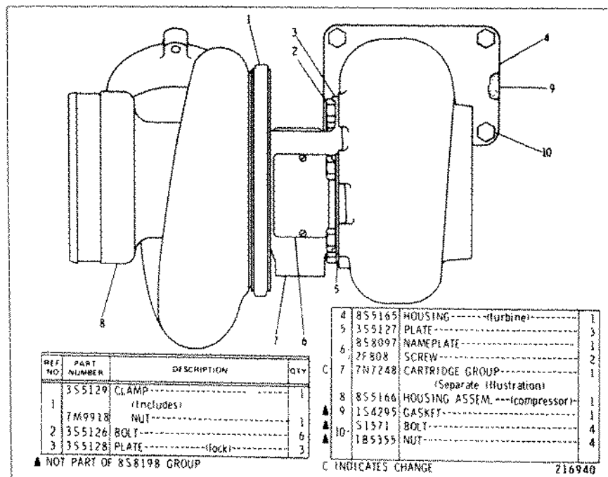
8S8198 TURBOCHARGER GROUP (8S8200 N/S)—Replaced by 8S8039 shown on Page 140 7N7248 Cartridge parts are shown on Page 158
