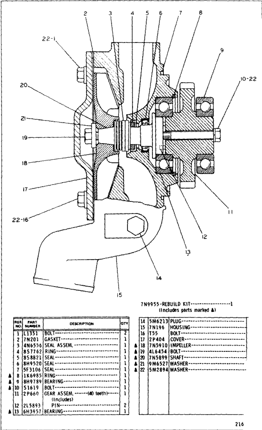
7N5909 WATER PUMP GROUP
