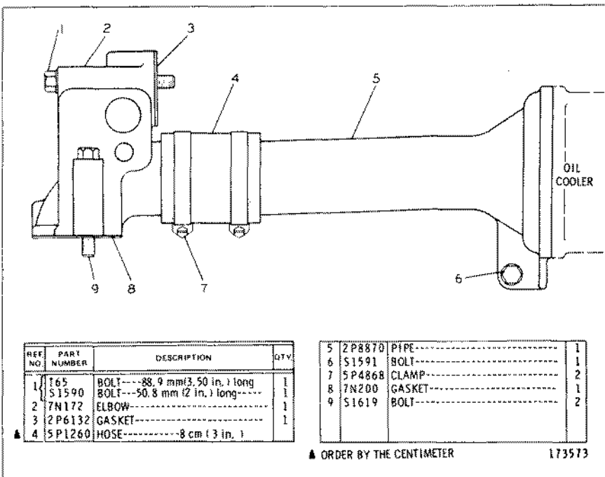
8N4527 WATER LINES GROUP
