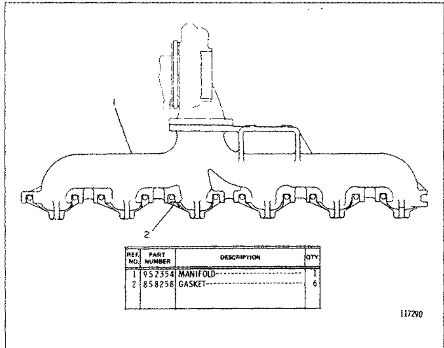
2P6573 EXHAUST MANIFOLD GROUP—Steiger—Ford & Industrial
