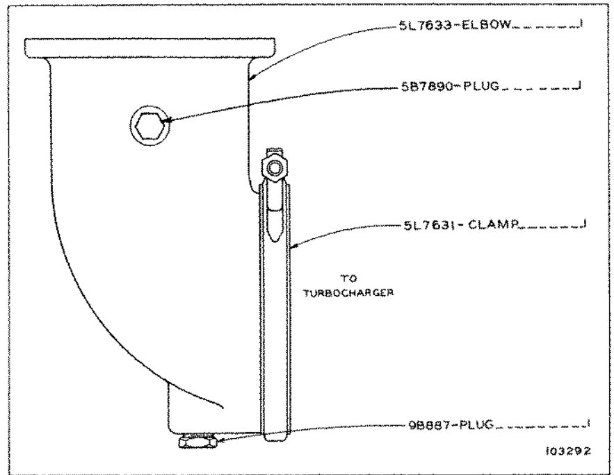
5L7660 EXHAUST ELBOW GROUP—4 inch (102 mm) AN ATTACHMENT
