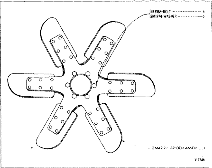
4N4684 BLOWER FAN GROUP—26 Inch (660 mm) Refer to Chart shown on Pages 126 and 127 for usage AN ATTACHMENT
