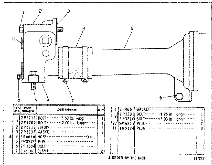
2P7730 WATER LINES GROUP—Turbocharged Engines
