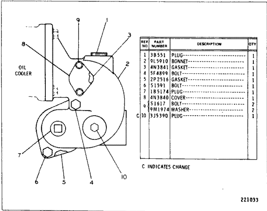
9N1245 WATER LINES GROUP—Elbow
