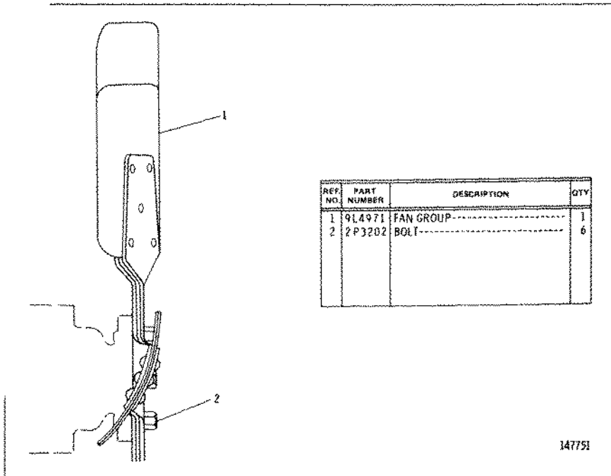
4N8752 SUCTION FAN GROUP—28 inch (711 mm) AN ATTACHMENT
