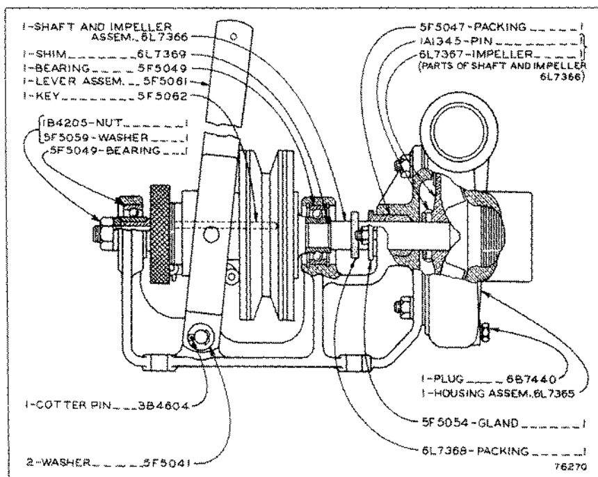
6L5875 BILGE WATER PUMP ASSEMBLY—R.H. Part of 6L5858 Bilge Water Pump Group AN ATTACHMENT
