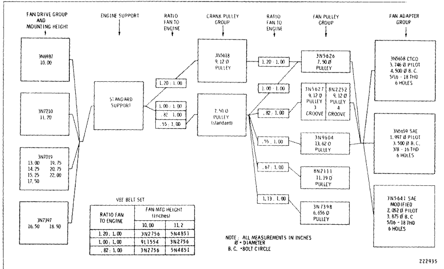
4N8585 FAN DRIVE CHART AN ATTACHMENT
