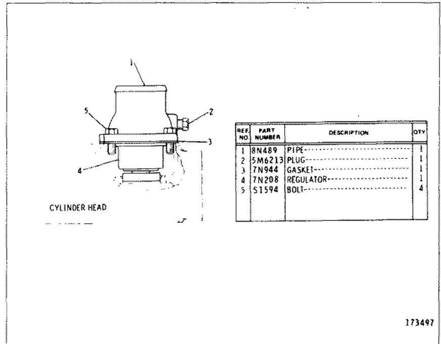
8N889 HOUSING AND REGULATOR GROUP
