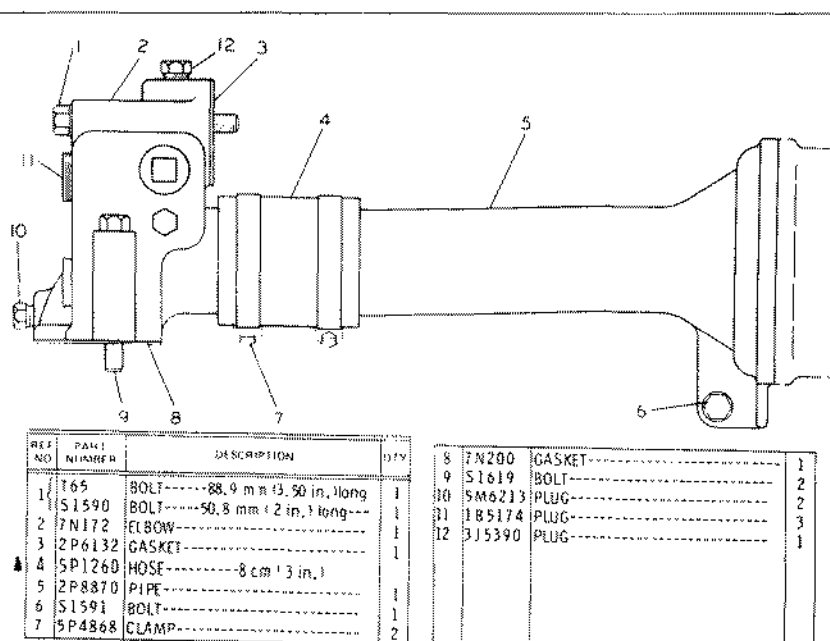
7N9905 WATER LINES GROUP
