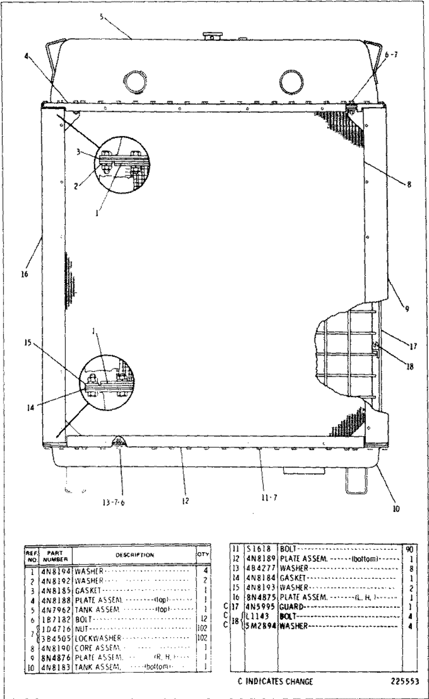
8N4874 RADIATOR GROUP Part of 7N9517 Radiator Group shown on Page 97A AN ATTACHMENT
