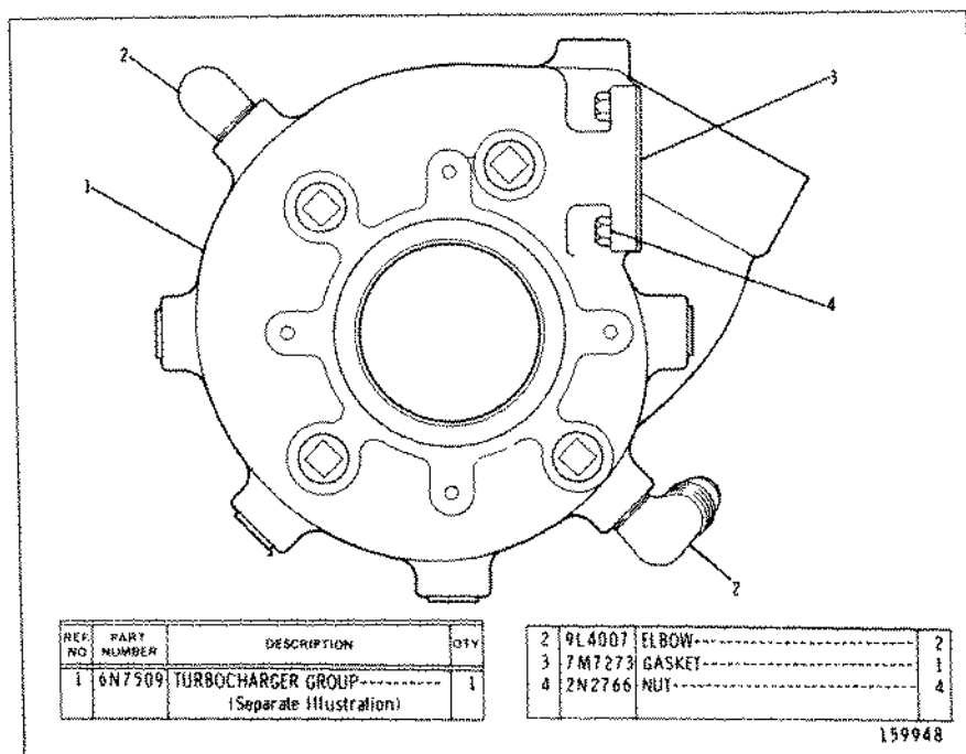
6N5961 TURBOCHARGER GROUP 6N7509 Turbocharger parts are shown on Page 150
