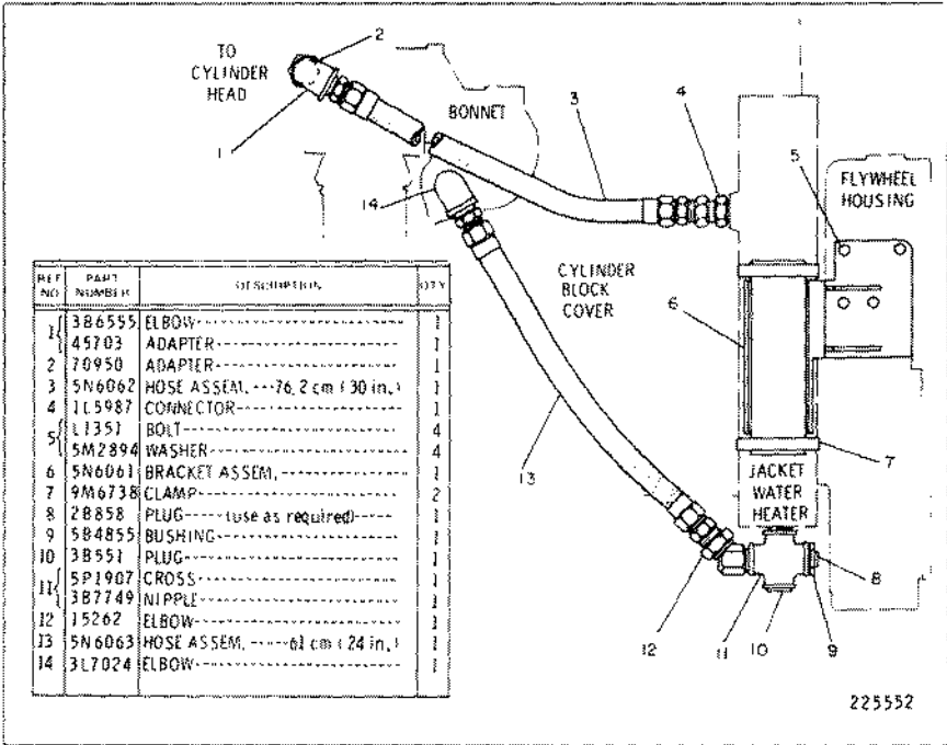
5N6064 JACKET WATER HEATER MOUNTING GROUP
