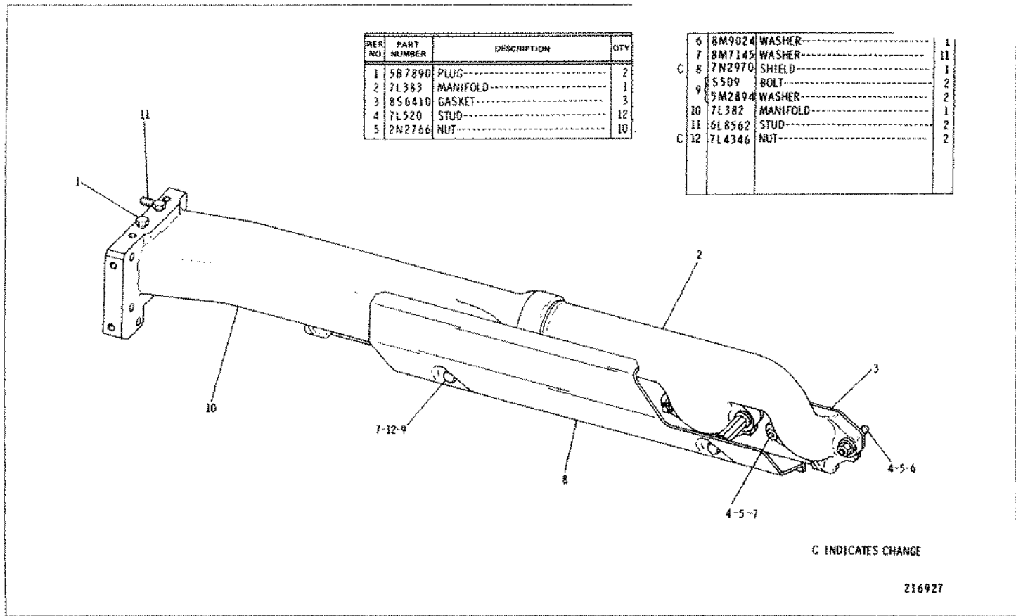
3N2888 EXHAUST MANIFOLD GROUP
