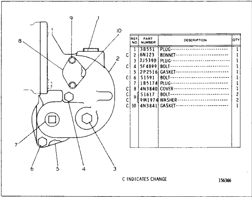
2P7728 WATER LINES GROUP—Elbow
