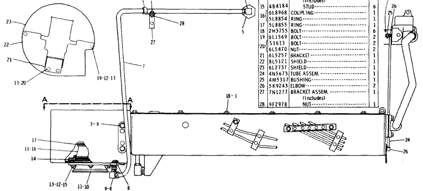
8N865 MANIFOLD SHIELD GROUP—Water Cooled—Part 1 Serial No. 66D33234—Up. AN ATTACHMENT
