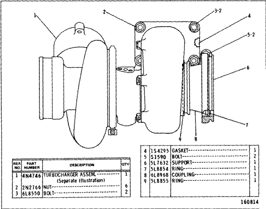
6N9296 TURBOCHARGER GROUP 4N4746 Turbocharger parts are shown on Page 153
