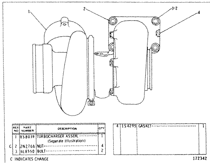
3N2882 TURBOCHARGER GROUP Serial No. 66D27000—Un 8S8039 Turbocharger
