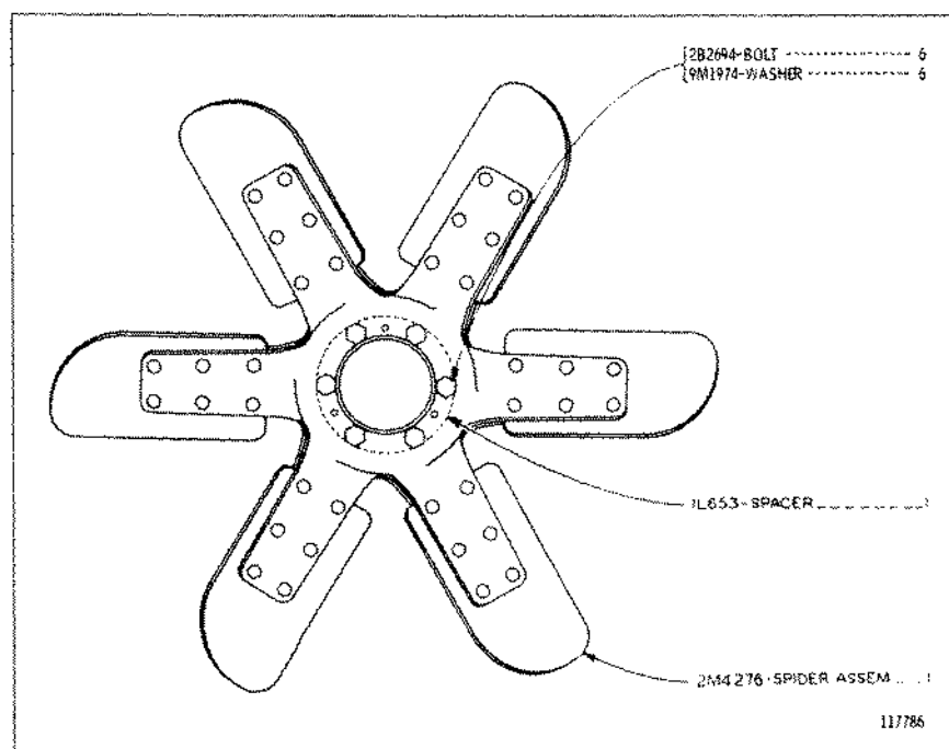
4N4683 SUCTION FAN GROUP—26 Inch (660 mm) Refer to Chart shown on Pages 126 and 127 for usage AN ATTACHMENT
