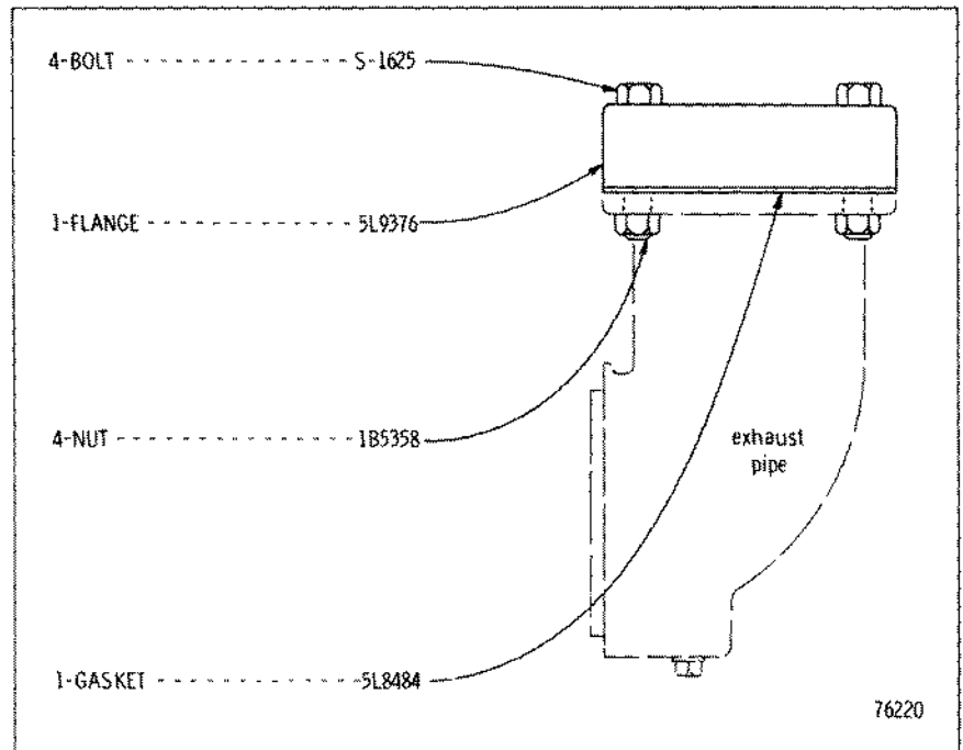
5L9377 EXHAUST FITTING GROUP—5 inch (127 mm) AN ATTACHMENT
