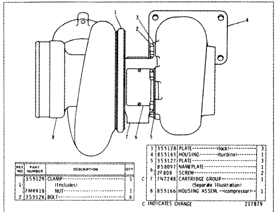
8S8039 TURBOCHARGER GROUP—Field Installation Also part of 3N2882 Turbocharger Group shown on Page 147 7N7248 Cartridge parts are shown on Page 158
