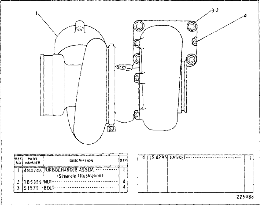
8N4172 TURBOCHARGER GROUP 4N4746 Turbocharger parts are shown on Page 153
