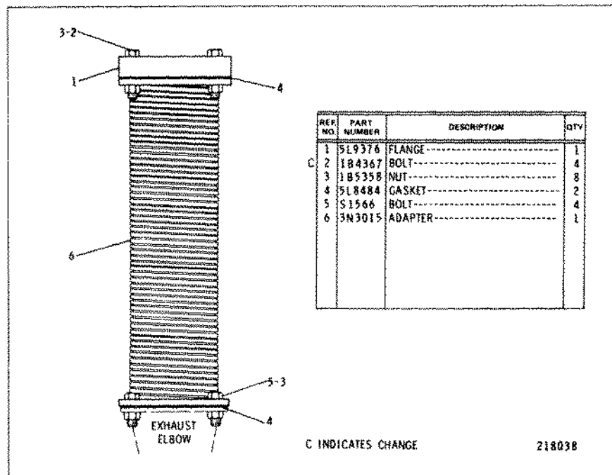
3N3016 VERTICAL EXHAUST FITTING GROUP—5 Inch (127 mm) AN ATTACHMENT
