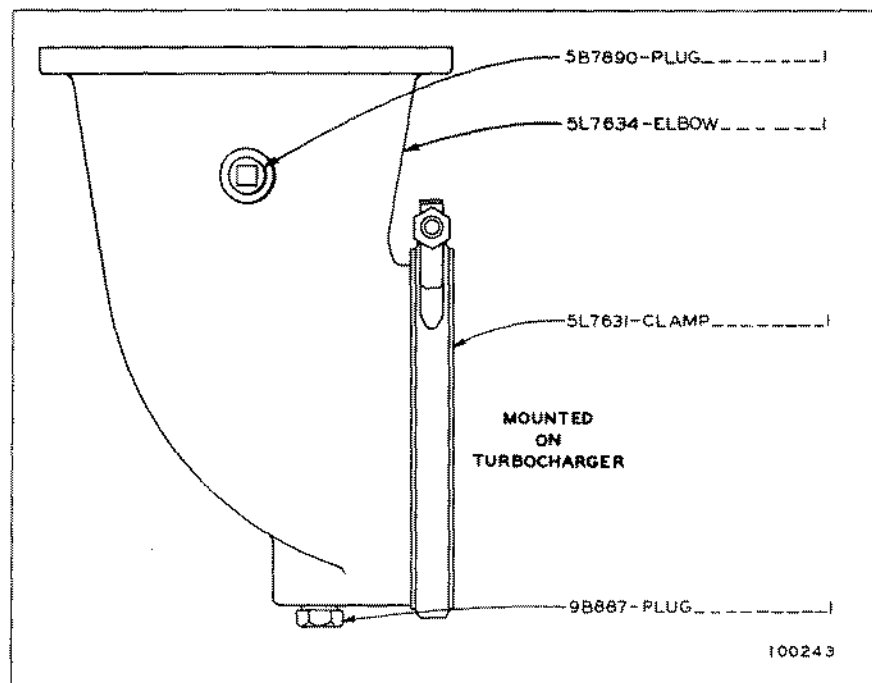
5L7661 EXHAUST ELBOW GROUP—5 in. FOR USE WITH WATER COOLED HOT TURBOCHARGER
