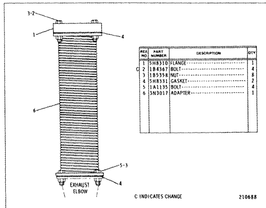
3N3018 VERTICAL EXHAUST FITTING GROUP—6 Inch (152 mm) AN ATTACHMENT
