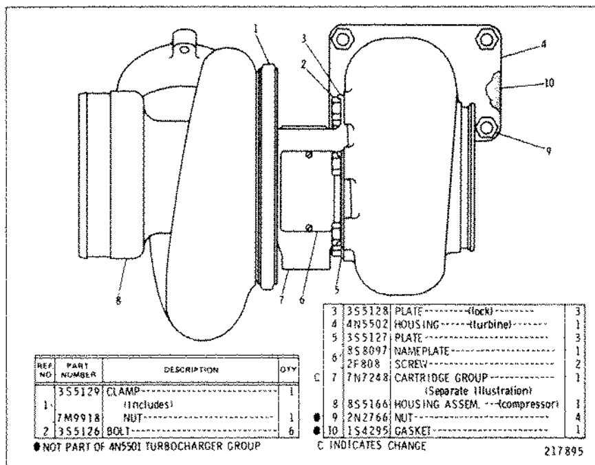
4N5501 TURBOCHARGER GROUP (3N3280 N/S) 7N7248 Cartridge parts are shown on Page 158
