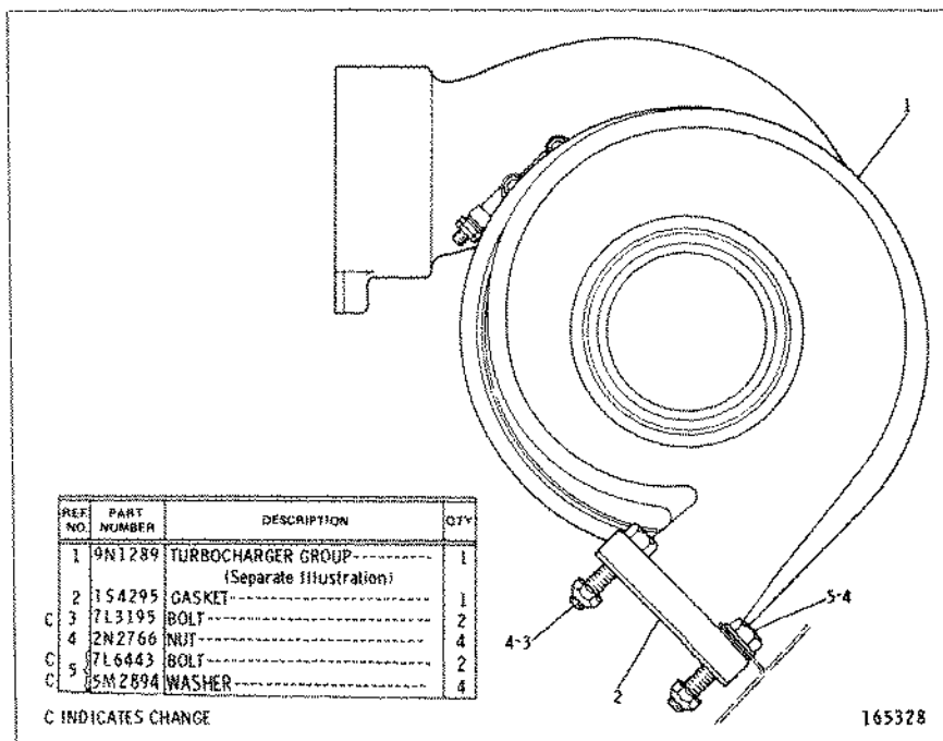
9N1290 TURBOCHARGER GROUP 9N1289 Turbocharger parts are shown on Page 155
