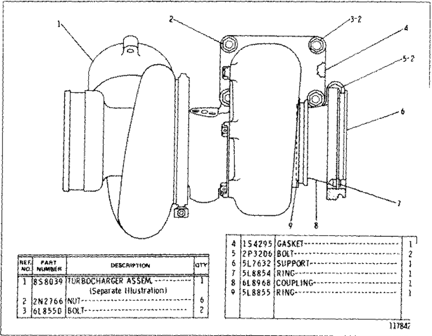
3N2882 TURBOCHARGER GROUP Serial No. 66D26832 to 66D26999 inclusive parts are shown on Page 149
