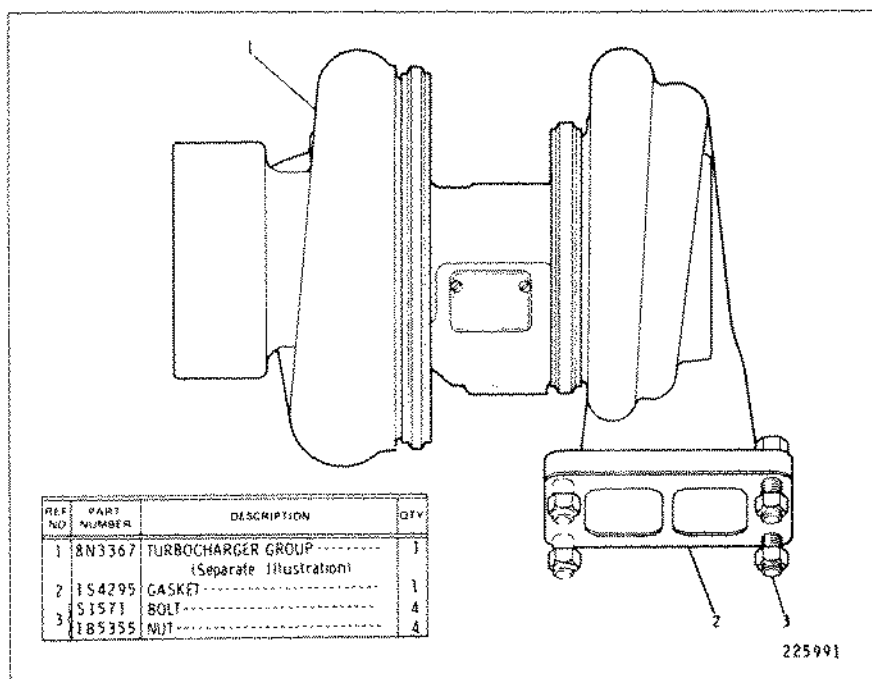
8N3382 TURBOCHARGER GROUP 8N3367 Turbocharger parts are shown on Page 150A
