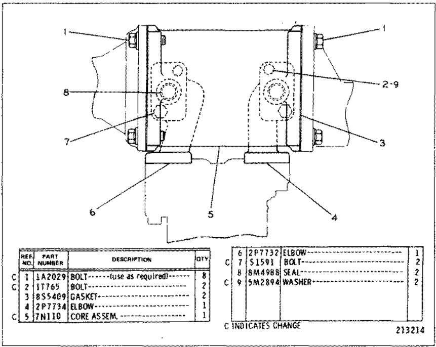
2P7738 ENGINE OIL COOLER GROUP
