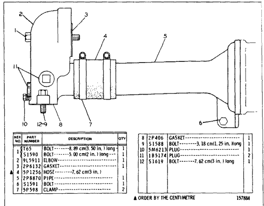
9N1246 WATER LINES GROUP—Turbocharged—Aftercooled Engine
