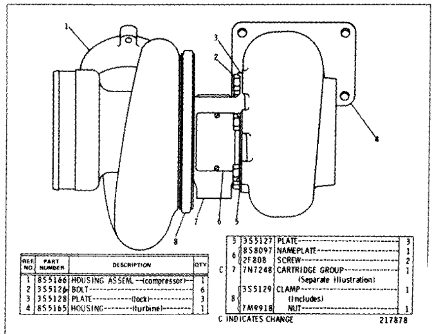
9L5345 TURBOCHARGER GROUP Part of 9L5802 Turbocharger Group shown on Page 146 7N7248 Cartridge parts are shown on Page 158
