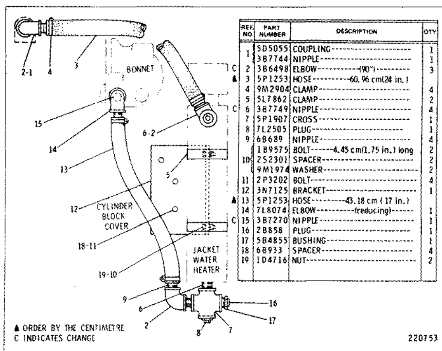
3N6728 JACKET WATER HEATER MOUNTING GROUP—Type 2 Serial No. 66D26832 to 66D32125 inclusive. Part of Jacket Water Heater and Mounting
