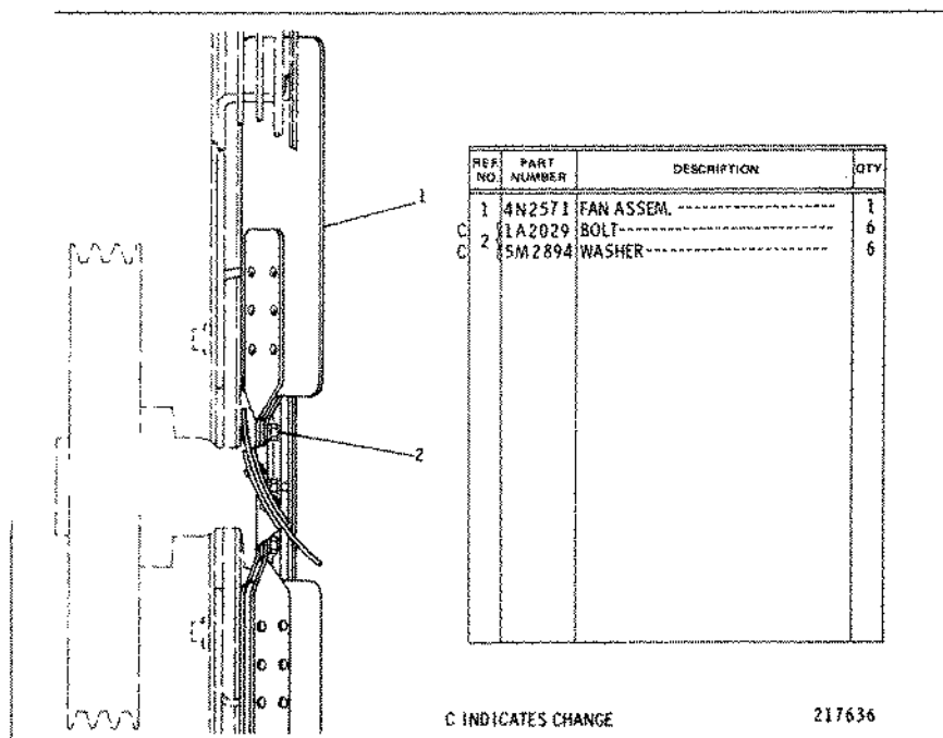
4N2569 BLOWER FAN GROUP—33 Inch (838 mm) Refer to Chart shown on Pages 126 and 127 for usage AN ATTACHMENT
