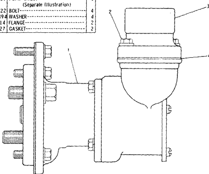
3N4927 AUXILIARY PUMP GROUP—Sea Water AN ATTACHMENT
