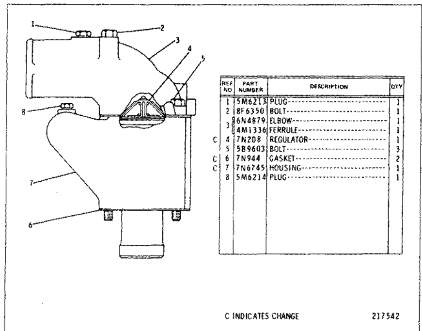
6N5782 HOUSING AND REGULATOR GROUP FOR USE WITH 7N3382 ENGINE ARRANGEMENT AN ATTACHMENT
