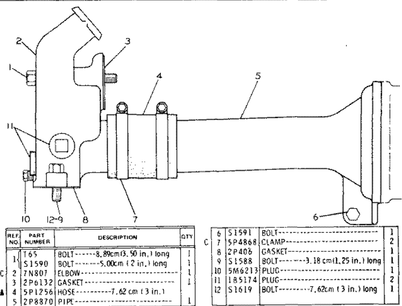
9N1246 WATER LINES GROUP—Turbocharged Aftercooled Engine—Type 2
