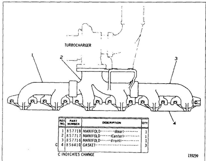
2P6574 EXHAUST MANIFOLD GROUP—Steiger & Mobile Engine
