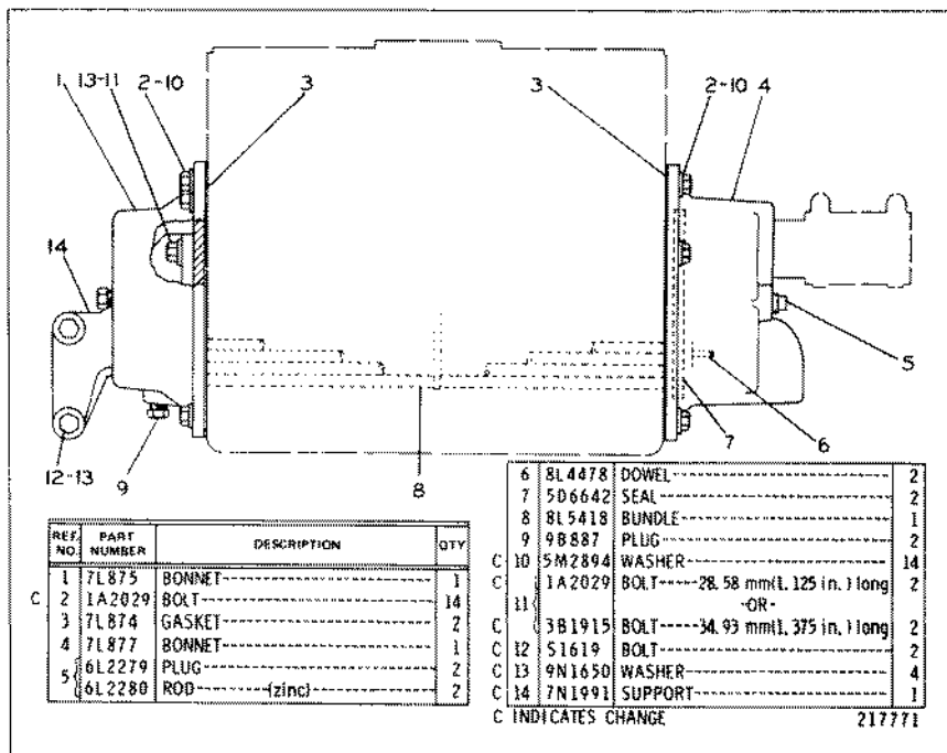
3N3270 HEAT EXCHANGER GROUP FOR USE WITH EXPANSION TANK AND AUXILIARY WATER LINES
