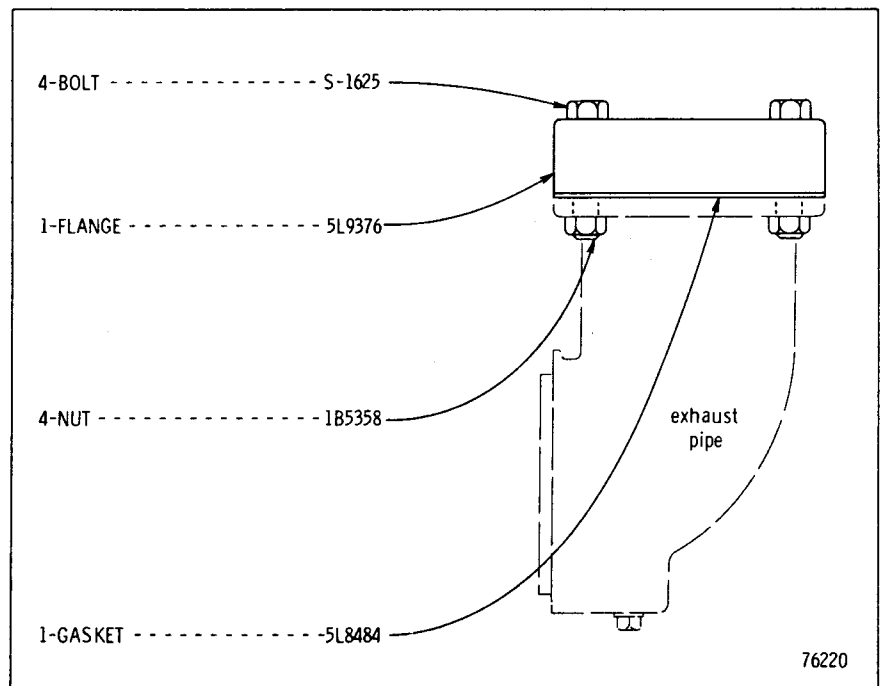
4L5801 EXHAUST PIPE GROUP—6 Inch Only separate parts serviced. AN ATTACHMENT
