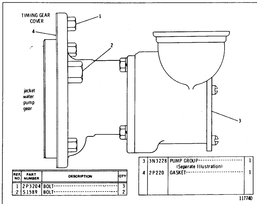
3N3229 AUXILIARY PUMP GROUP—Sea Water
