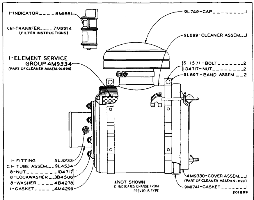
9L463 AIR CLEANER GROUP FOR USE WITH MOBILE APPLICATION ENGINE AN ATTACHMENT
