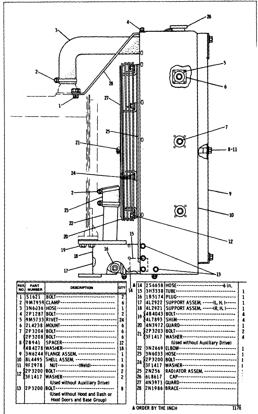
3N6694 RADIATOR GROUP—High Capacity FOR USE WITH DUCT FLANGE. AN ATTACHMENT
