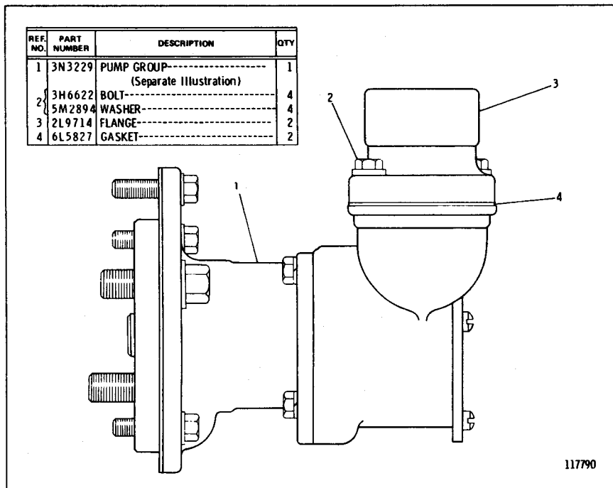
3N4927 AUXILIARY PUMP GROUP—Sea Water 3N3229 Pump parts are shown on Page 66 AN ATTACHMENT
