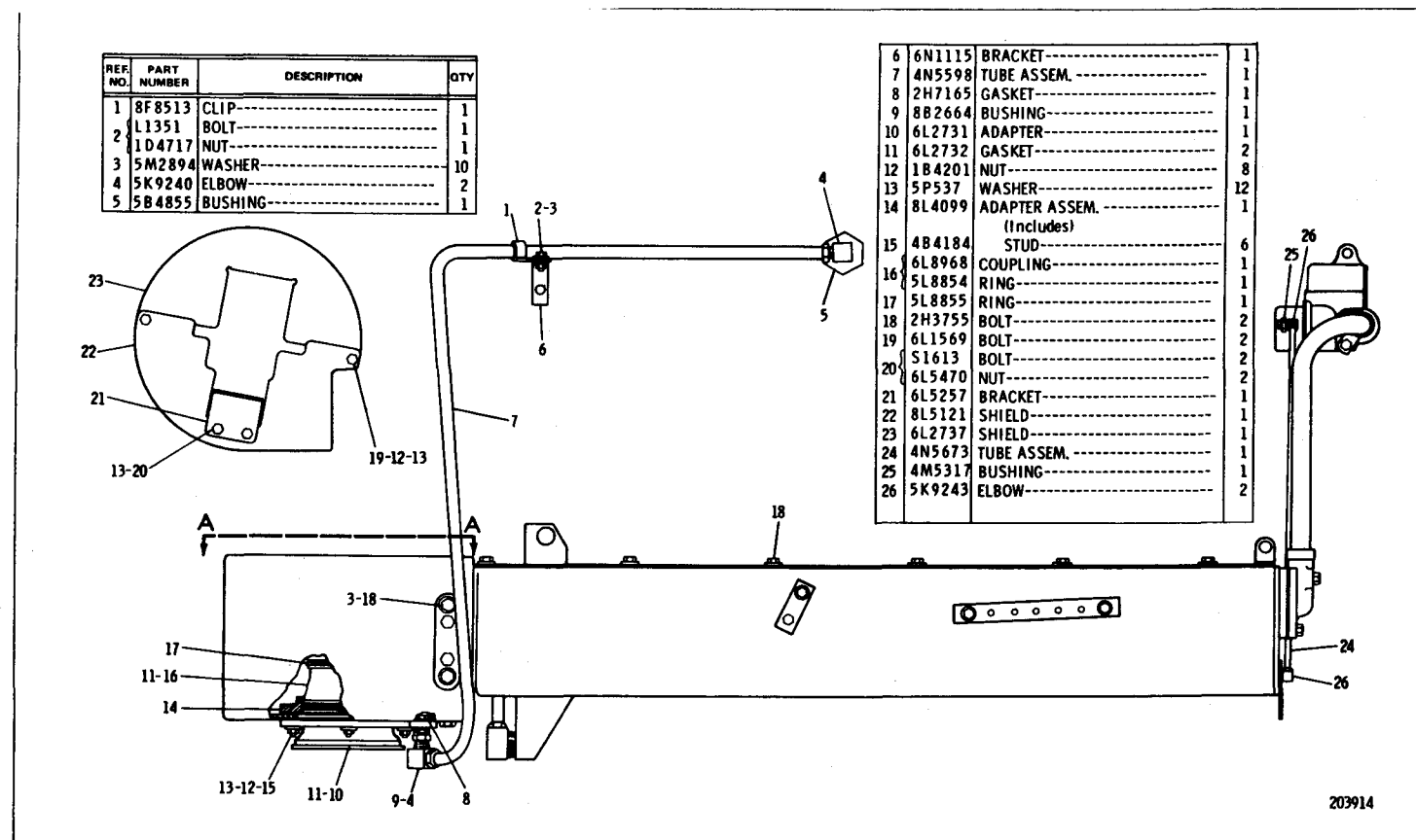
6N1302 MANIFOLD SHIELD GROUP—Water Cooled—Part 1 AN ATTACHMENT
