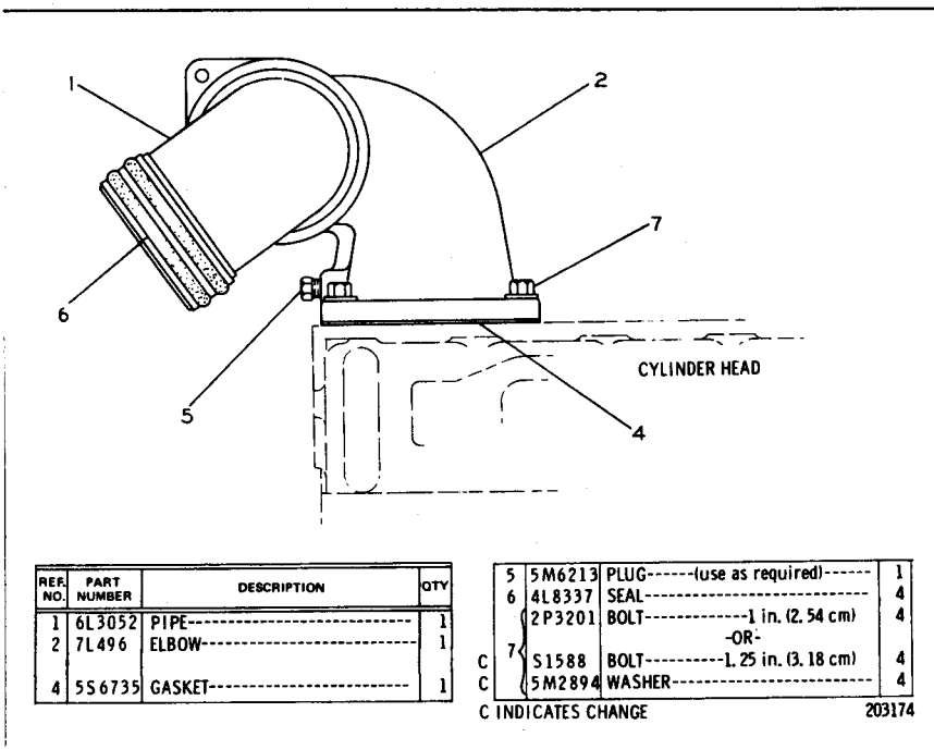
AIR LINES (3N2880 N/S)
