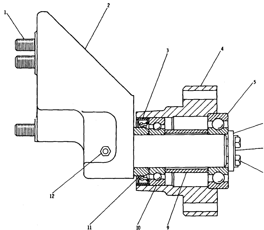
3N6987 FAN DRIVE GROUP Refer to Chart shown on Page 77 for usage. AN ATTACHMENT
