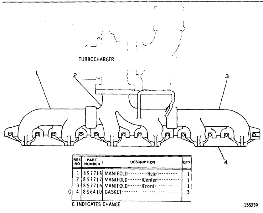
2P6574 EXHAUST MANIFOLD GROUP
