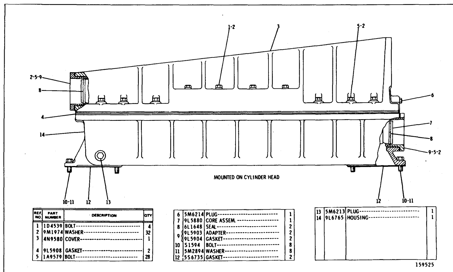
6N3745 AFTERCOOLER WATER GROUP Serial No. 66D17936-Up
