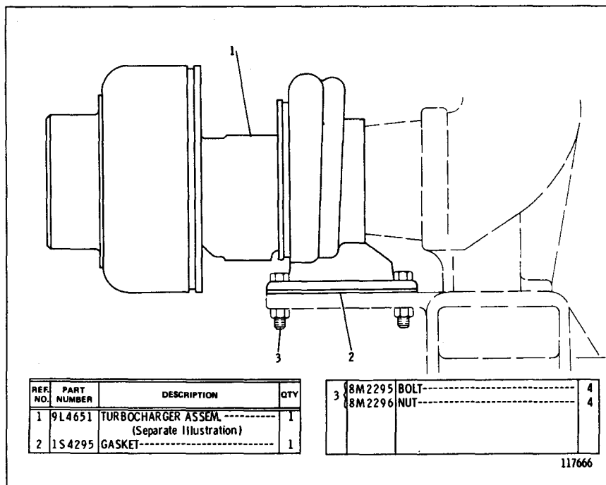
TURBOCHARGER (3N6970 N/S) 9L4651 Turbocharger parts are shown on Page 102
