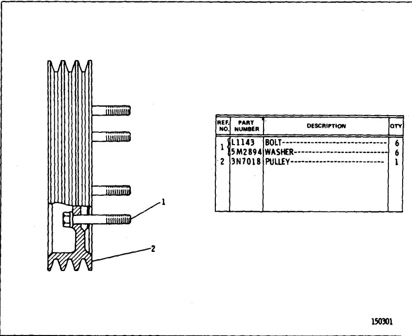
3N5629 PULLEY GROUP
