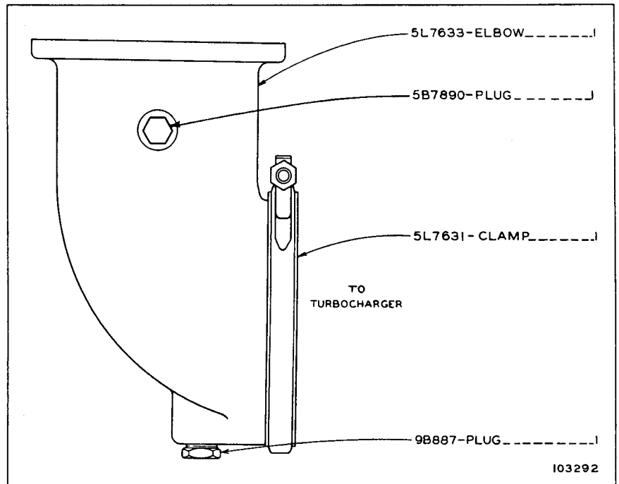
5L7660 EXHAUST ELBOW GROUP—4 Inch AN ATTACHMENT
