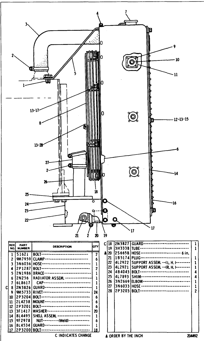
3N2790 RADIATOR GROUP—High Capacity AN ATTACHMENT
