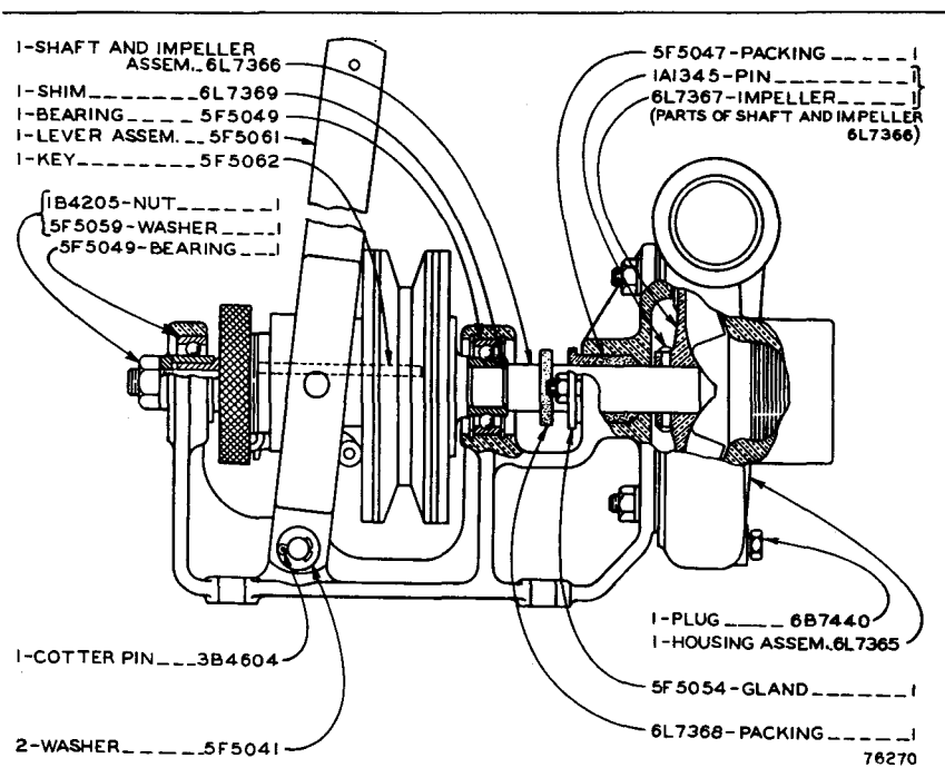
6L5875 BILGE WATER PUMP ASSEMBLY—R.H. Part of 6L5858 Bilge Water Pump Group shown on Page 61
