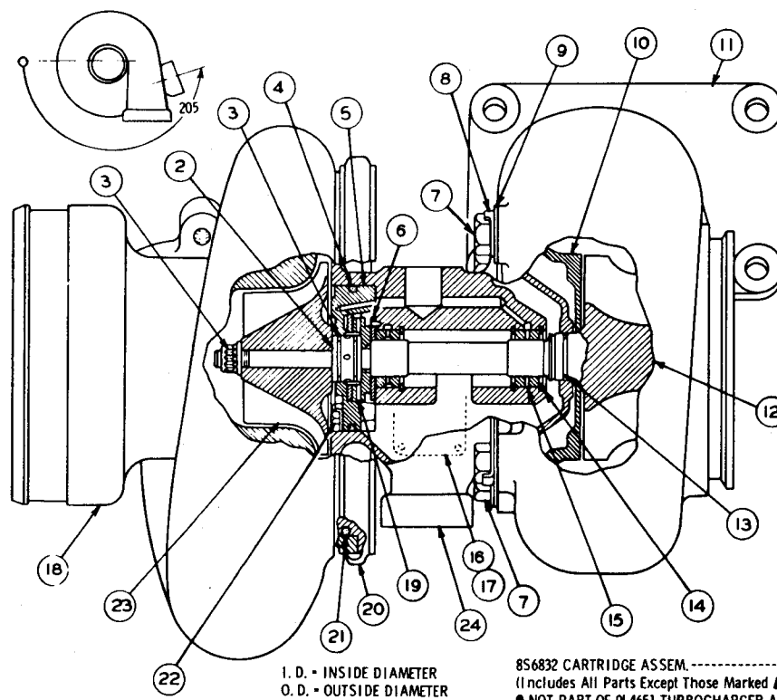
9L4651 TURBOCHARGER ASSEMBLY Part of Turbocharger shown on Page 101
