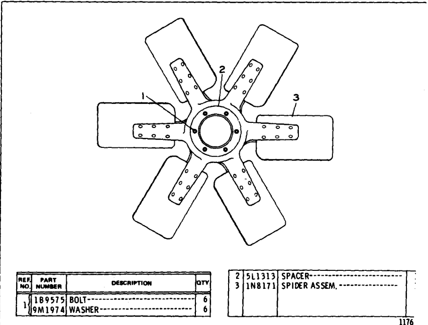
4N8752 SUCTION FAN GROUP--28 Inch Only separate parts serviced. AN ATTACHMENT
