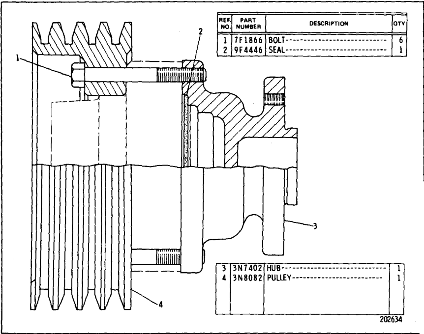
3N8083 FAN PULLEY GROUP Also available as an Attachment for use with 6N1309 Procurement Arrangemen
