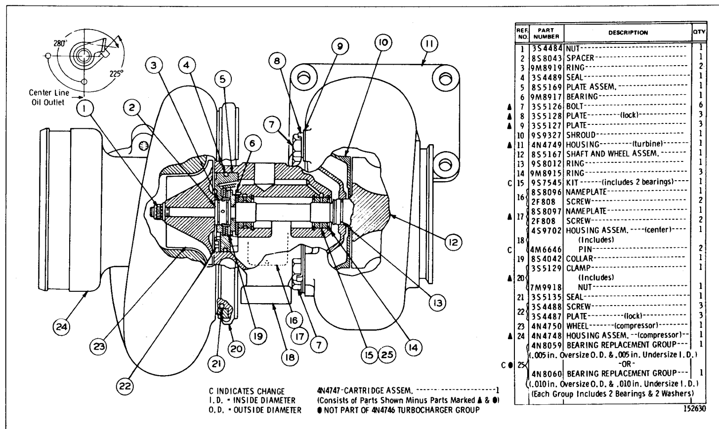
4N4746 TURBOCHARGER GROUP FOR USE WITH 50 HERTZ ELECTRIC SET
