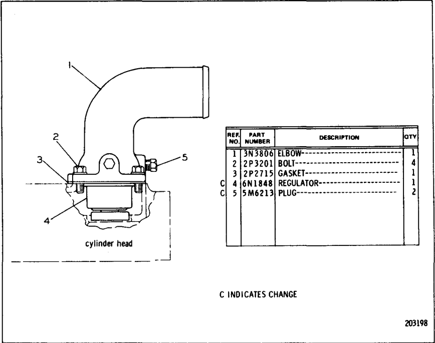
3N3279 HOUSING AND REGULATOR GROUP FOR USE WITH EXPANSION TANK. AN ATTACHMENT
