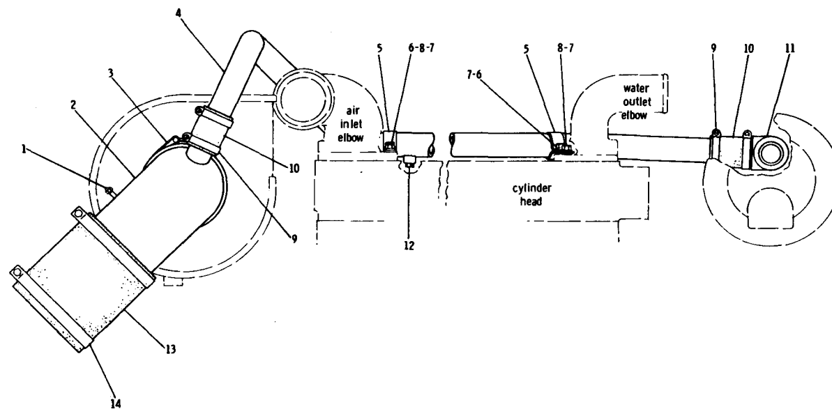
3N6073 EXHAUST ELBOW GROUP—Water Cooled AN ATTACHMENT
