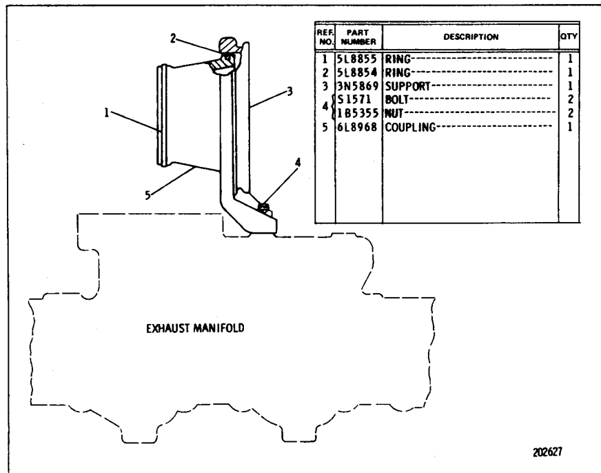
3N5870 EXHAUST ELBOW ADAPTER GROUP AN ATTACHMENT
