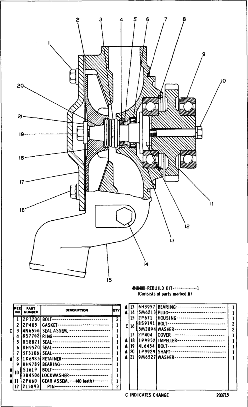
WATER PUMP (2P662 N/S) See Page 272 for Gasket Kits
