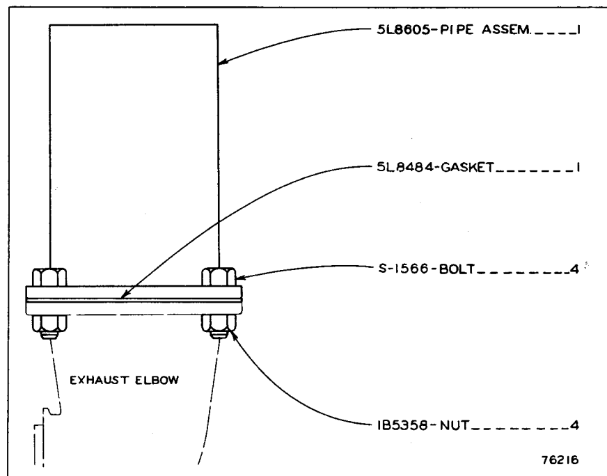
5L8632 EXHAUST PIPE GROUP—5 Inch AN ATTACHMENT
