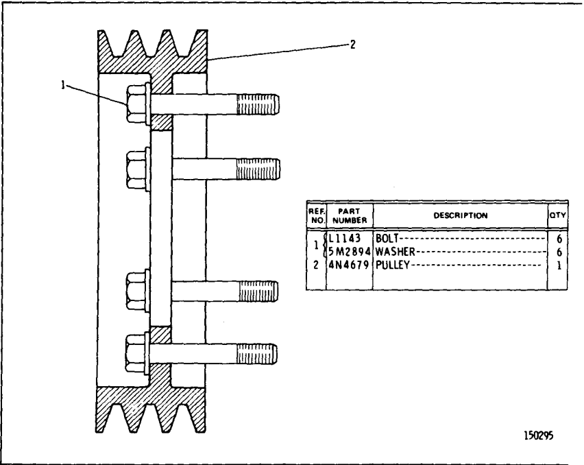
3N5626 FAN PULLEY GROUP See Page 77 for usage
