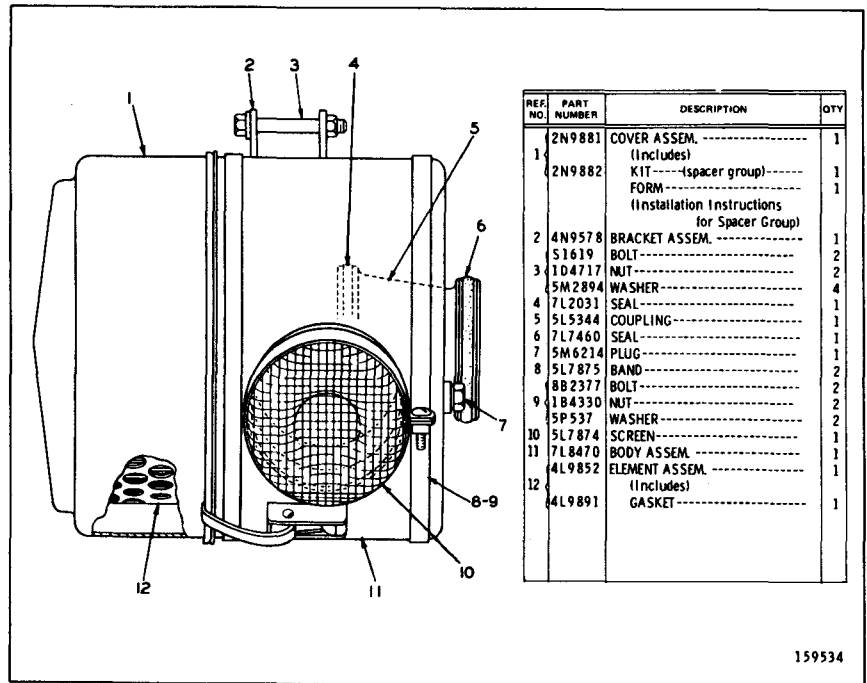
6N4041 AIR CLEANER GROUP FOR USE WITH AFTERCOOLER
