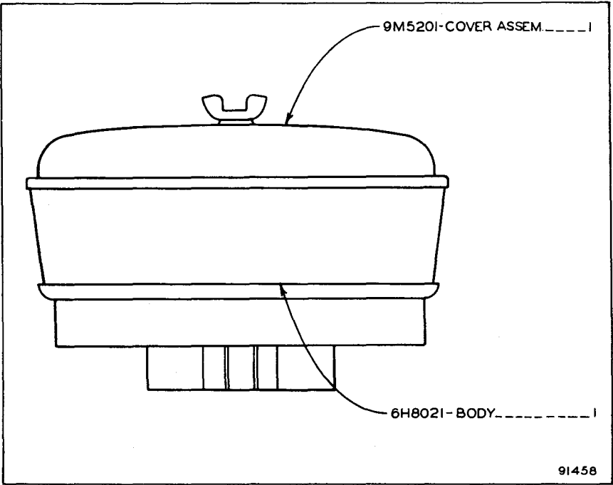
5L7942 AIR PRECLEANER GROUP AN ATTACHMENT
