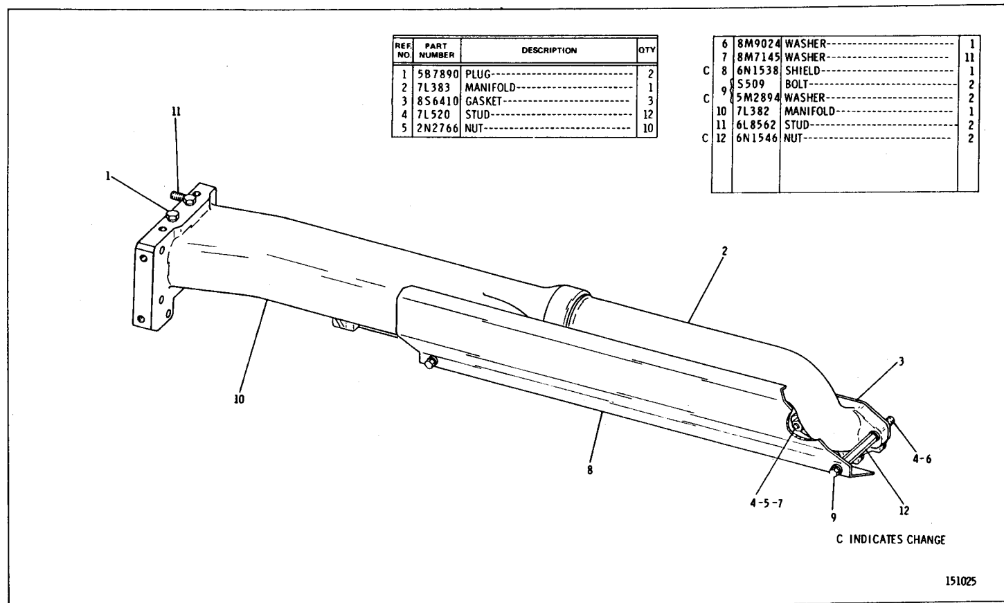
EXHAUST MANIFOLD (3N2888 N/S) Serial No. 66D12370 to 66D15040 inclusive
