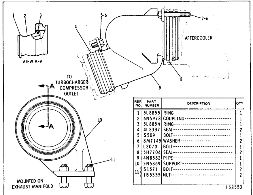
6N3322 AIR LINES GROUP Serial No. 66D16503-Up
