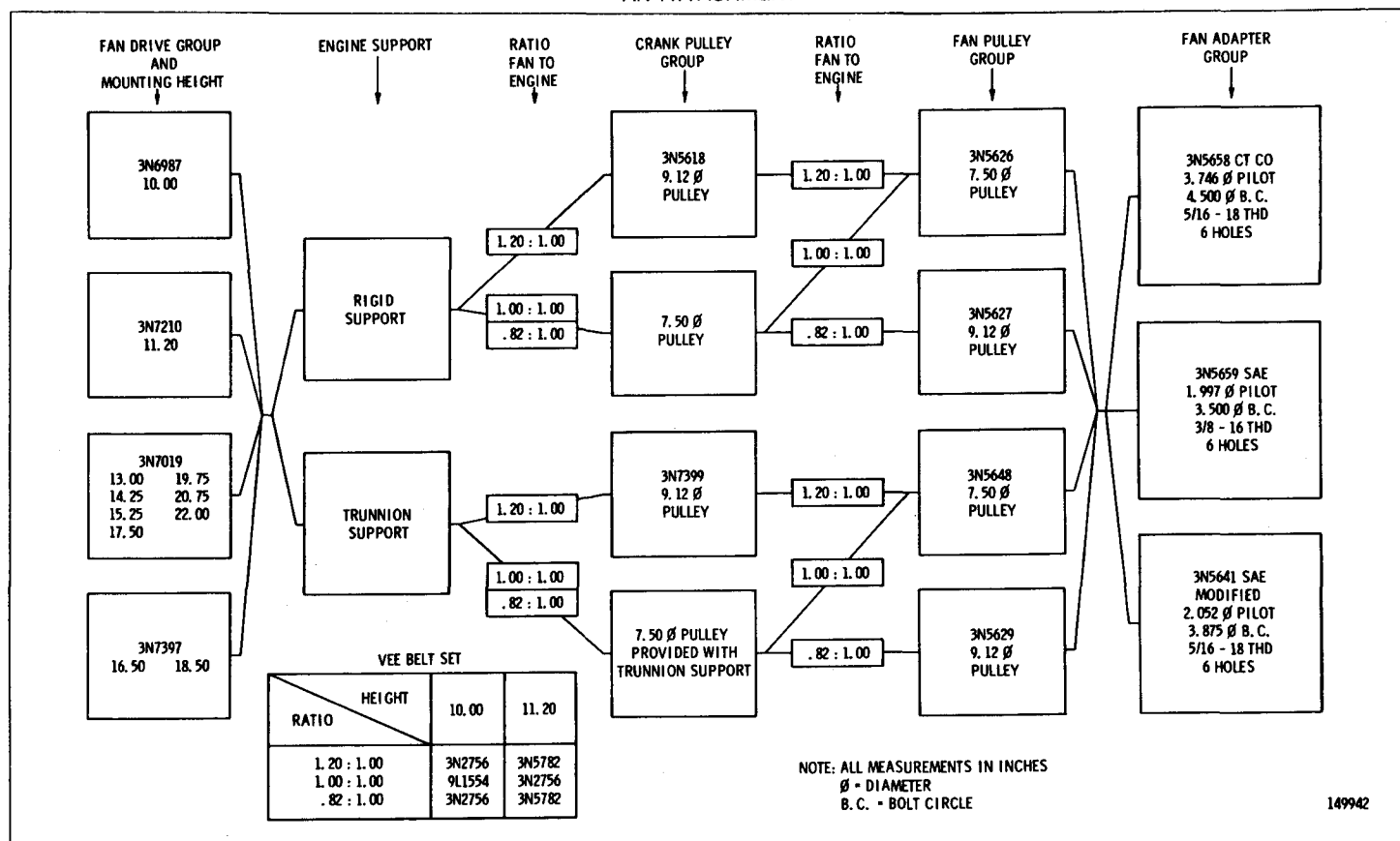
FAN DRIVE CHART AN ATTACHMENT
