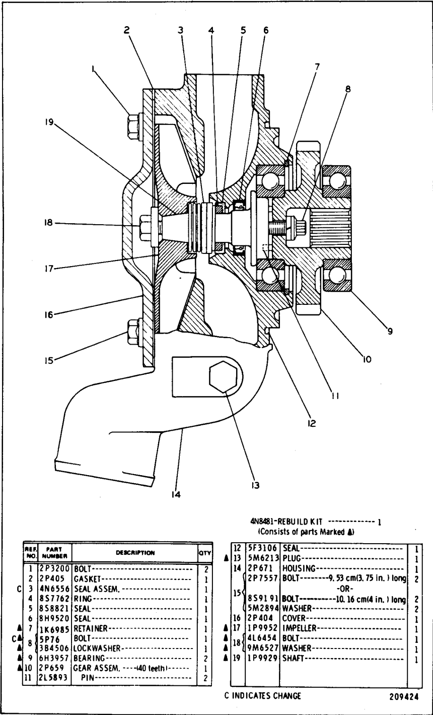
2P661 WATER PUMP GROUP—With Spline Drive and Bottom Inlet See Page 272 for Gasket Kits AN ATTACHMENT
