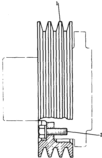
3N6934 PULLEY GROUP FOR USE WITH TRUNNION SUPPORT, AN ATTACHMENT
