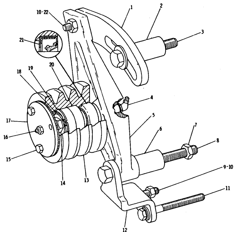
3N2755 BELT TIGHTENER GROUP FOR USE WITH FAN DRIVE AND WITHOUT ALTERNATOR AN ATTACHMENT
