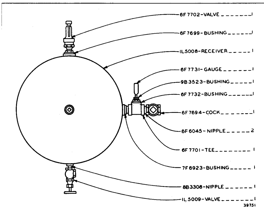
1L5010 AIR RECEIVER GROUP
