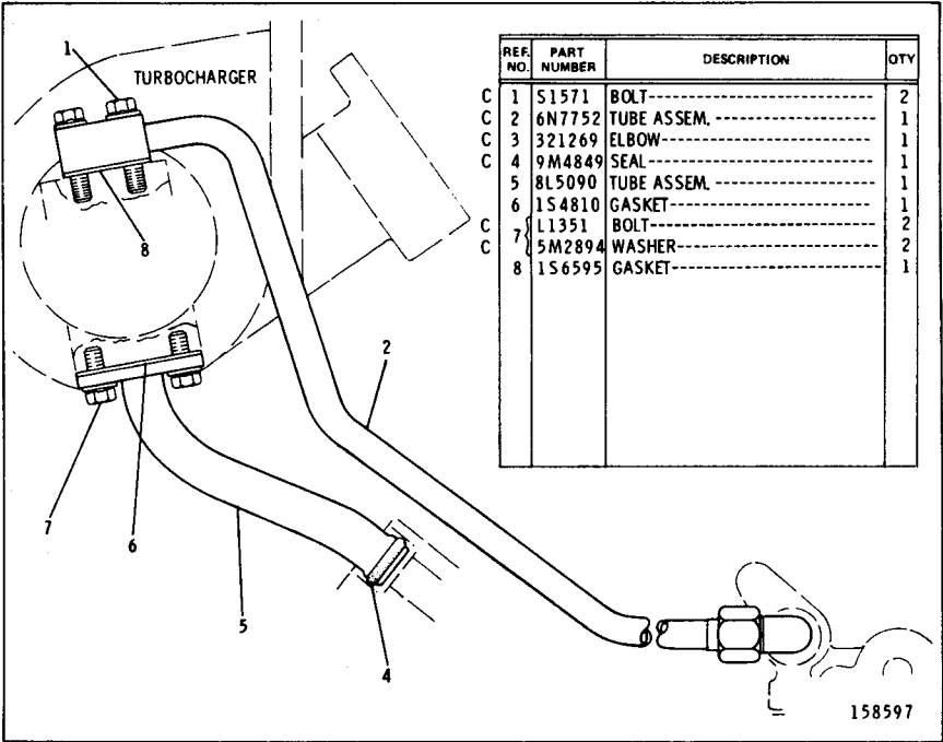
4N7122 TURBOCHARGER OIL LINES GROUP Serial No. 66D16949-Up
