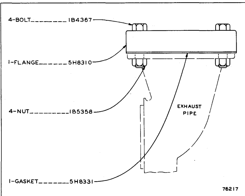
5L8601 EXHAUST FLANGE GROUP—6 Inch AN ATTACHMENT
