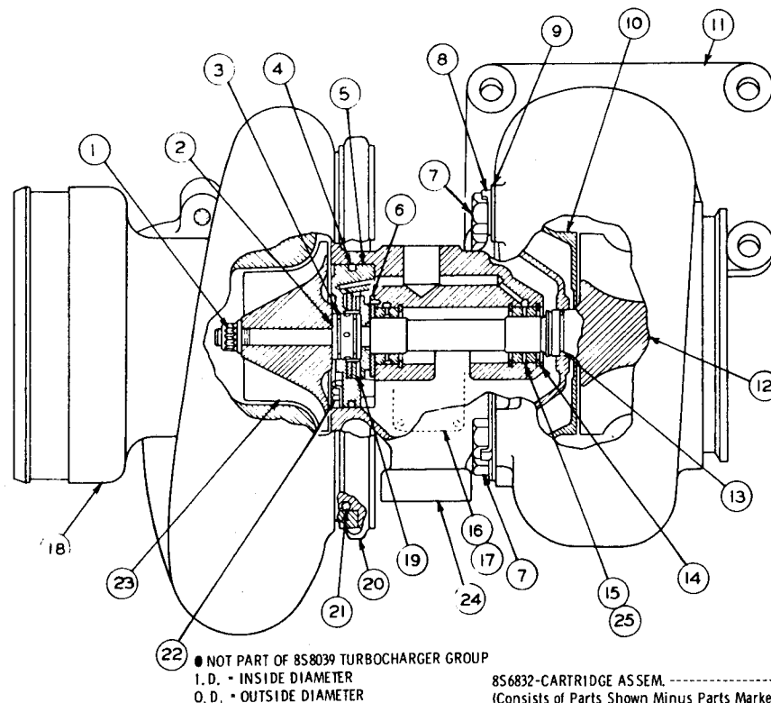
8S8039 TURBOCHARGER ASSEMBLY Part of Turbocharger shown on Page 99
