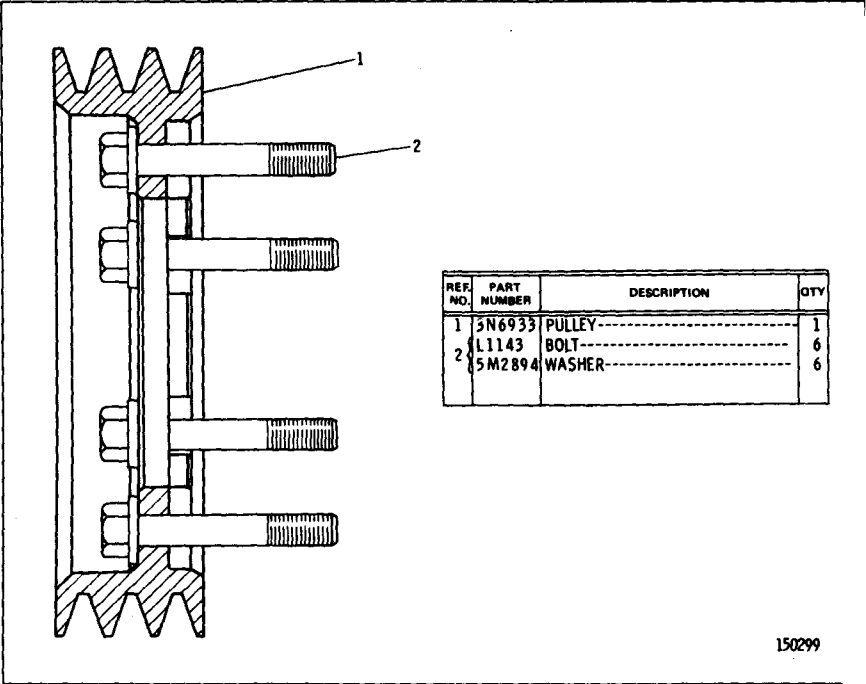
3N5648 PULLEY GROUP Refer to Chart shown on Page 77 for usage AN ATTACHMENT
