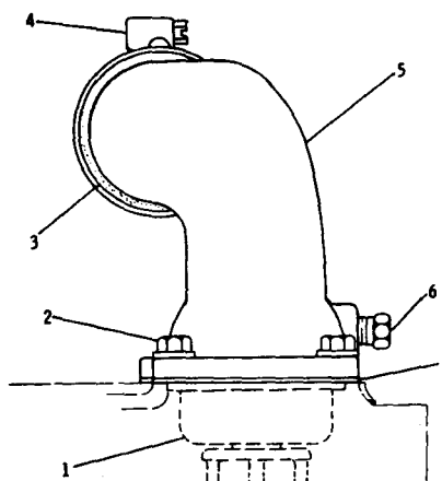
CYLINDER HEAD
