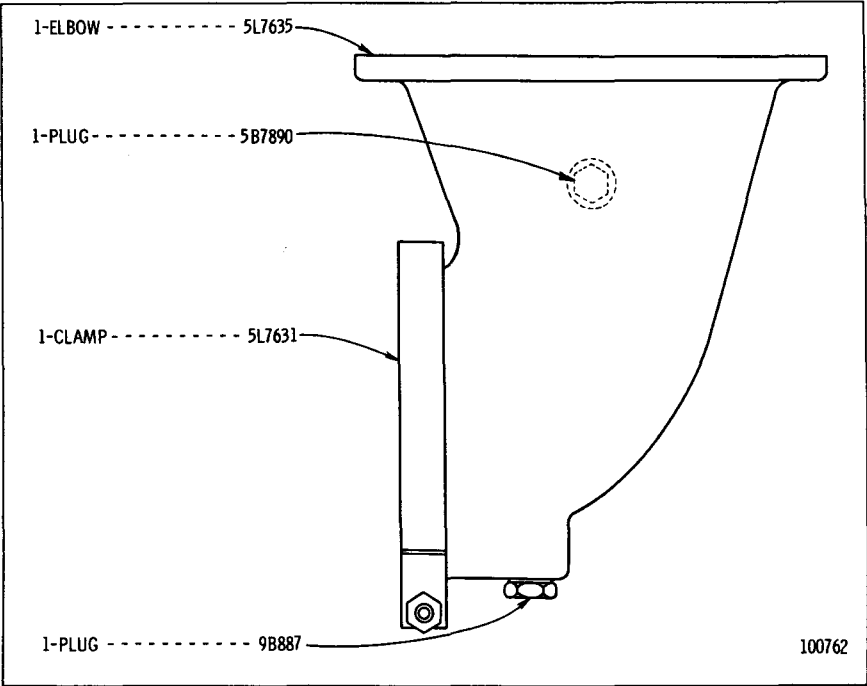
6L2927 EXHAUST ELBOW GROUP—6 Inch AN ATTACHMENT
