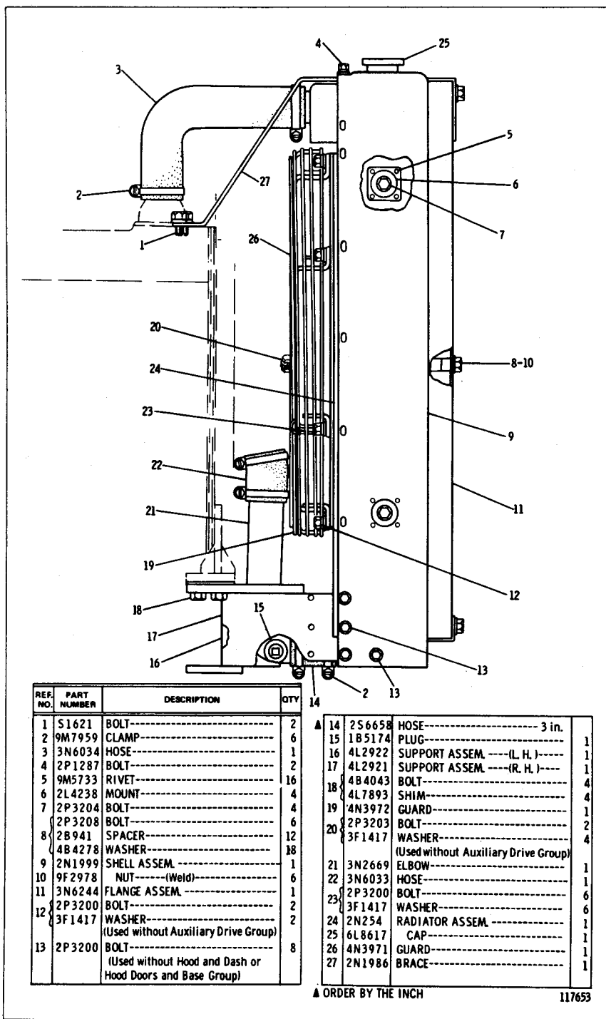
3N6693 RADIATOR GROUP—Standard Capacity FOR USE WITH DUCT FLANGE. AN ATTACHMENT
