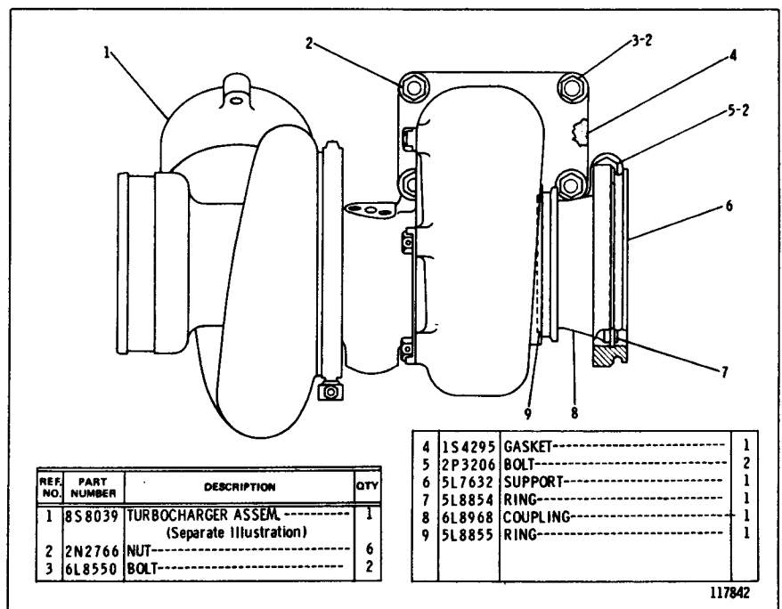
3N3018 EXHAUST FITTING GROUP—Vertical—6 Inch AN ATTACHMENT
