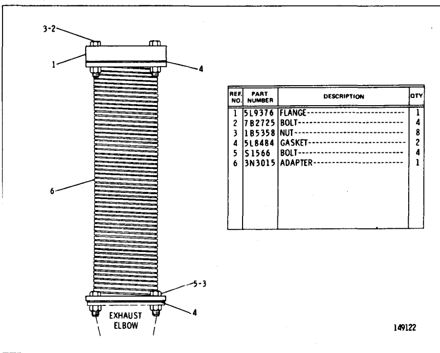
3N3016 VERTICAL EXHAUST FITTING GROUP—5 Inch
