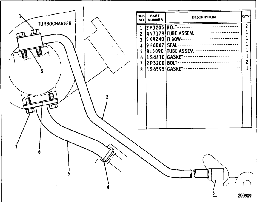
4N7122 TURBOCHARGER OIL LINES GROUP Serial No. 66D12370 to 66D16948 inclusive
