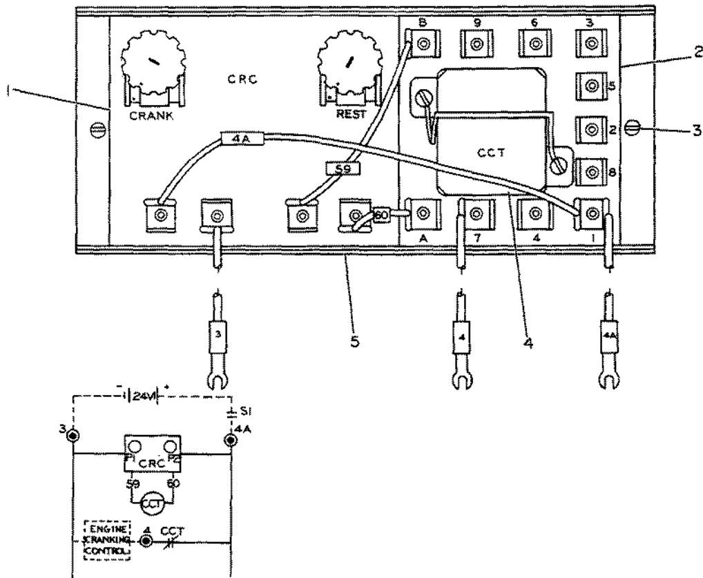
WIRING DIAGRAM
