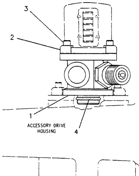
4N1402 DRIVE GP-TACHOMETER (SINGLE) An Attachment
