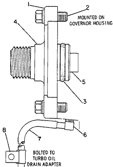
9L5867 DRIVE GP-TACHOMETER An Attachment
