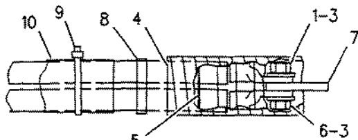
NEUTRAL CONNECTION
