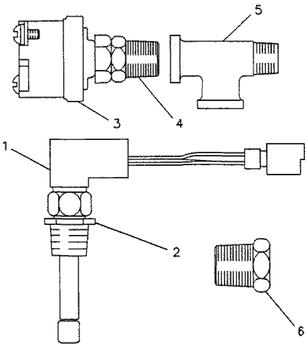
7417 5N8518 CONTACTOR GP-OIL PRESSURE & WATER TEMPERATURE An Attachment
