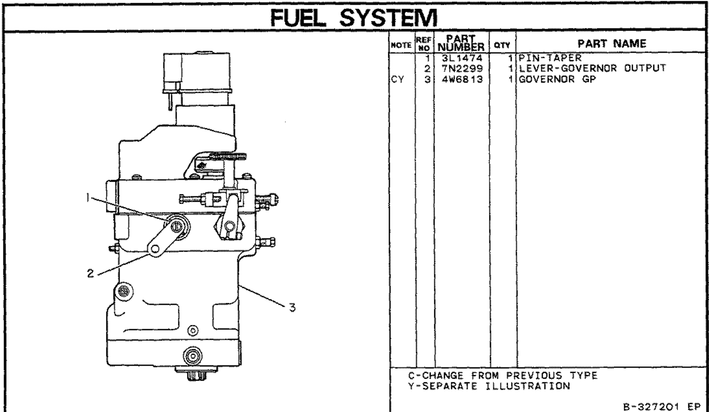
8N5874 GOVERNOR GP-WOODWARD 4W6813-Page 128 Type 1 An Attachment
