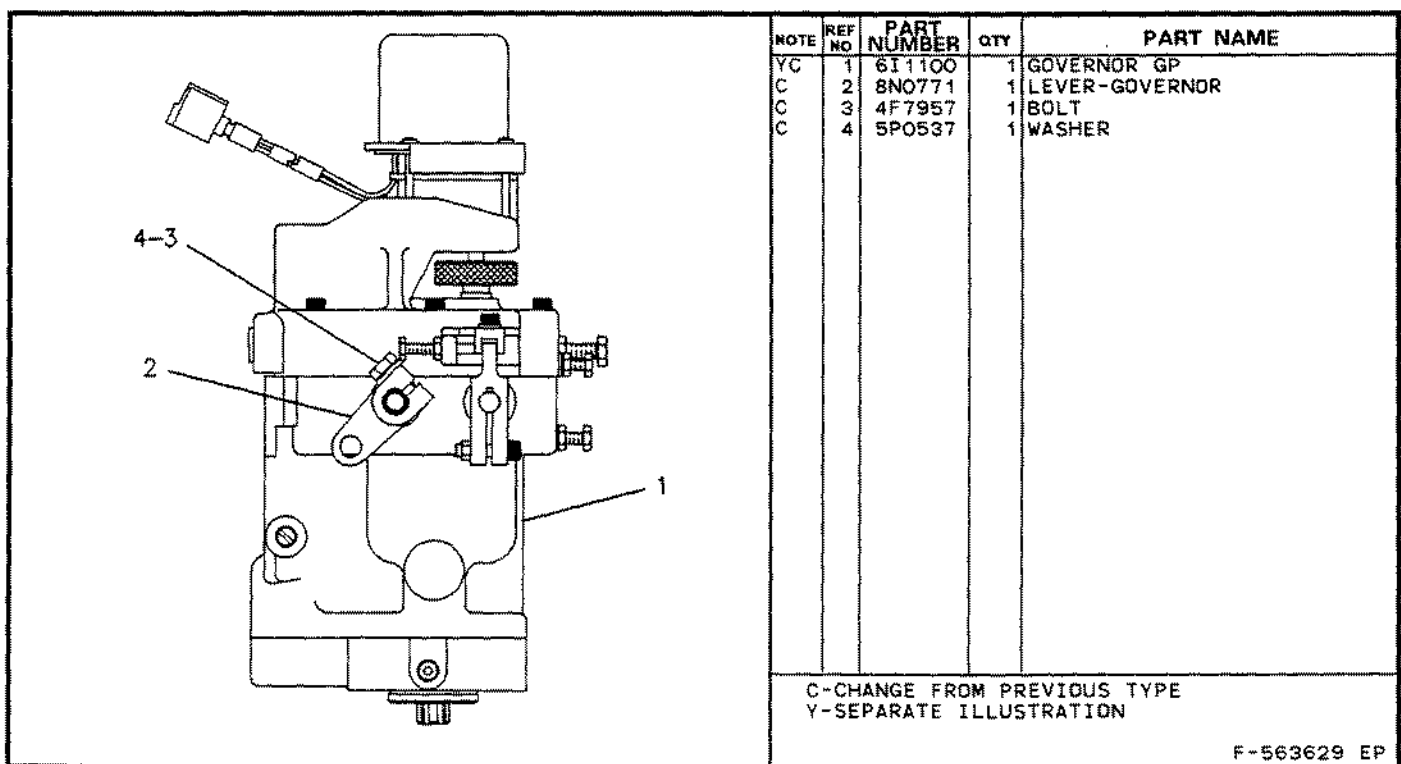
8N5874 GOVERNOR GP-WOODWARD 6I1100-Page 129.01 Type 2 An Attachment
