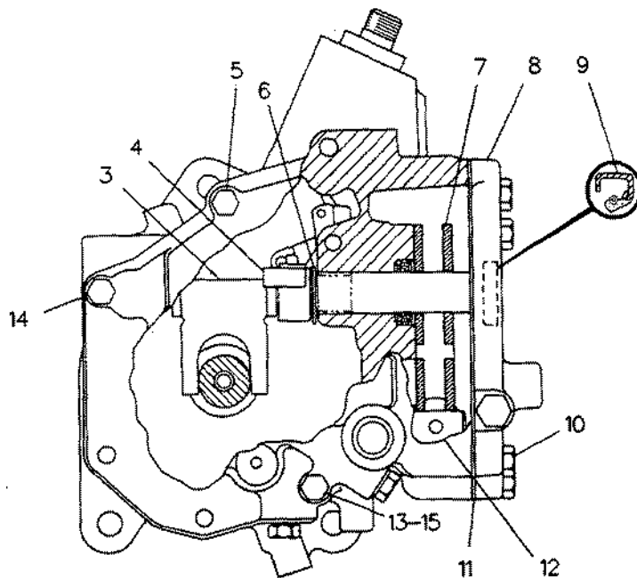
VIEW C-C
