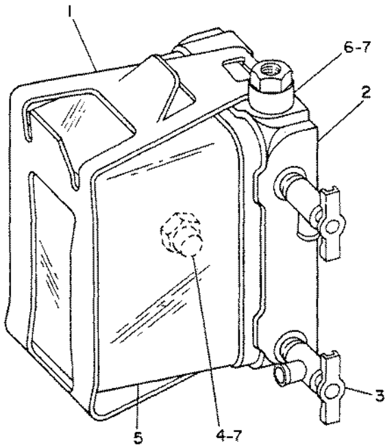
9N6519 SEPARATOR GP-WATER An Attachment
