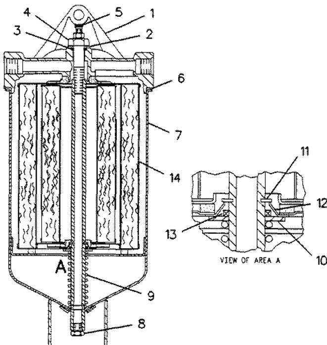
2W4234 SEPARATOR GP-WATER An Attachment
