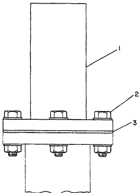
2W5223 PIPE GP-EXHAUST - 3 INCH An Attachment
