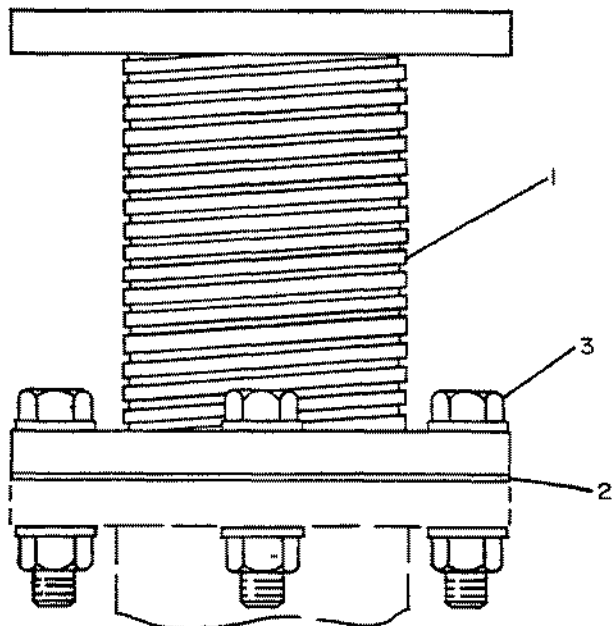
2W5219 FITTING GP-EXHAUST - FLEXIBLE (3 IN) An Attachment
