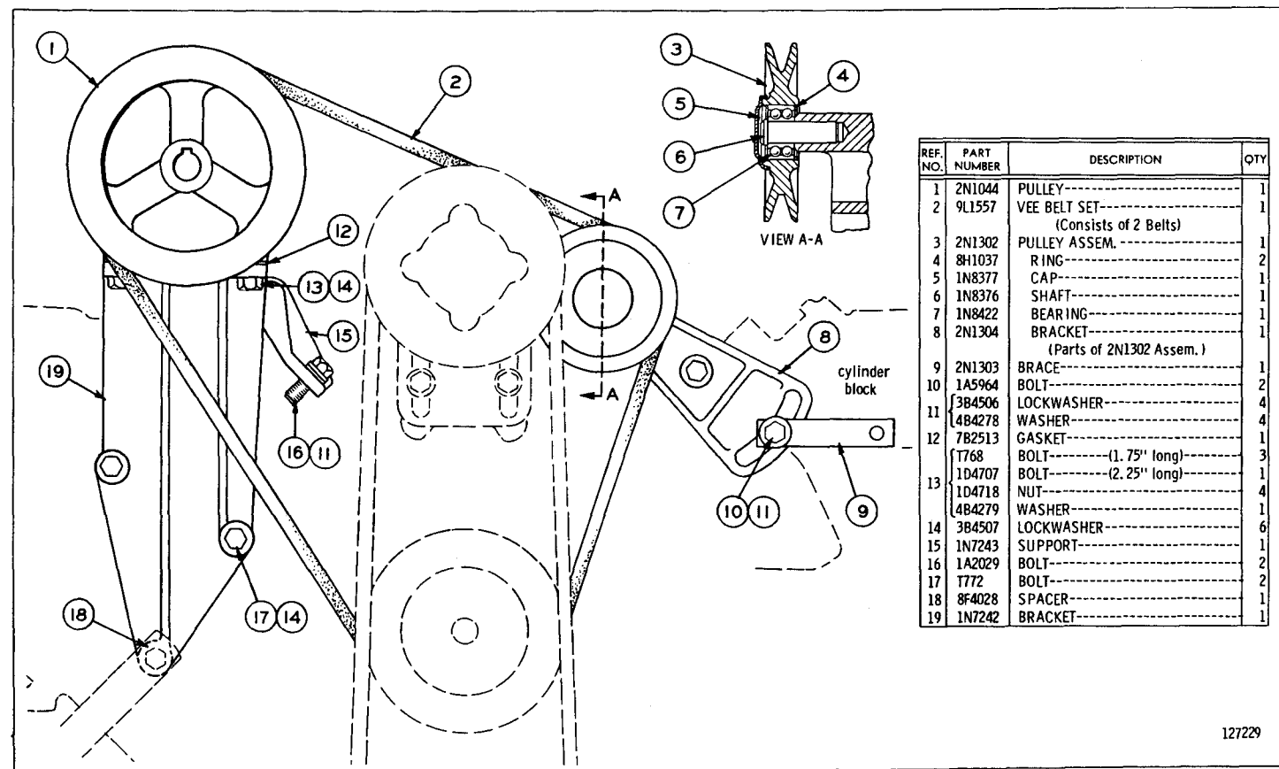
2N1371 AIR COMPRESSOR MOUNTING AND DRIVE GROUP—Type 1 FOR USE WITH HIGH-MOUNT FAN
