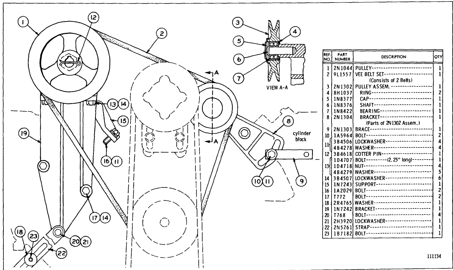
2N1371 AIR COMPRESSOR MOUNTING AND DRIVE GROUP—Type 2 FOR USE WITH HIGH-MOUNT FAN
