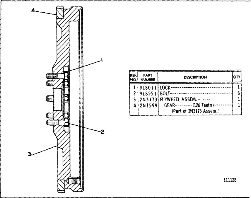
2N8367 FLYWHEEL GROUP FOR USE WITH S.A.E. NO. 3 FLYWHEEL HOUSING Only separate parts serviced
