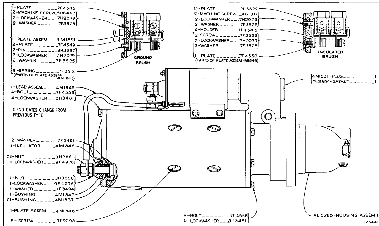
9L3597 STARTING MOTOR ASSEMBLY-12 Volt-Part 1-Type 2 Part of 2N3195 Electric Starting Group shown on Page 109
