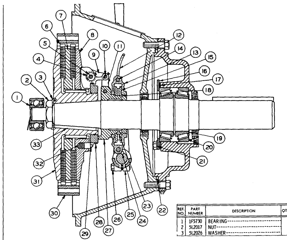
2N1373 CLUTCH ASSEMBLY--Side View Specification No. 33219 Part of 2N1374 Clutch Group shown on Page 90
