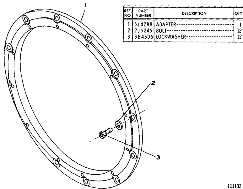
2N4968 ADAPTER GROUP Provides a .562" thick S.A.E. No. 2 to S.A.E. No. 3 Flywheel Housing Adapter to bolt to aluminum flywheel housing
