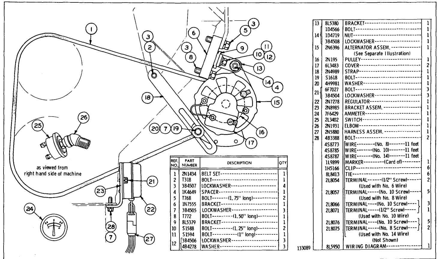
1N9289 ALTERNATOR GROUP--12 Volt, 35 Ampere--Type 4 2N6396 Alternator parts are shown on Pages 124 and 125
