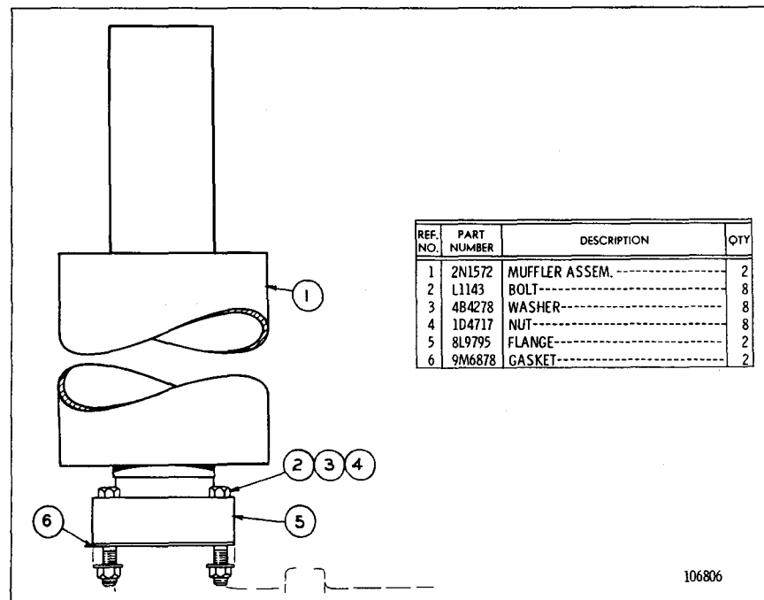
2N1646 MUFFLER GROUP
