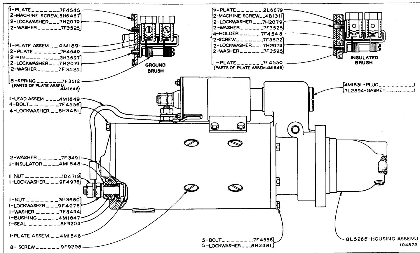
9L3597 STARTING MOTOR ASSEMBLY-12 Volt-Part 1-Type 1 Part of 2N3195 Electric Starting Group shown on Page 109
