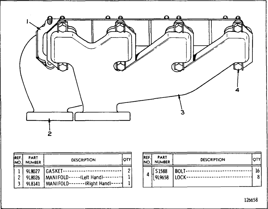
2N2467 MANIFOLD GROUP
