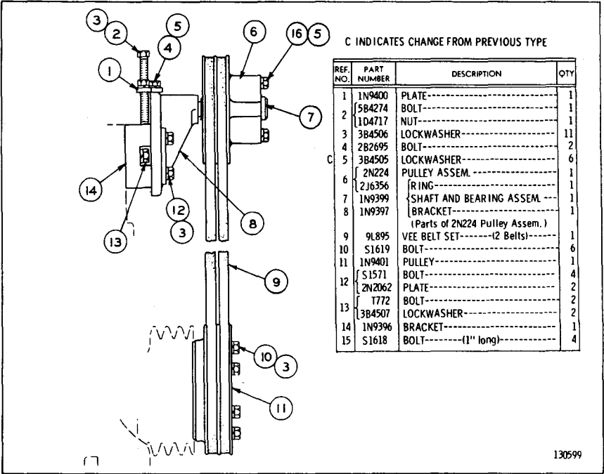
2N223 FAN MOUNTING AND DRIVE GROUP-Type 3
