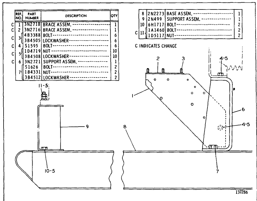
2N2101 BASE GROUP--Factory Installation FOR USE WITH DIESEL ELECTRIC SETS
