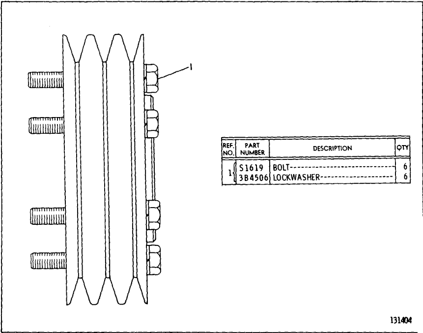
9L7461 CRANKSHAFT PULLEY GROUP
