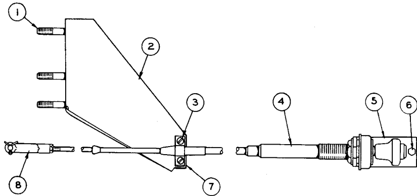
2N2111 GOVERNOR CONTROL GROUP FOR USE WITH DIESEL ELECTRIC SETS Only separate parts serviced
