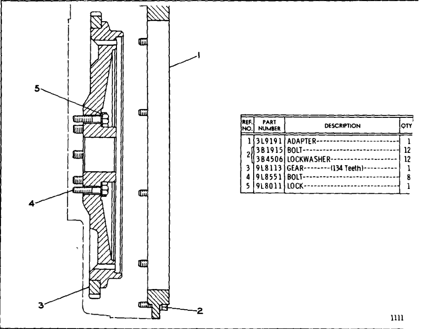
2N7184 TRANSMISSION MOUNTING GROUP FOR USE WITH S.A.E. NO. 2 FLYWHEEL HOUSING
