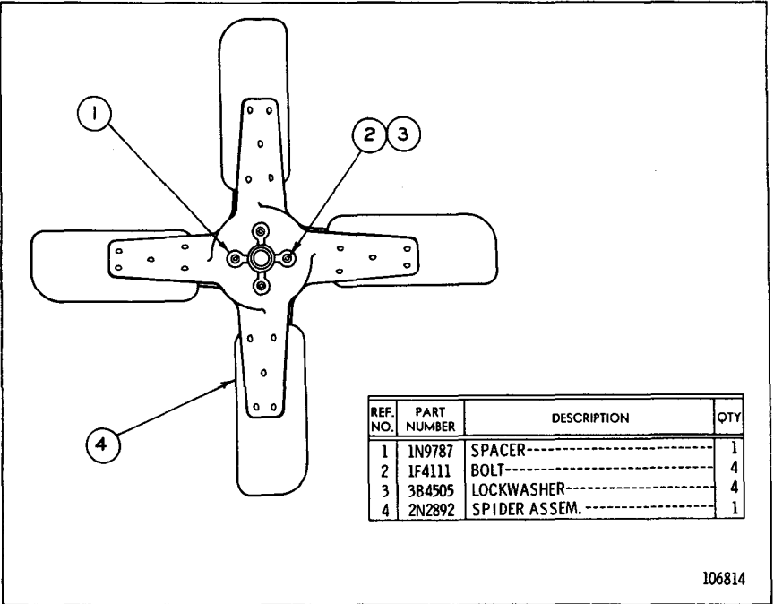
2N2895 BLOWER FAN GROUP—22" Diameter—1.58" Projected Width
