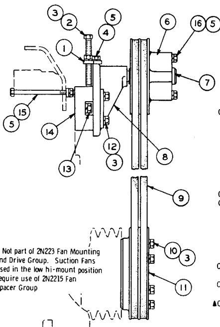
2N223 FAN MOUNTING AND DRIVE GROUP-Type 2
