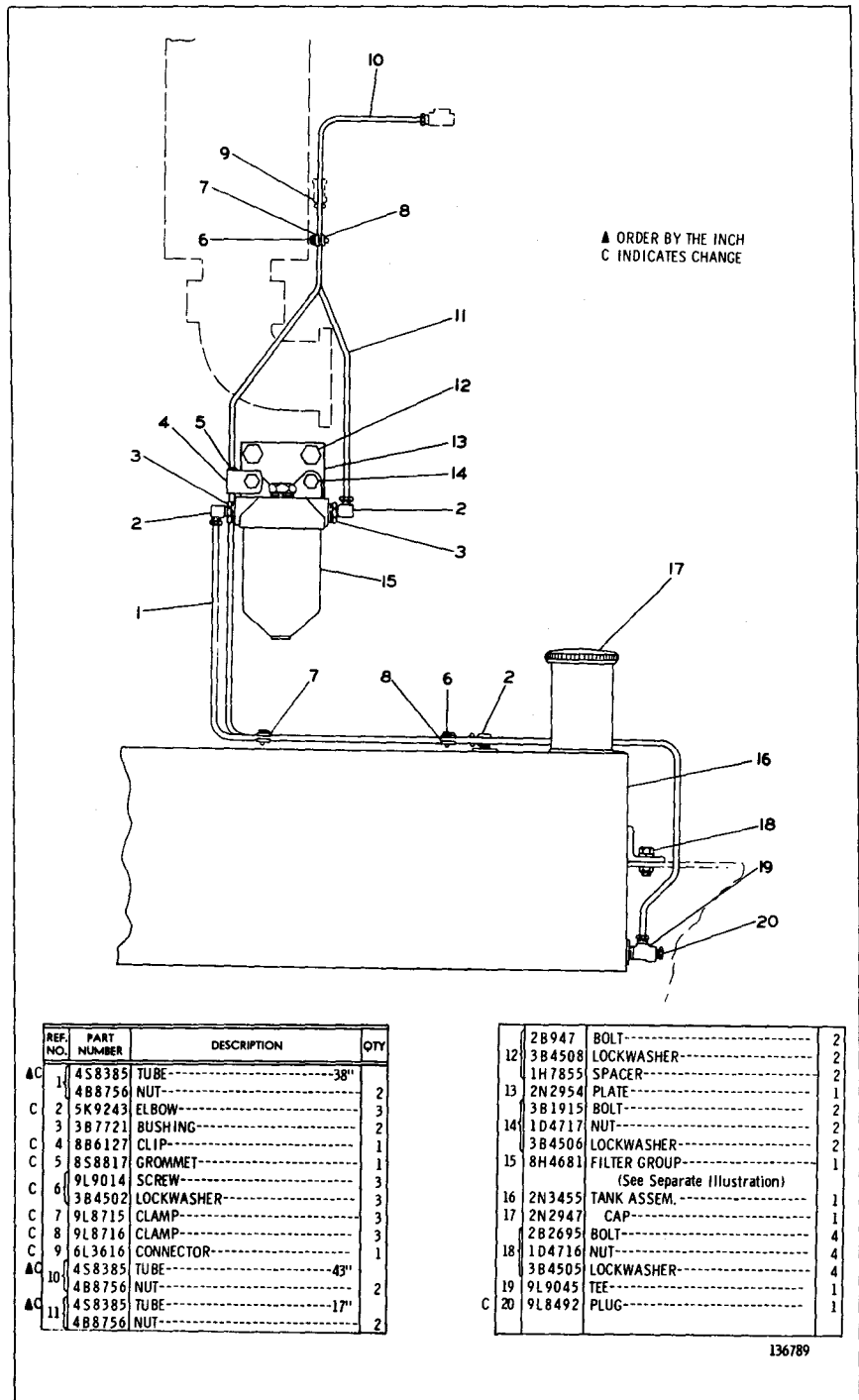
2N3435 FUEL TANK GROUP--50 U.S. Gallon FOR USE WITH 2N2101 BASE GROUP AND DIESEL ELECTRIC SETS 8H4681 Filter parts are shown on Page 52
