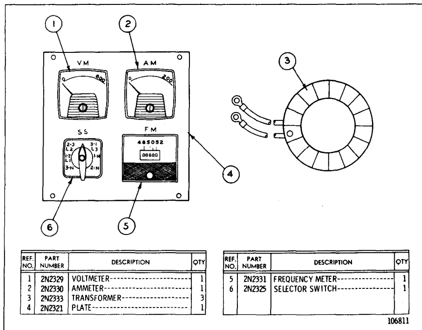
2N2338 METER GROUP—220/380—400 Volt, 50 hertz FOR USE WITH 2N2218 GENERATOR GROUP
