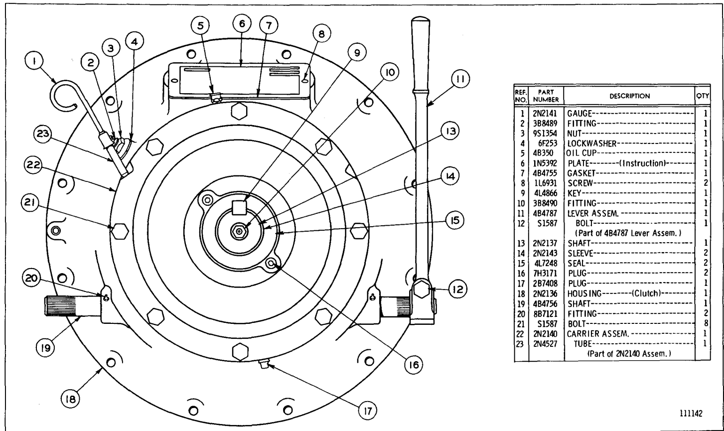
2N1373 CLUTCH ASSEMBLY—End View Specification No. 33219 Part of 2N1374 Clutch Group shown on Page 90
