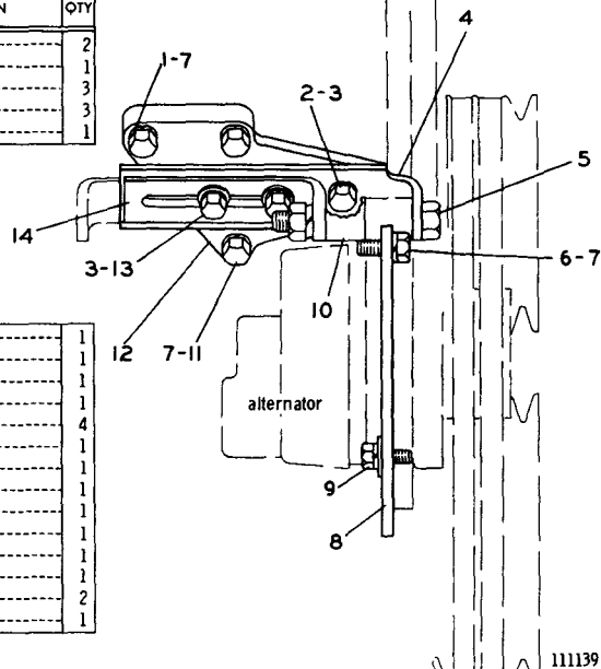
2N1904 ALTERNATOR MOUNTING GROUP—Type 2
