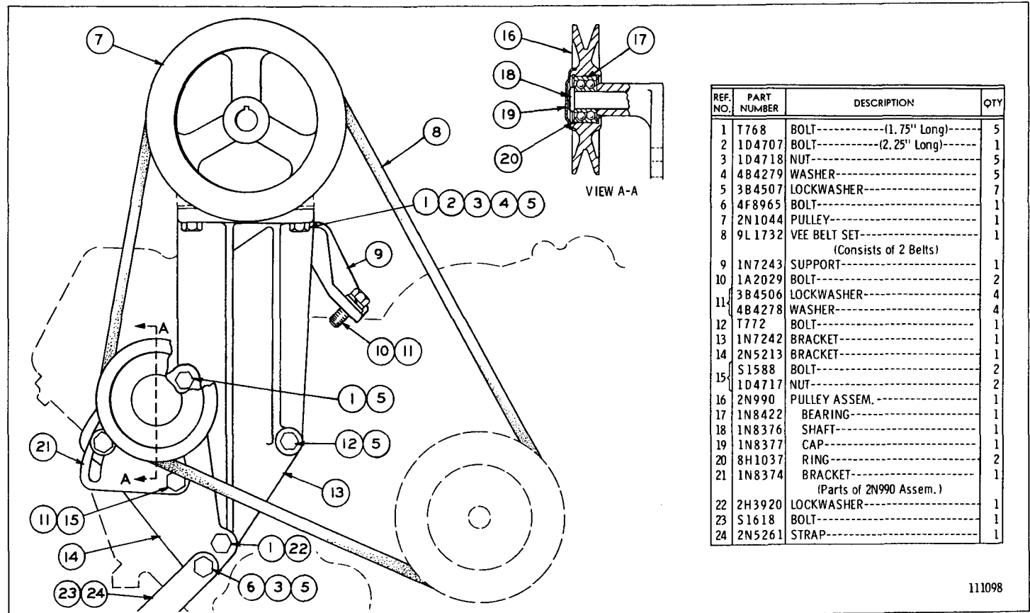
2N1370 AIR COMPRESSOR MOUNTING AND DRIVE GROUP—Type 2
