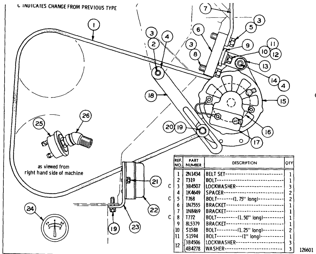
1N9289 ALTERNATOR GROUP--12 Volt, 35 Ampere--Type 2 8L5410 Alternator parts are shown on Page 123
