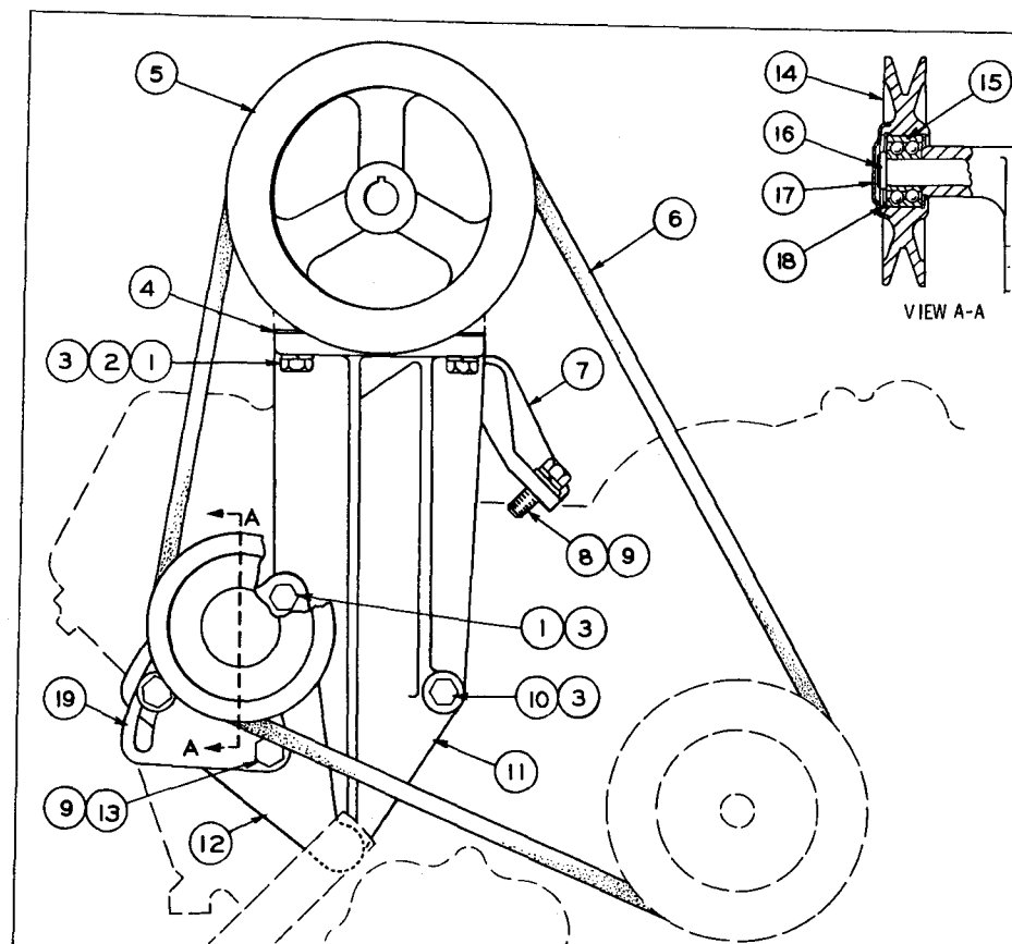
2N1370 AIR COMPRESSOR MOUNTING AND DRIVE GROUP--Type 1
