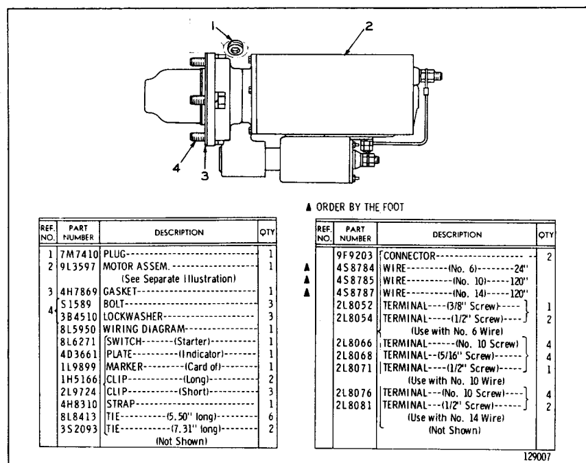
2N3195 ELECTRIC STARTING GROUP--12 Volt FOR USE WITH S.A.E. NO. 3 FLYWHEEL HOUSING 9L3597 Motor parts are shown on Pages 114 through 117
