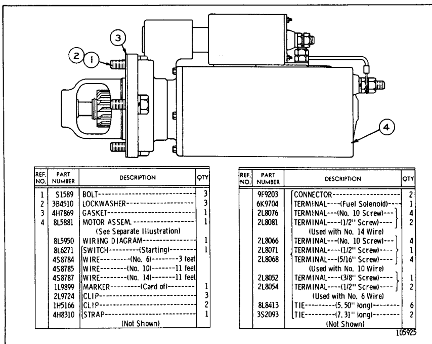
8L5949 ELECTRIC STARTING GROUP--12 Volt 8L5881 Motor parts are shown on Pages 110 through 113
