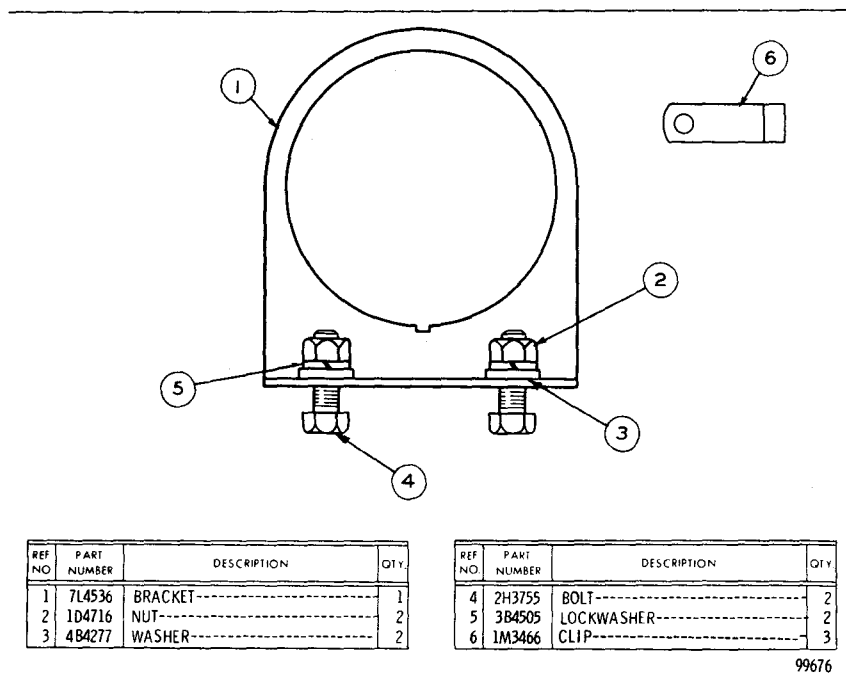
7L4535 TACHOMETER MOUNTING GROUP Part of 2N5745 Tachometer Drive and Mounting Group
