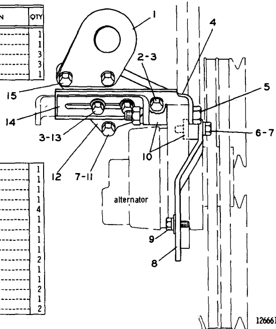
2N1904 ALTERNATOR MOUNTING GROUP—Type 1
