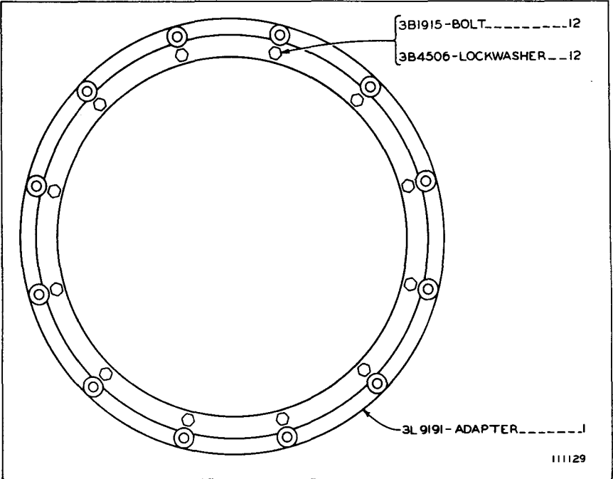
2N4969 ADAPTER GROUP Provides a 1" thick S.A.E. No. 2 to S.A.E. No. 3 Flywheel Housing Adapter to bolt to aluminum flywheel housing
