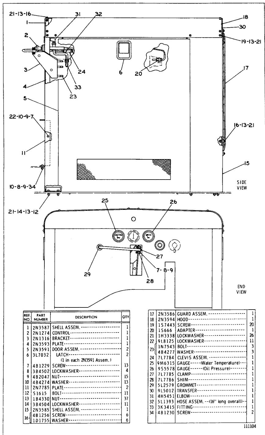
2N3595 ENGINE ENCLOSURE GROUP-Type 2
