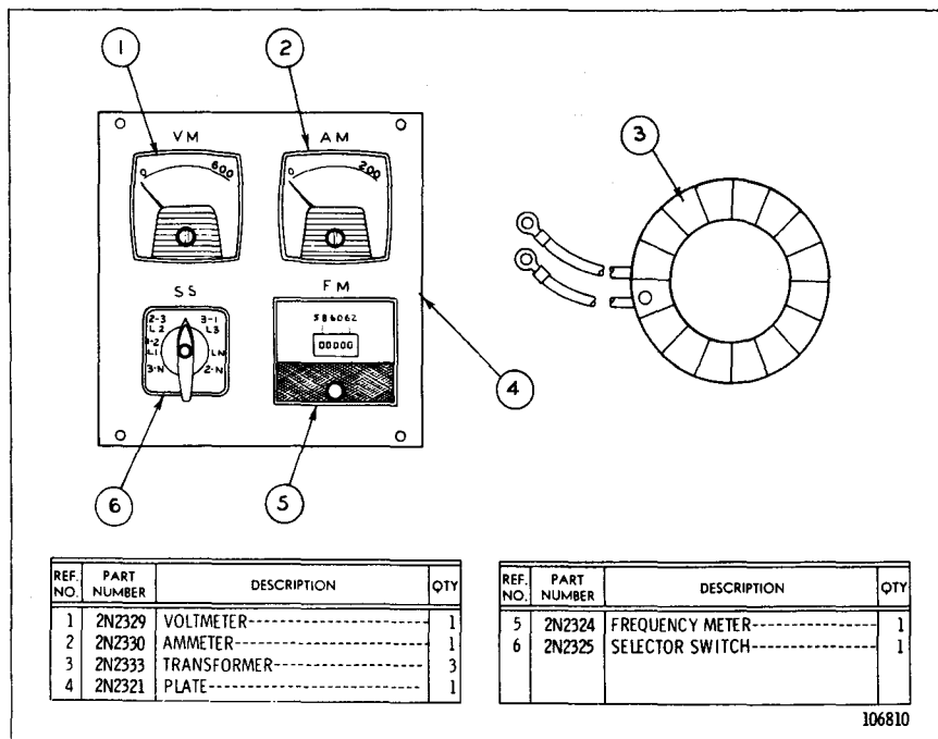
2N2337 METER GROUP—240/416—480 Volt, 60 hertz FOR USE WITH 2N2218 GENERATOR GROUP
