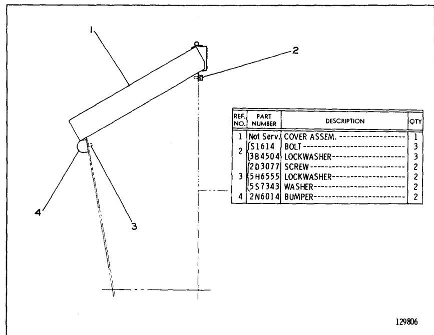
2N5292 INSTRUMENT PANEL COVER GROUP Part of 2N3592 Engine Enclosure Group shown on Page 98
