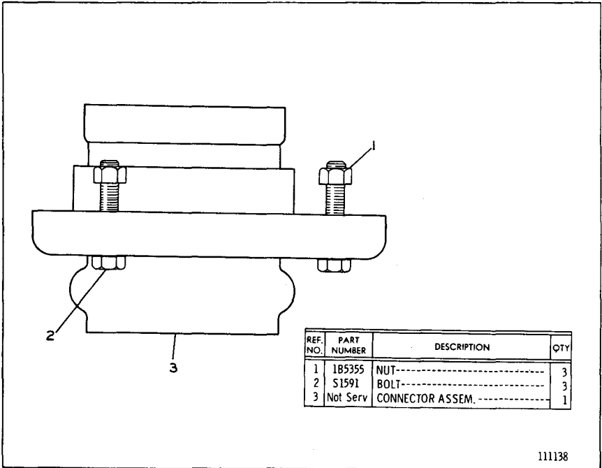
9L7147 EXHAUST CONNECTOR GROUP--2 Required FOR USE WITH 2N2467 MANIFOLD GROUP
