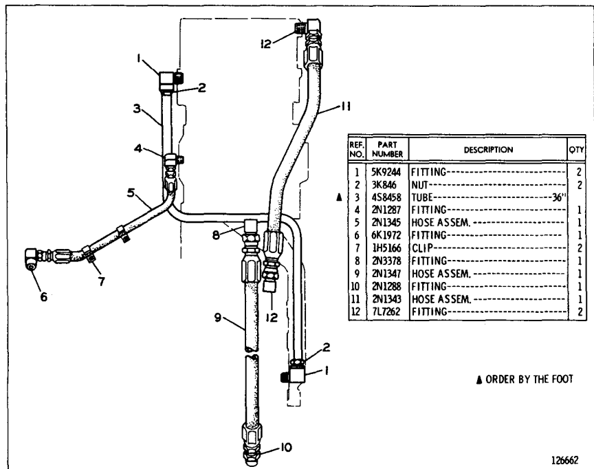
2N996 AIR COMPRESSOR CONNECTIONS GROUP
