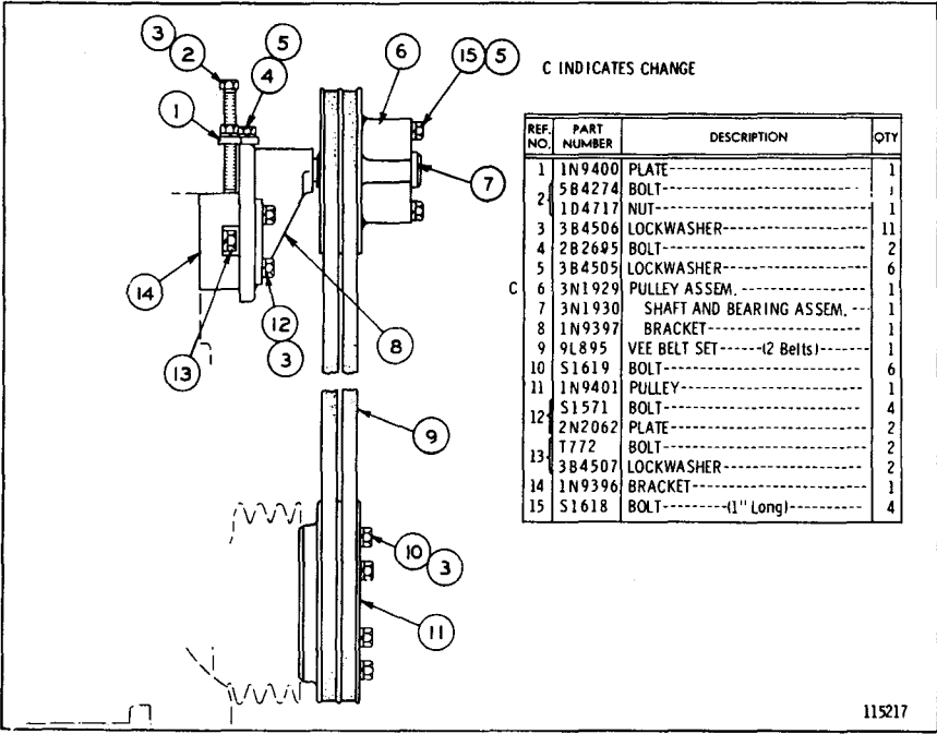
2N223 FAN MOUNTING AND DRIVE GROUP-Type 4
