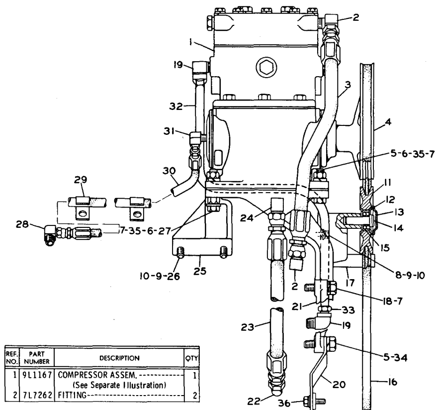
2N6446 AIR COMPRESSOR GROUP--Type 1 9L1167 Air Compressor parts are shown on Page 82
