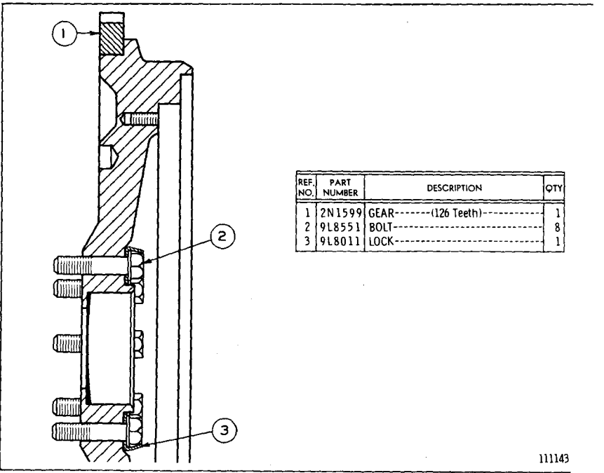
2N3489 FLYWHEEL GROUP FOR USE WITH S.A.E. NO. 3 FLYWHEEL HOUSING
