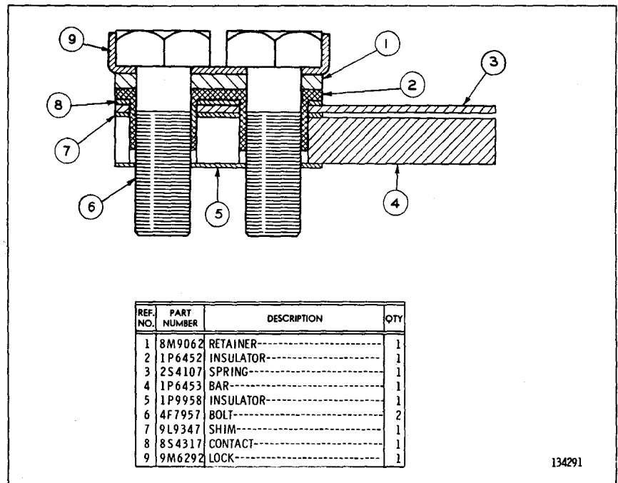
9L9345 GOVERNOR TORQUE SPRING GROUP-Type 2
