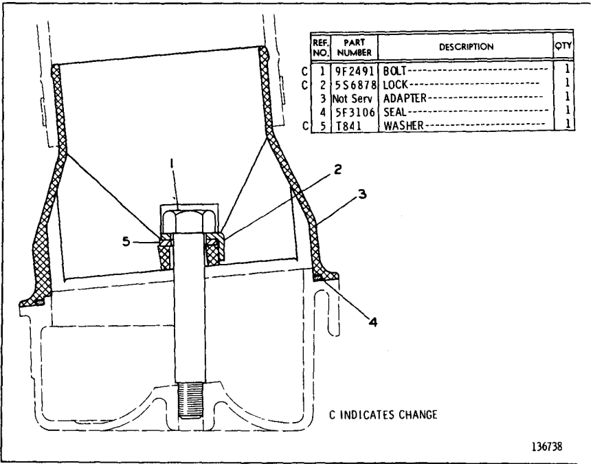
2N5841 AIR INLET HOSE CONNECTIONS GROUP
