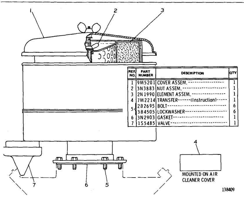
3N3212 AIR CLEANER GROUP Effective with Serial No. 96M1963
