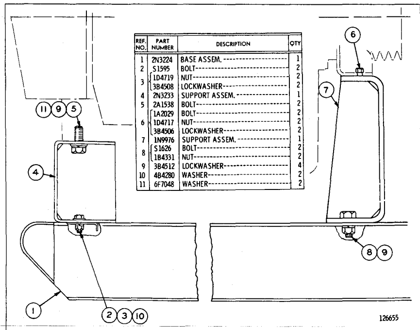
2N3842 BASE GROUP-Type 1
