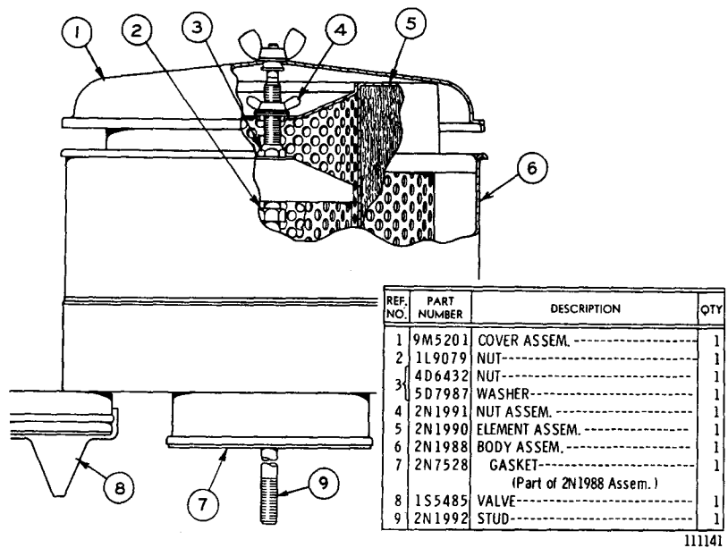
1N9970 AIR CLEANER ASSEMBLY Serial No. 96M1 to 96M1962 inclusive Part of 2N905 Air Cleaner Group shown on Page 67
