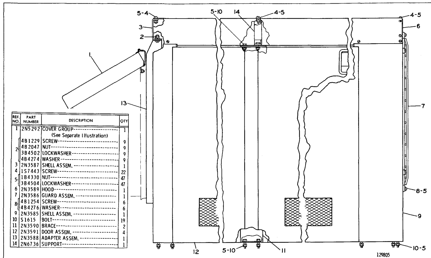
2N3592 ENGINE ENCLOSURE GROUP FOR USE WITH 2N1646 MUFFLER GROUP AND 2N2101 BASE GROUPS SHOWN ON PAGES 74 and 97 2N5292 Cover parts are shown on Page 97
