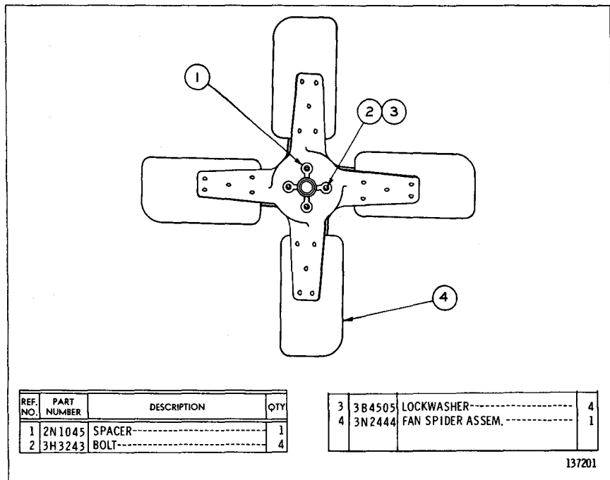
3N2445 SUCTION FAN GROUP--22" Diameter
