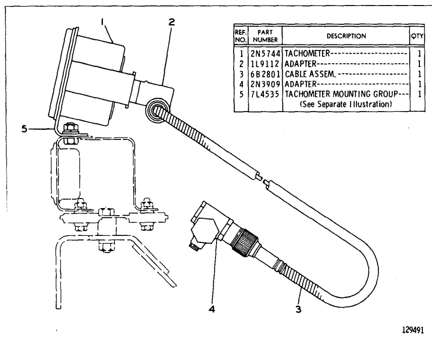
2N5745 TACHOMETER DRIVE AND MOUNTING GROUP
