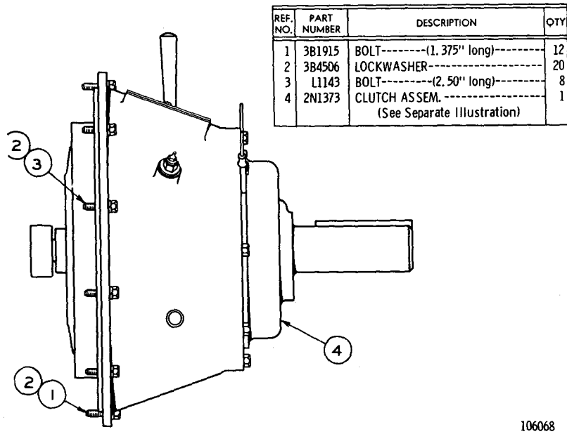
2N1374 CLUTCH GROUP FOR USE WITH S.A.E. NO. 2 FLYWHEEL HOUSING 2N1373 Clutch parts are shown on Pages 88 and 89
