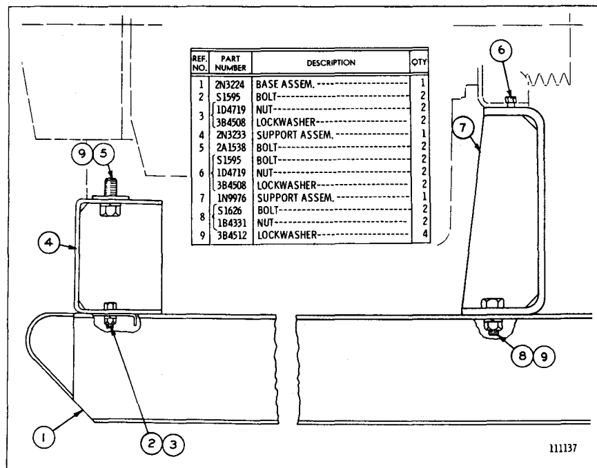
2N3842 BASE GROUP-Type 2
