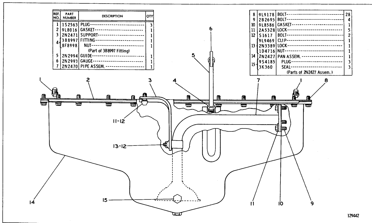
2N3388 OIL PAN GROUP—Deep Sump FOR MOUNTING A 30° TILT CENTER SUMP OIL PUMP
