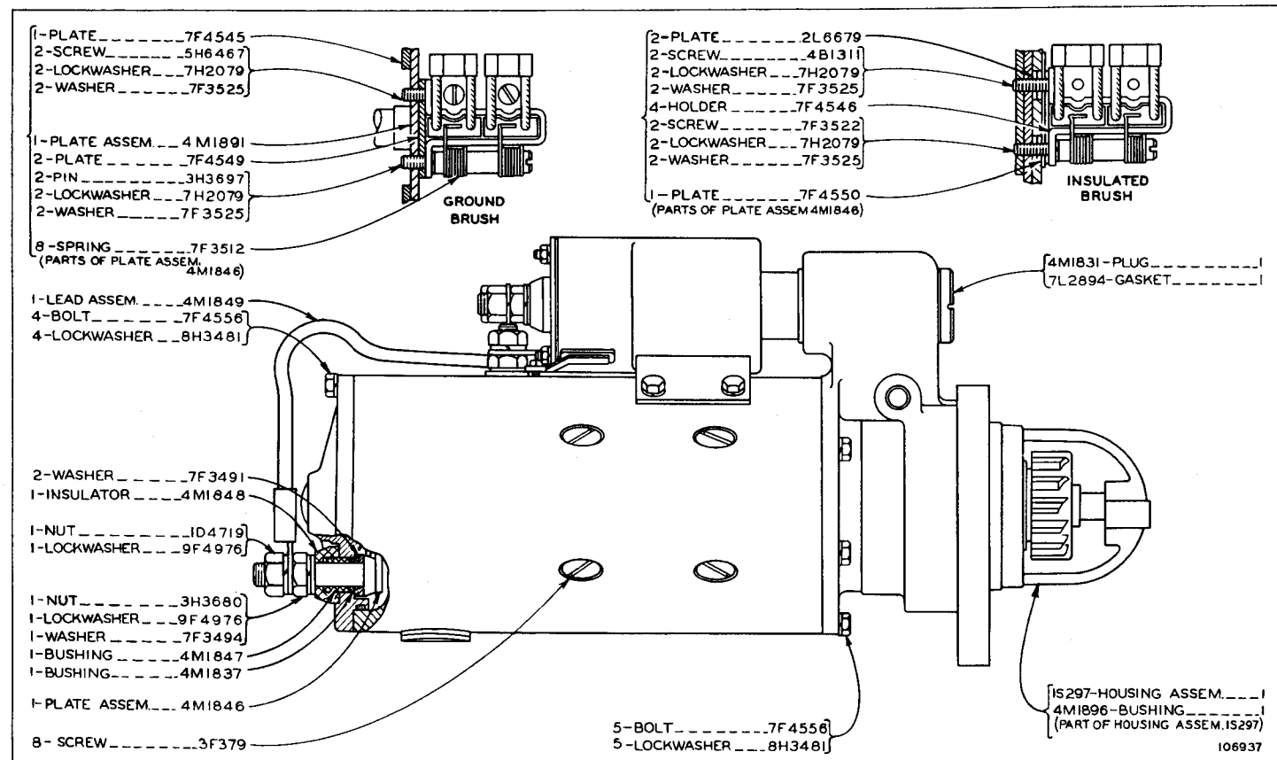
8L5881 STARTING MOTOR ASSEMBLY-12 Volt-Part 1-Type 2 Part of 8L5949 Electric Starting Group and 3N3353 Electrical System shown on Pages 109 and 135
