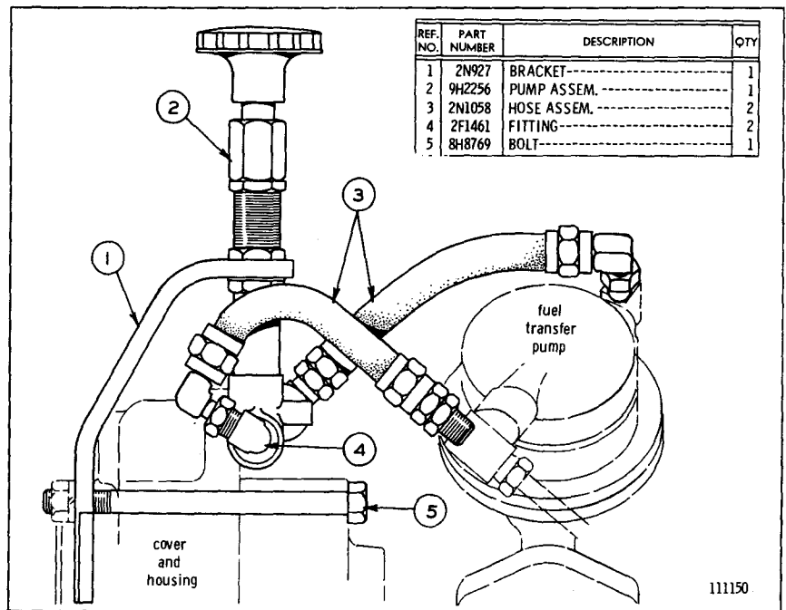
2N1057 FUEL PRIMING PUMP AND LINES GROUP
