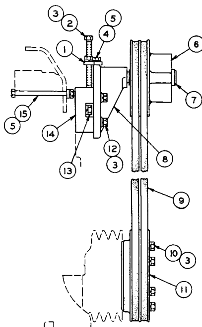
2N223 FAN MOUNTING AND DRIVE GROUP-Type 1
