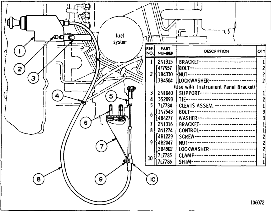
2N1317 GOVERNOR CONTROL GROUP
