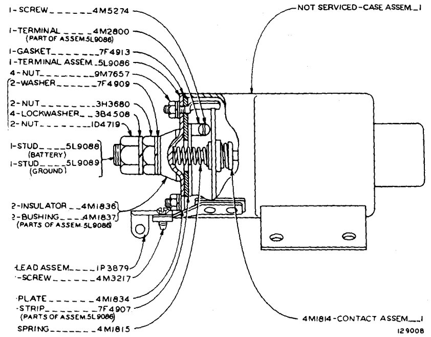
7L6586 SOLENOID SWITCH ASSEMBLY—12 Volt Part of 8L5881 and 9L3597 Motor Assemblies shown on Pages 111, 113, 115 and 117
