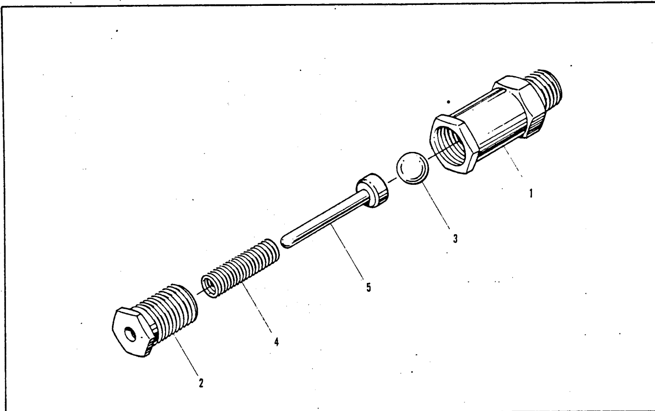
5-5 FIG. , SAFETY VALVE, LL-1034-7 (Model AC-74058-A)
