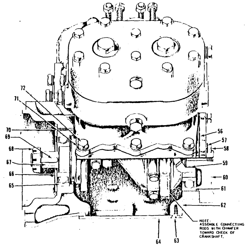
FIG. 5-2, FLANGE TYPE TU-FLO AIR COMPRESSOR ASSEMBLY (Air Brake), LL-529-88 (Model 275725)
