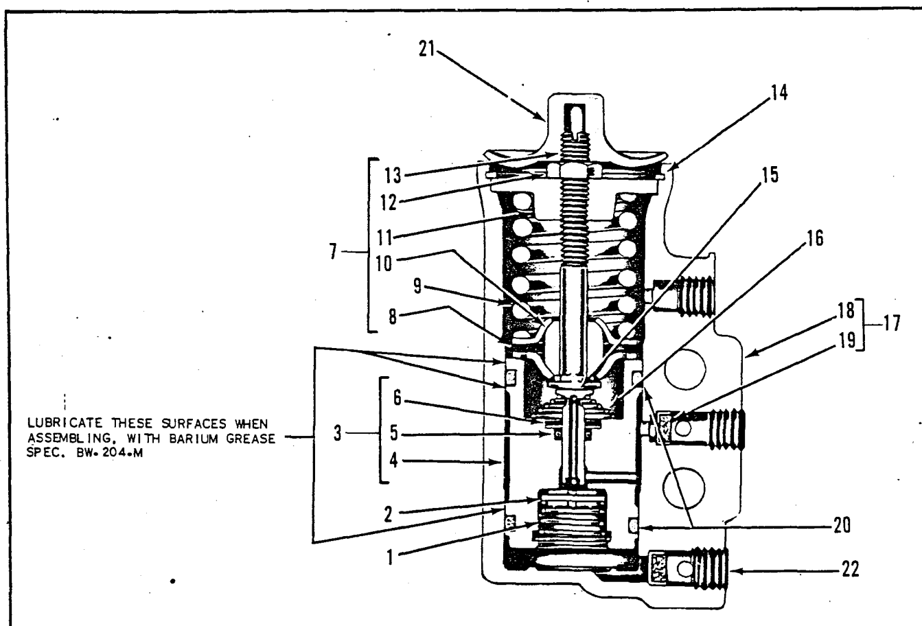
FIG. 5-3, TYPE D2 AIR GOVERNOR ASSEMBLY (Air Brake), LL-529-152 (Model 275200)
