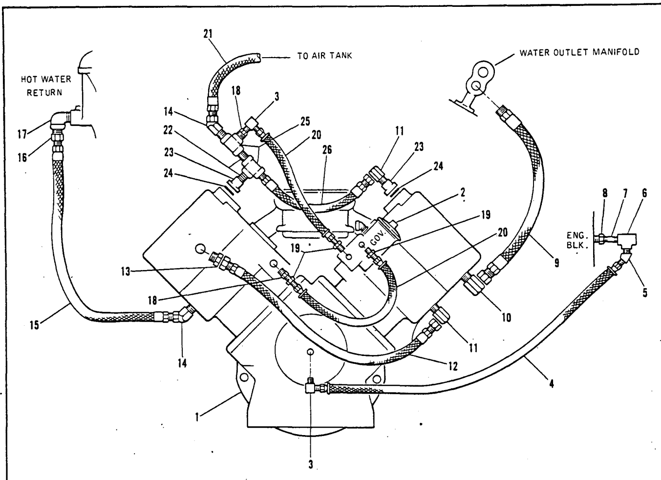
FIG. 5-1A AIR COMPRESSOR CIRCUIT & PLUMBING (by GMC 6-71 Diesel Eng.)
