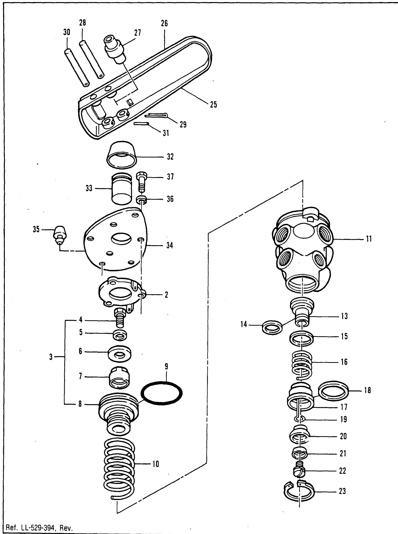
FIG. 5-6, TREADLE VALVE ASSEMBLY (Air Brake), LL-529-394
