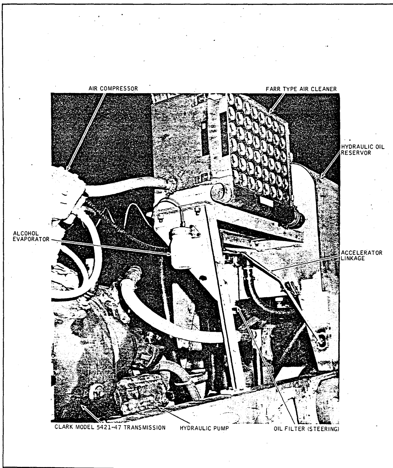
FIG. 5-7 , PHOTO VIEW—ALCOHOL EVAPORATOR, MOUNTING
