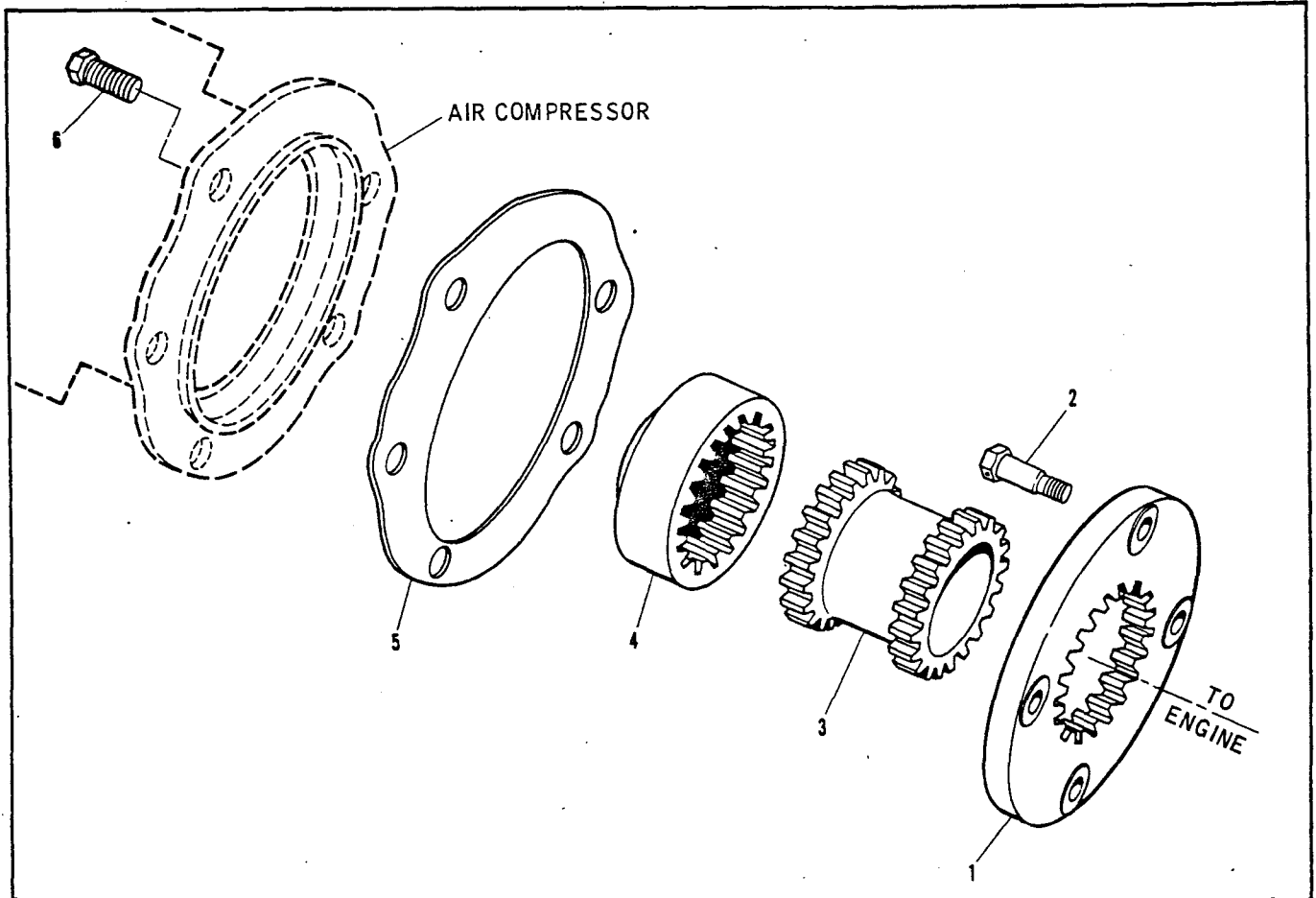
FIG.5-2A, AIR COMPRESSOR DRIVE (Mounted to Eng.) (With GMC Models 6-71, 8V-71 Diesel Eng.)
