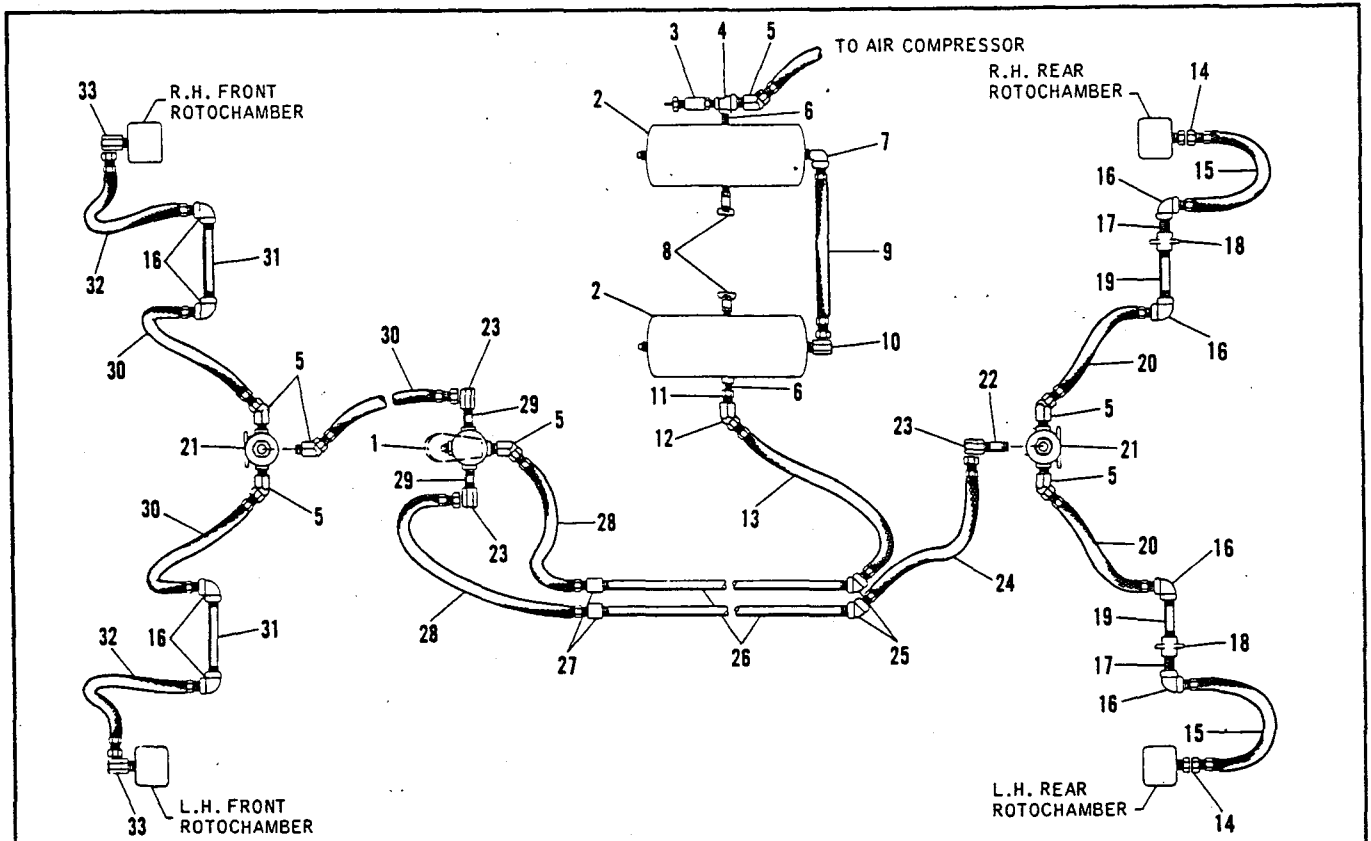
FIG. 5-1, AIR BRAKE CIRCUIT & PLUMBING, BL-6622 (Tank to Valve to Rotochamber)
