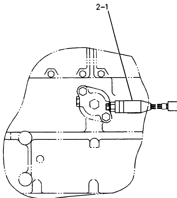
MOUNTING LOCATION FOR OIL PRESSURE SWITCH
