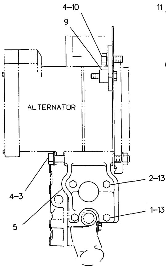
SIDE VIEW OF ENGINE
