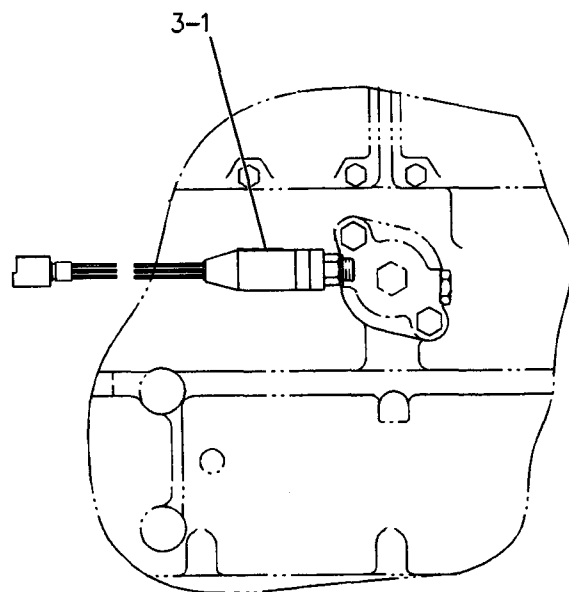
MOUNTING LOCATION FOR OIL PRESSURE SWITCH
