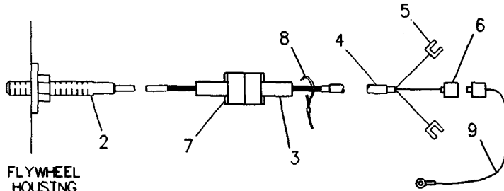
REAR VIEW
