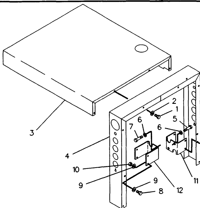
7E1482 ENCLOSURE GP-ENGINE For Use With Mounting & Radiator An Attachment
