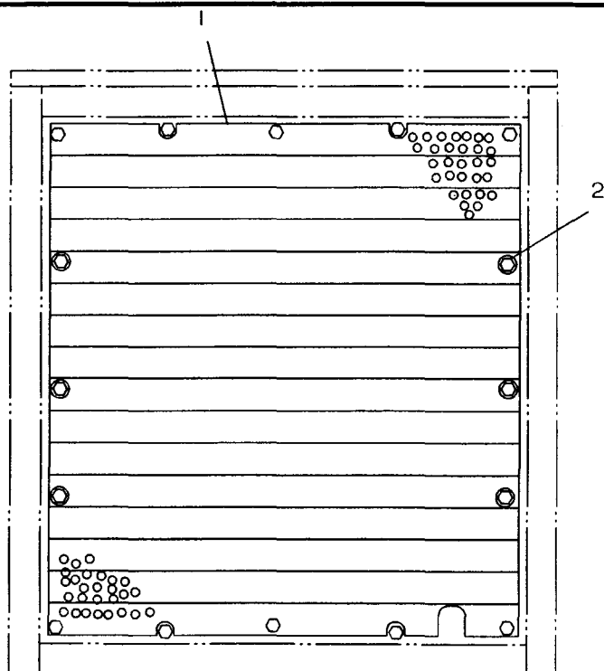
9Y1331 GRILL GP For Use With Radiator Support Gp Or Radiator Module Gp An Attachment
