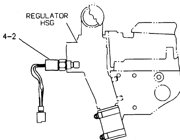
MOUNTING LOCATION FOR WATER TEMPERATURE ALARM CONTACTOR
