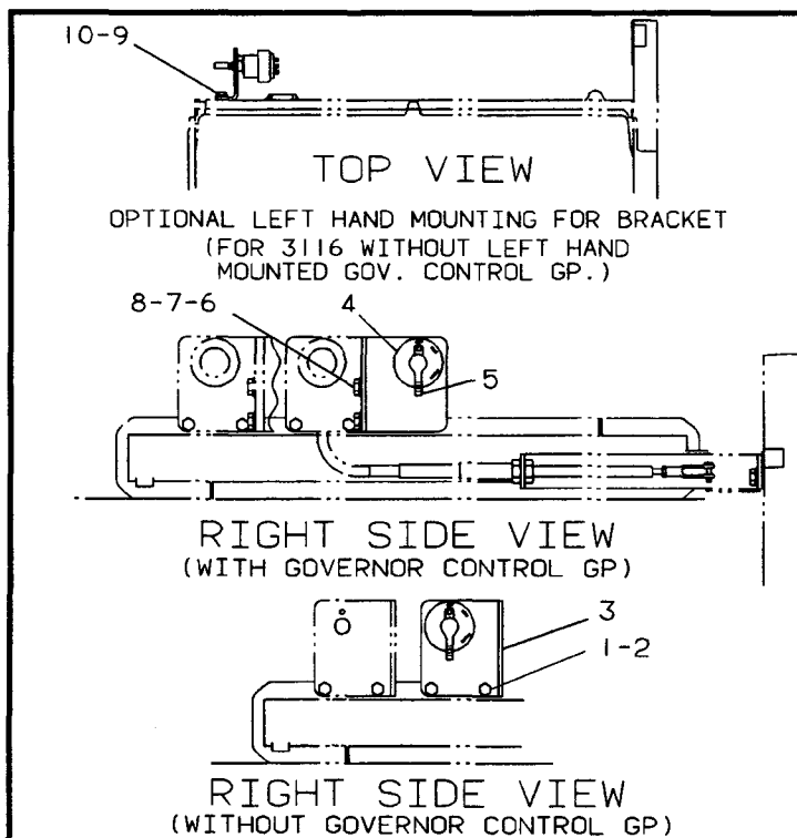
9Y7003 SWITCH GP 9W1077-Page 323
