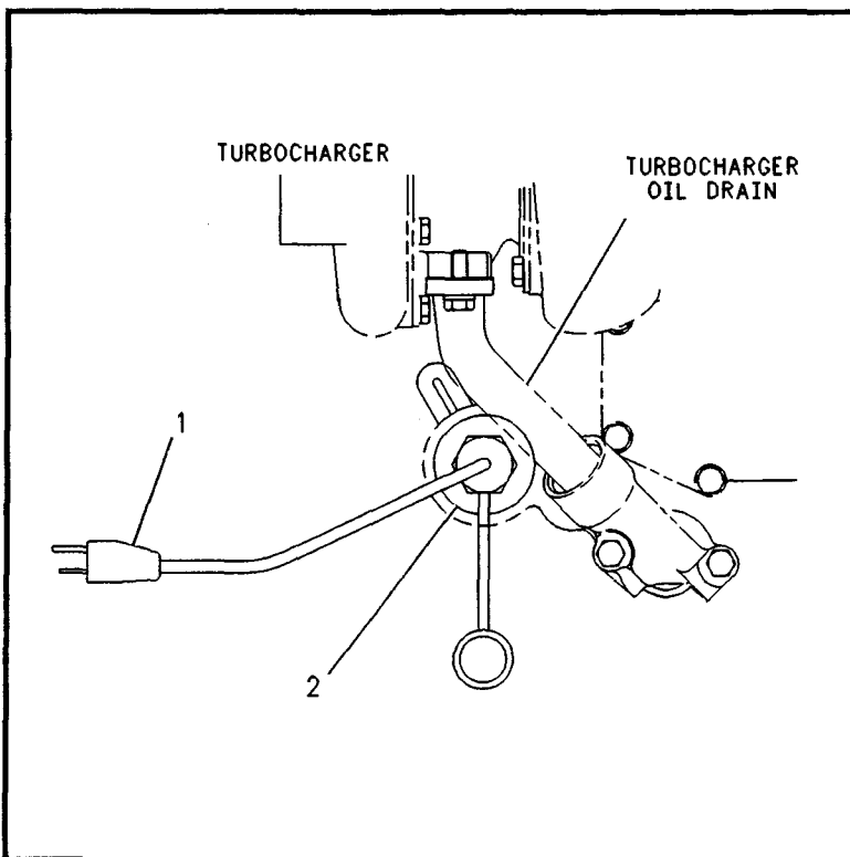
9Y5316 HEATER GP-JACKET WATER
