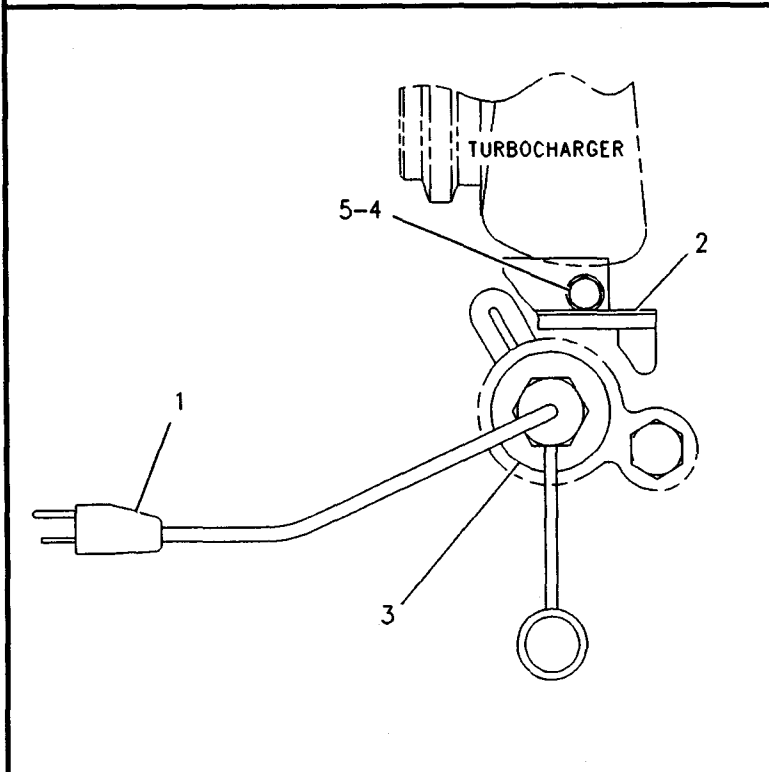
7E6310 HEATER GP-JACKET WATER An Attachment
