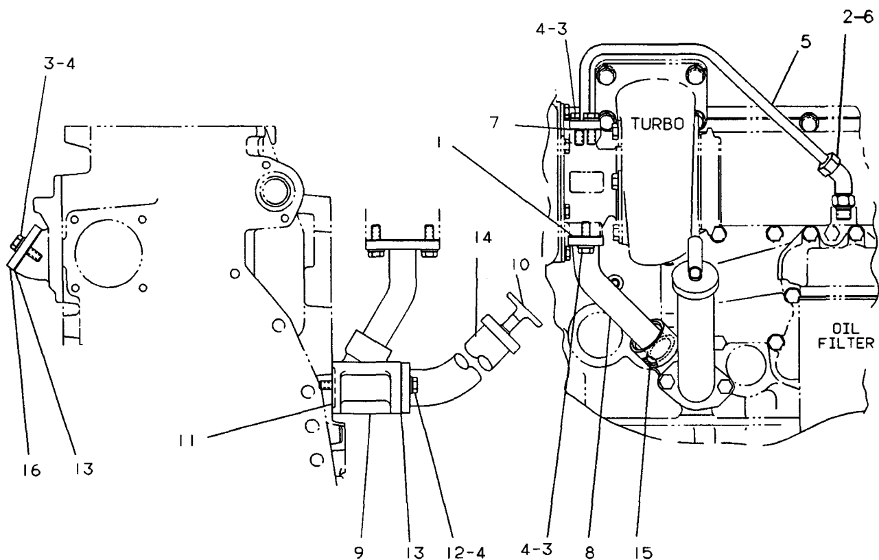
REAR VIEW
