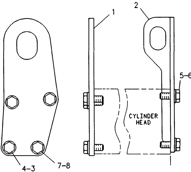
REAR VIEW RIGHT SIDE VIEW
