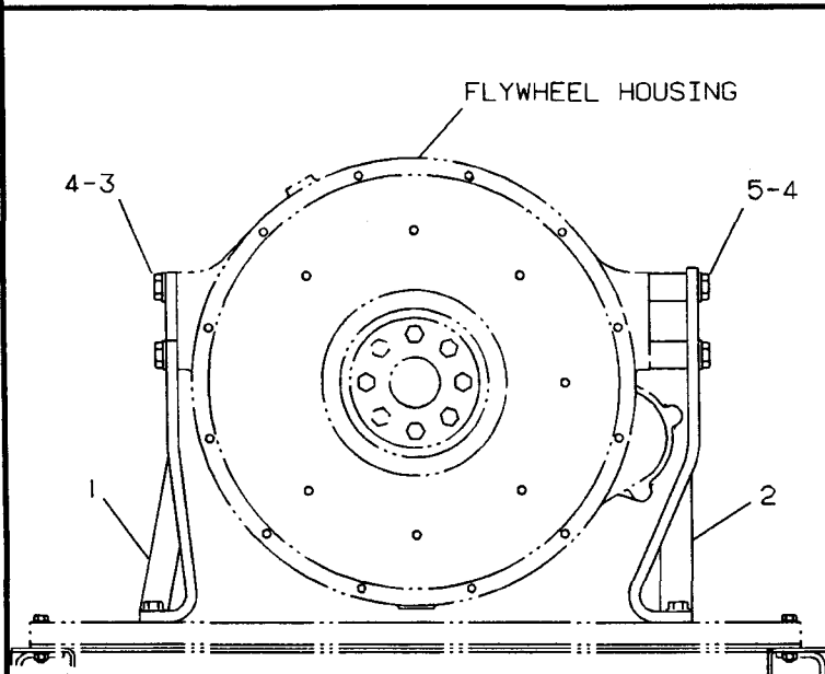
REAR VIEW
