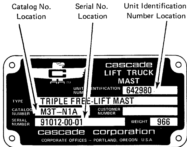
Fig. 1 Product Nameplate
