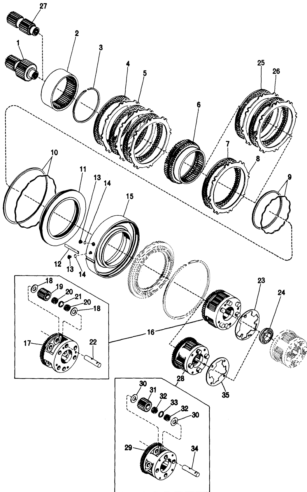
FIG. 9-1. FORWARD CLUTCH AND PLANETARY
