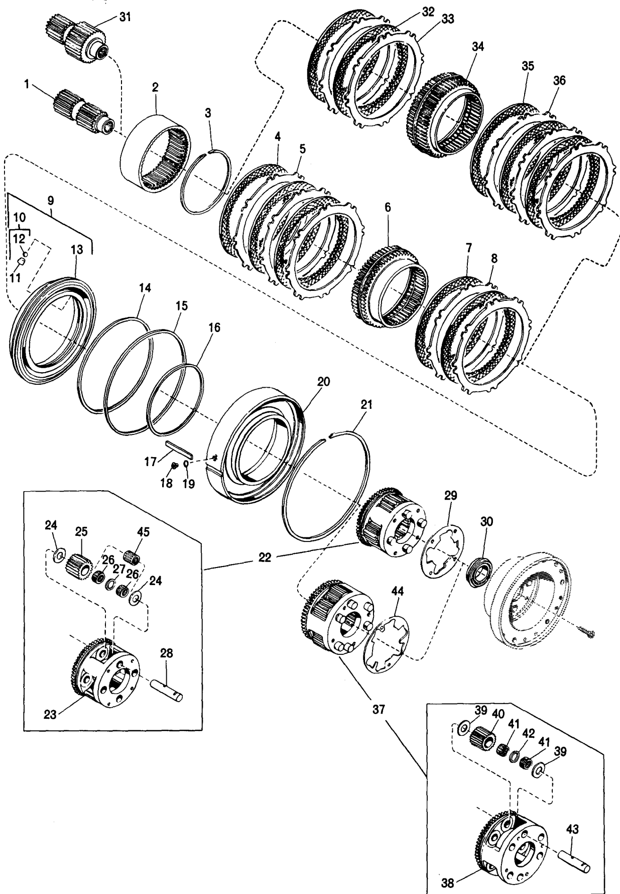
FIG. 9-2. FORWARD CLUTCH AND PLANETARY
