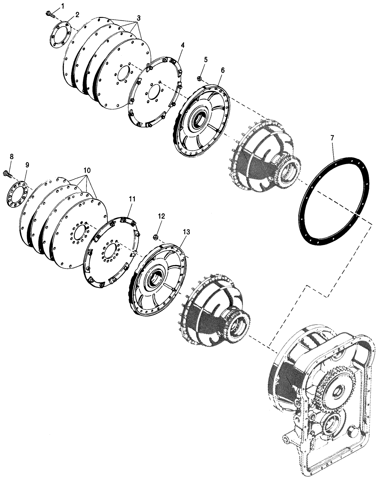
FIG. 3. FLEX DISK AND CONVERTER DRIVE
