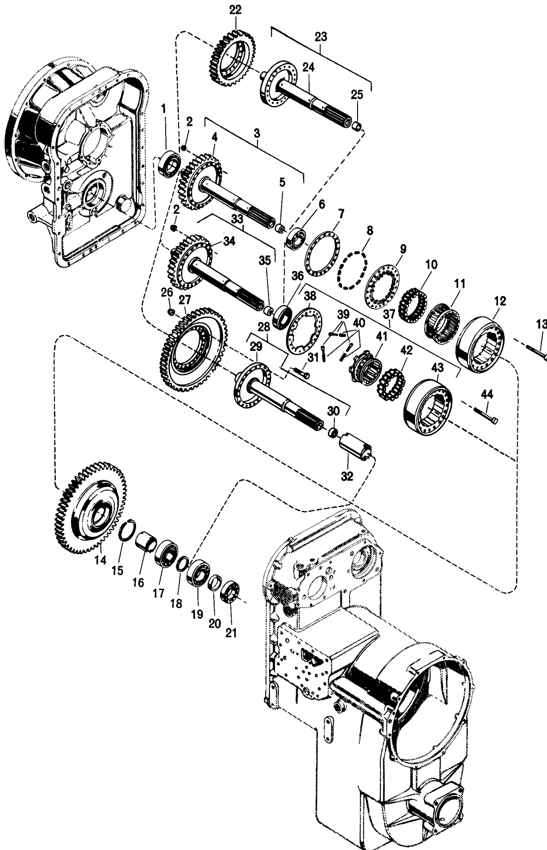
FIG. 6. TURBINE DRIVEN GEARS AND FREEWHEEL UNIT
