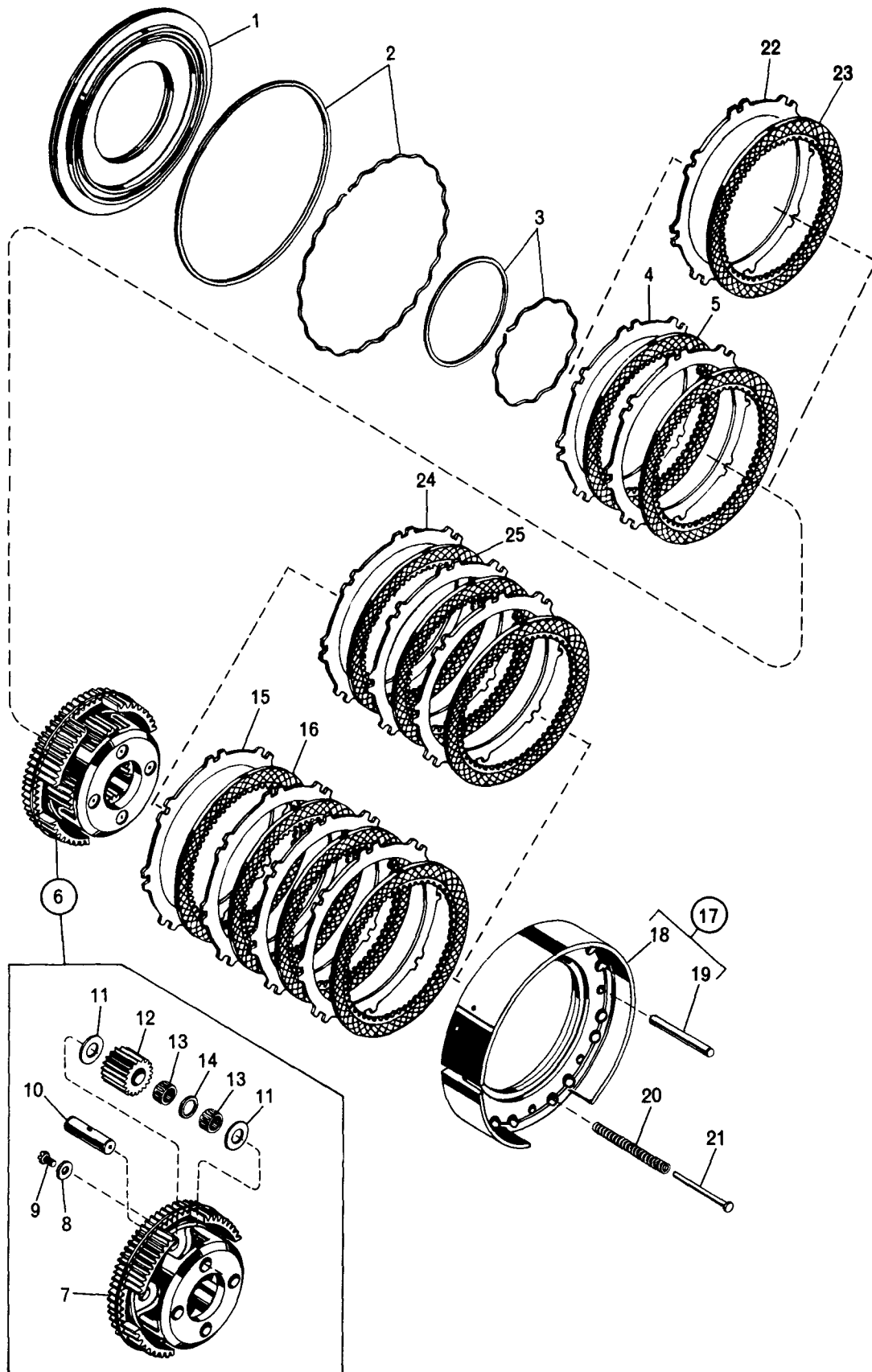
FIG. 8. REVERSE CLUTCH AND PLANETARY
