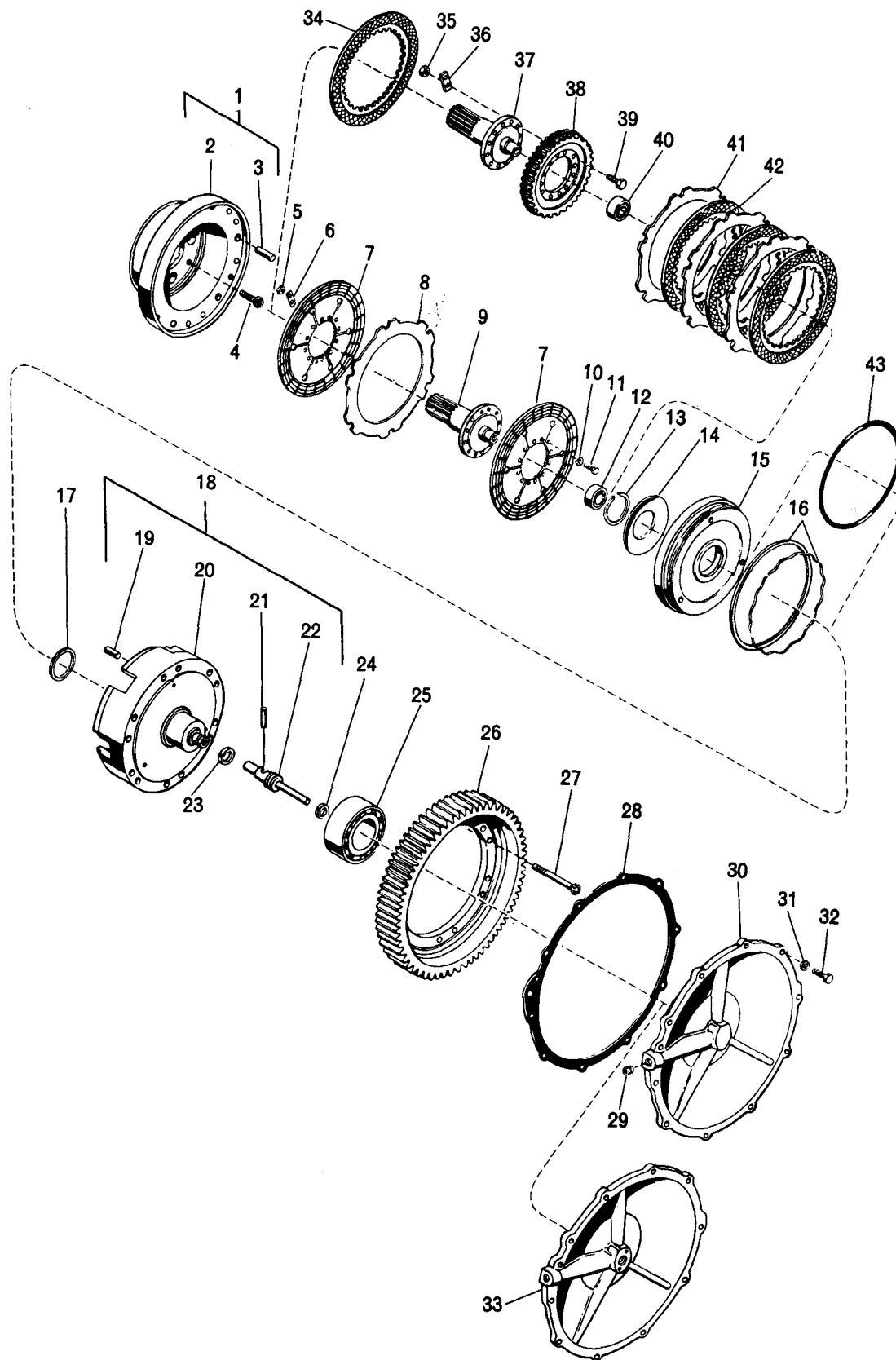
FIG. 10. HIGH-RANGE CLUTCH AND TRANSFER DRIVE GEAR
