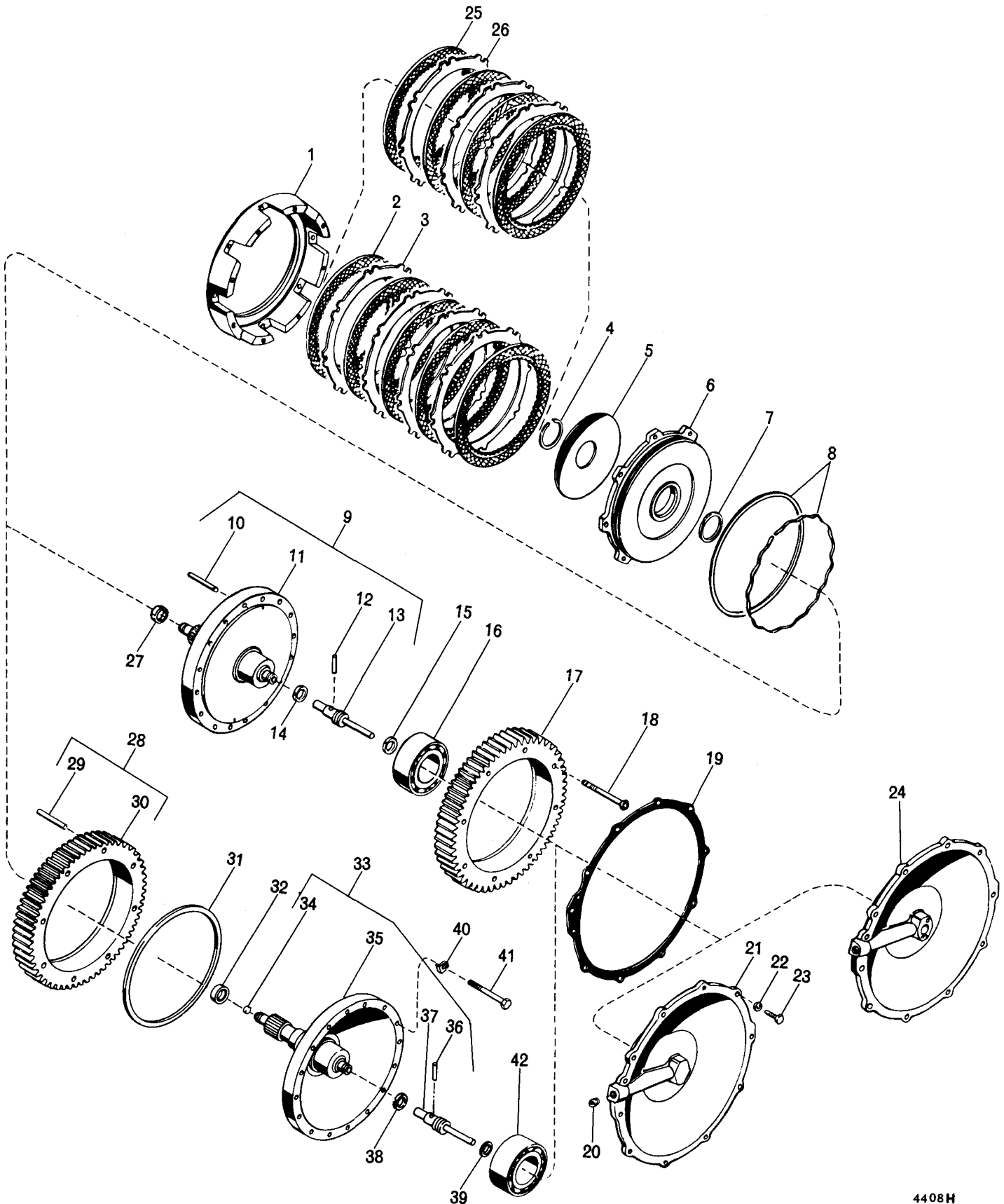
FIG. 11. LOW-RANGE CLUTCH
