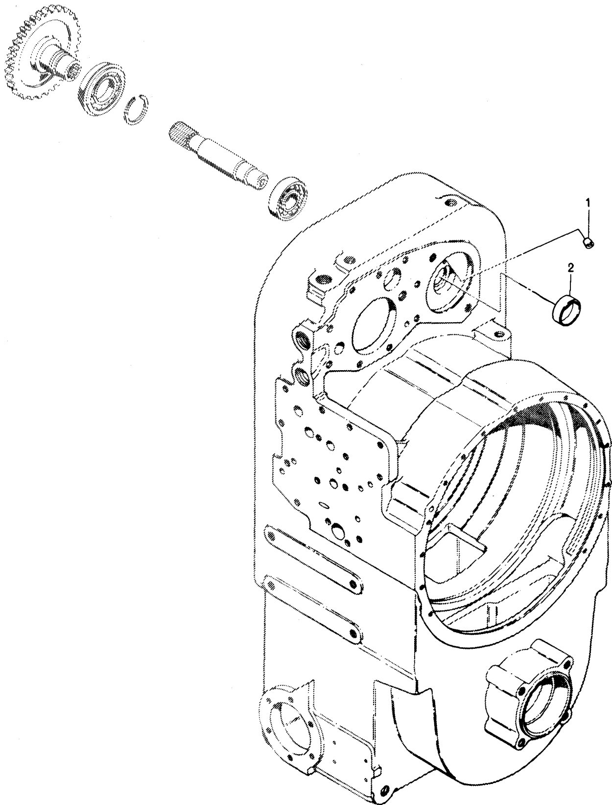
FIG. 15. POWER TAKEOFF
