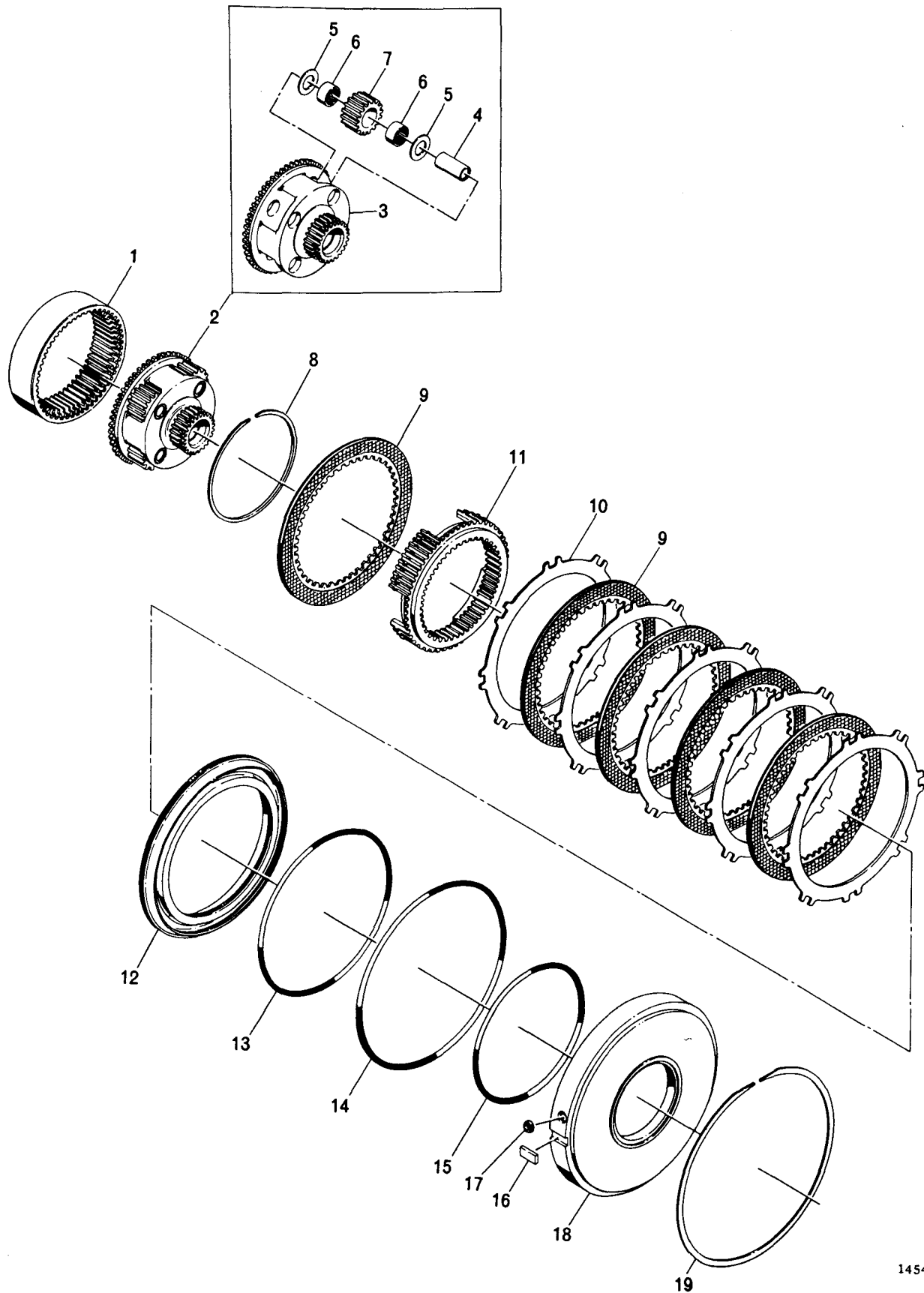
FIG. 9. FORWARD CLUTCH AND PLANETARY
