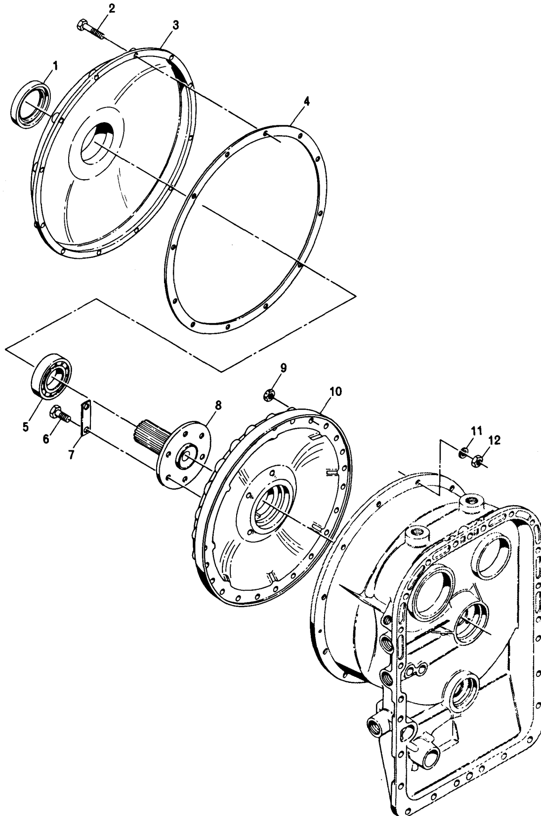
FIG. 2. TRANSMISSION FRONT COVER AND CONVERTER DRIVE
