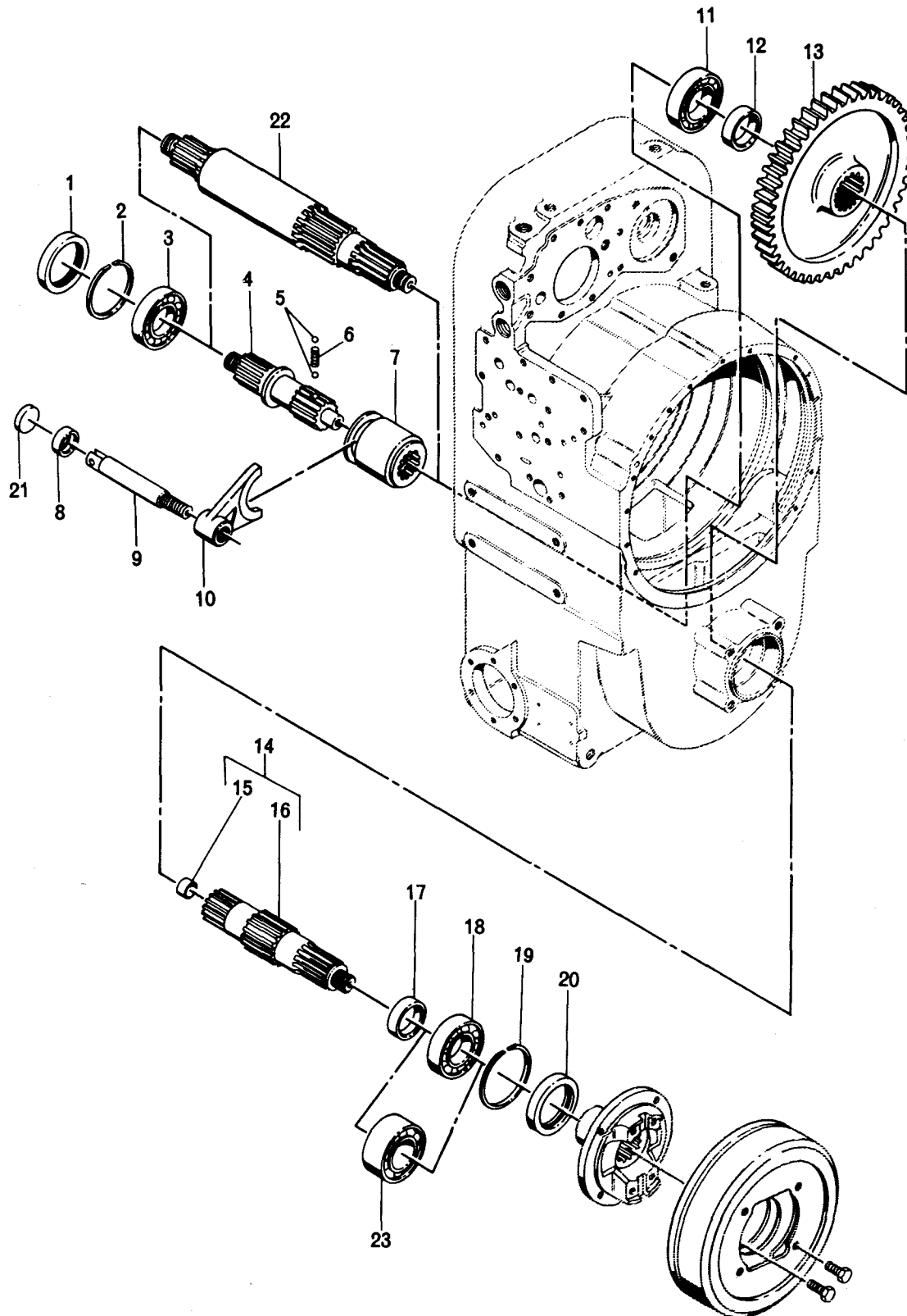
FIG. 12. FRONT OUTPUT DISCONNECT CLUTCH AND REAR OUTPUT SHAFT
