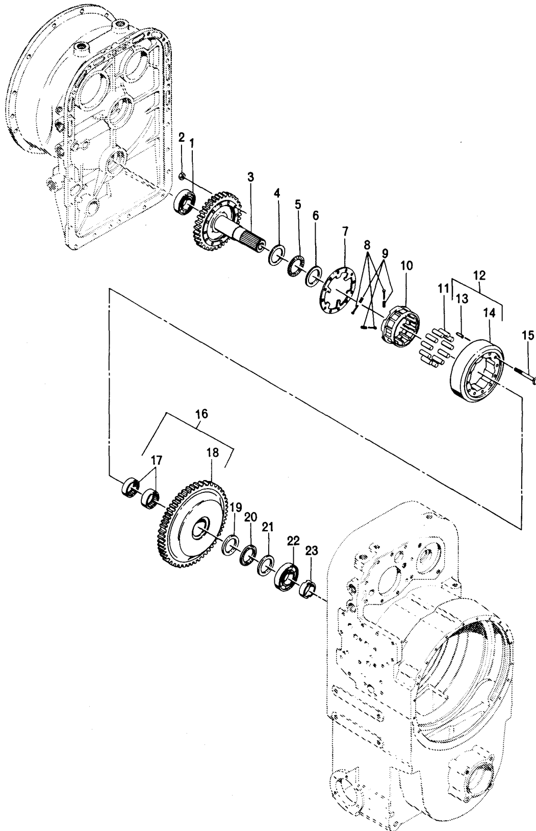
FIG. 6. TURBINE DRIVEN GEARS AND FREEWHEEL UNIT
