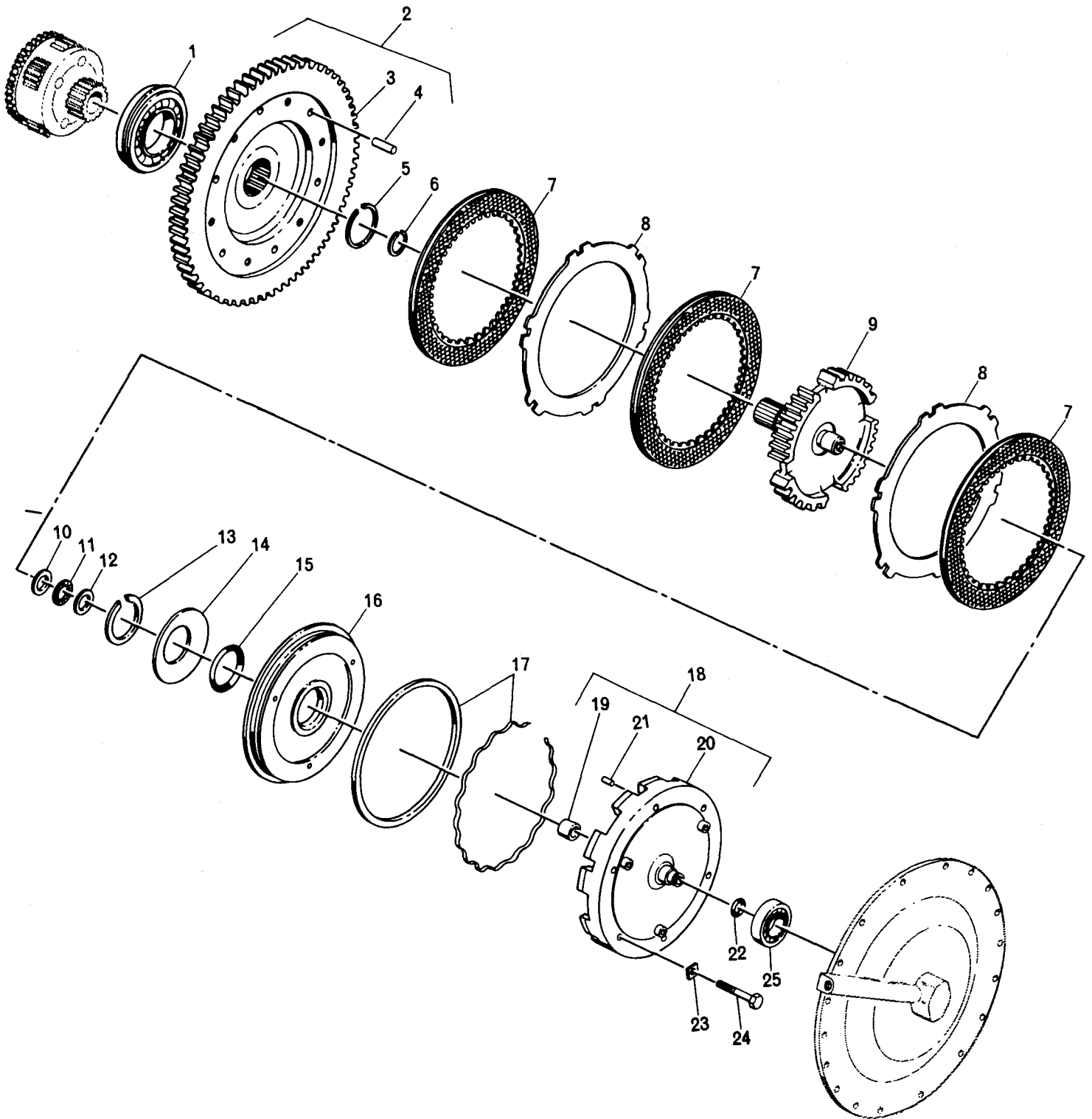
FIG. 10. HIGH-RANGE CLUTCH AND TRANSFER DRIVE GEAR
