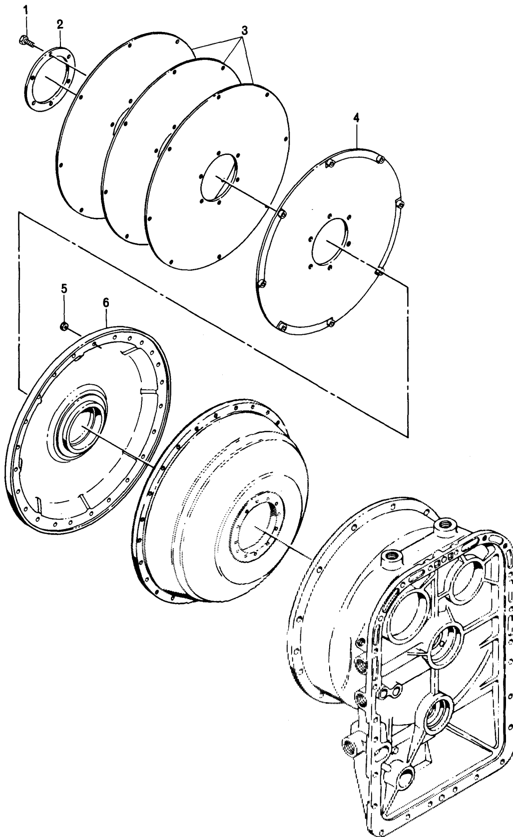
FIG. 3. FLEX DISK, CONVERTER DRIVE AND DRY CONVERTER TYPE HOUSING
