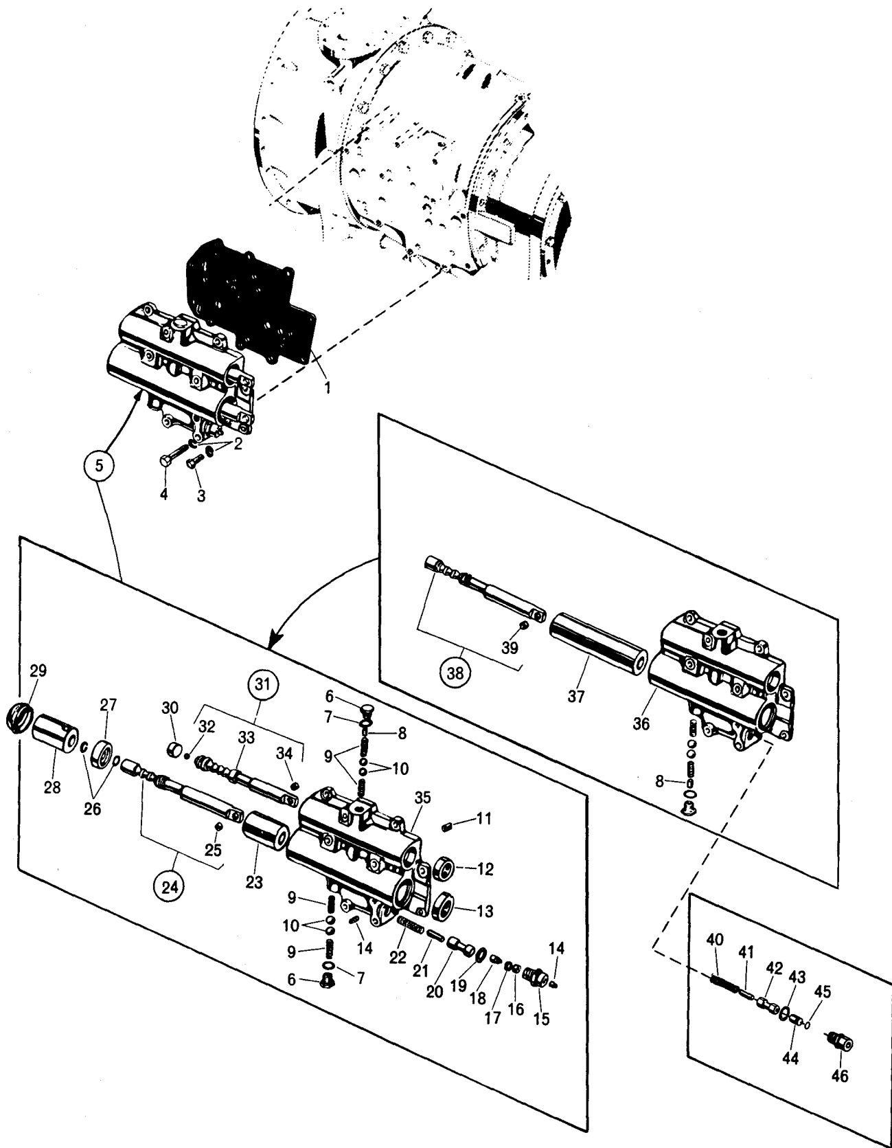
FIG 13-1. CONTROL VALVE BODY
