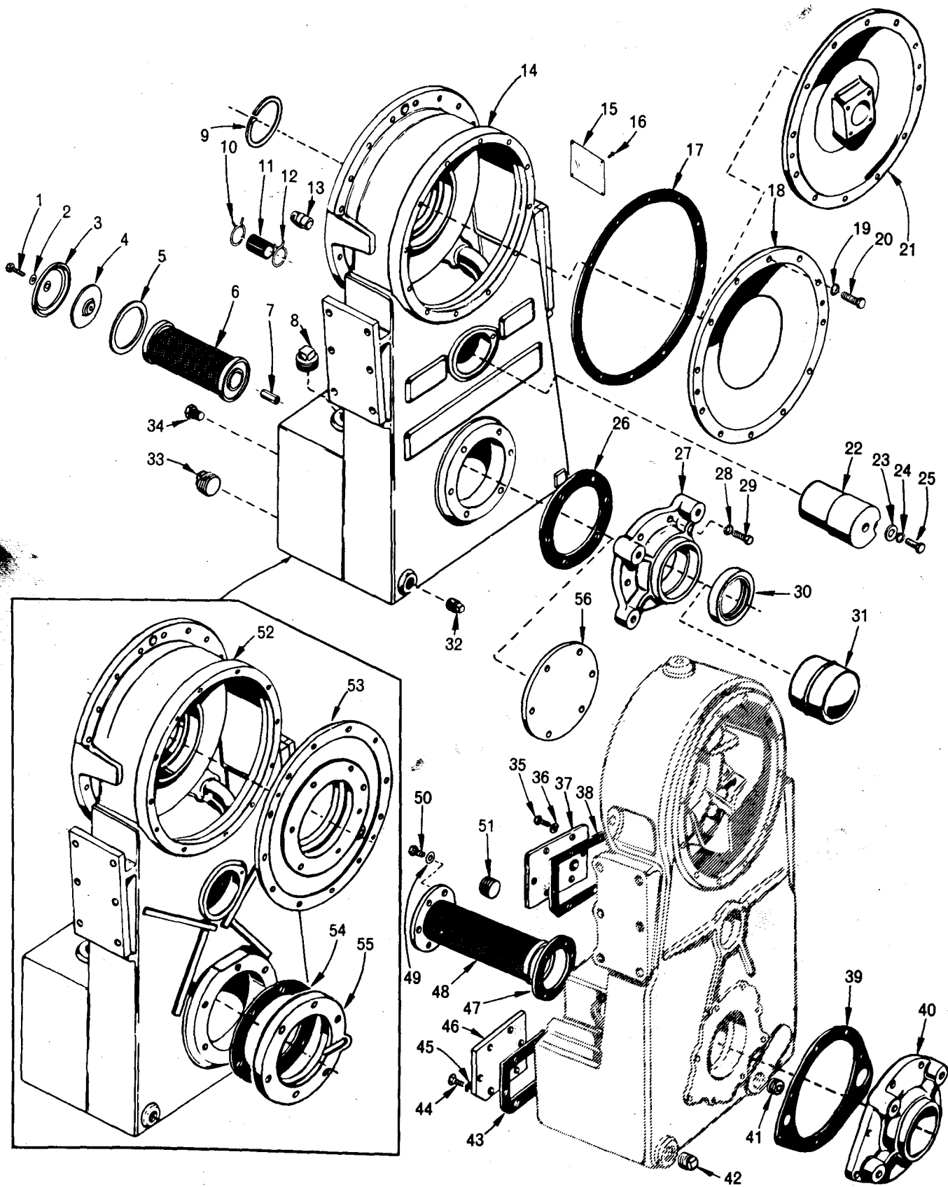
FIG 11. TRANSFER GEAR HOUSING
