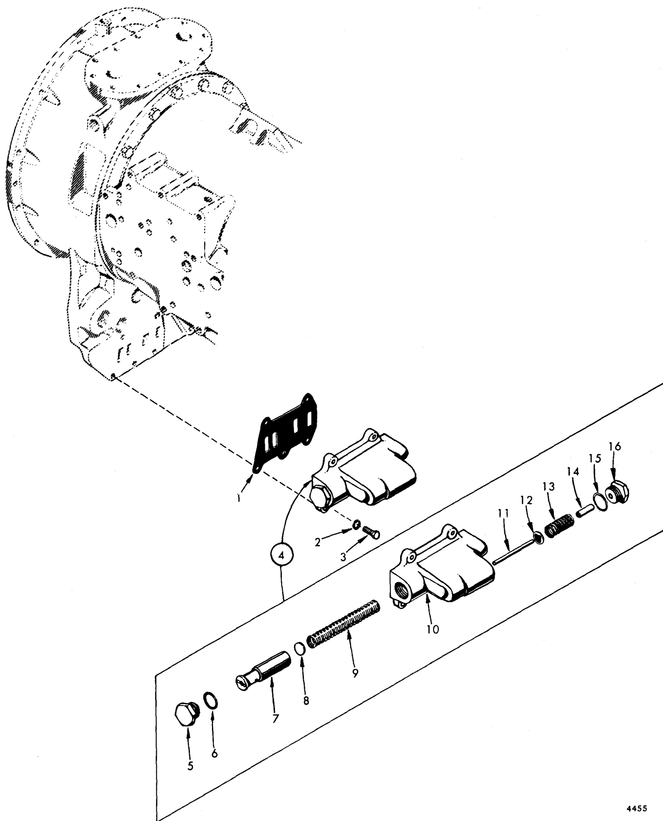
FIG 14. PRESSURE REGULATOR VALVE
