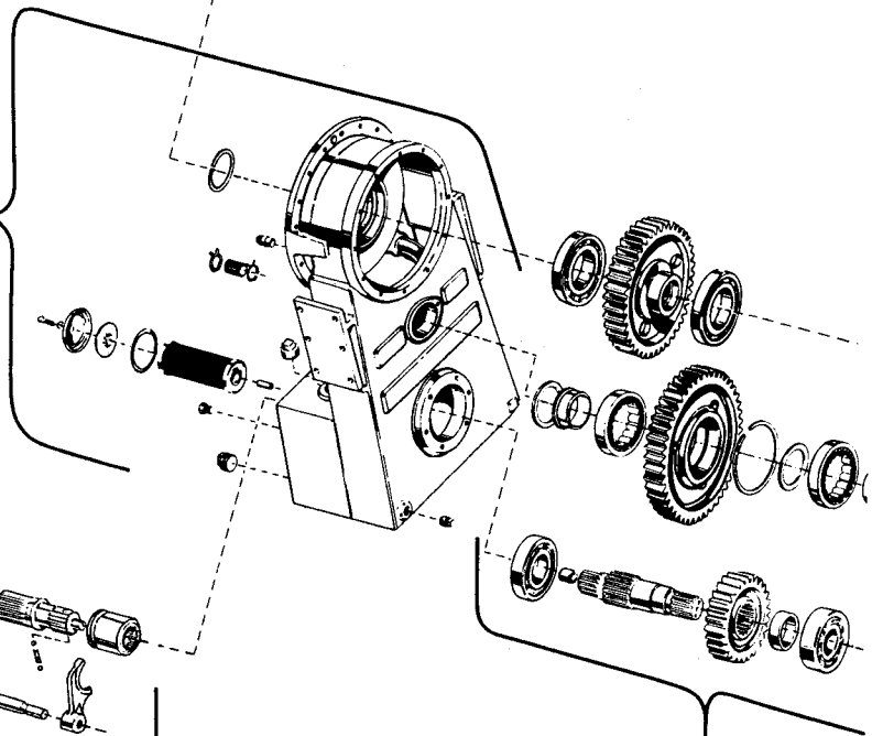
TRANSFER GEAR SECTION Page 12-1.1
