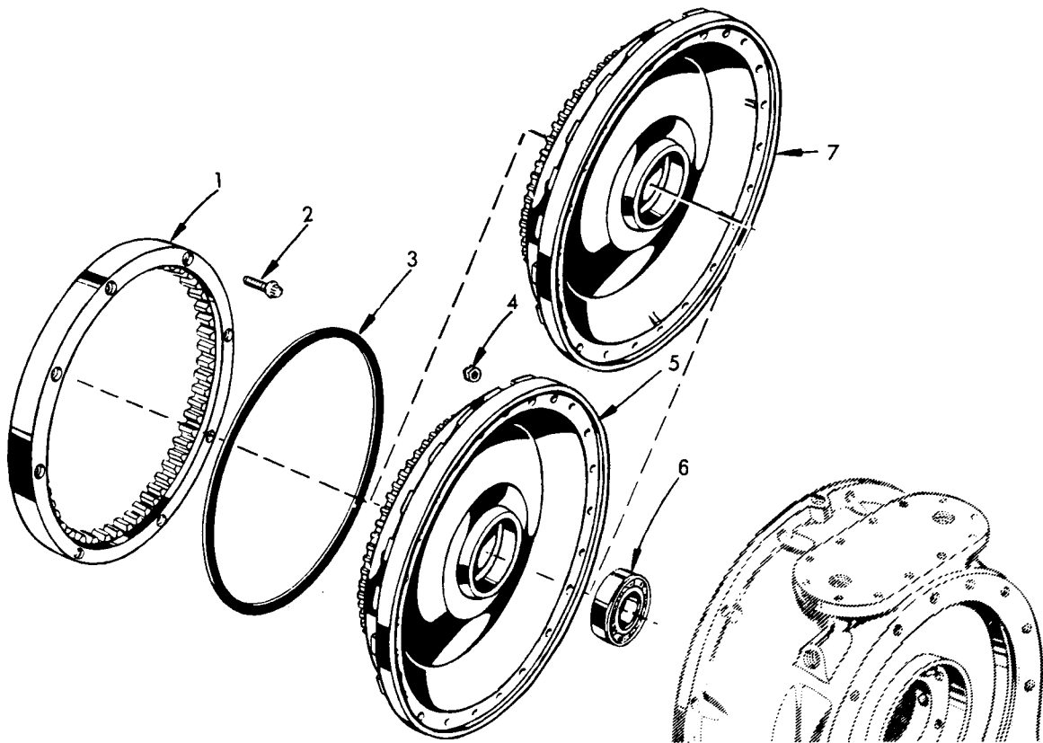
FIG 2. TORQUE CONVERTER DRIVE
