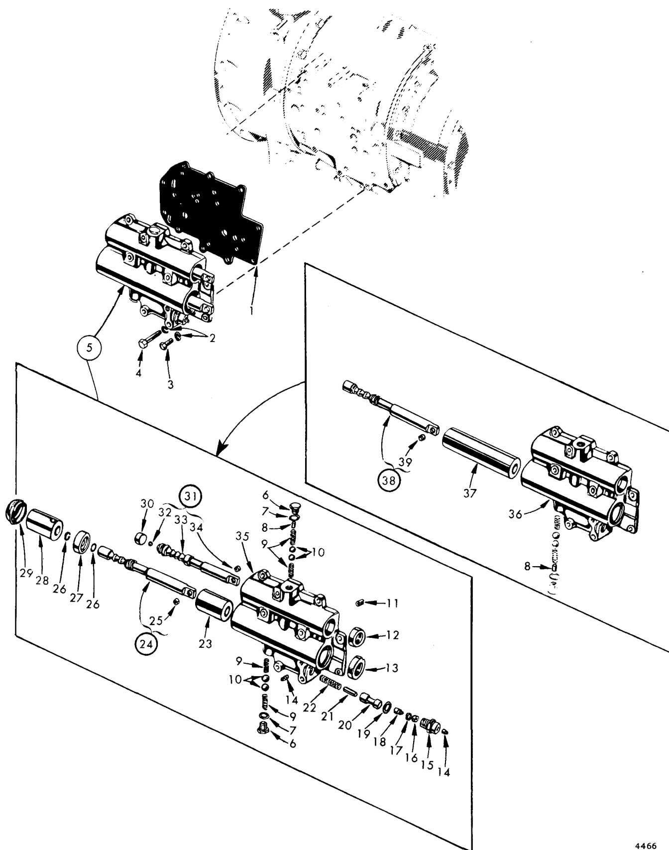
FIG 13-1. CONTROL VALVE BODY SECTION, EXPLODED VIEW.
