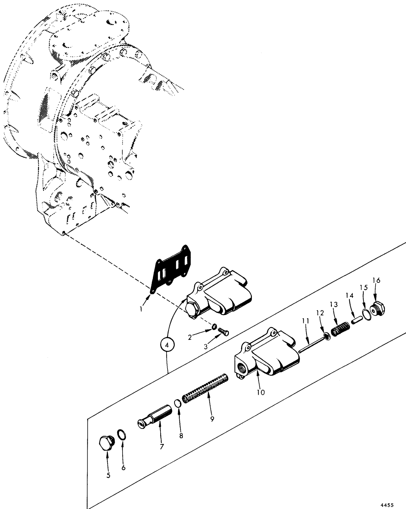
FIG 14. PRESSURE REGULATOR VALVE
