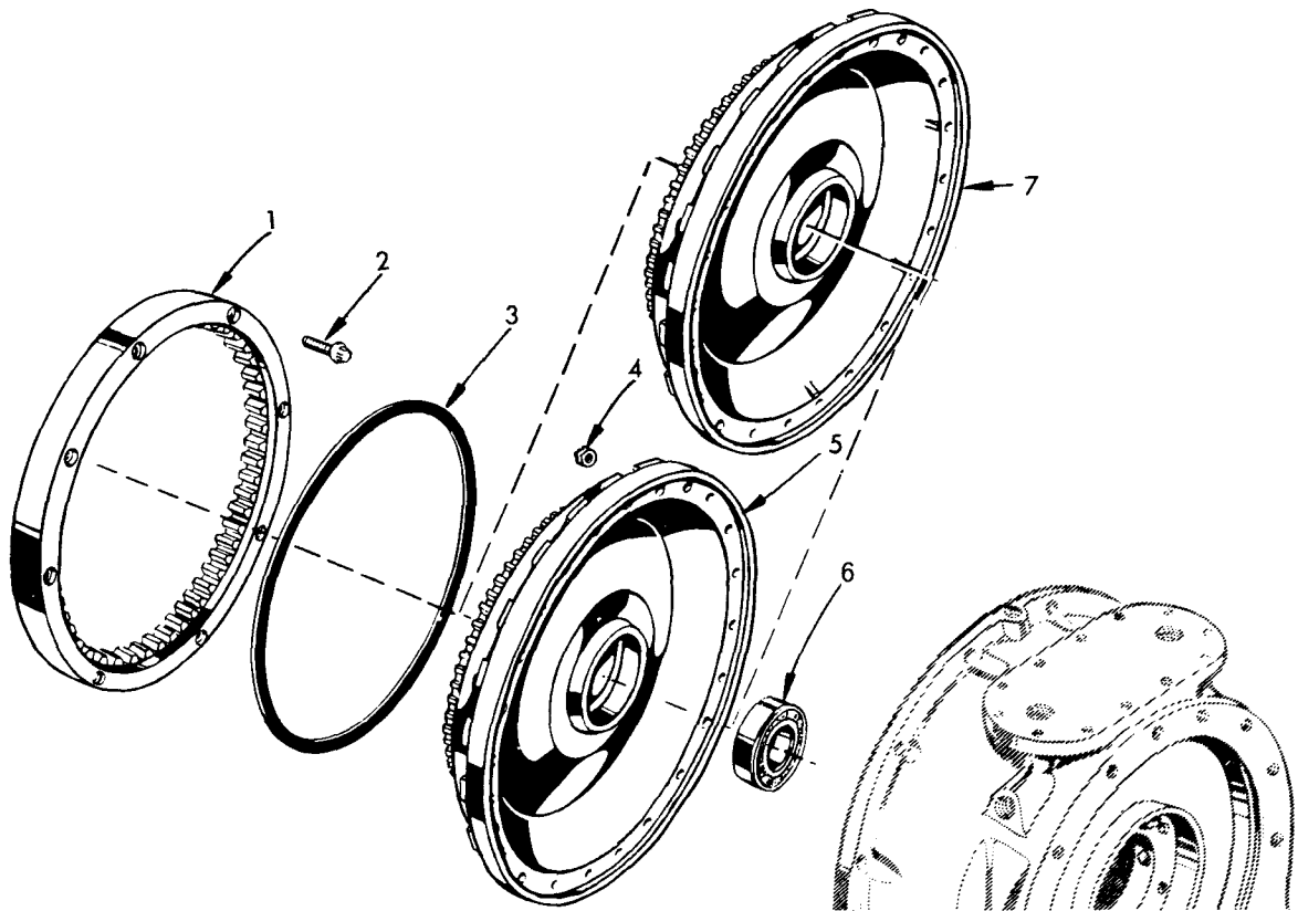
FIG 2. TORQUE CONVERTER DRIVE
