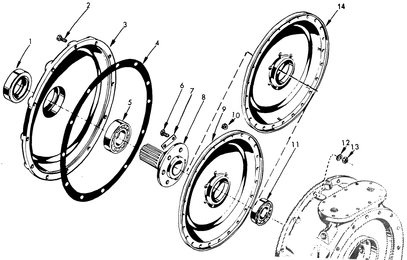
FIG 2. TORQUE CONVERTER DRIVE
