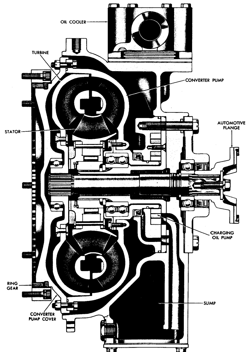
Model TC 300 converter (3-element)—cross-section view
