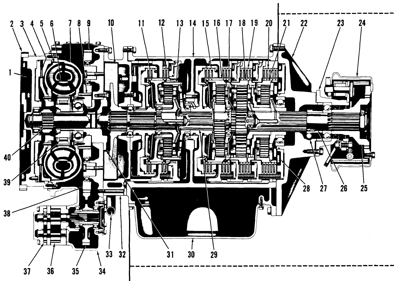
STRAIGHT-THROUGH MODEL WITH PARKING BRAKE
