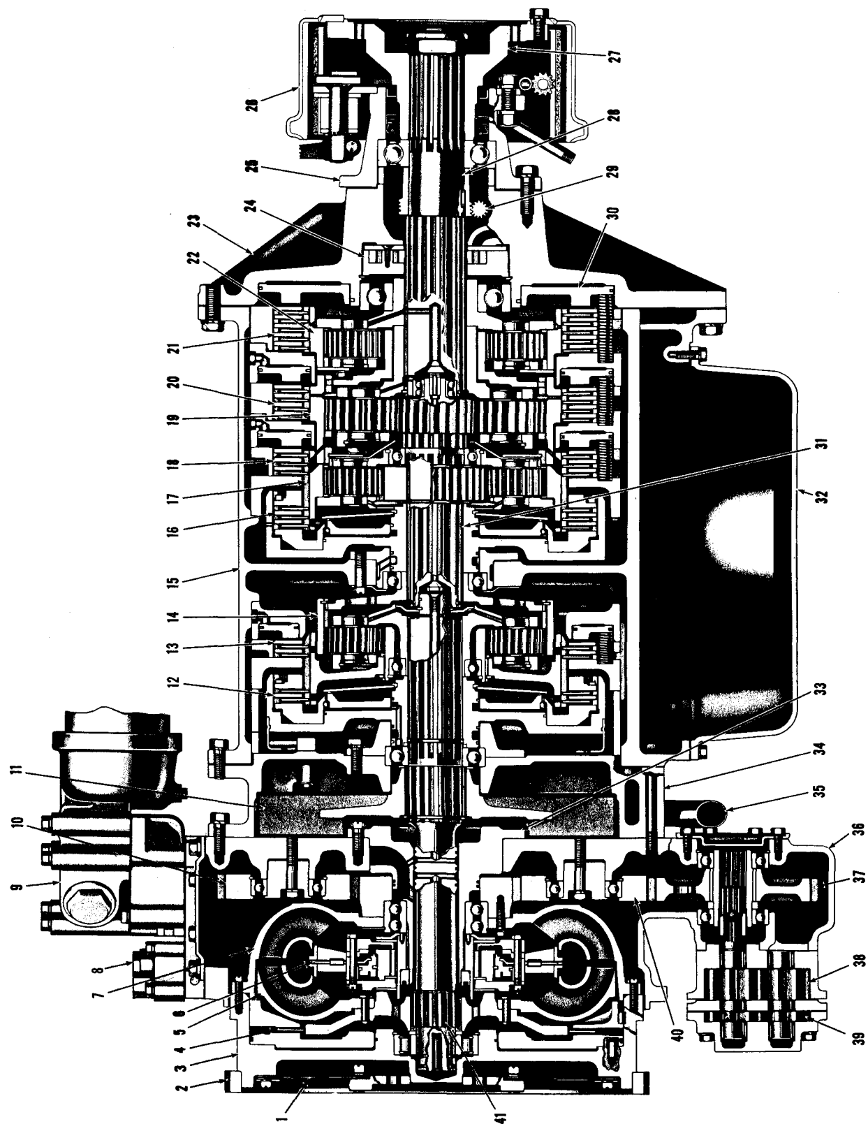
Model VCLBT 5860 Powershift Transmission Cross Section
