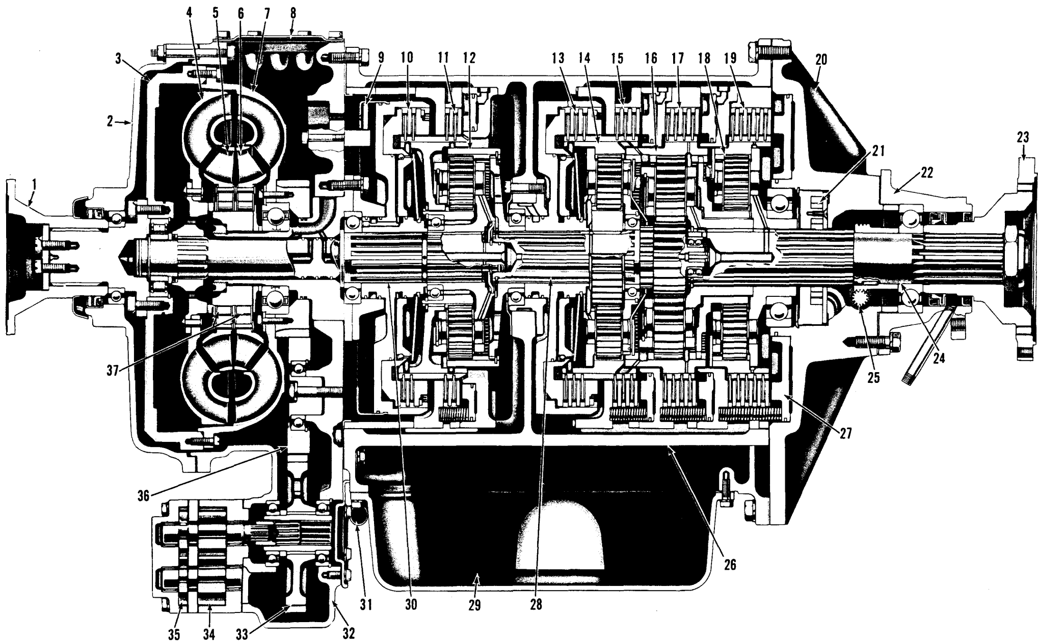
Model CT 5640, 5840, 5860 Powershift Transmission Cross Section
