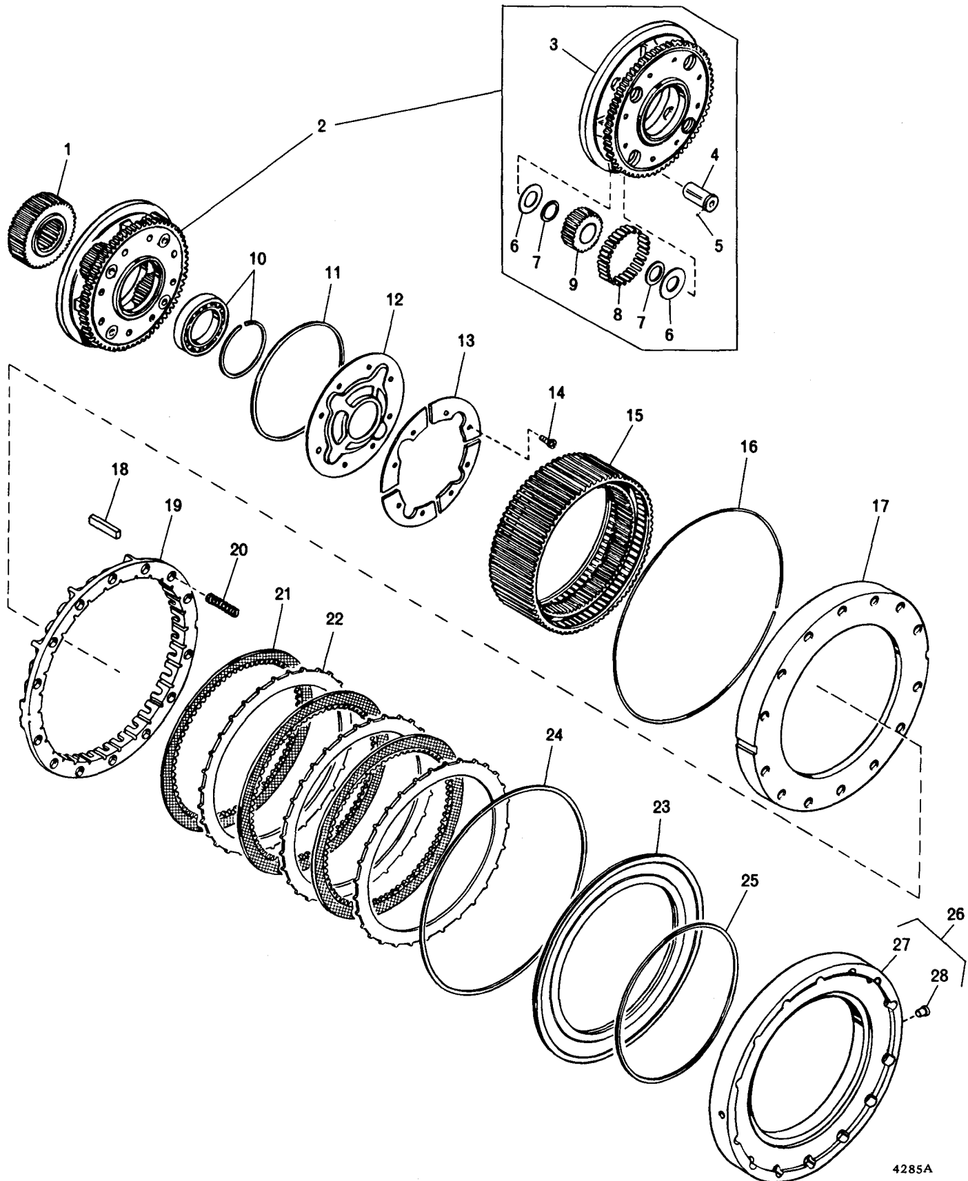
FIG 21. INTERMEDIATE RANGE PLANETARY AND INTERMEDIATE RANGE CLUTCH
