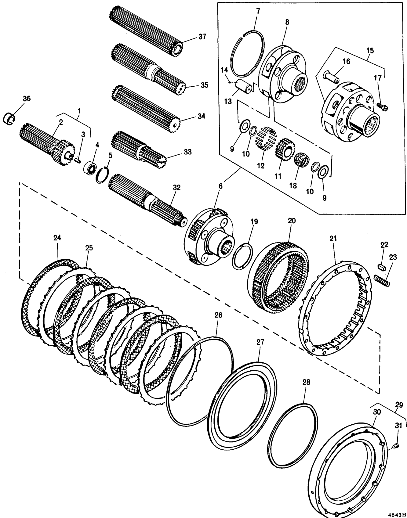
FIG 22. LOW RANGE PLANETARY, LOW RANGE CLUTCH AND OUTPUT SHAFT
