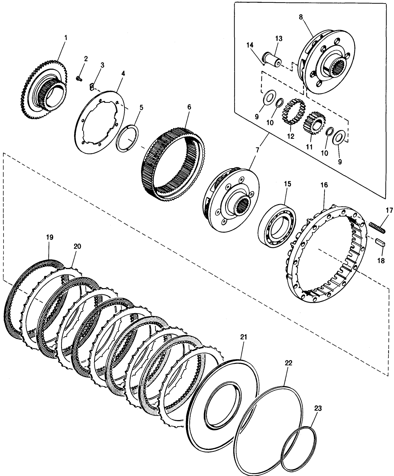
FIG 23. REVERSE RANGE PLANETARY AND REVERSE RANGE CLUTCH
