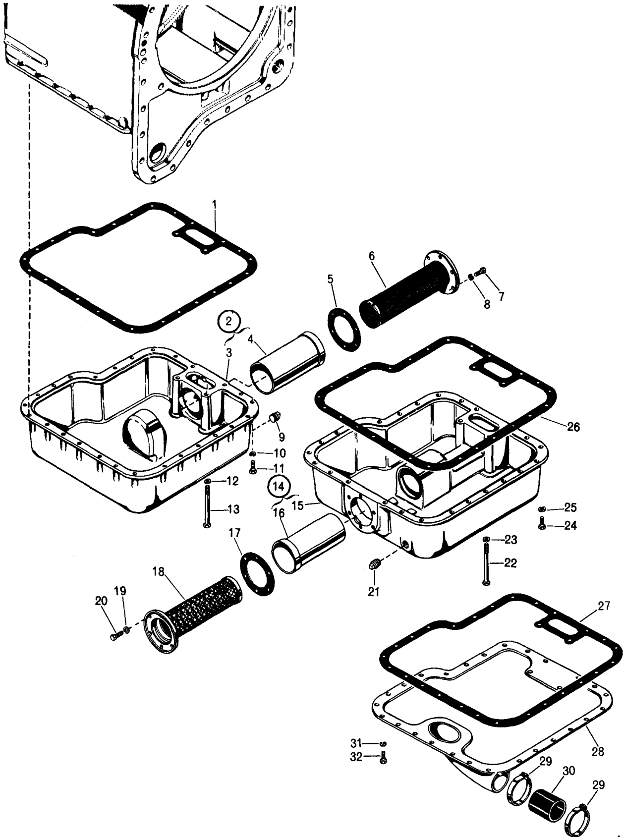
FIG 20. OIL PAN
