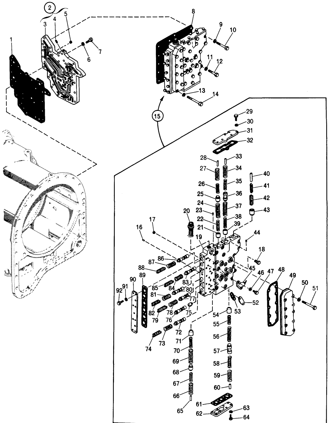
FIG 19-3 CONTROL VALVE BODY
