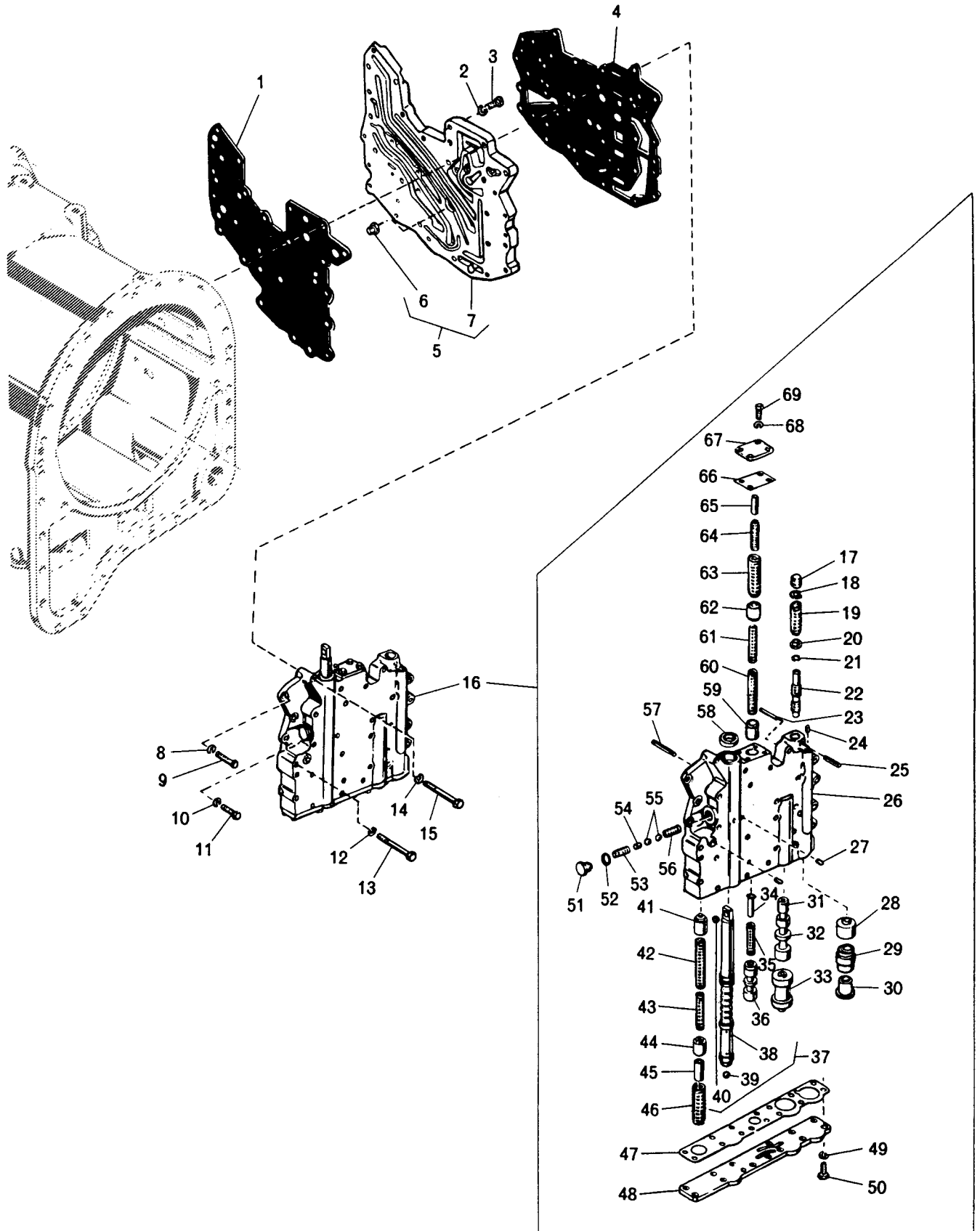
FIG 19-1 CONTROL VALVE BODY
