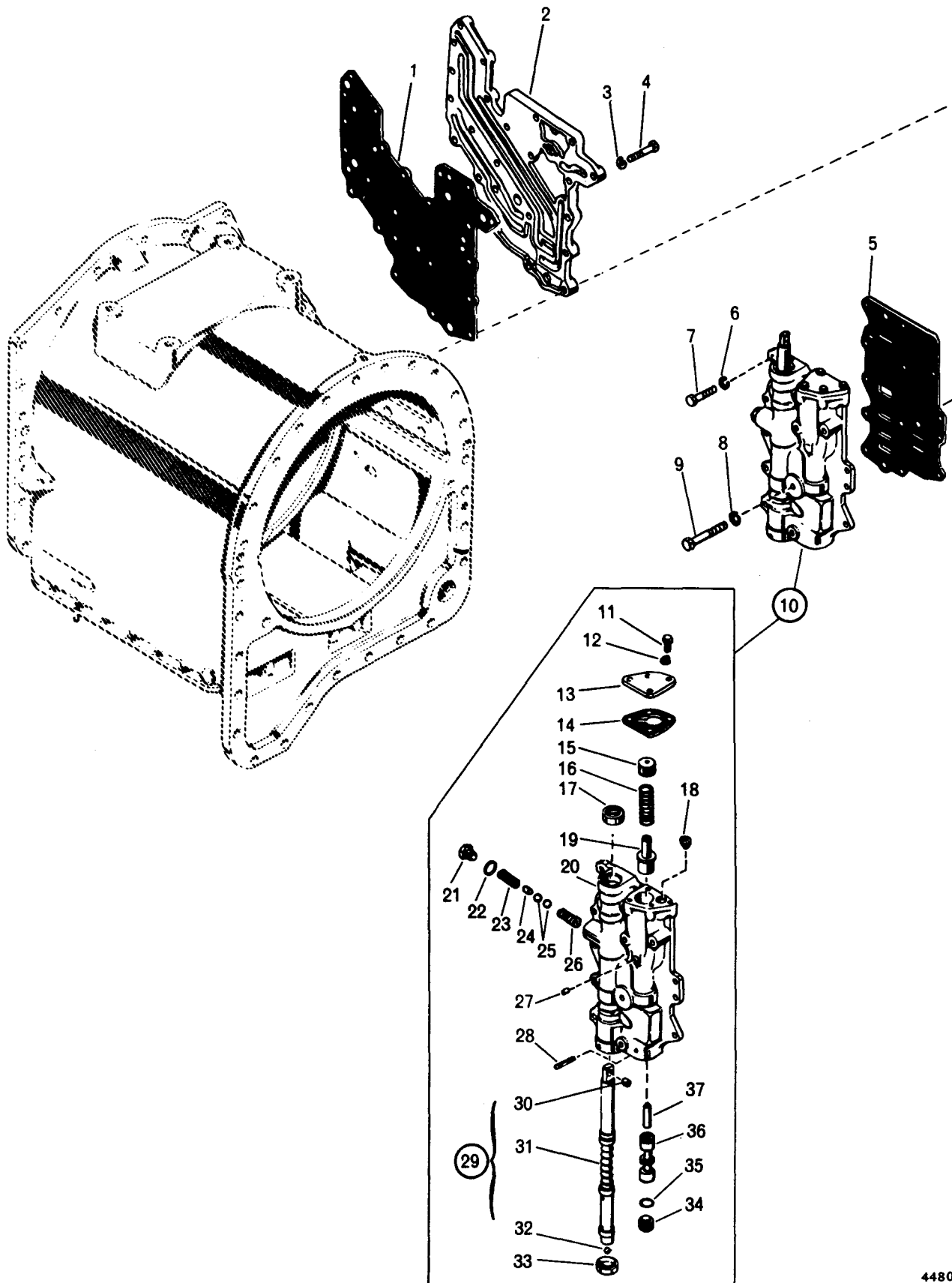
FIG 19 CONTROL VALVE BODY
