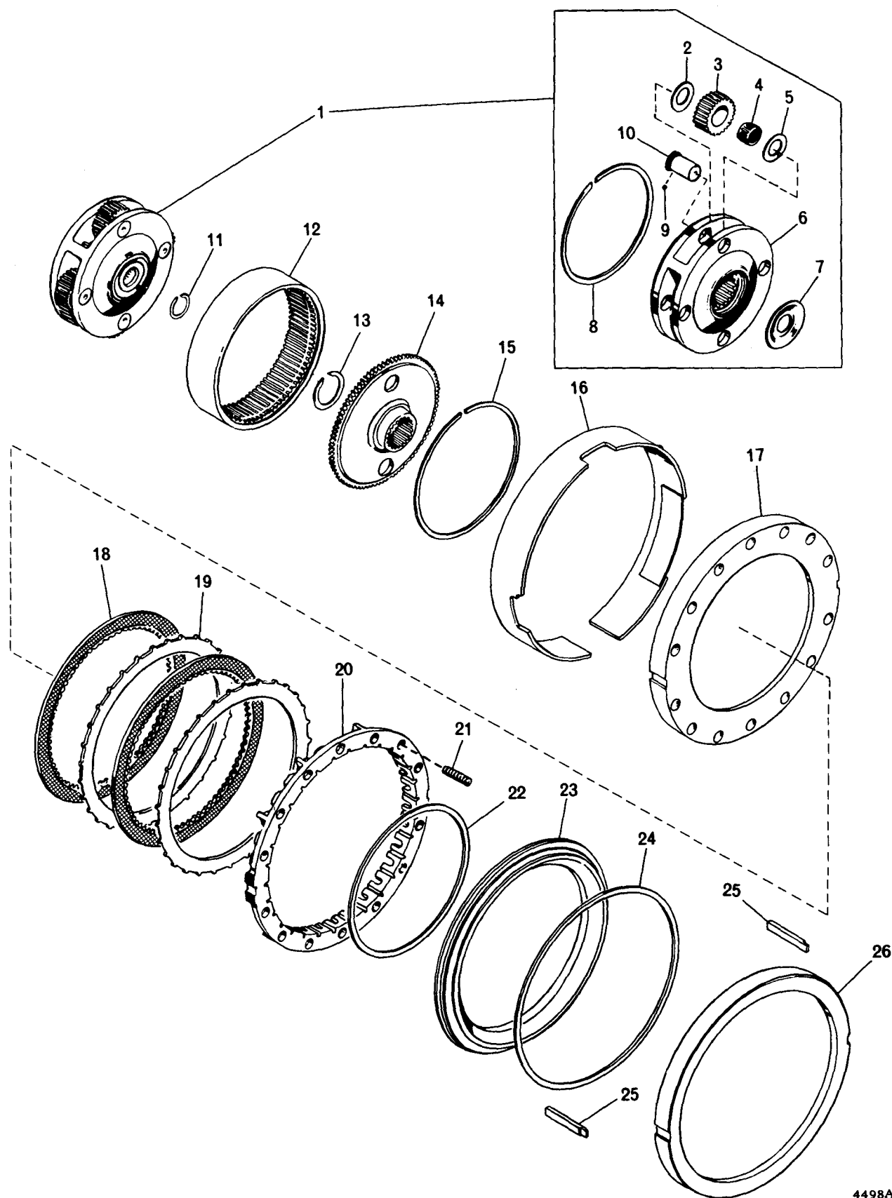
FIG 16 SPLITTER LOW RANGE AND SPLITTER HIGH RANGE PLANETARY AND SPLITTER HIGH RANGE CLUTCH
