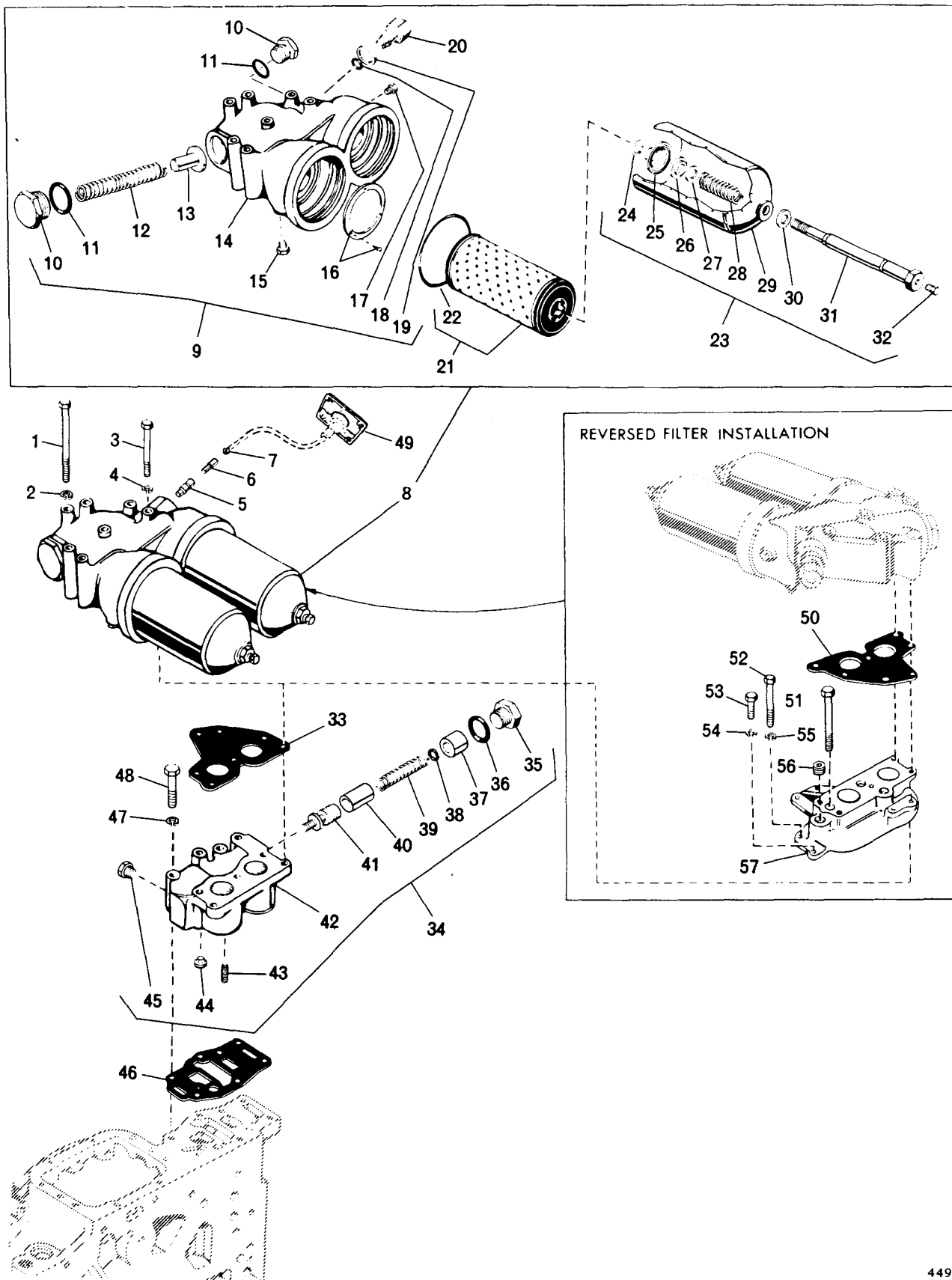
FIG 11-1 MAIN PRESSURE REGULATOR VALVE AND OIL FILTER
