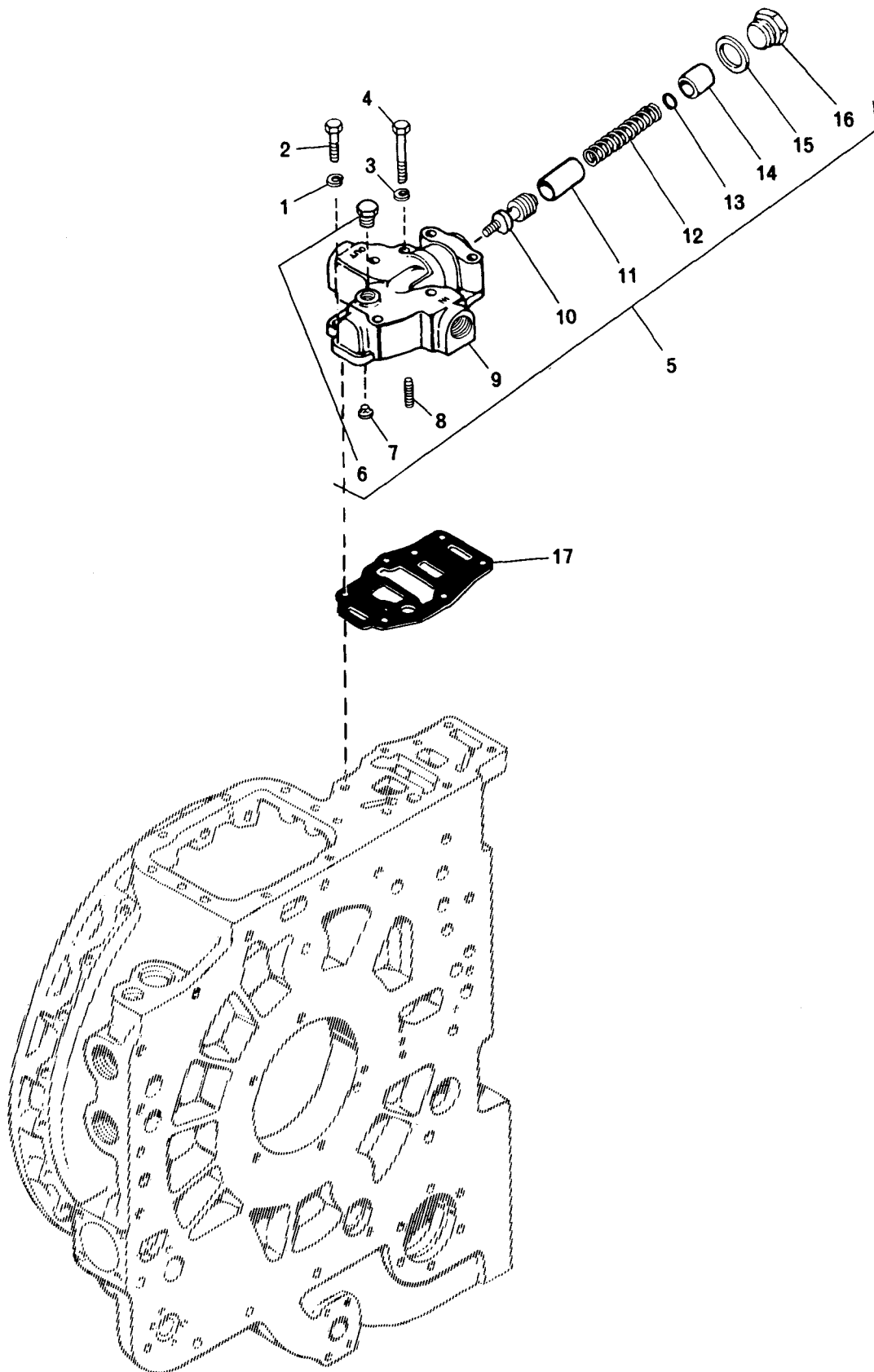
FIG 11 MAIN PRESSURE REGULATOR VALVE AND OIL FILTER
