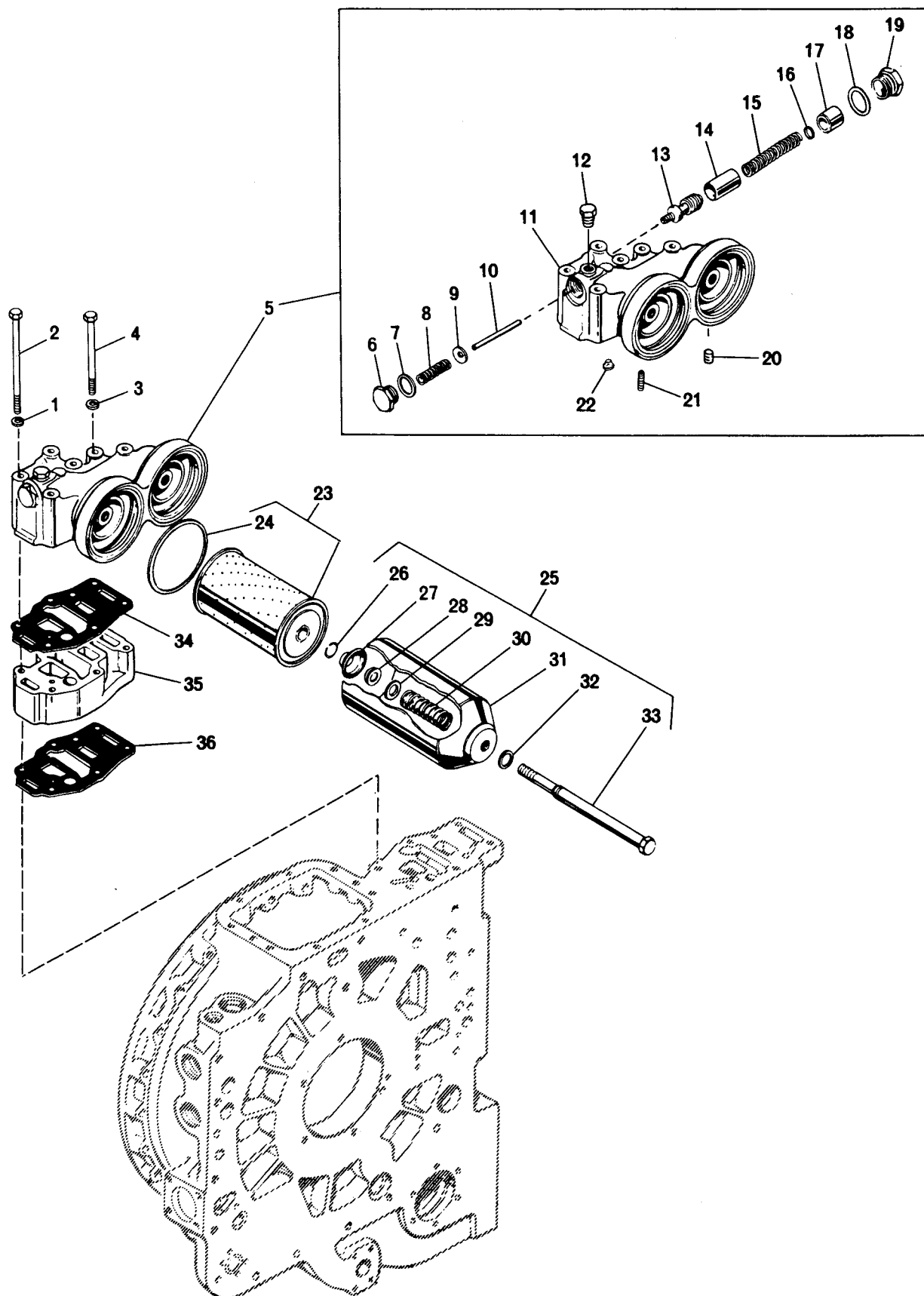
FIG 11-2 MAIN PRESSURE REGULATOR VALVE AND OIL FILTER
