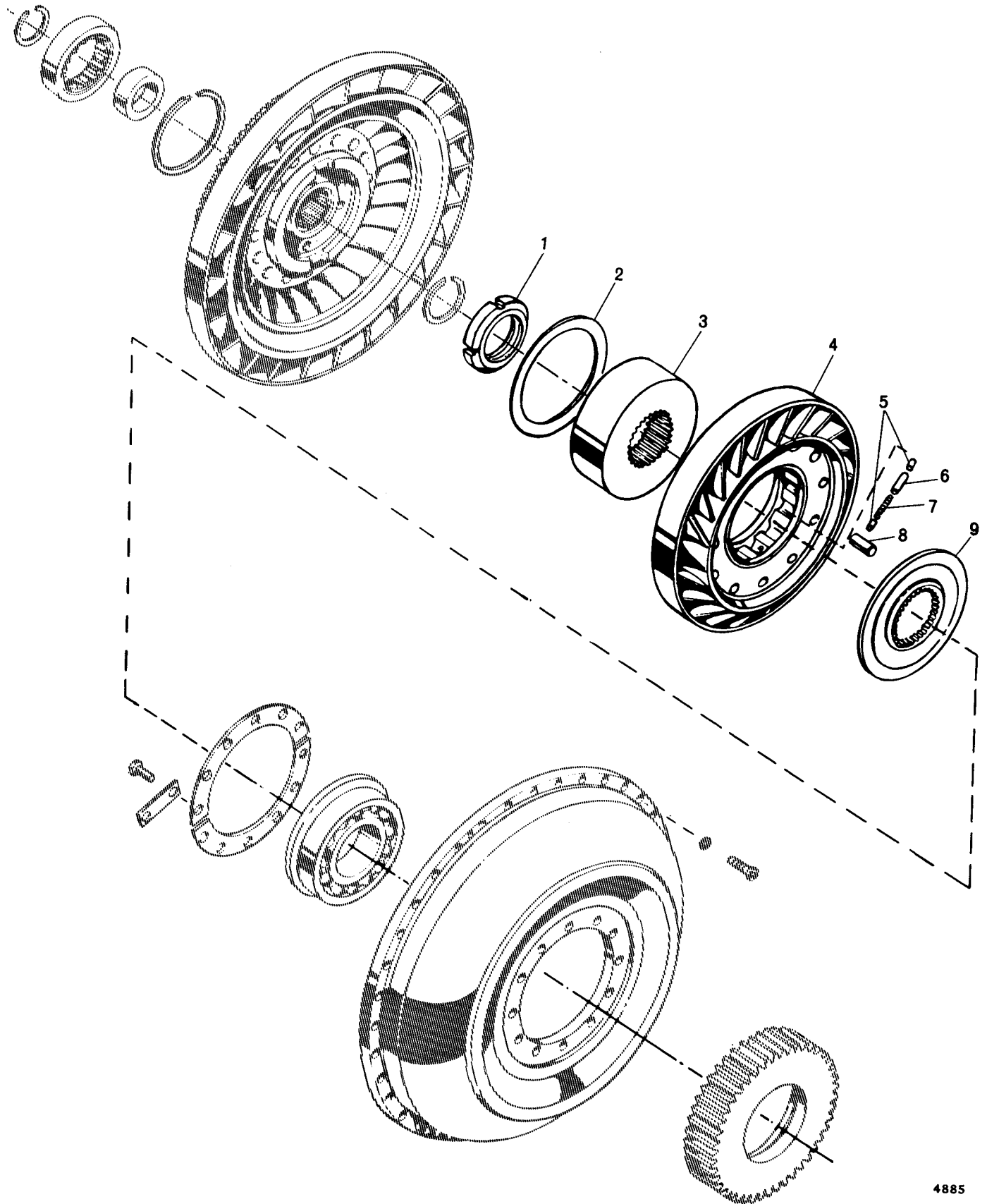
FIG 6-1 STATOR
