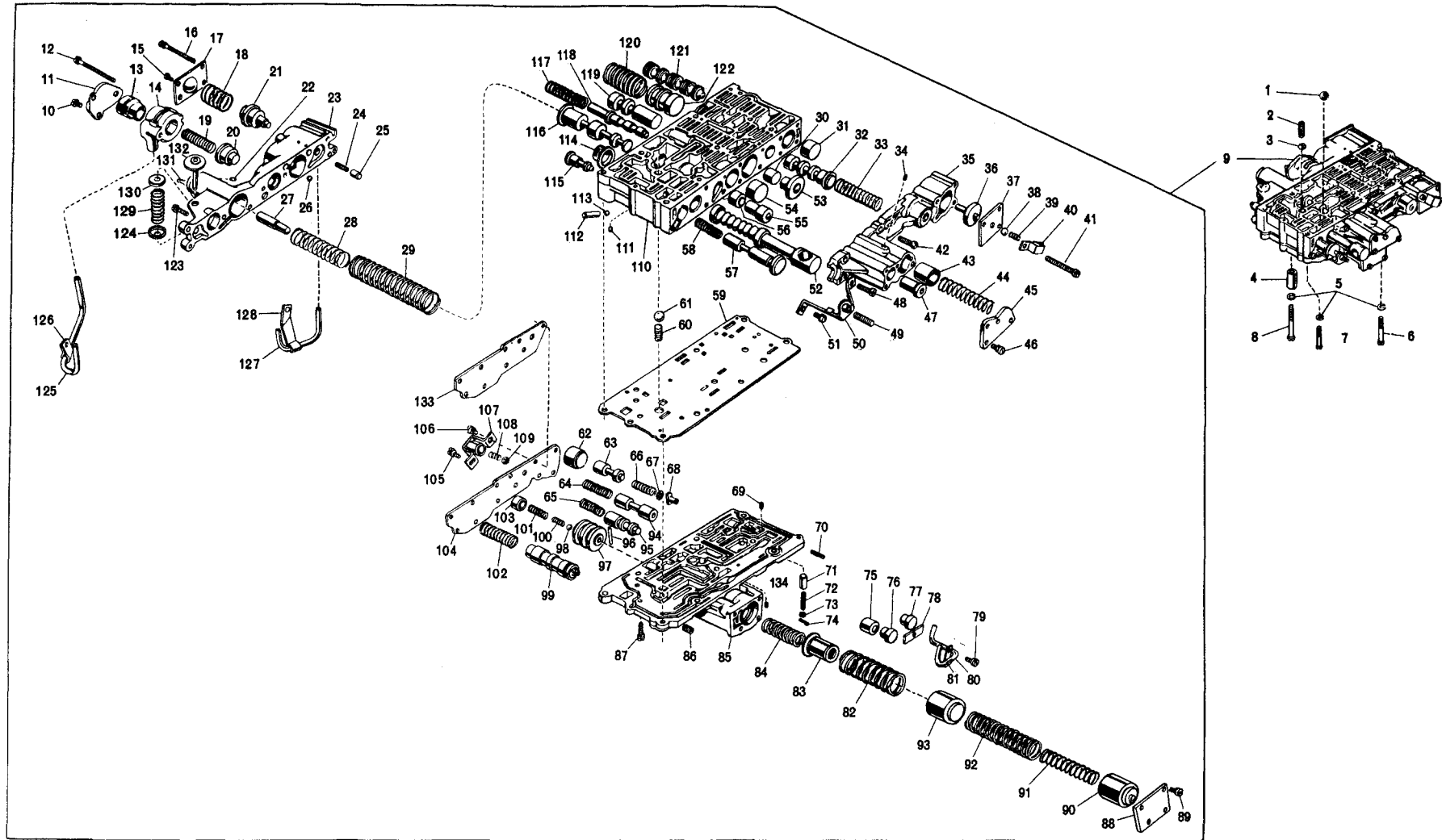
FIG. 11 CONTROL VALVE
