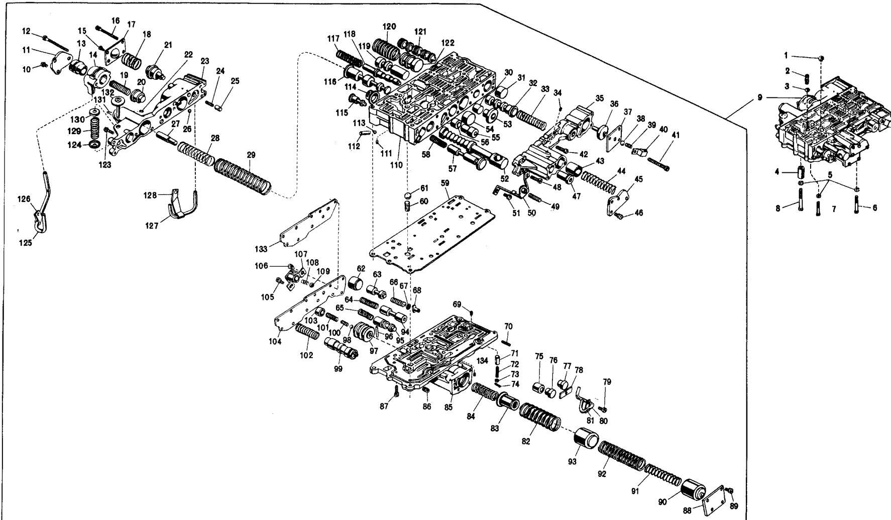
FIG. 11 CONTROL VALVE
