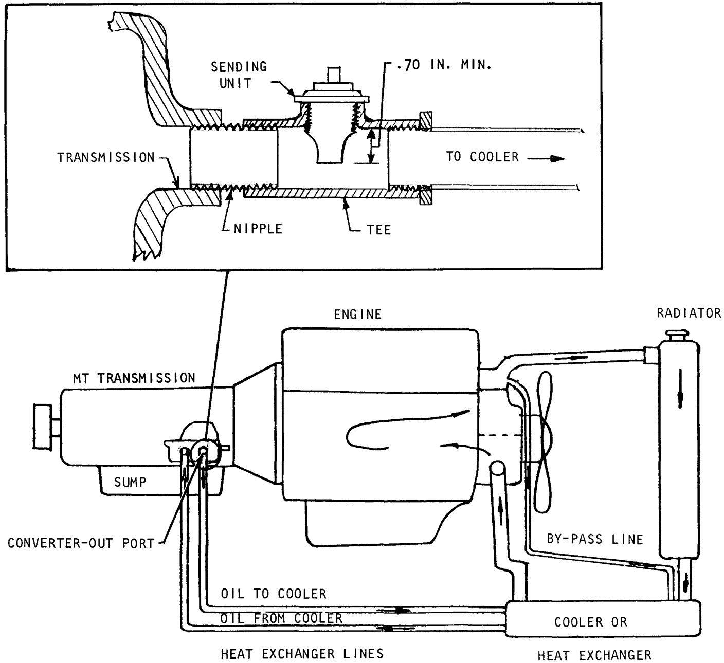
FIG. 2. TYPICAL TEMPERATURE SENDING UNIT INSTALLATION
