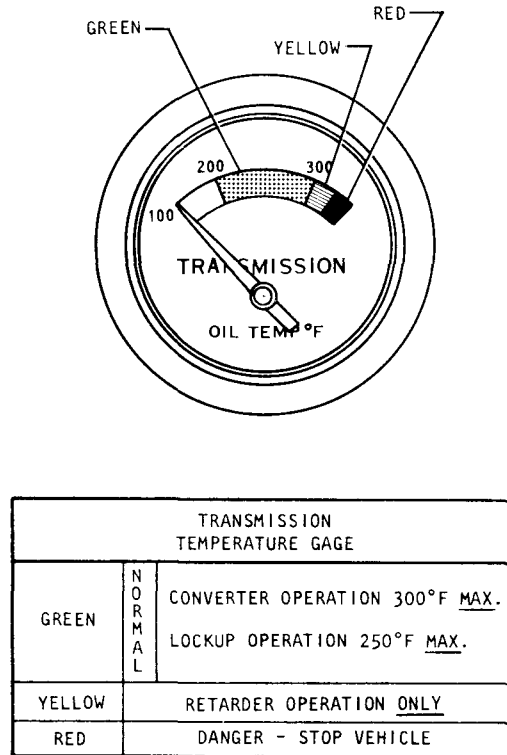
FIG. 1. MT TEMPERATURE GAGE AND DECAL
