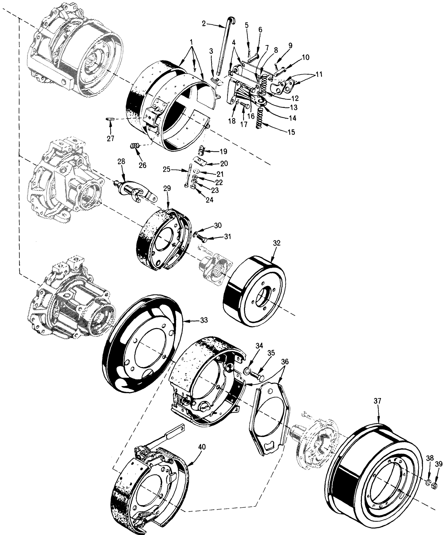
FIG. 9 PARKING BRAKE
