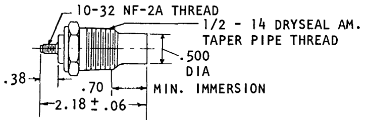
SENDING UNIT
