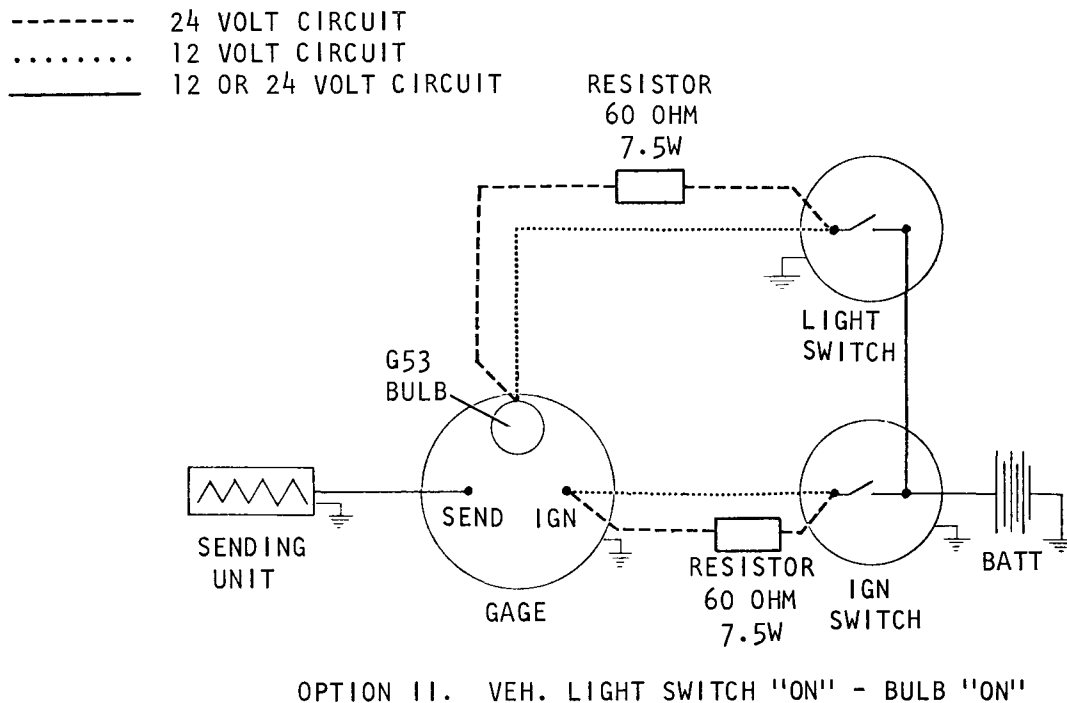
FIG. 4. RECOMMENDED CIRCUIT FOR TEMPERATURE GAGE - 12 OR 24 VOLT SYSTEM
