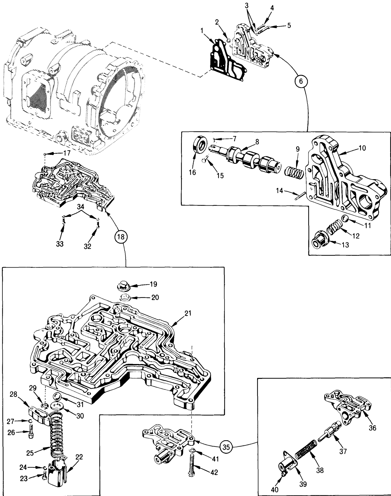
FIG. 10 RETARDER CONTROL VALVE, OIL TRANSFER PLATE AND DOWNSHIFT VALVE
