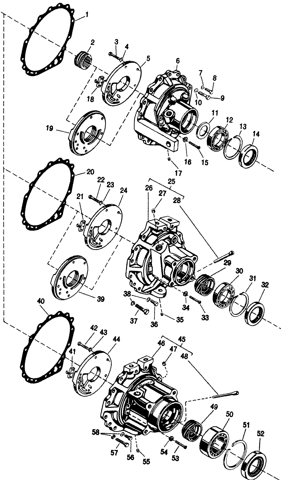
FIG. 8 REAR BEARING RETAINER
