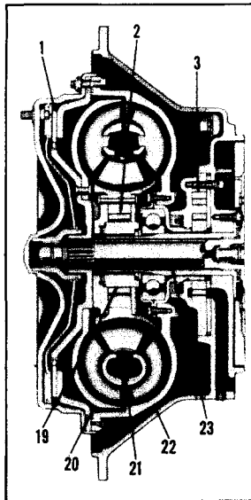
SAE #2 CONVERTER HOUSING OPTION
