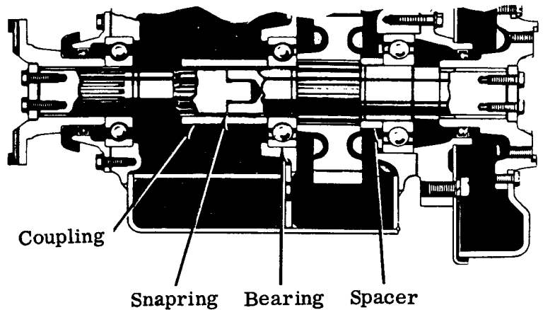
Fig. 2. Standard configuration
