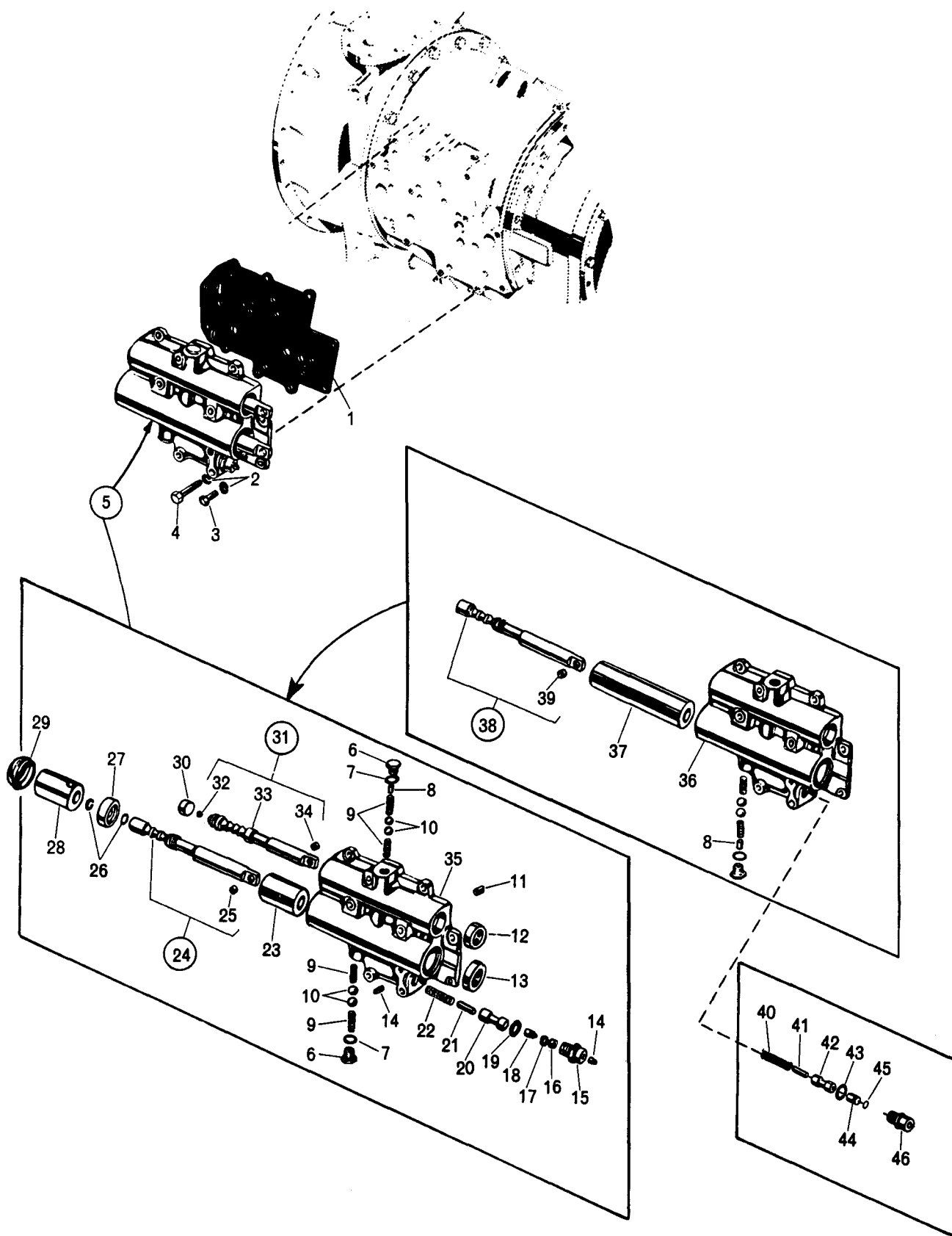
FIG 13-1. CONTROL VALVE BODY
