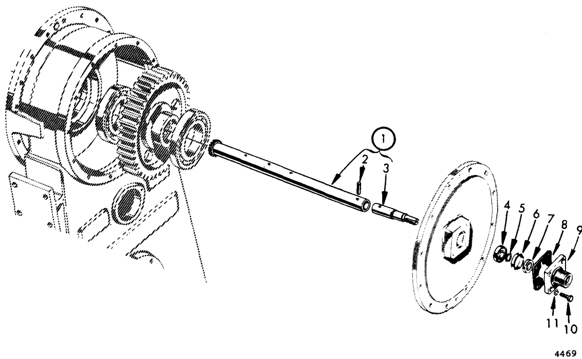
FIG 17. GOVERNOR DRIVE
