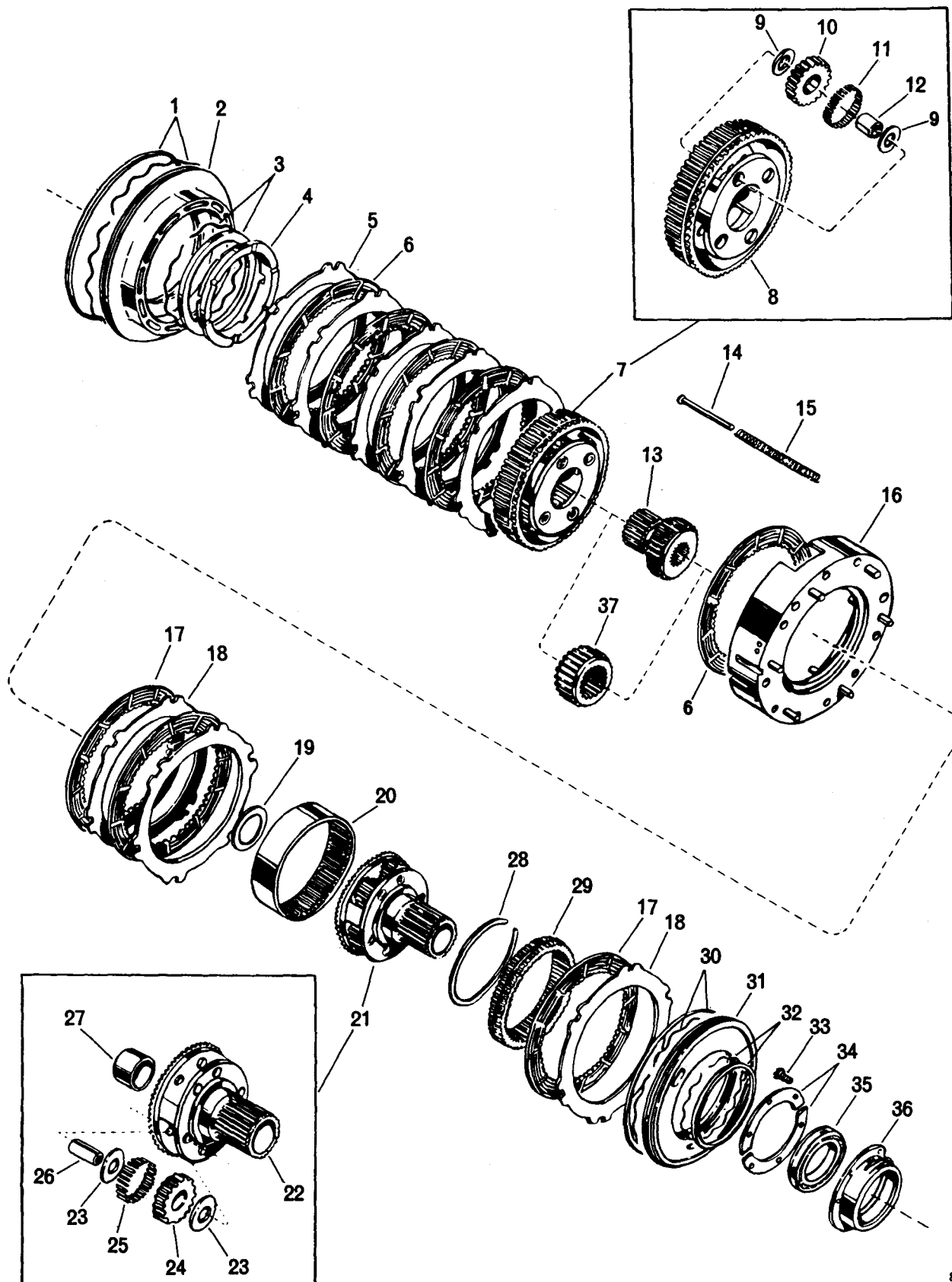
FIG 7. FORWARD AND REVERSE PLANETARIES AND CLUTCHES
