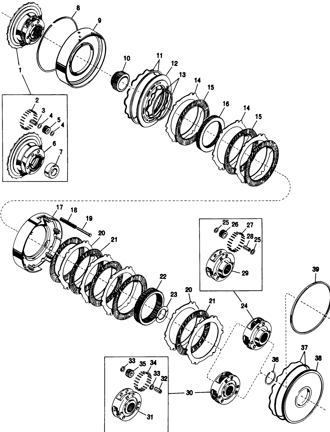
FIG 10. HIGH AND LOW-RANGE PLANETARIES AND CLUTCHES
