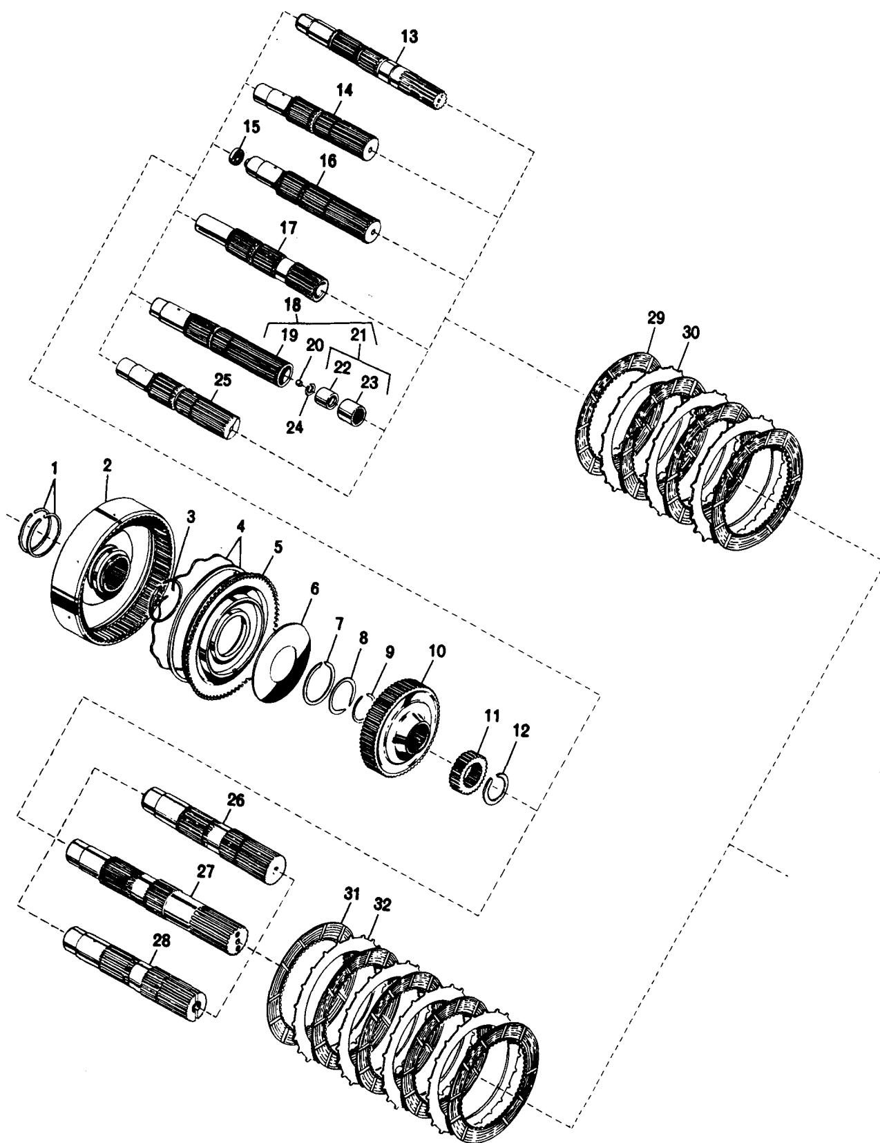
FIG 9. MAIN SHAFT AND INTERMEDIATE-RANGE CLUTCH
